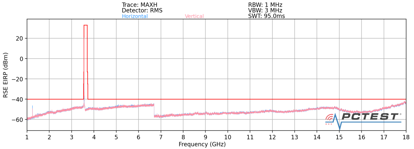
Plot 7-69. Radiated Spurious Plot 1 - 18GHz (Band 48)
