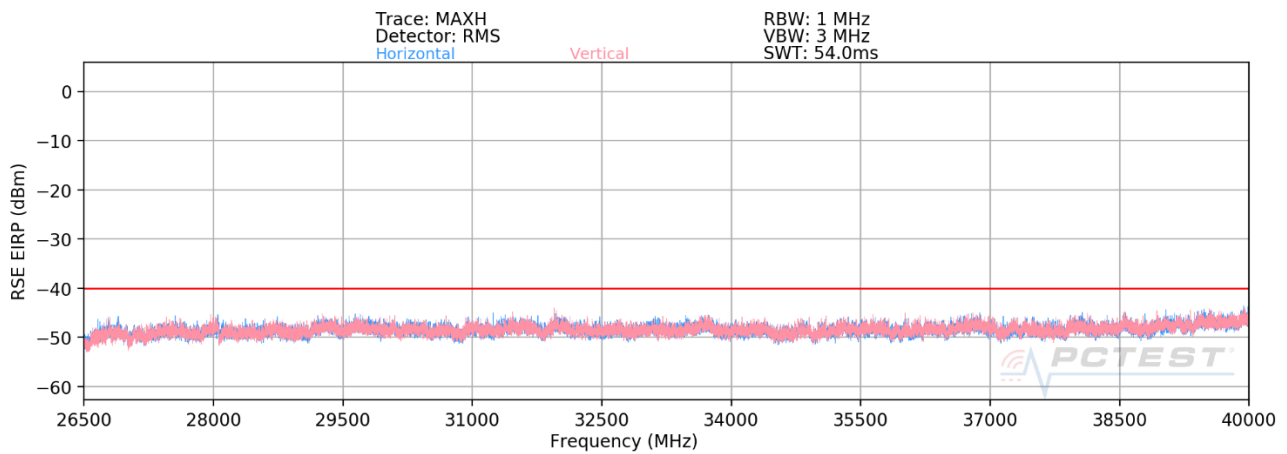
Plot 7-71. Radiated Spurious Plot 26.5 - 40GHz (Band 48)
