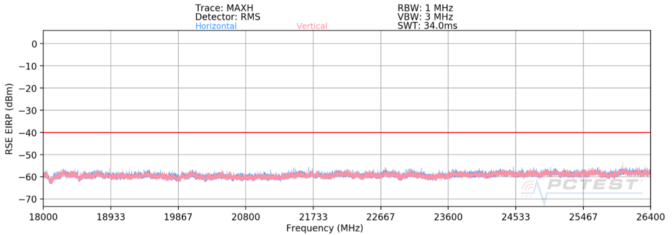
Plot 7-70. Radiated Spurious Plot 18 - 26.5GHz (Band 48)
