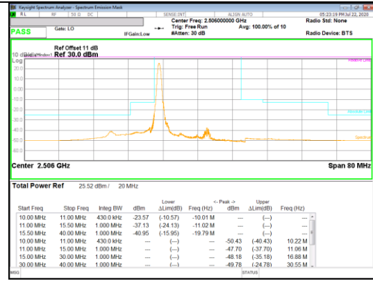
LTE B41 QPSK Low channel 1RB_Offset Low
