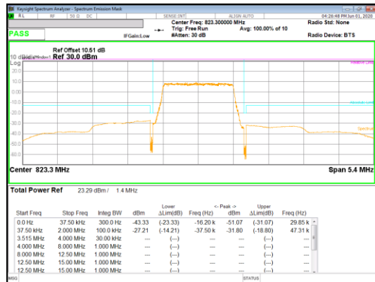
LTE B26 QPSK High channel FRB
