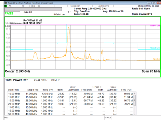
LTE B41 QPSK Mid channel 1RB_Offset Low
