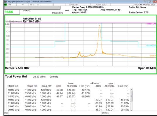
LTE B41 QPSK Low channel 1RB_Offset High
