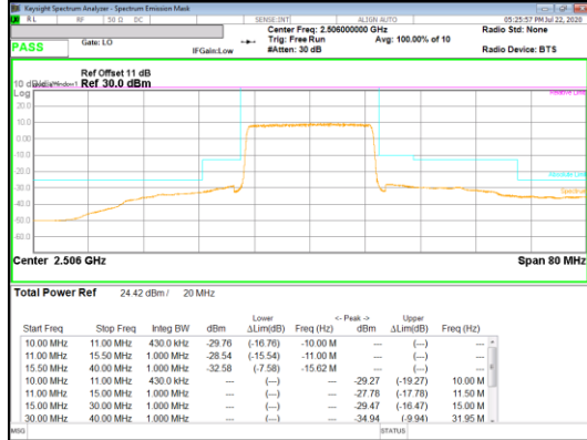
LTE B41 QPSK Low channel FRB
