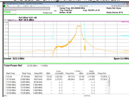
LTE B26 QPSK High channel 1RB_Offset High
