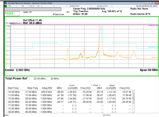
LTE B41 QPSK Mid channel 1RB_Offset High
