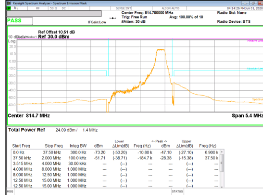
LTE B26 QPSK Low channel 1RB_Offset High
