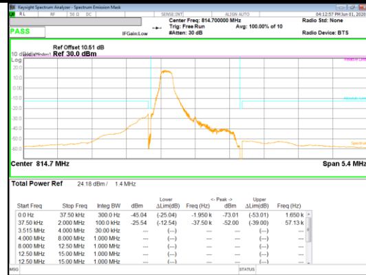
LTE B26 QPSK Low channel 1RB_Offset Low
