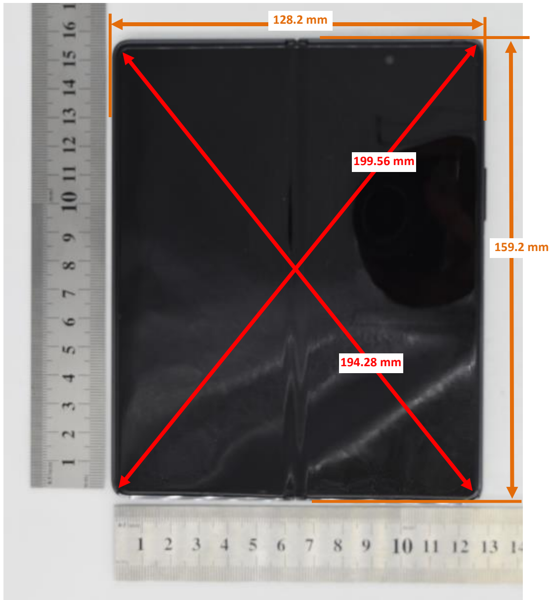
Overall Dimensions DUT Folder Opened
