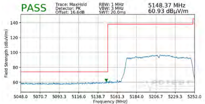
Plot 7-368. Radiated Lower Band Edge Plot MIMO (Peak – UNII Band 1)
