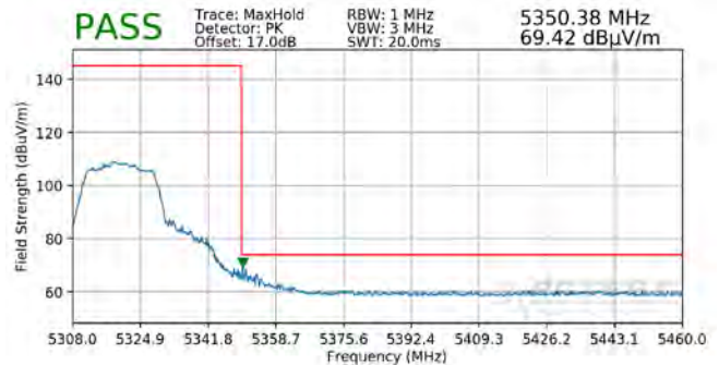
Plot 7-354. Radiated Upper Band Edge Plot MIMO (Peak – UNII Band 2A)
