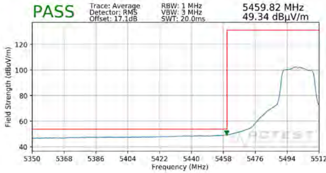
Plot 7-355. Radiated Lower Band Edge Plot MIMO (Average – UNII Band 2C)
