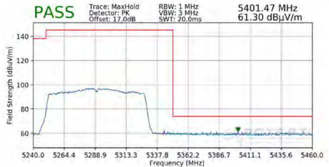
Plot 7-370. Radiated Upper Band Edge Plot MIMO (Peak – UNII Band 2A)
