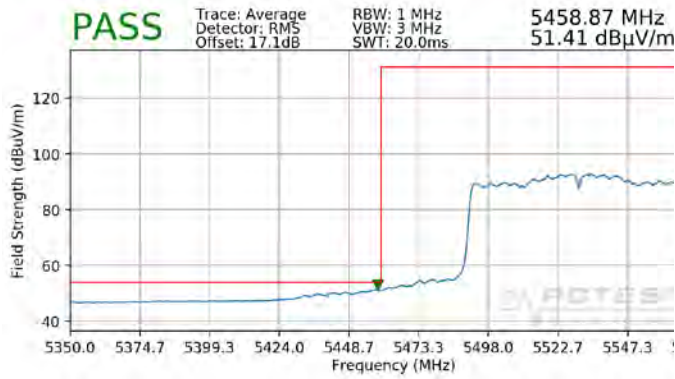
Plot 7-371. Radiated Lower Band Edge Plot MIMO (Average – UNII Band 2C)
