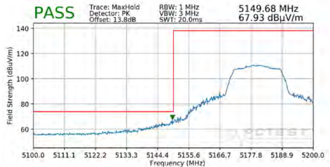
Plot 7-352. Radiated Lower Band Edge Plot MIMO (Peak – UNII Band 1)
