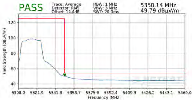
Plot 7-307. Radiated Upper Band Edge Plot SISO ANT1 (Average – UNII Band 2A)
