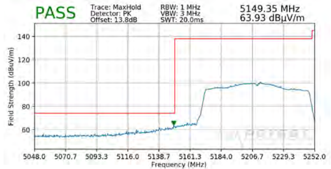
Plot 7-322. Radiated Lower Band Edge Plot SISO ANT1 (Peak – UNII Band 1)
