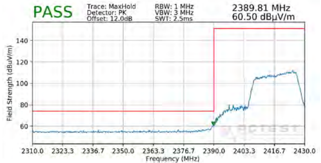
Plot 7-104. Radiated Restricted Lower Band Edge Measurement SISO ANT1 (Peak – 242 Tones)
