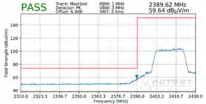
Plot 7-146. Radiated Restricted Lower Band Edge Measurement MIMO (Peak – 242 Tones)
