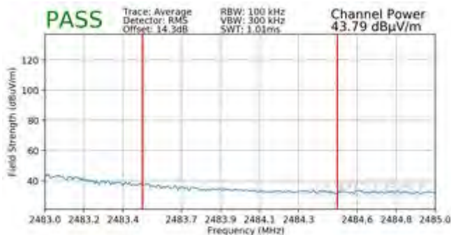
Plot 7-143. Radiated Restricted Upper Band Edge Measurement MIMO (Average – 26 Tones)
