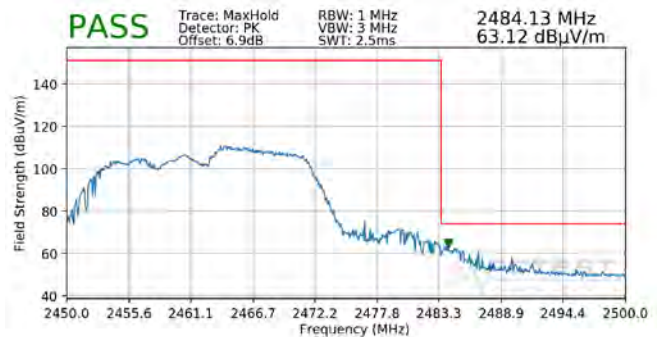
Plot 7-140. Radiated Restricted Upper Band Edge Measurement MIMO (Peak – 106 Tones)
