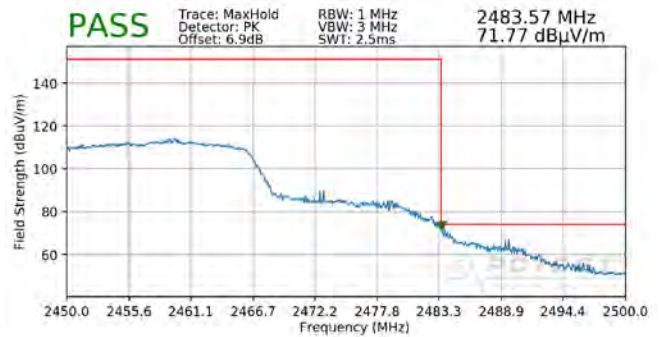
Plot 7-150. Radiated Restricted Upper Band Edge Measurement MIMO (Peak – 242 Tones)
