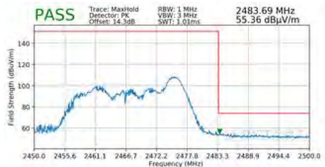
Plot 7-142. Radiated Restricted Upper Band Edge Measurement MIMO (Peak – 26 Tones)
