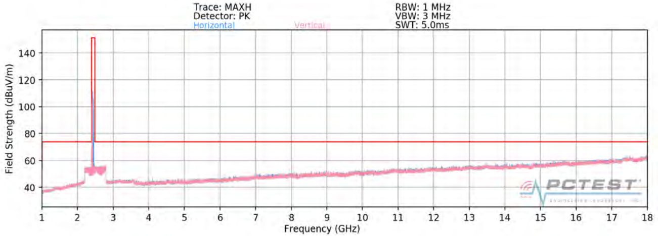
Plot 7-66. Radiated Spurious Plot above 1GHz SISO ANT1 (802.11ax OFDMA – 106 Tones – Ch. 6 – CLOSED)
