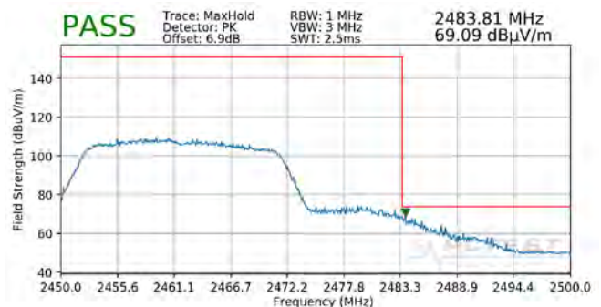
Plot 7-152. Radiated Restricted Upper Band Edge Measurement MIMO (Peak – 242 Tones)
