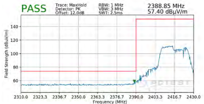
Plot 7-92. Radiated Restricted Lower Band Edge Measurement SISO ANT1 (Peak – 106 Tones)
