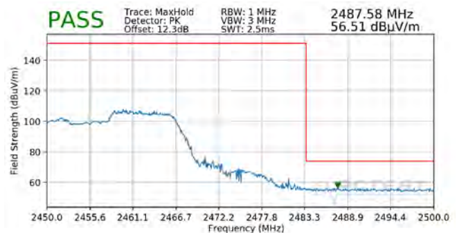
Plot 7-116. Radiated Restricted Upper Band Edge Measurement SISO ANT2 (Peak – 106 Tones)
