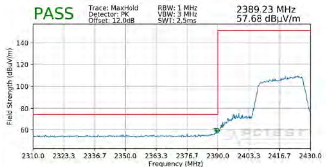
Plot 7-136. Radiated Restricted Lower Band Edge Measurement MIMO (Peak – 106 Tones)
