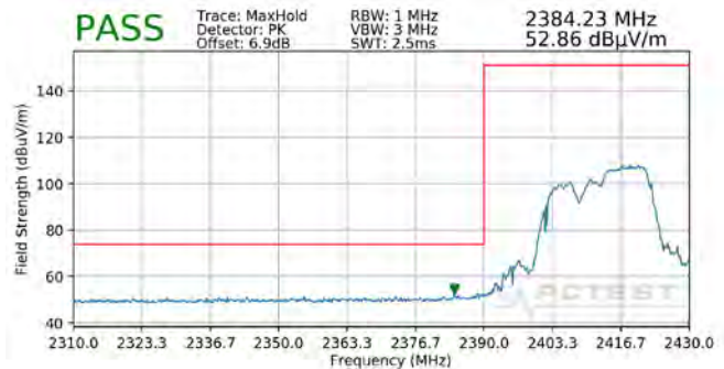
Plot 7-134. Radiated Restricted Lower Band Edge Measurement MIMO (Peak – 106 Tones)
