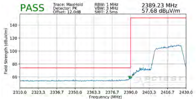
Plot 7-148. Radiated Restricted Lower Band Edge Measurement MIMO (Peak – 242 Tones)
