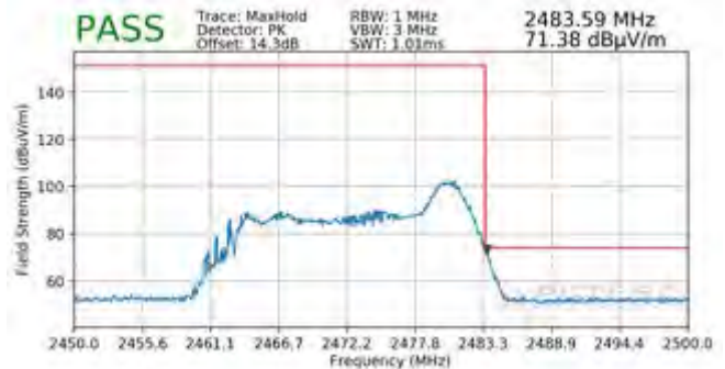
Plot 7-122. Radiated Restricted Upper Band Edge Measurement SISO ANT2 (Peak – 26 Tones)
