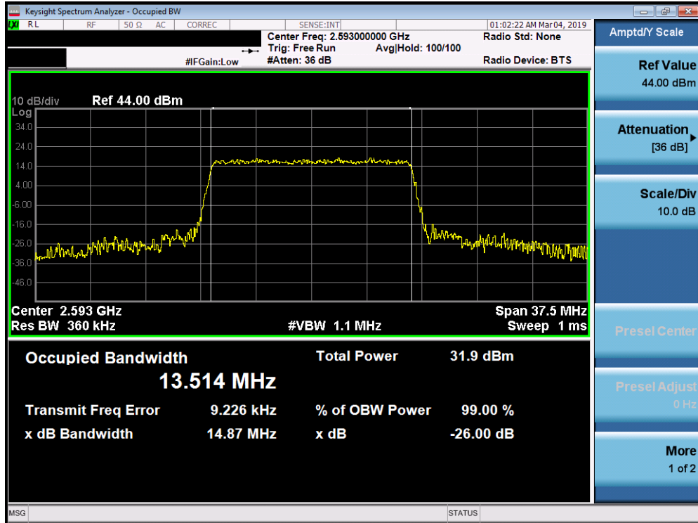
Plot 7-78. Occupied Bandwidth Plot (Band 41 PC3 - 15.0MHz 64-QAM - Full RB Configuration)
