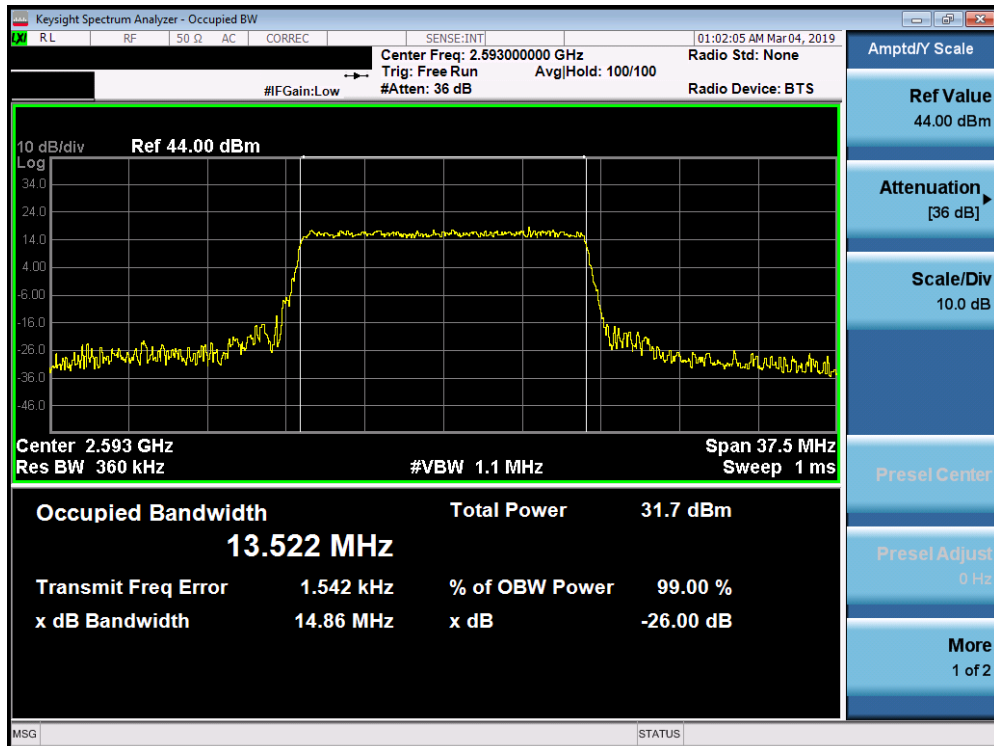
Plot 7-77. Occupied Bandwidth Plot (Band 41 PC3 - 15.0MHz 16-QAM - Full RB Configuration)
