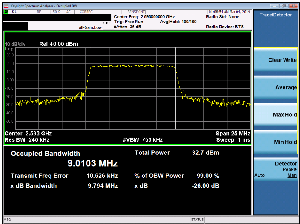
Plot 7-73. Occupied Bandwidth Plot (Band 41 PC3 - 10.0MHz QPSK - Full RB Configuration)
