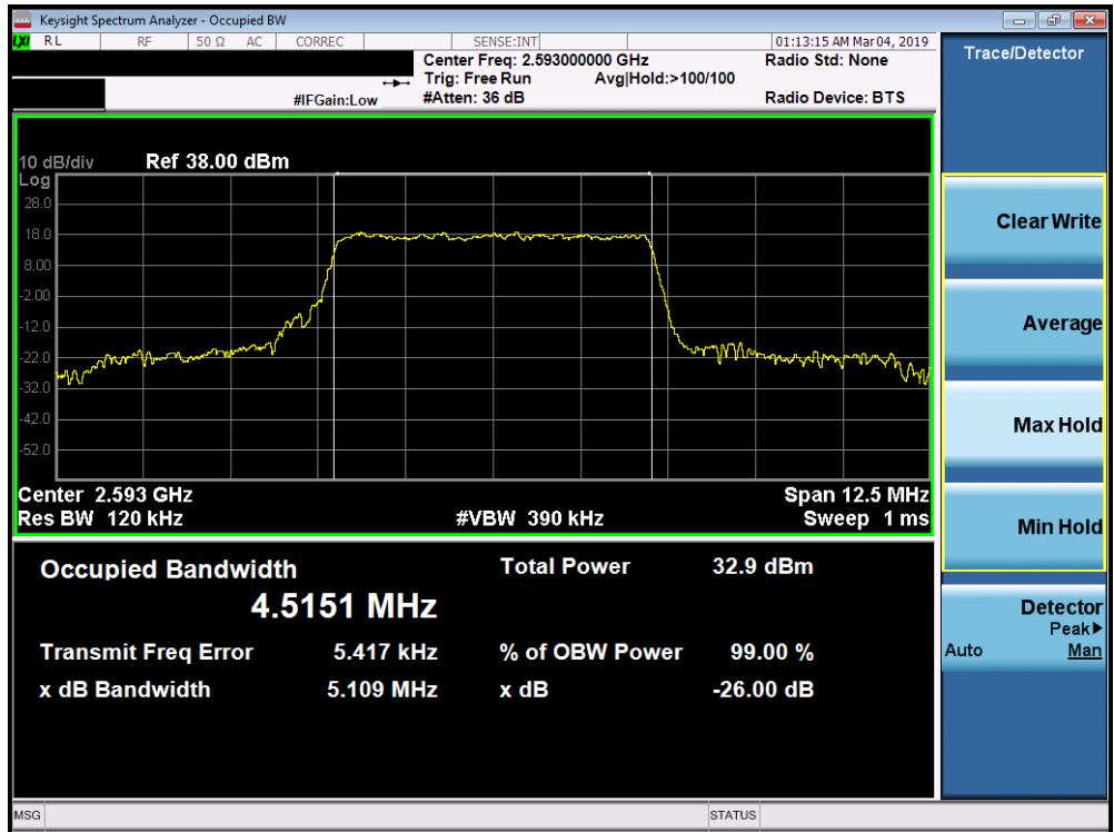
Plot 7-70. Occupied Bandwidth Plot (Band 41 PC3 - 5.0MHz QPSK - Full RB Configuration)
