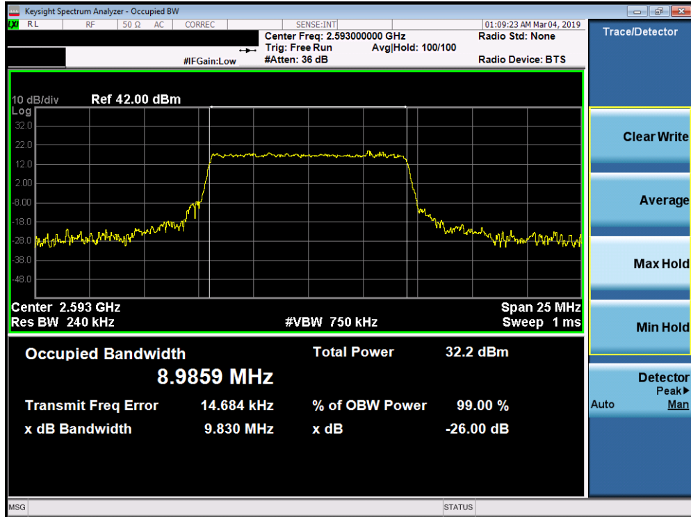
Plot 7-74. Occupied Bandwidth Plot (Band 41 PC3 - 10.0MHz 16-QAM - Full RB Configuration)
