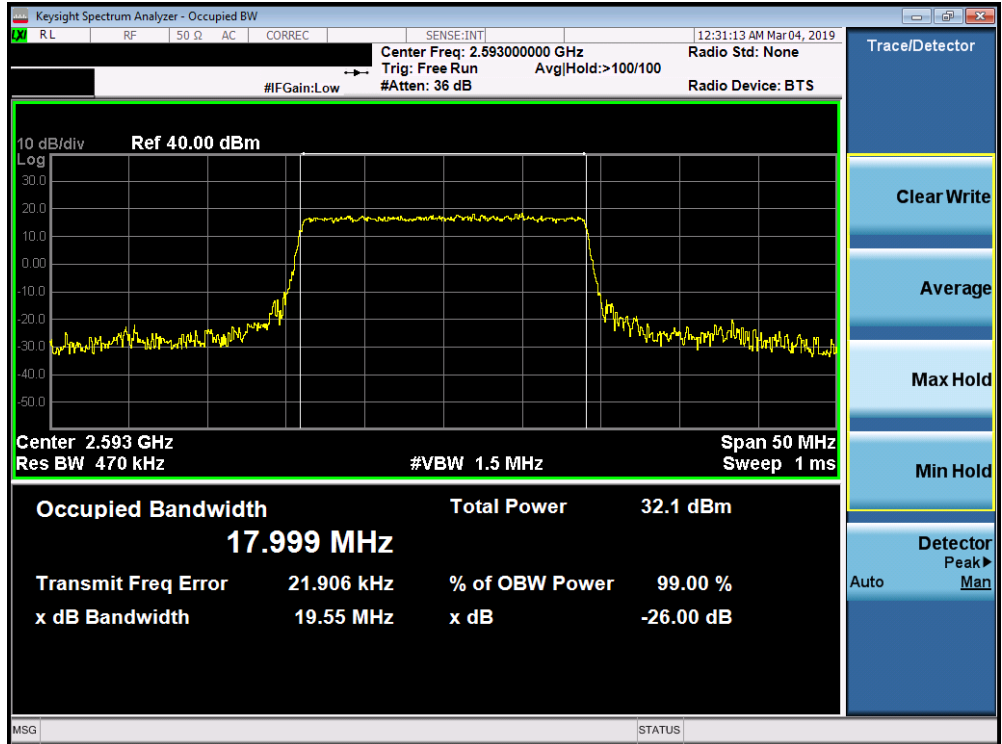
Plot 7-80. Occupied Bandwidth Plot (Band 41 PC3 - 20.0MHz 16-QAM - Full RB Configuration)
