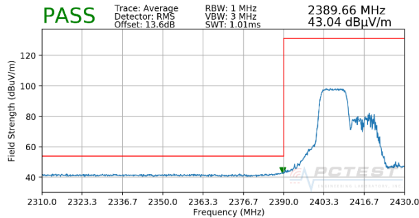
Plot 7-1. Radiated Restricted Lower Band Edge Measurement SISO ANT2 (Average – 106 Tones - OPEN)
