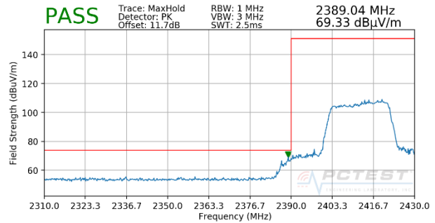
Plot 7-22. Radiated Restricted Lower Band Edge Measurement MIMO (Peak – 242 Tones - OPEN)
