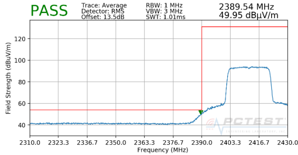
Plot 7-9. Radiated Restricted Lower Band Edge Measurement SISO ANT2 (Average – 242 Tones - OPEN)
