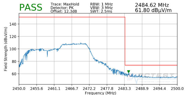
Plot 7-4. Radiated Restricted Upper Band Edge Measurement SISO ANT2 (Peak – 106 Tones - OPEN)
