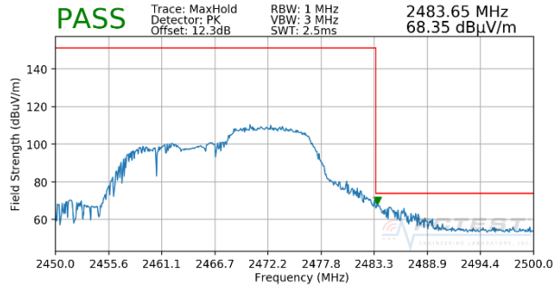
Plot 7-6. Radiated Restricted Upper Band Edge Measurement SISO ANT2 (Peak – 106 Tones - OPEN)
