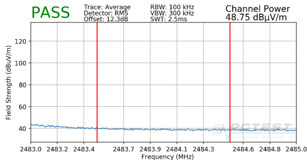
Plot 7-15. Radiated Restricted Upper Band Edge Measurement SISO ANT2 (Average – 242 Tones - OPEN)
