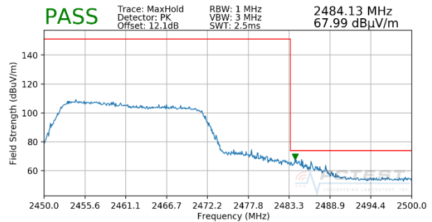
Plot 7-24. Radiated Restricted Upper Band Edge Measurement MIMO (Peak – 242 Tones - OPEN)
