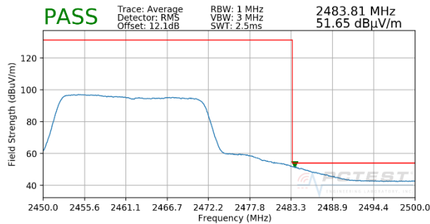
Plot 7-23. Radiated Restricted Upper Band Edge Measurement MIMO (Average – 242 Tones - OPEN)
