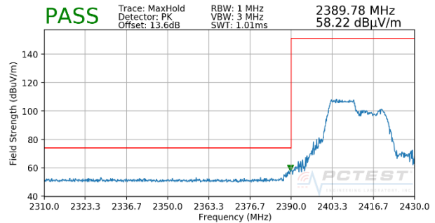
Plot 7-2. Radiated Restricted Lower Band Edge Measurement SISO ANT2 (Peak – 106 Tones - OPEN)
