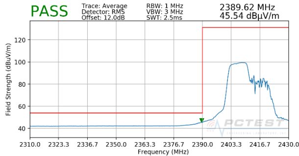
Plot 7-17. Radiated Restricted Lower Band Edge Measurement MIMO (Average – 106 Tones - OPEN)
