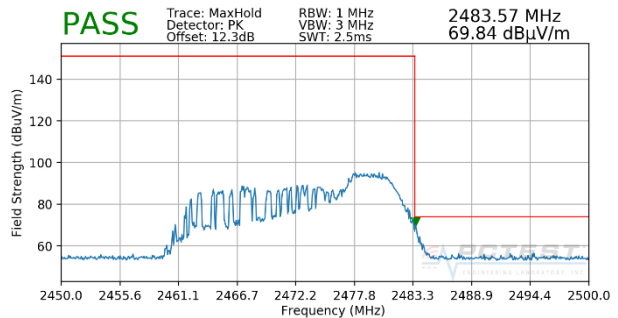
Plot 7-8. Radiated Restricted Upper Band Edge Measurement SISO ANT2 (Peak – 26 Tones - OPEN)
