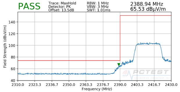
Plot 7-10. Radiated Restricted Lower Band Edge Measurement SISO ANT2 (Peak – 242 Tones - OPEN)
