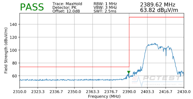
Plot 7-18. Radiated Restricted Lower Band Edge Measurement MIMO (Peak – 106 Tones - OPEN)
