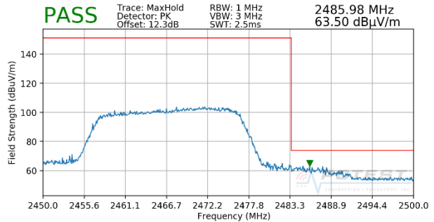
Plot 7-14. Radiated Restricted Upper Band Edge Measurement SISO ANT2 (Peak – 242 Tones - OPEN)
