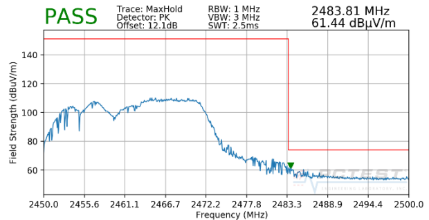
Plot 7-20. Radiated Restricted Upper Band Edge Measurement MIMO (Peak – 106 Tones - OPEN)
