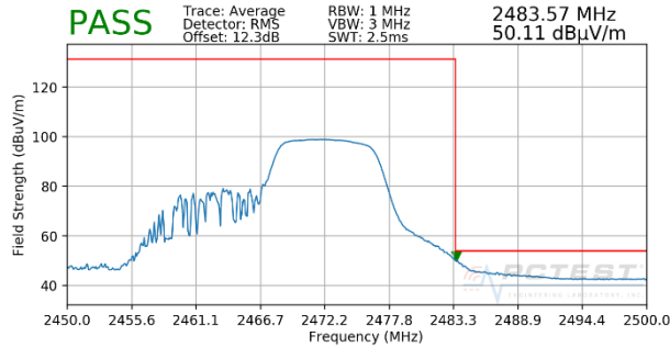
Plot 7-5. Radiated Restricted Upper Band Edge Measurement SISO ANT2 (Average – 106 Tones - OPEN)
