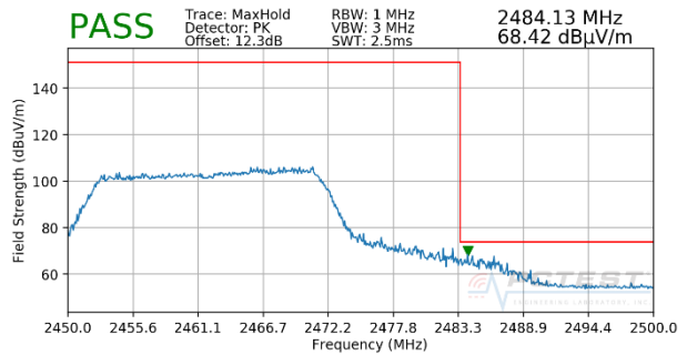
Plot 7-12. Radiated Restricted Upper Band Edge Measurement SISO ANT2 (Peak – 242 Tones - OPEN)
