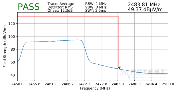
Plot 7-11. Radiated Restricted Upper Band Edge Measurement SISO ANT2 (Average – 242 Tones - OPEN)
