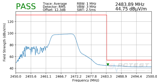
Plot 7-3. Radiated Restricted Upper Band Edge Measurement SISO ANT2 (Average – 106 Tones - OPEN)
