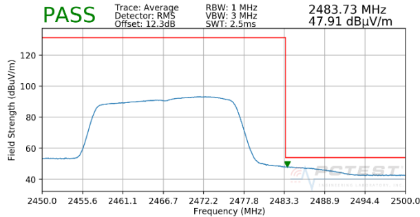
Plot 7-13. Radiated Restricted Upper Band Edge Measurement SISO ANT2 (Average – 242 Tones - OPEN)
