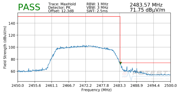
Plot 7-16. Radiated Restricted Upper Band Edge Measurement SISO ANT2 (Peak – 242 Tones - OPEN)
