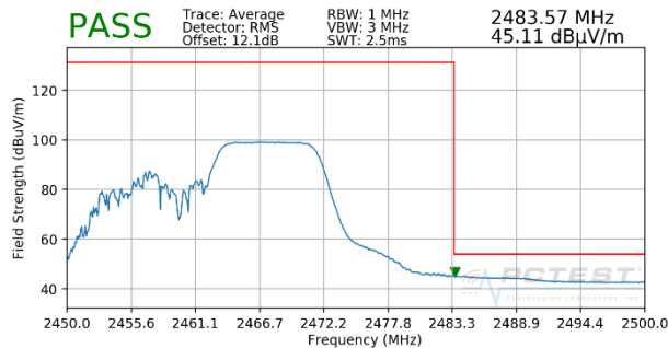
Plot 7-19. Radiated Restricted Upper Band Edge Measurement MIMO (Average – 106 Tones - OPEN)
