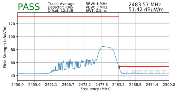
Plot 7-7. Radiated Restricted Upper Band Edge Measurement SISO ANT2 (Average – 26 Tones - OPEN)
