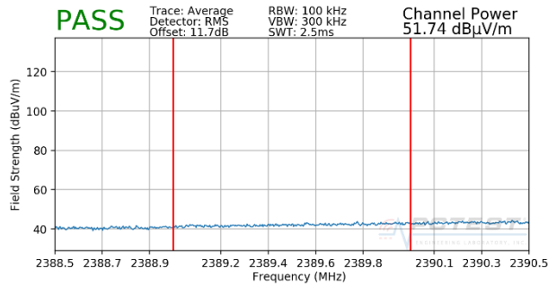
Plot 7-21. Radiated Restricted Lower Band Edge Measurement MIMO (Average – 242 Tones - OPEN)
