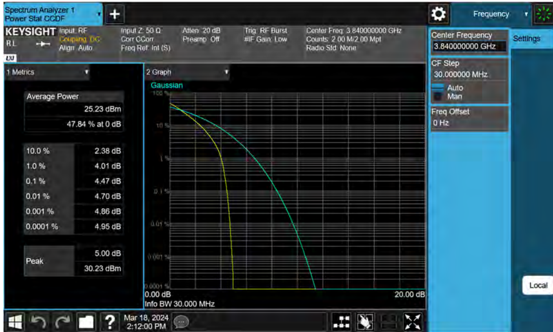
n77(3700~3980 MHz)_30 M_PAR_Mid_QPSK_FullRB
