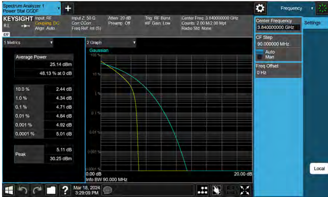
n77(3700~3980 MHz)_90 M_PAR_Mid_QPSK_FullRB
