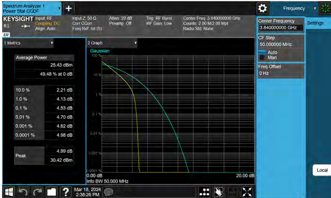
n77(3700~3980 MHz)_50 M_PAR_Mid_QPSK_FullRB
