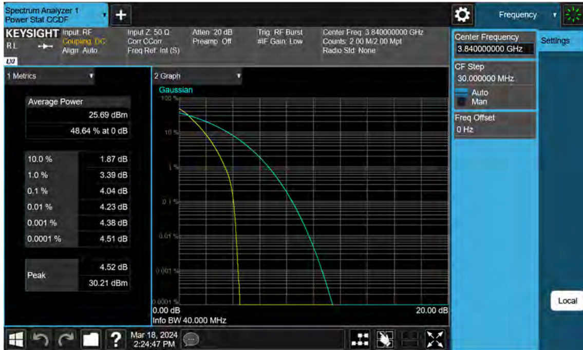
n77(3700~3980 MHz)_40 M_PAR_Mid_BPSK_FullRB
