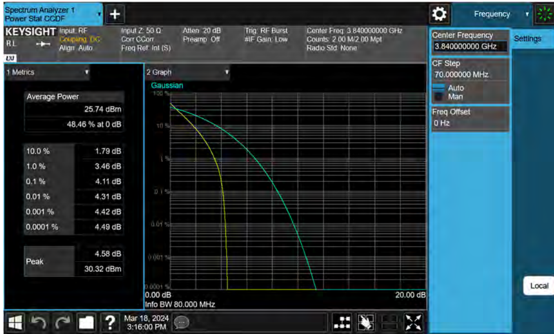
n77(3700~3980 MHz)_80 M_PAR_Mid_BPSK_FullRB
