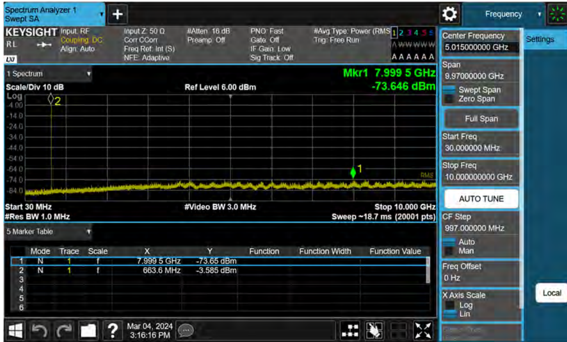
Sub6 n71. Conducted Spurious Plot _ (133600ch_10 MHz_BPSK_RB 1_1)
