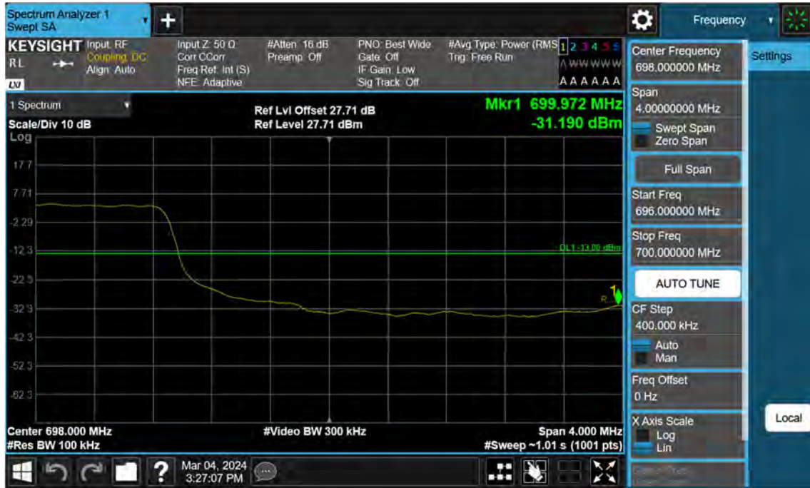
Sub6 n71. Upper Band Edge Plot (15 M BW Ch.138100 BPSK_ Full RB)
