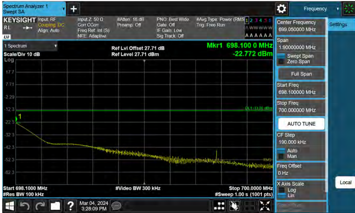
Sub6 n71. Upper Band Edge Plot (15 M BW Ch.138100 BPSK_RB1_Offset 78)_2
