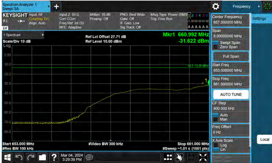
Sub6 n71. Lower Extended Band Edge Plot (20 M BW Ch.134600 BPSK_ Full RB)
