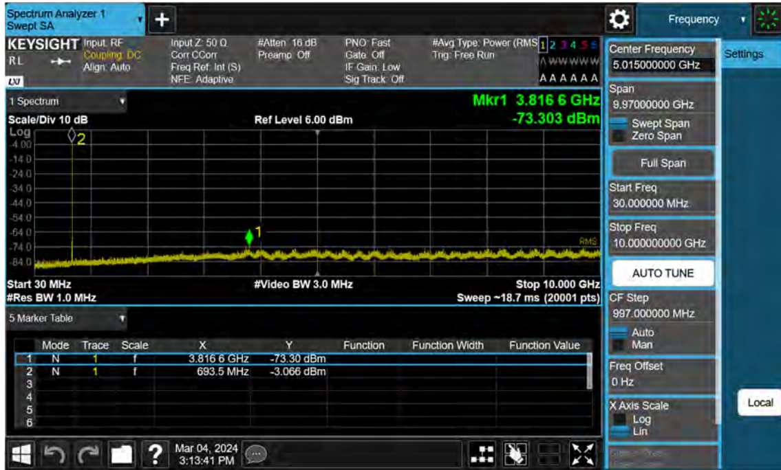
Sub6 n71. Conducted Spurious Plot_ (139100ch_5 MHz_BPSK_RB 1_1)
