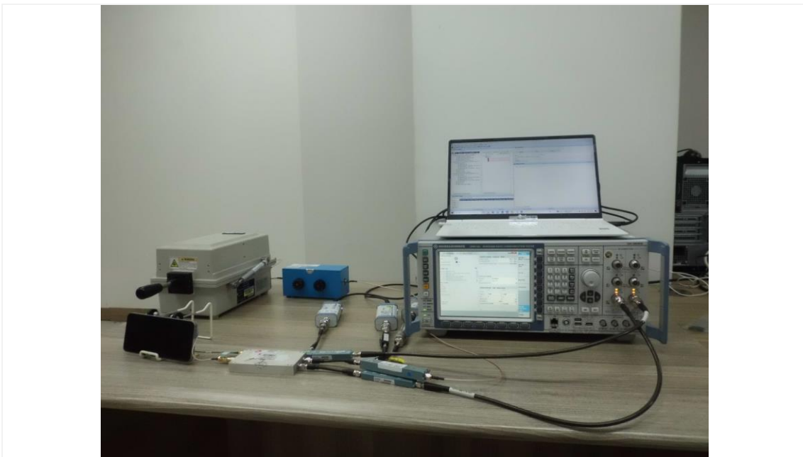
Test setup photo-8 (8-1(f) System level compliance)
