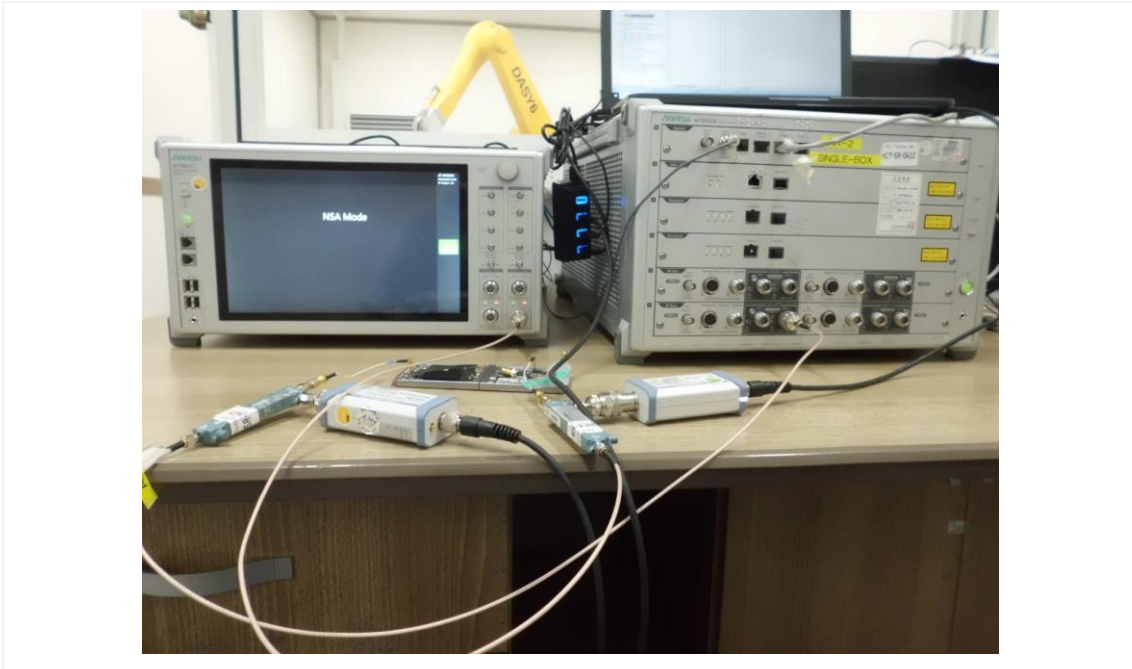
Test setup photo-5 (8-1(c) 5G Sub 6 NSA)
