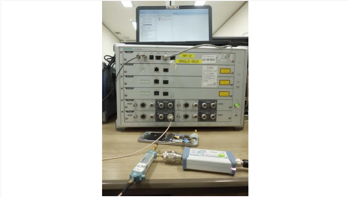
Test setup photo-3 (8-1(a) 5G Sub 6)
