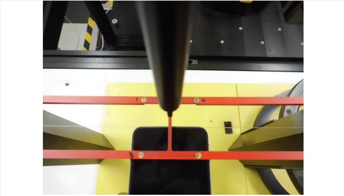
Test setup photo_Front
