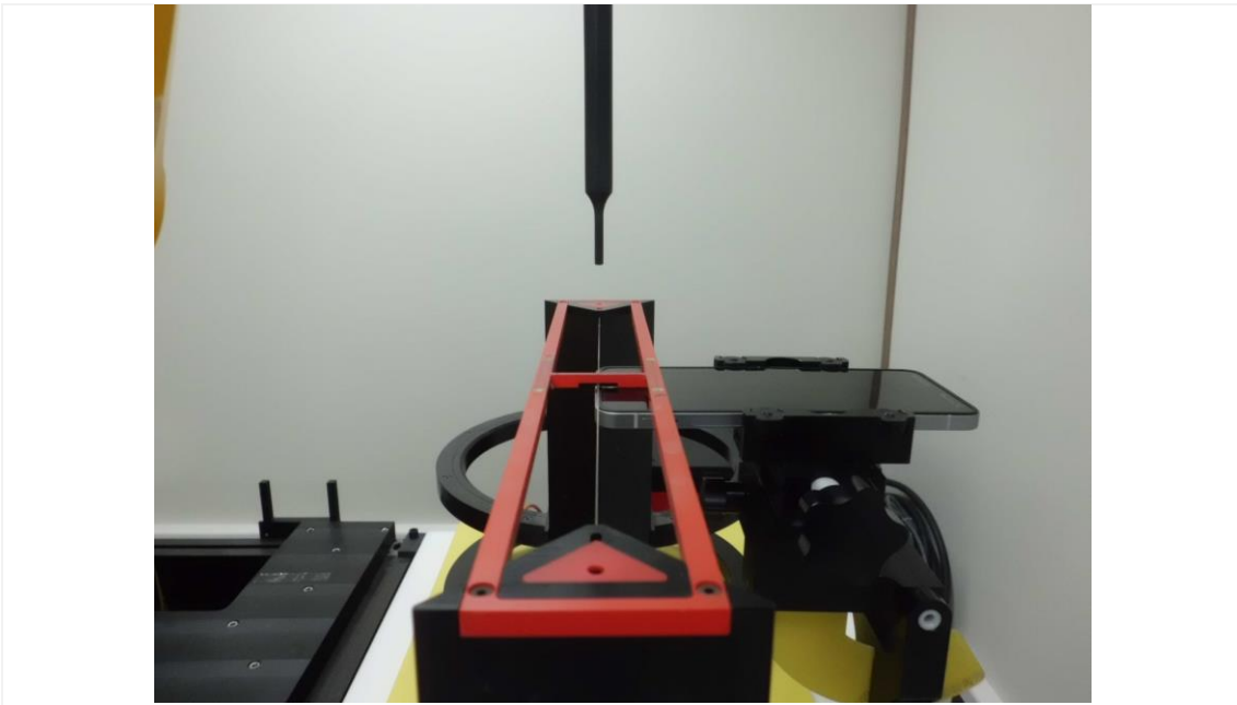
Test setup photo_Side
