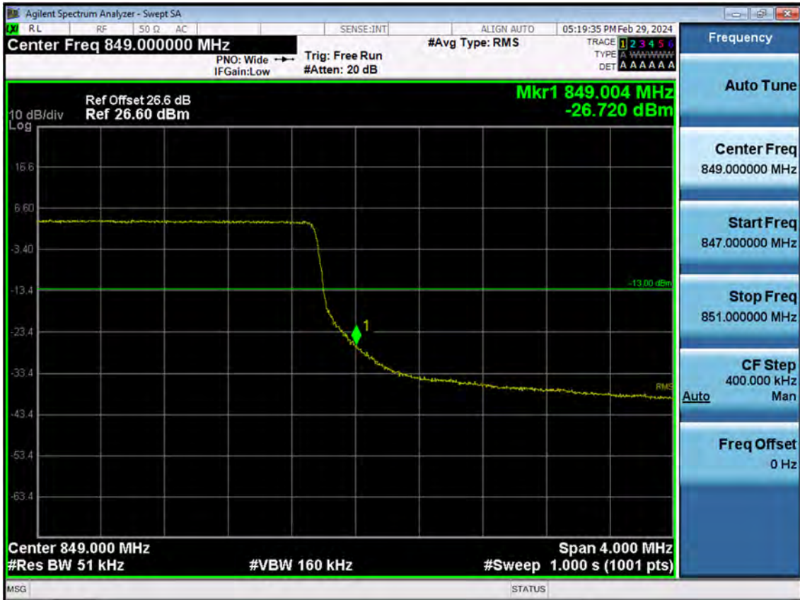
BAND5/26. Upper Band Edge Plot (5 M BW Ch.27015 QPSK_RB25_Offset 0)
