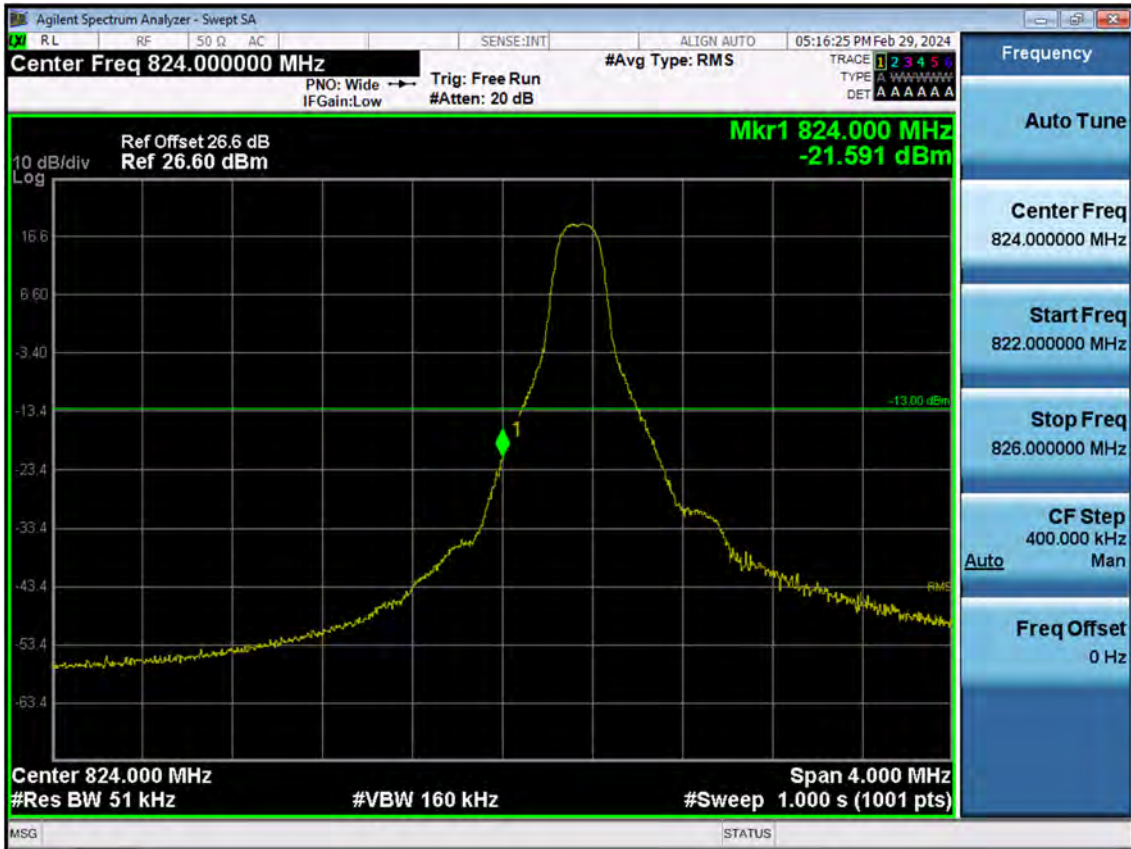
BAND5/26. Lower Band Edge Plot (5 M BW Ch.26815 QPSK_RB1_Offset 0)
