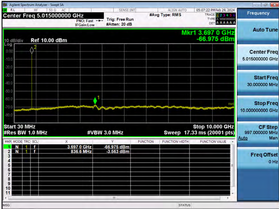
BAND5/26. Conducted Spurious Plot (26915ch_1.4 MHz_QPSK_RB 1_0)
