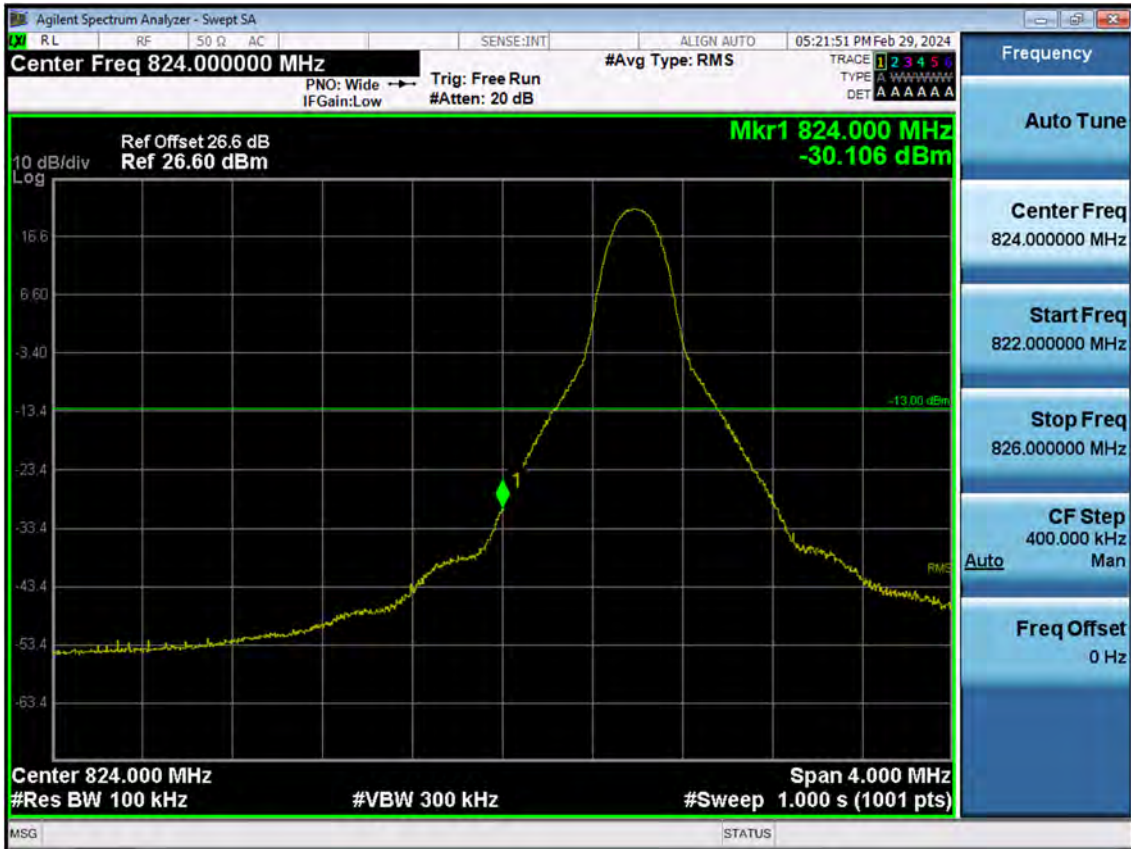
BAND5/26. Lower Band Edge Plot (10 M BW Ch.26840 QPSK_RB1_Offset 0)
