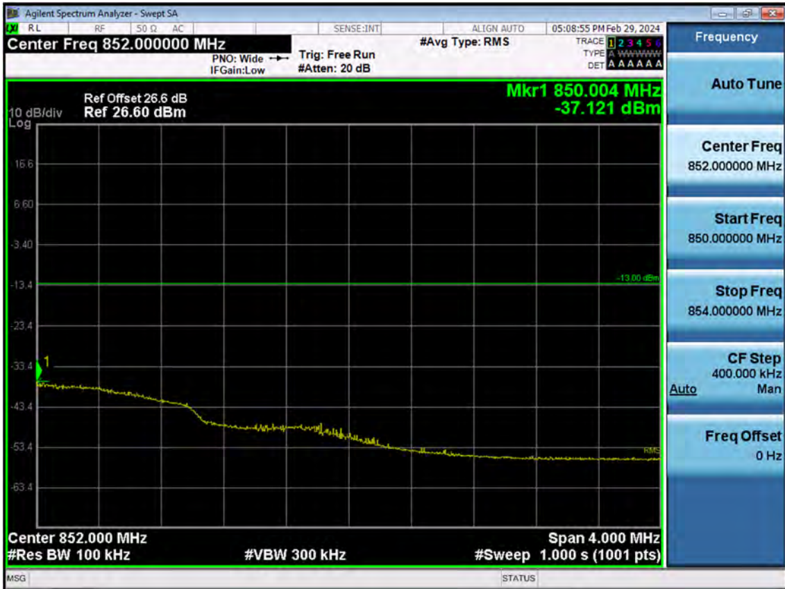
BAND5/26. Upper Extended Band Edge Plot (1.4 M BW Ch.27033 QPSK_RB6_0)
