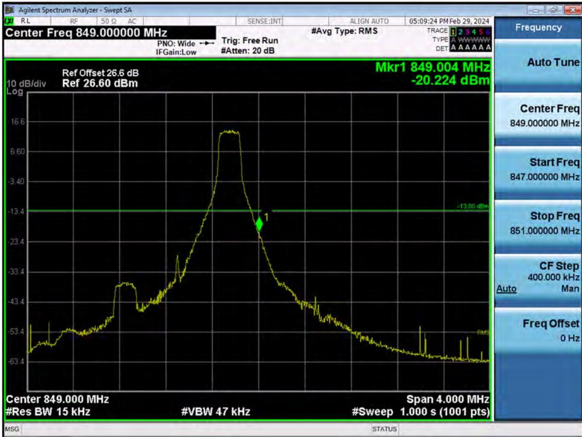
BAND5/26. Upper Band Edge Plot (1.4 M BW Ch.27033 QPSK_RB1_Offset 5)
