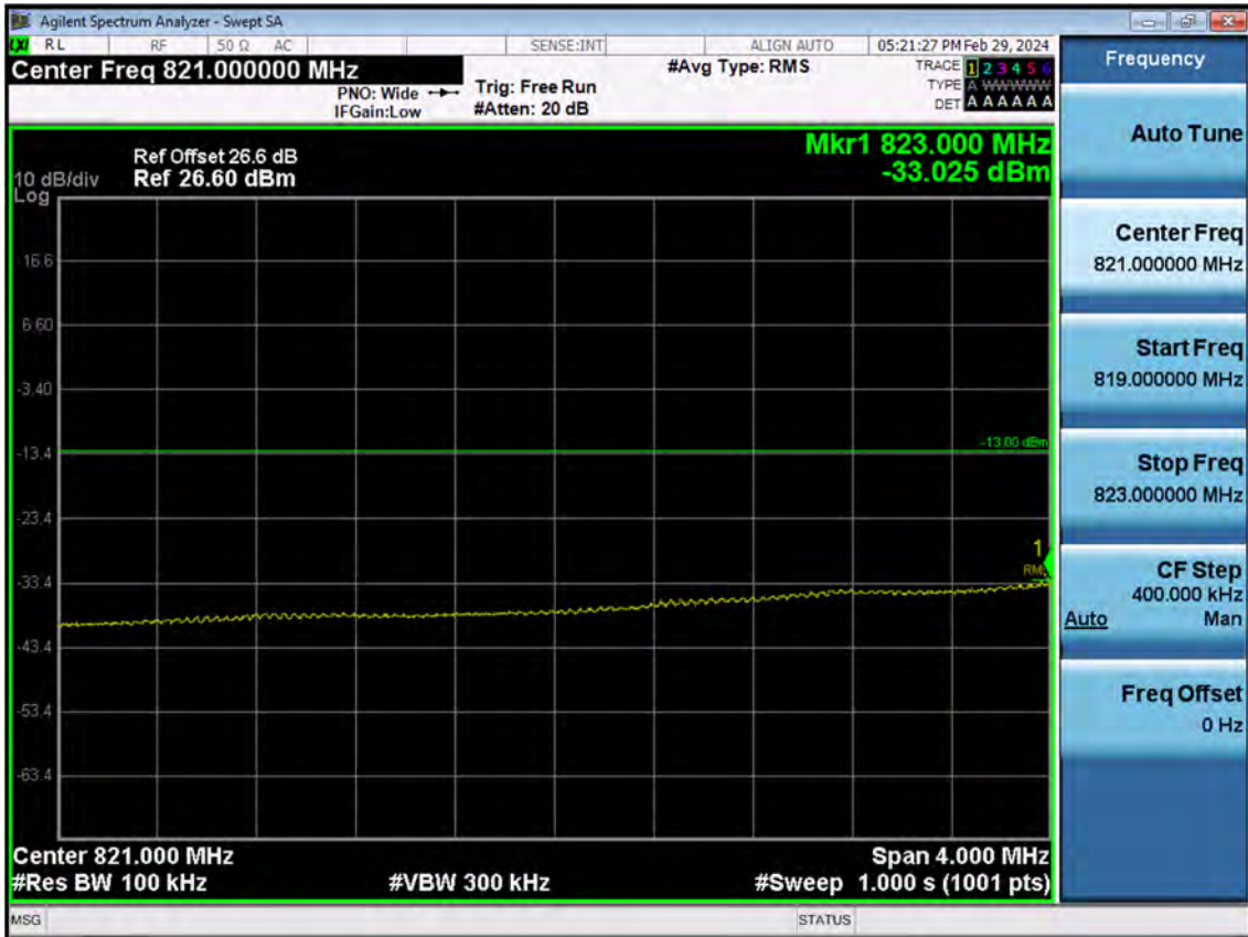
BAND5/26. Lower Extended Band Edge Plot (10 M BW Ch.26840 QPSK_RB50_0)
