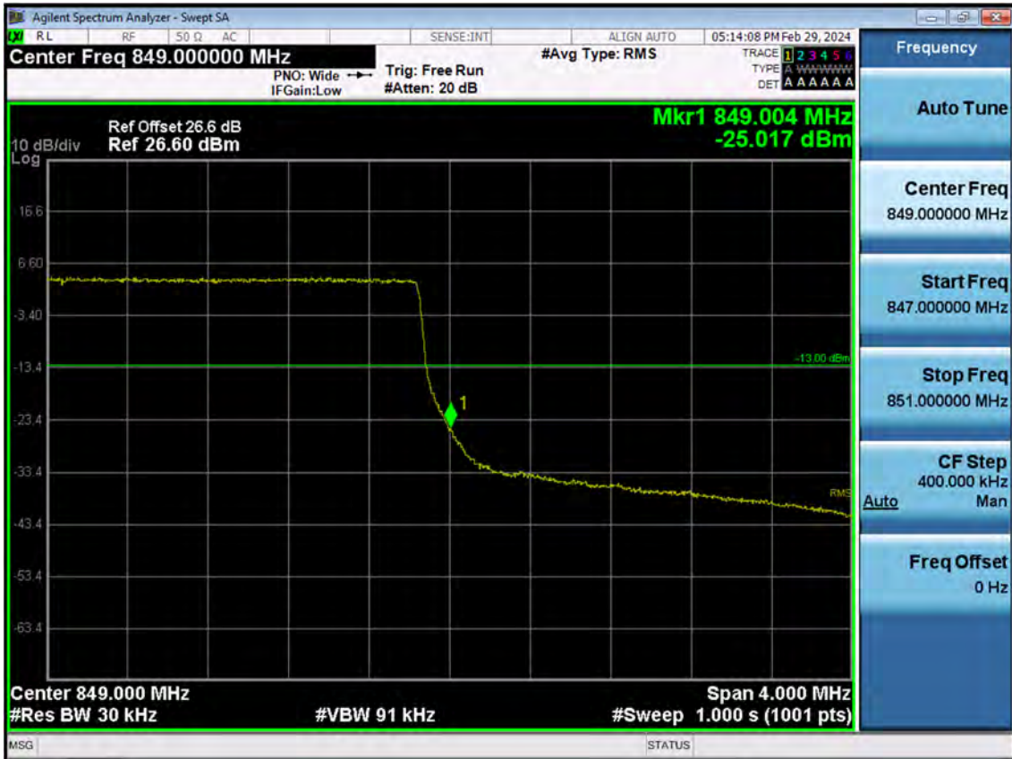
BAND5/26. Upper Band Edge Plot (3 M BW Ch.27025 QPSK_RB15_Offset 0)
