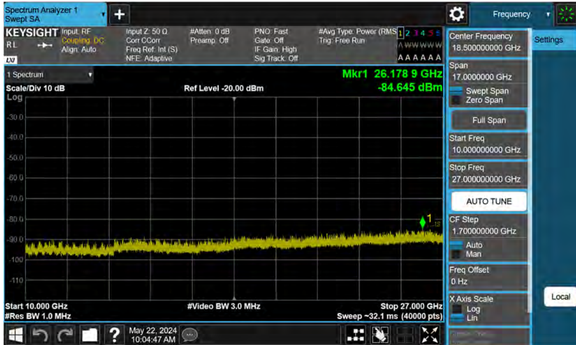
Sub6 n41_30 M_Conducted Spurious(Above10 G)_Low_BPSK_1RB
