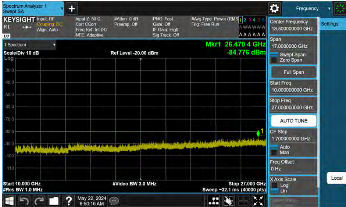
Sub6 n41_20 M_Conducted Spurious(Above10 G)_Low_BPSK_1RB
