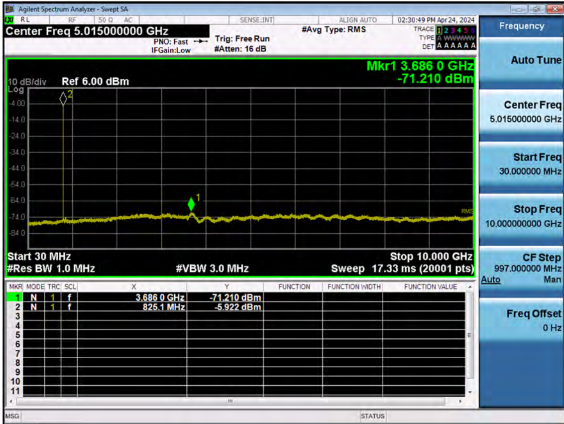
Sub6 n5_15 M_Conducted Spurious(30 M-10 G)_Low_BPSK_1RB
