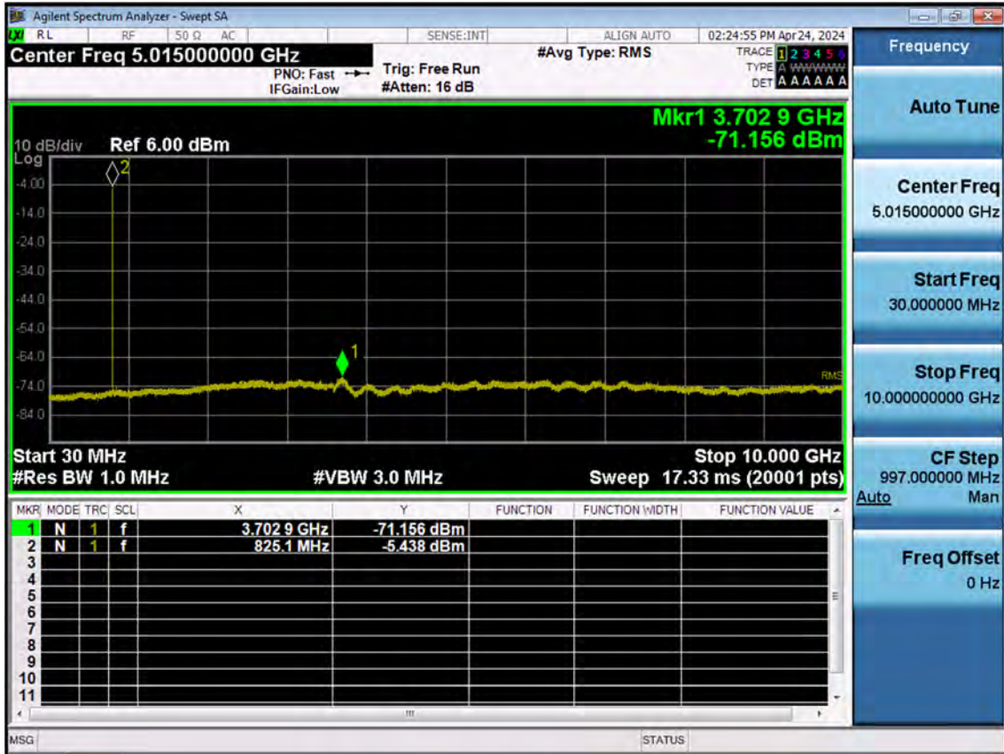
Sub6 n5_10 M_Conducted Spurious(30 M-10 G)_Low_BPSK_1RB
