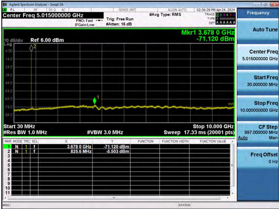
Sub6 n5_20 M_Conducted Spurious(30 M-10 G)_Low_BPSK_1RB
