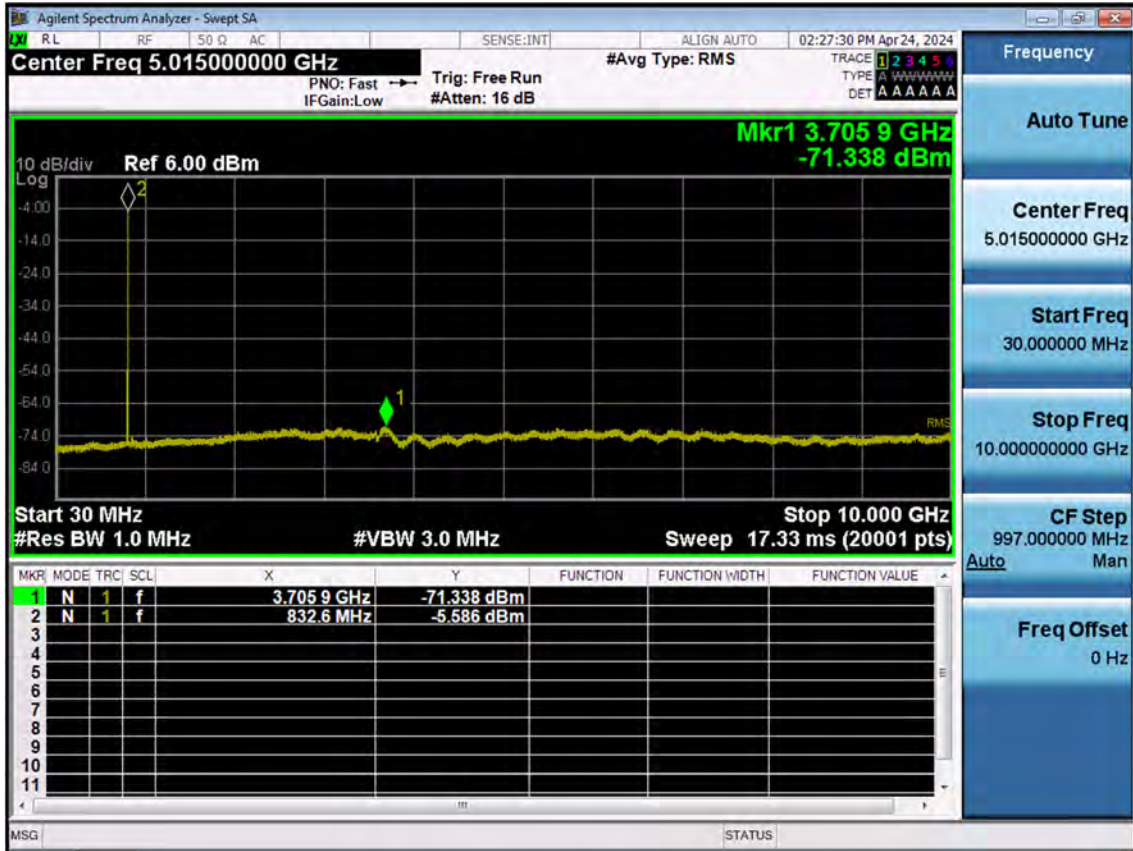
Sub6 n5_10 M_Conducted Spurious(30 M-10 G)_Mid_BPSK_FullRB
