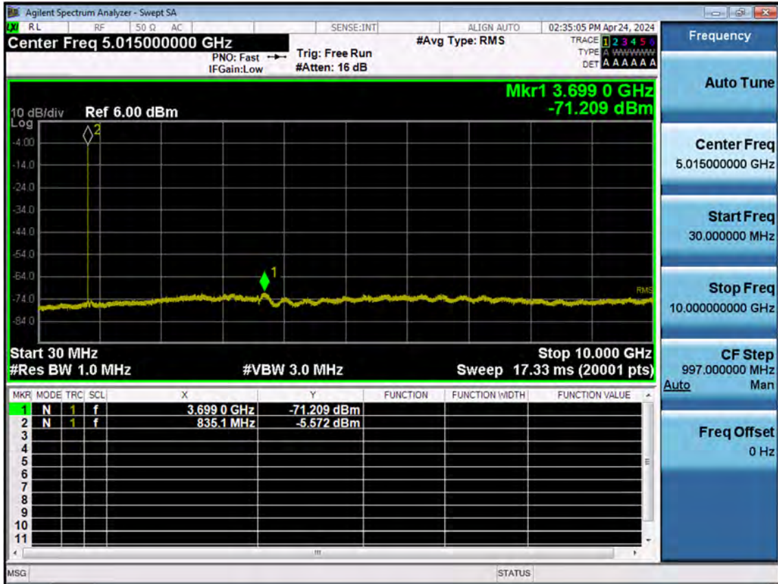
Sub6 n5_15 M_Conducted Spurious(30 M-10 G)_High_BPSK_1RB
