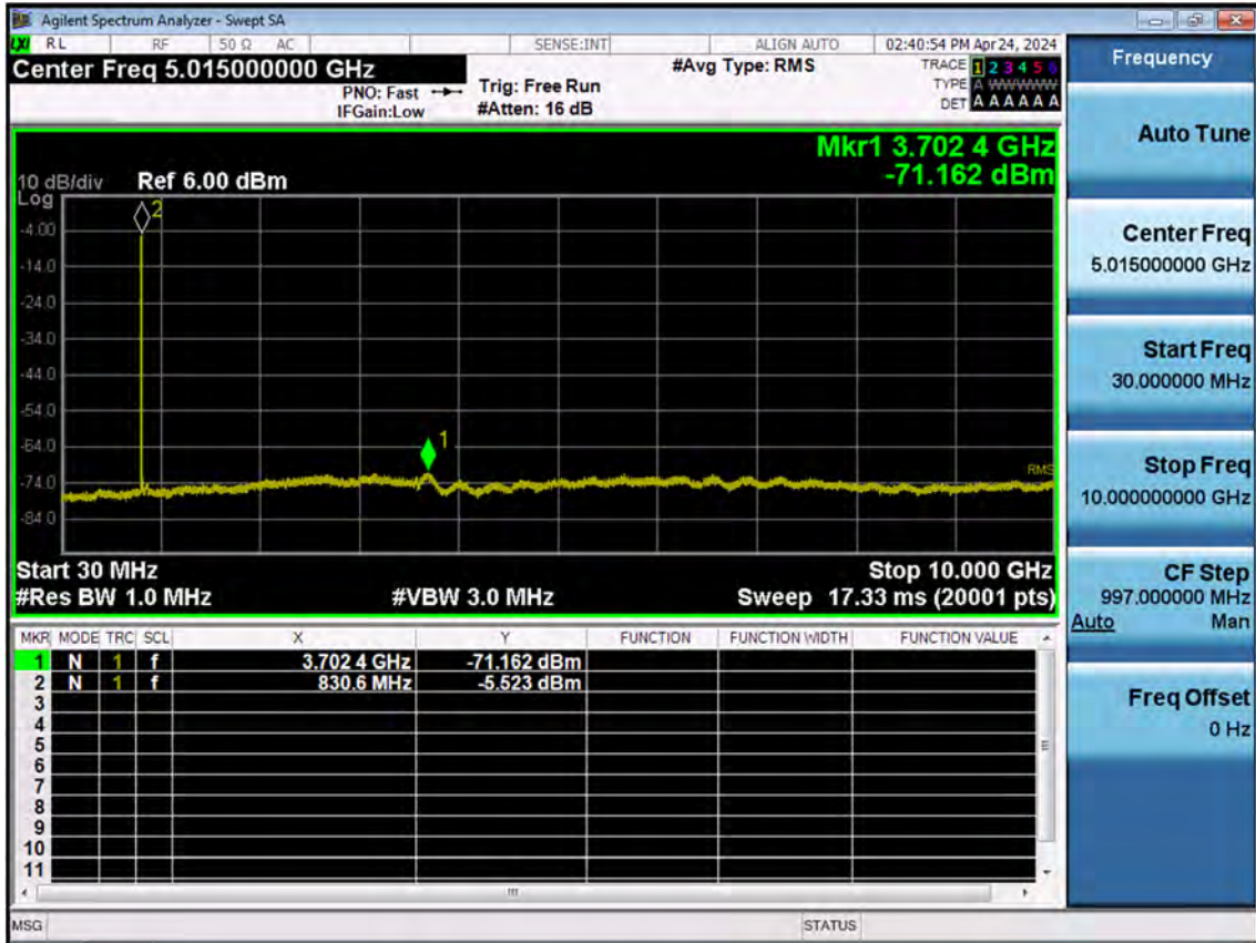
Sub6 n5_20 M_Conducted Spurious(30 M-10 G)_High_BPSK_1RB
