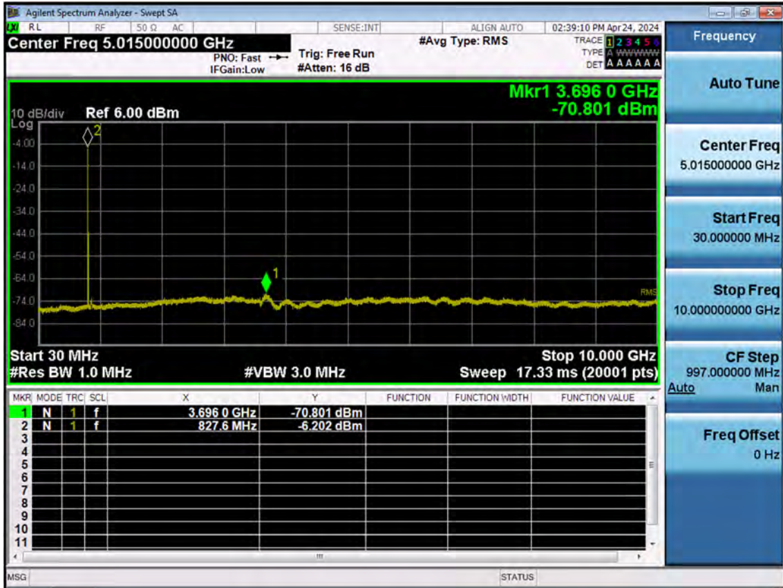
Sub6 n5_20 M_Conducted Spurious(30 M-10 G)_Mid_BPSK_FullRB
