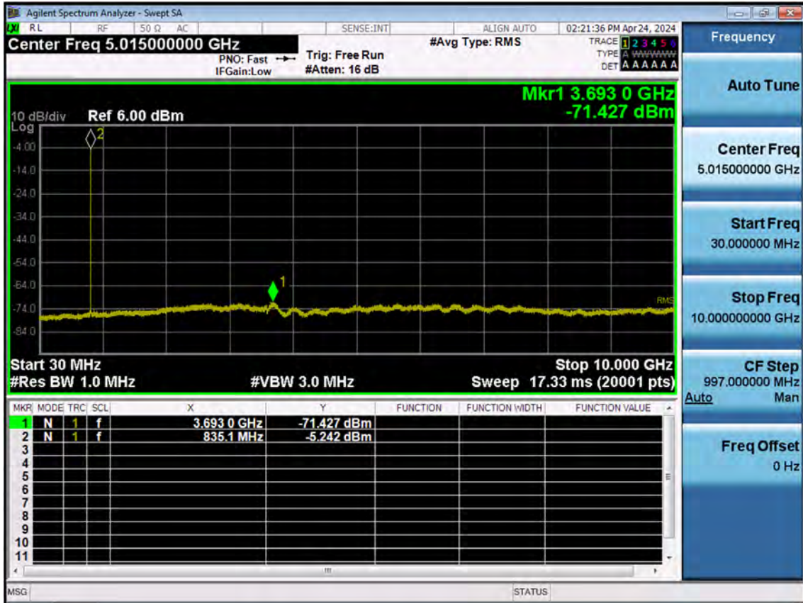
Sub6 n5_5 M_Conducted Spurious(30 M-10 G)_Mid_BPSK_FullRB
