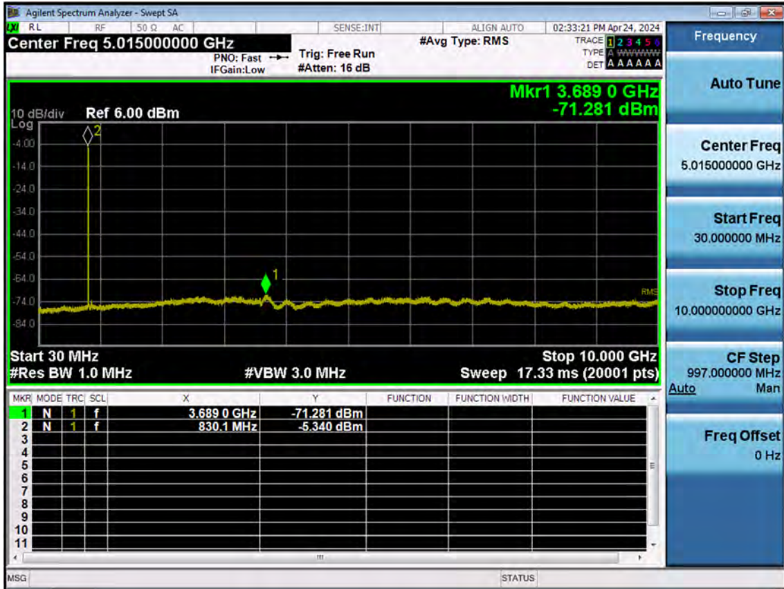
Sub6 n5_15 M_Conducted Spurious(30 M-10 G)_Mid_BPSK_FullRB
