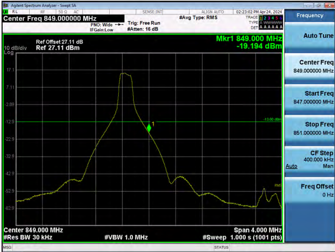
Sub6 n5_5 M_Band Edge_High_BPSK_1RB
