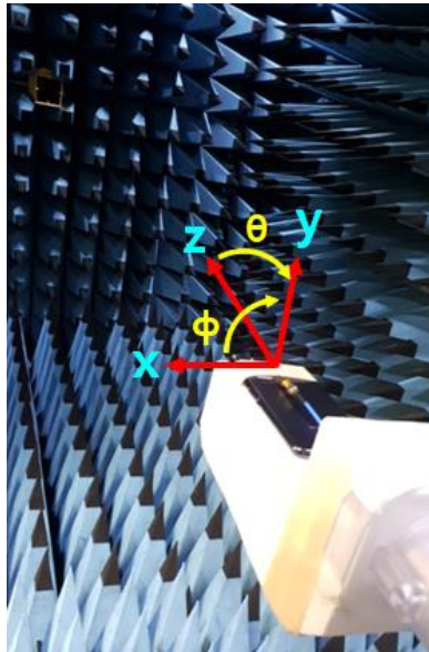
Figure 1: Geometry for SC-54E for Radiation patterns.
