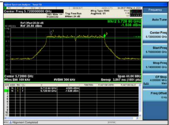
802.11n(HT40) UNII Band
