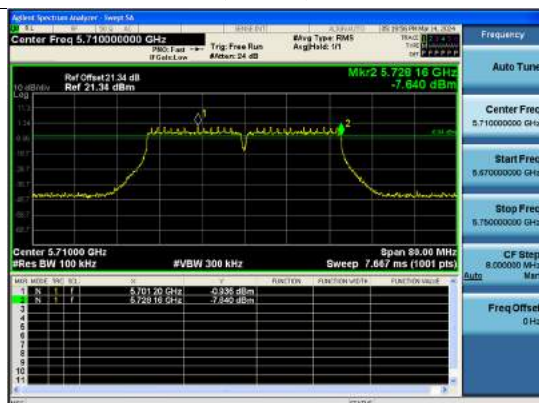
802.11ac(VHT40) UNII Band
