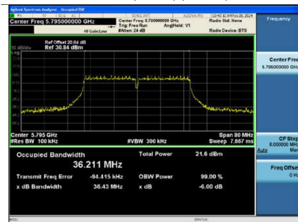
802.11ac(VHT40) (CH.159)
