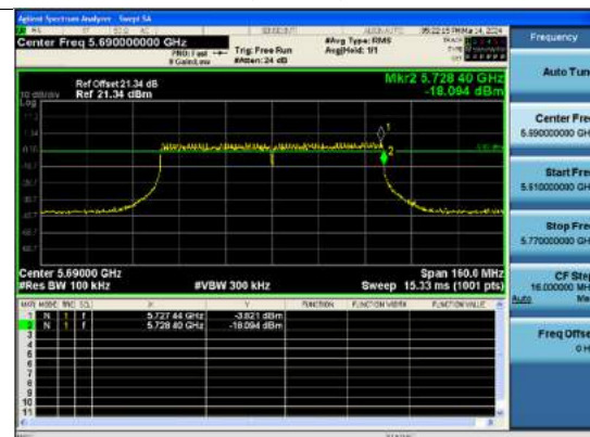
802.11ac(VHT80) UNII Band
