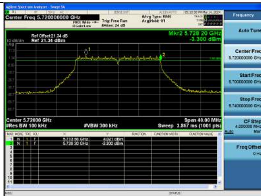
802.11ac(VHT20) UNII Band
