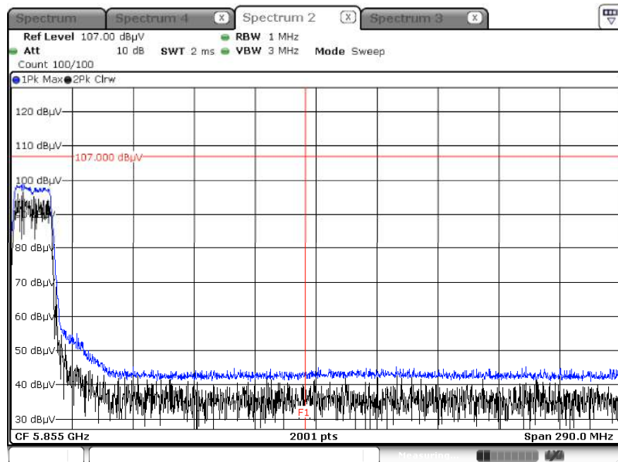
Peak Result (802.11ac_VHT20, Ch.144, X-H)
