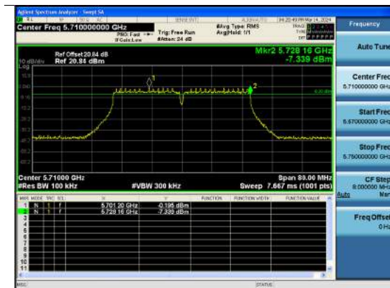
802.11ac(VHT40) UNII Band
