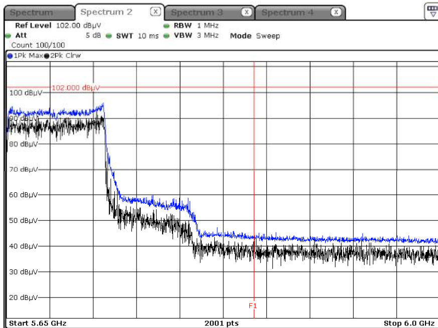
Peak result (802.11ax(HE80 Ch.138, SU))
