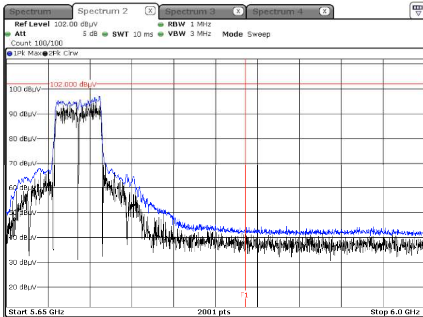
Peak result (802.11ax(HE40 Ch.142, 484T RU 65))
