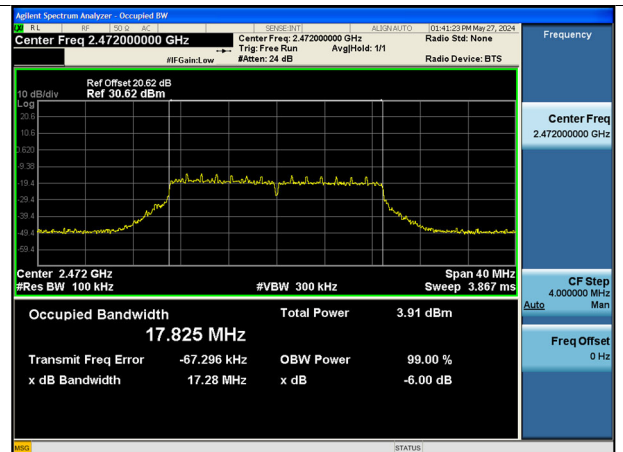
802.11ac_VHT20-CH 13
