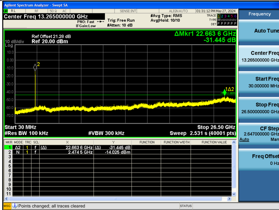
[ANT. 2] 802.11ac_VHT20_Ch.13_MCS4
