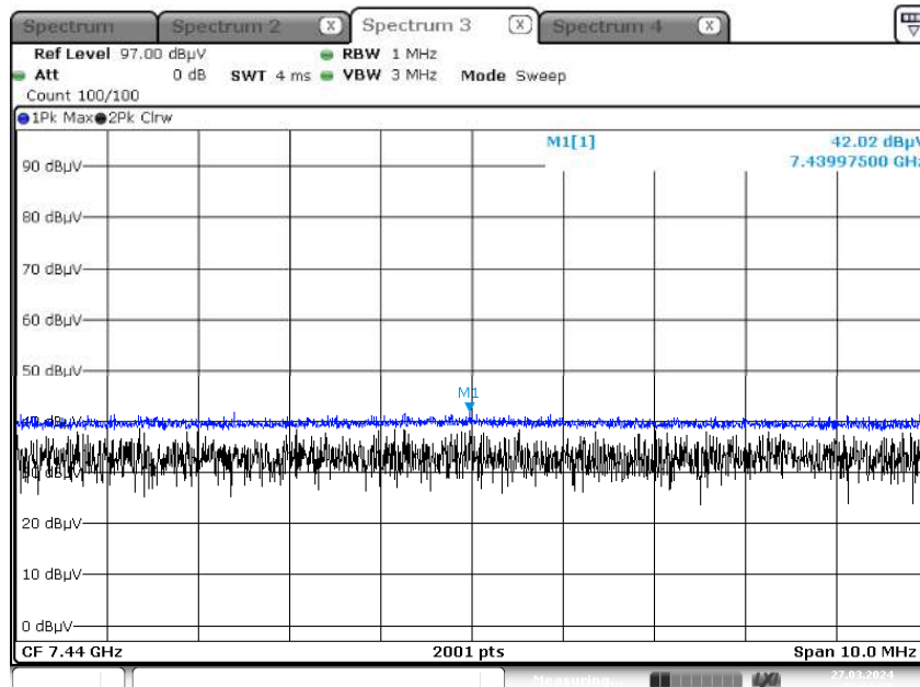
Radiated Spurious Emissions plot – Peak & Average Result (GFSK, Ch.78 3rd Harmonic, Y-H)
