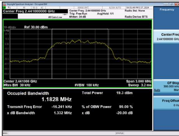
Dual ANT. 1 8DPSK 20 dB BW & 99% OBW (CH. 39)
