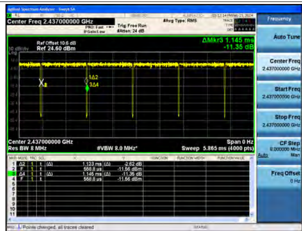
242 Tones (MCS 0)
