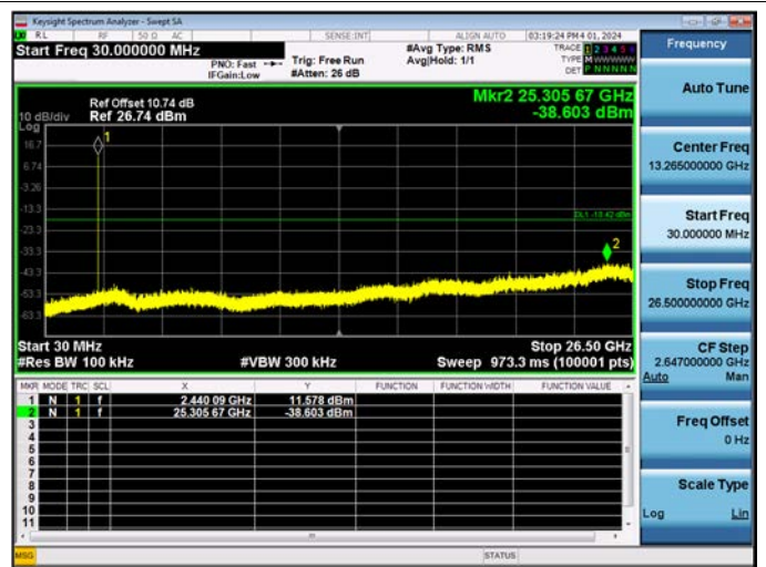
Dual BT Ant. 2 Conducted Spurious Emission
