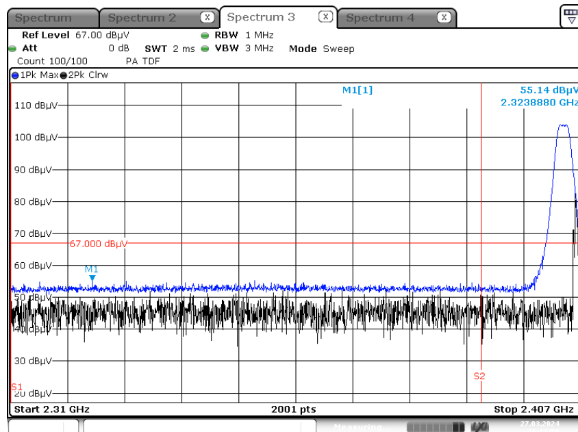
Radiated Restricted Band Edges plot – Peak Result (Ch.0, Z-V)
