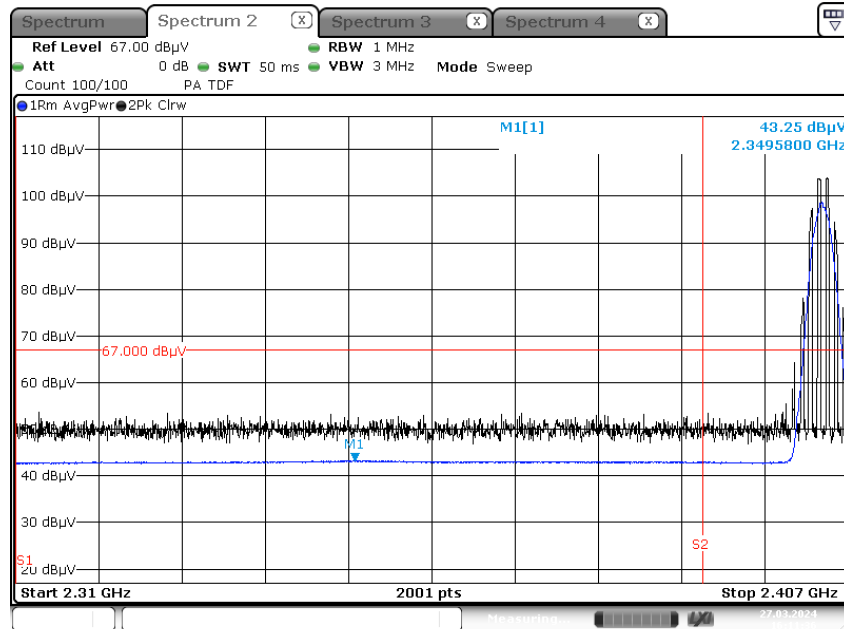
Radiated Restricted Band Edges plot – Average Result (Ch.0, Z-V)
