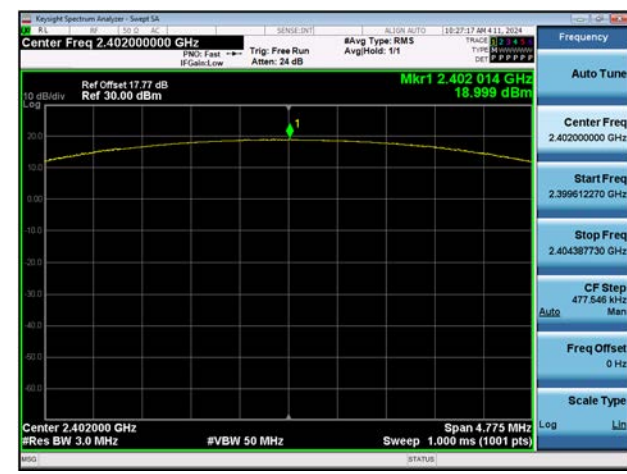
ANT.1 8DPSK : Peak Power (CH. 0)
