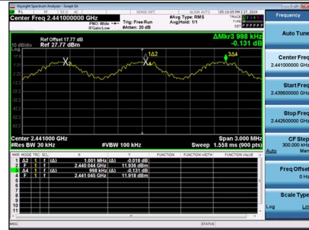
Dual ANT. 1 \pi/4 DQPSK : Channel Separation
