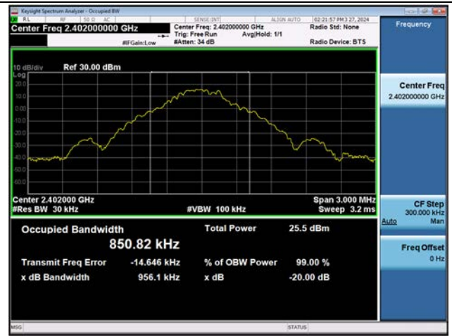
ANT. 2 \pi /4DQPSK 20 dB BW & 99% OBW (CH. 0)
