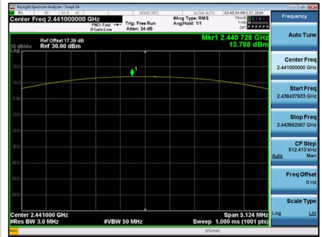
Dual ANT.2 8DPSK : Peak Power (CH.39)
