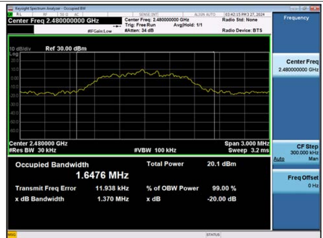
Dual ANT. 2 8DPSK 20 dB BW &amp; 99% OBW (CH. 78)
