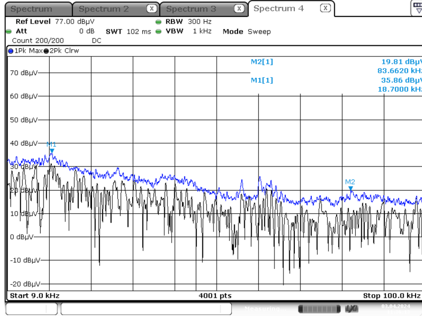
Frequency Range : 9 kHz - 100 kHz
