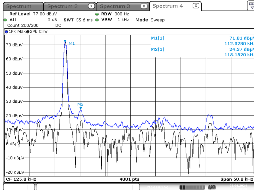
Frequency Range : 100 kHz - 150kHz
