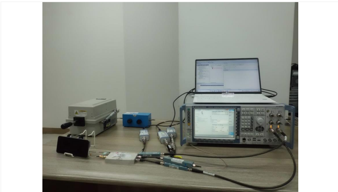
Test setup photo-8 (7-1(f) System level compliance)
