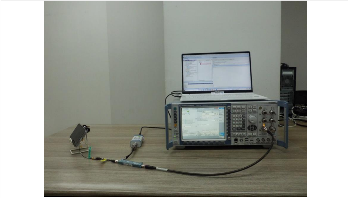
Test setup photo-1 (7-1(a) Legacy)
