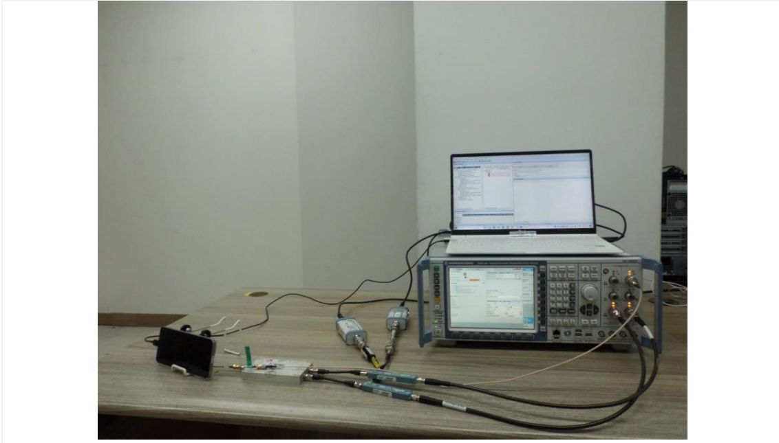
Test setup photo-7 (7-1(e) WLAN DBS)
