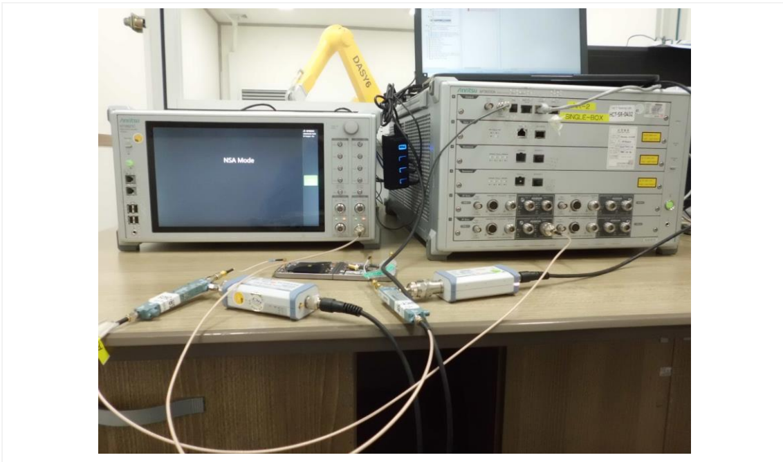
Test setup photo-6 (7-1(c) 5G Sub 6 NSA)
