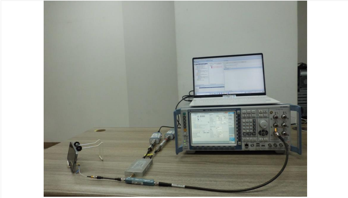
Test setup photo-3 (7-1(c) Legacy)
