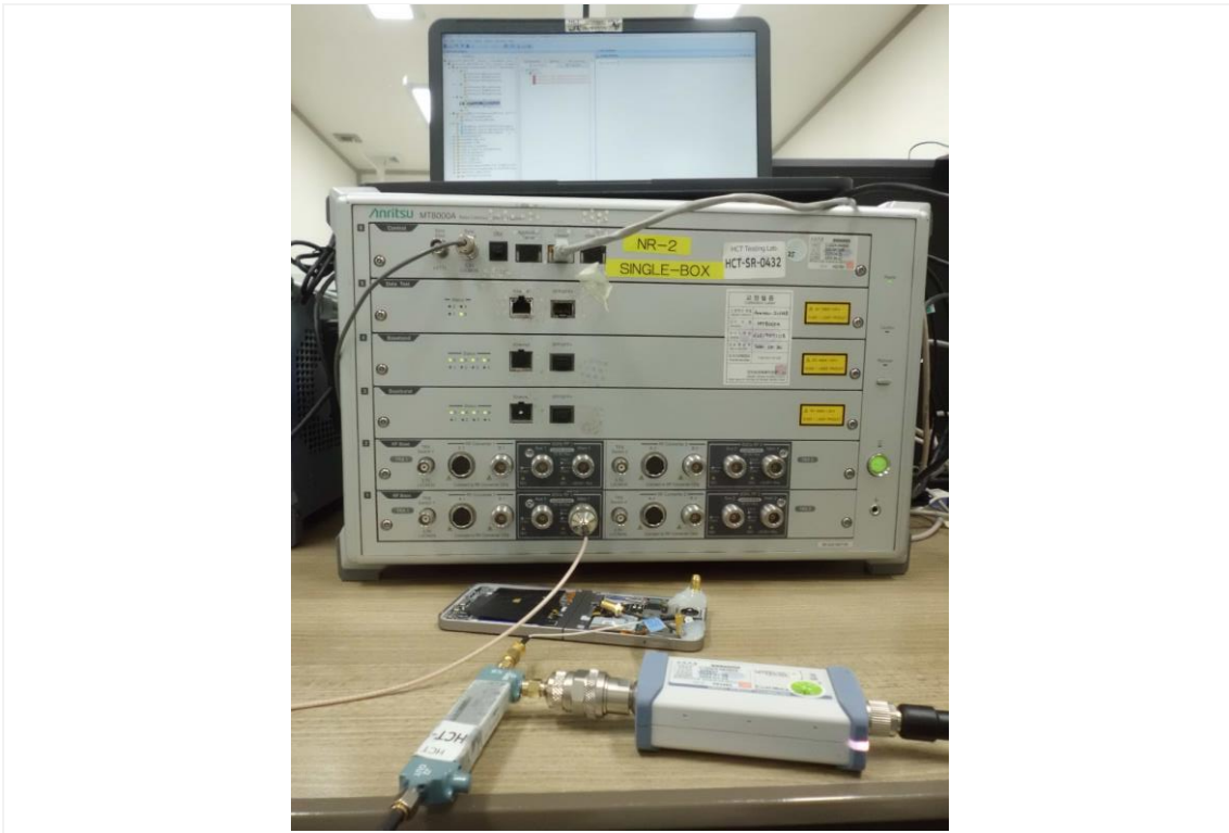
Test setup photo-4 (7-1(a) 5G Sub 6)
