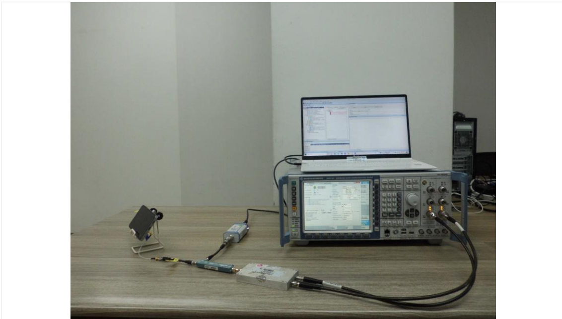
Test setup photo-2 (7-1(b) Legacy)
