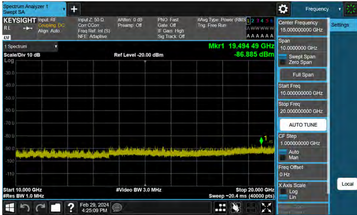
NR66_25 M_Conducted Spurious(Above10 G)_Mid_BPSK_FullRB
