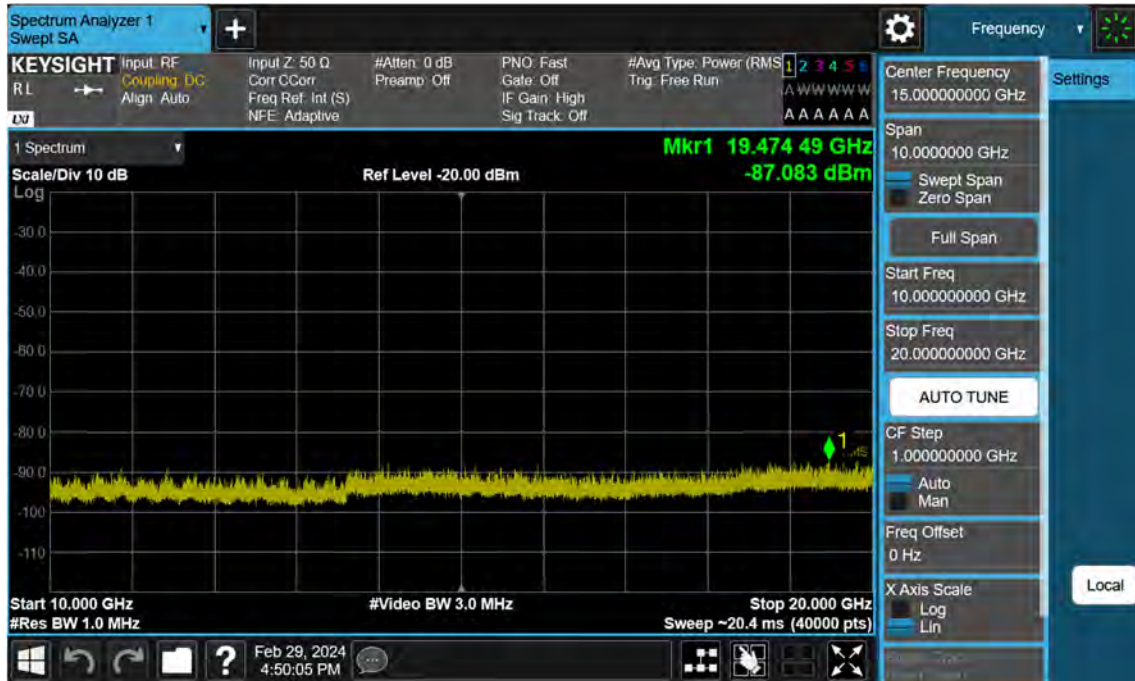
NR66_40 M_Conducted Spurious(Above10 G)_Mid_BPSK_FullRB
