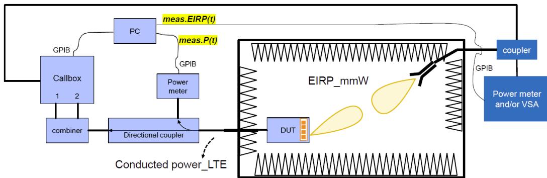
Figure 7-1 mmW NR radiated power measurement setup – Test Setup Photos 13 and 14
