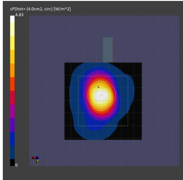
Figure 12-2 4cm 2 psPD distribution measured at input.power.limit of 5.0 dBm on the folder open, left edge for n260 beam 14
