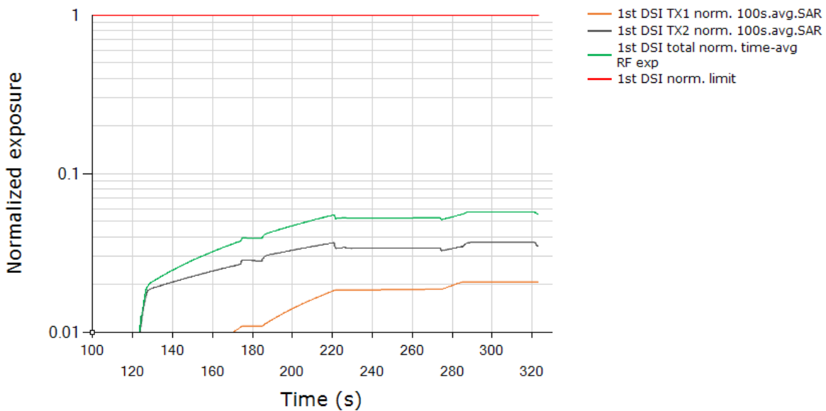
Total Normalized Time-averaged RF Exposure (1st DSI) Tech: LTE, Band 66 / Tech: NR5G SUB6, Band n41
