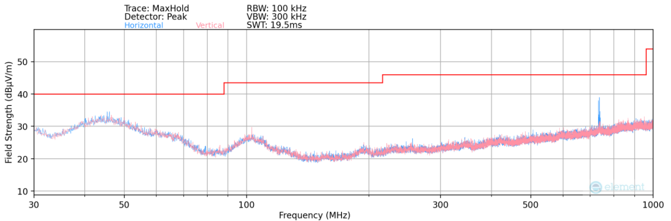
Plot 7-2. Radiated Spurious Plot below 1GHz – Open
