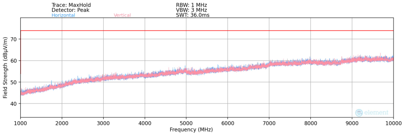
Plot 7-3. Radiated Spurious Plot above 1GHz – Half Open
