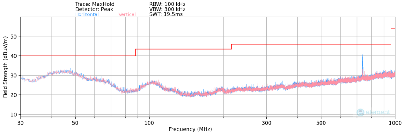
Plot 7-1. Radiated Spurious Plot below 1GHz – Half Open
