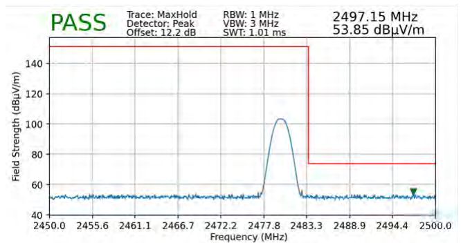
Plot 7-102. Radiated Restricted Upper Band Edge Measurement with WCP (Peak) – ANT1
