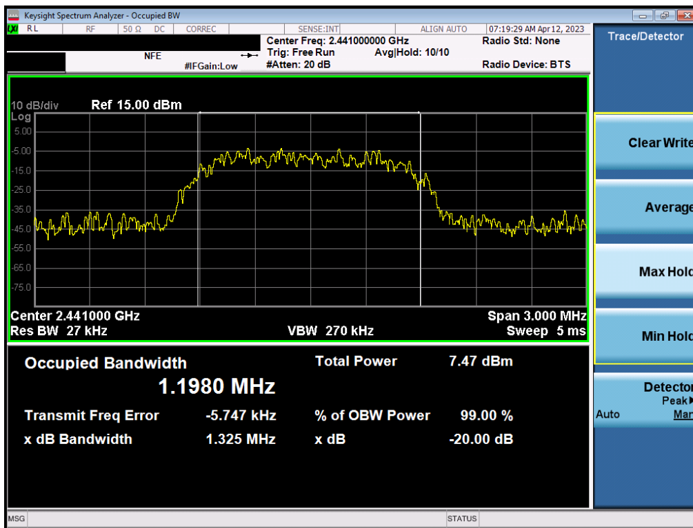
Plot 7-14. 20dB Bandwidth Plot (Bluetooth, 2Mbps – Ch. 39) – ANT2
