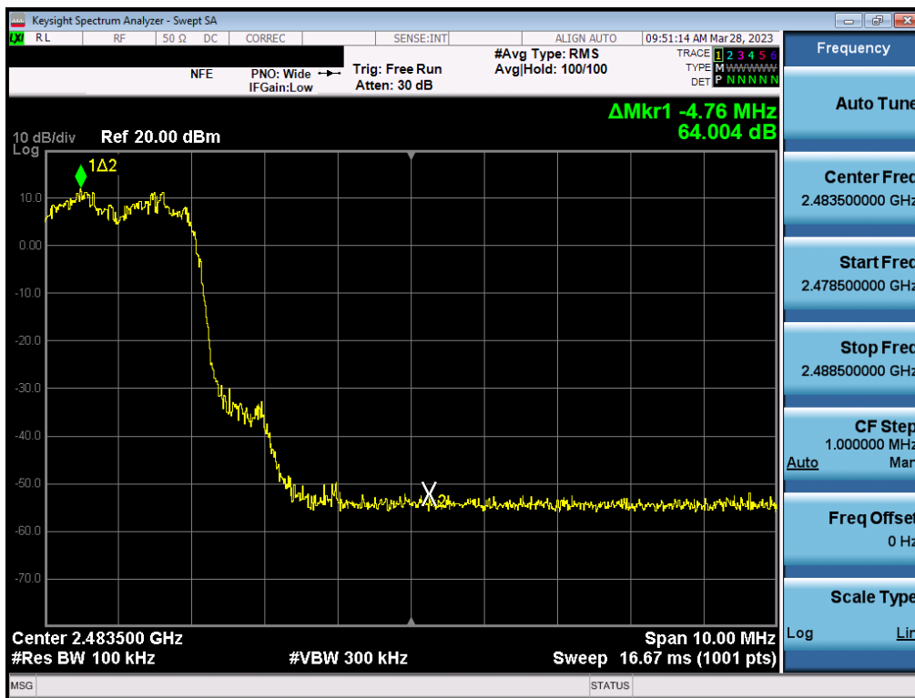
Plot 7-62. Band Edge Plot (Bluetooth with Hopping Enabled, 3 Mbps – Ch. 78) – ANT2
