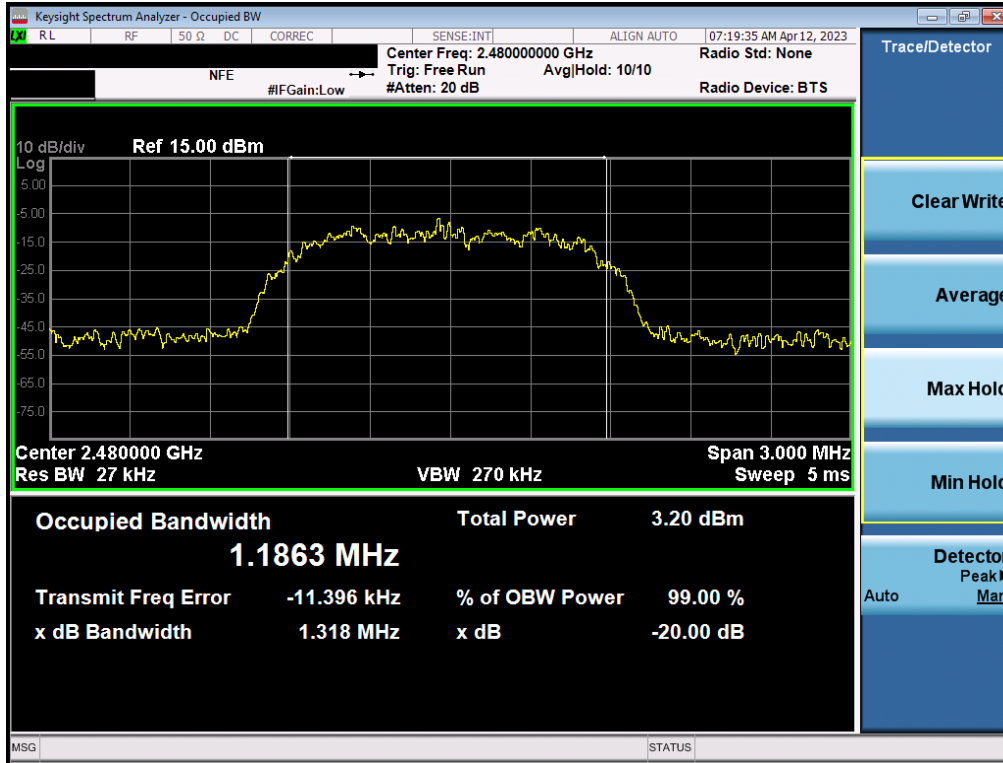
Plot 7-15. 20dB Bandwidth Plot (Bluetooth, 2Mbps – Ch. 78) – ANT2
