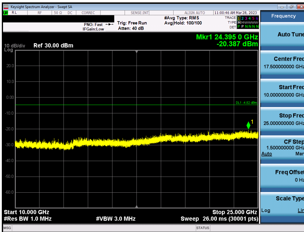
Plot 7-72. Conducted Spurious Plot (Bluetooth, N/AMbps – Ch. 0) – ANT1
