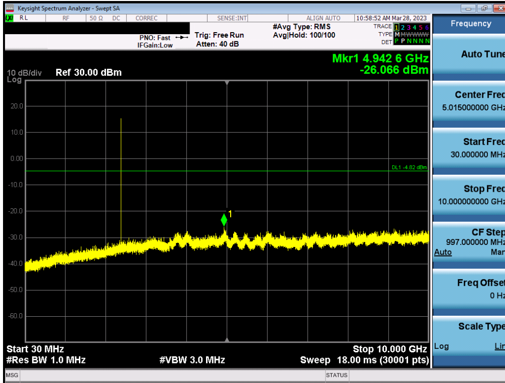
Plot 7-71. Conducted Spurious Plot (Bluetooth, N/AMbps – Ch. 0) – ANT1
