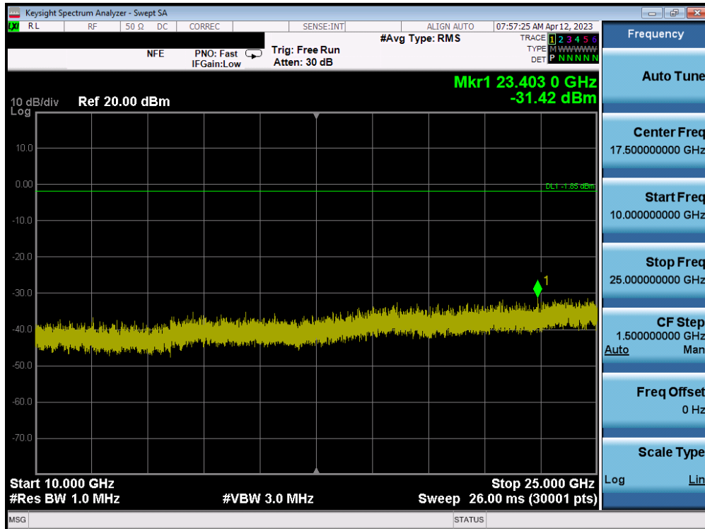
Plot 7-80. Conducted Spurious Plot (Bluetooth, N/AMbps – Ch. 39) – ANT2
