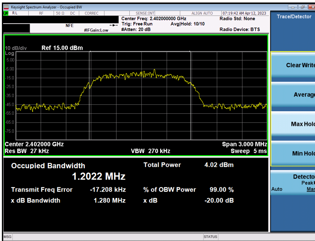
Plot 7-16. 20dB Bandwidth Plot (Bluetooth, 3Mbps – Ch. 0) – ANT2
