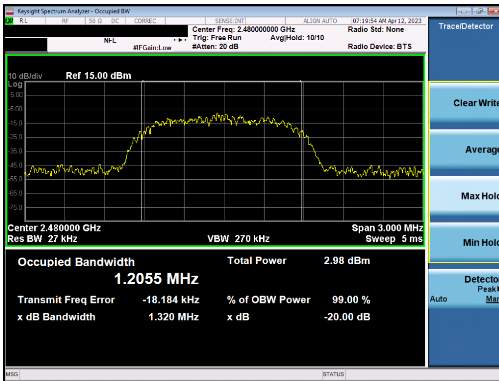
Plot 7-18. 20dB Bandwidth Plot (Bluetooth, 3Mbps – Ch. 78) – ANT2
