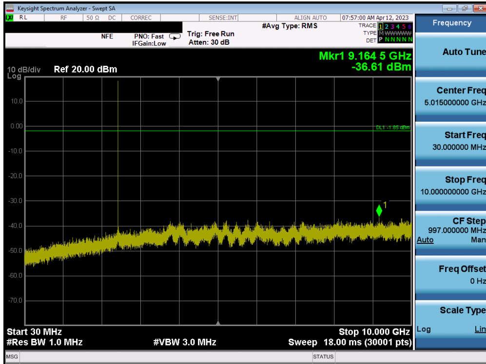
Plot 7-79. Conducted Spurious Plot (Bluetooth, N/AMbps – Ch. 39) – ANT2
