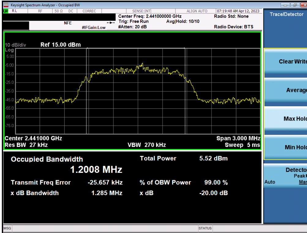
Plot 7-17. 20dB Bandwidth Plot (Bluetooth, 3Mbps – Ch. 39) – ANT2
