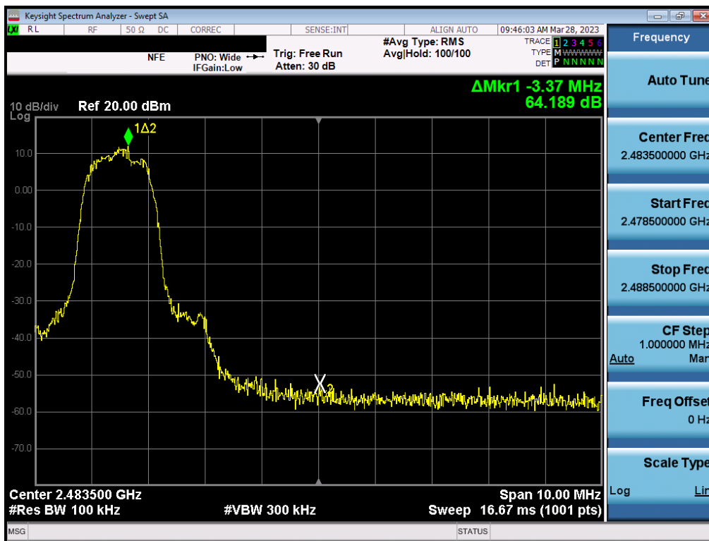
Plot 7-60. Band Edge Plot (Bluetooth with Hopping Disabled, 3 Mbps – Ch. 78) – ANT2
