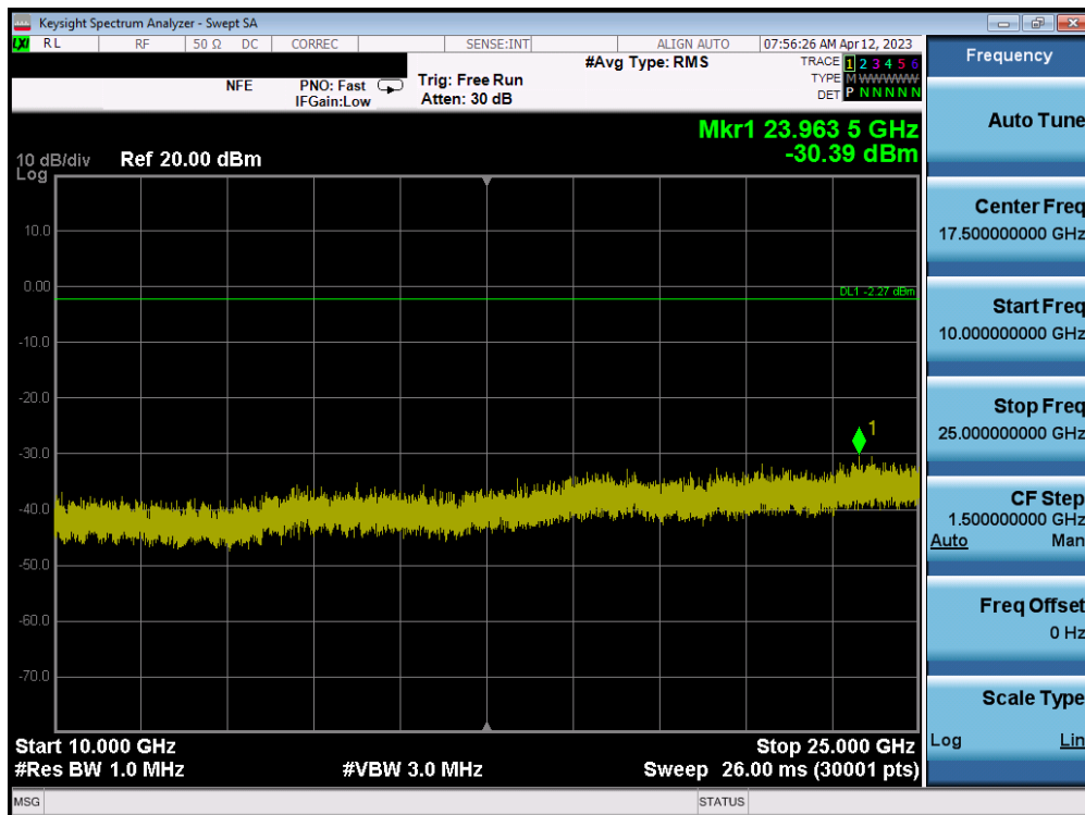
Plot 7-78. Conducted Spurious Plot (Bluetooth, N/AMbps – Ch. 0) – ANT2
