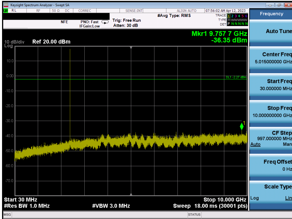
Plot 7-77. Conducted Spurious Plot (Bluetooth, N/AMbps – Ch. 0) – ANT2
