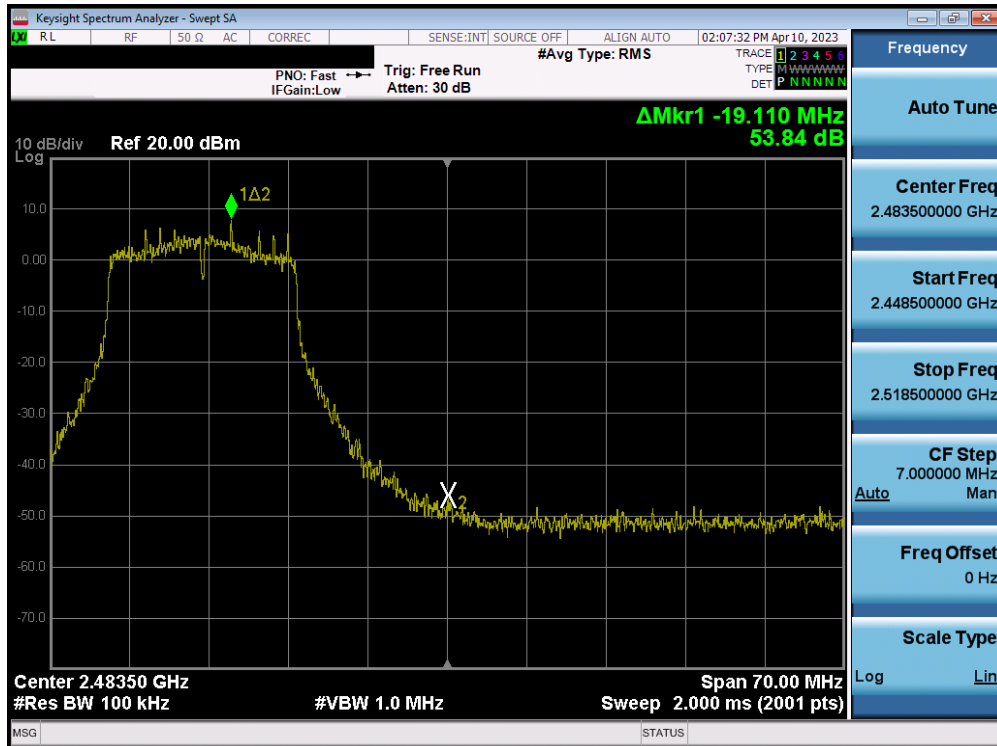
Plot 7-76. Band Edge Plot MIMO ANT1 (802.11g - Ch. 11)
