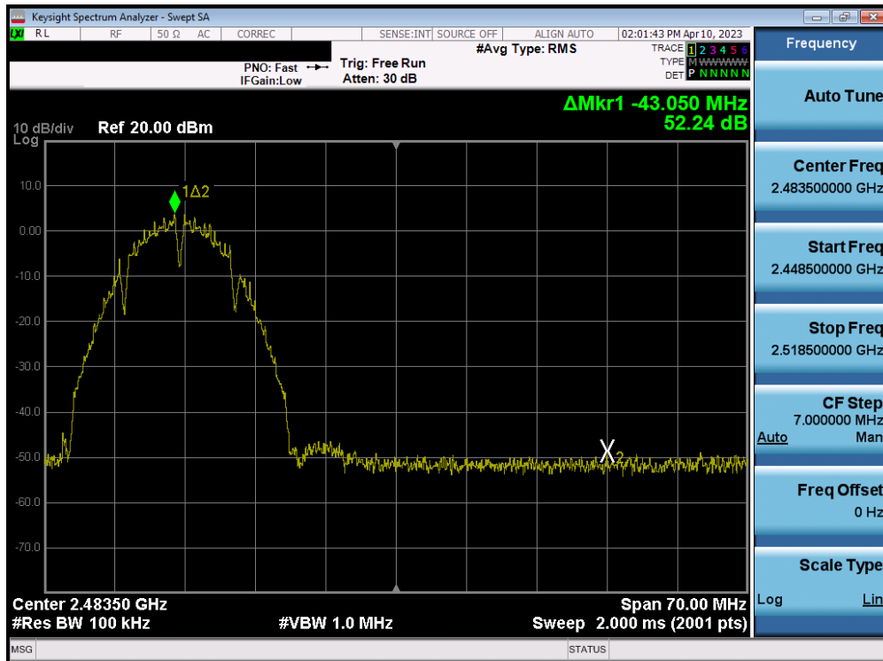
Plot 7-72. Band Edge Plot MIMO ANT1 (802.11b – Ch. 11)
