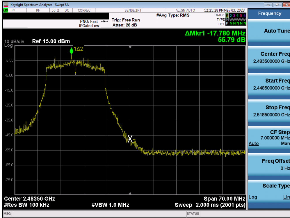
Plot 7-81. Band Edge Plot MIMO ANT1 (802.11n (2.4GHz) – Ch. 12)
