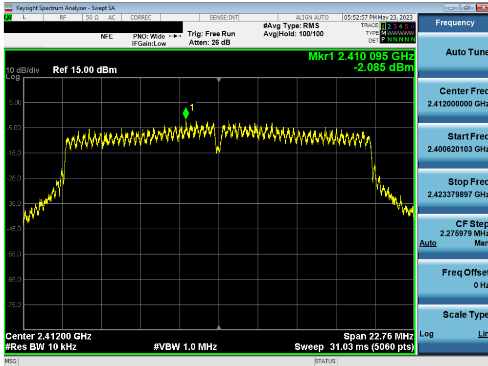
Plot 7-46. Power Spectral Density Plot MIMO ANT1 (802.11ac (2.4GHz) – Ch. 1)
