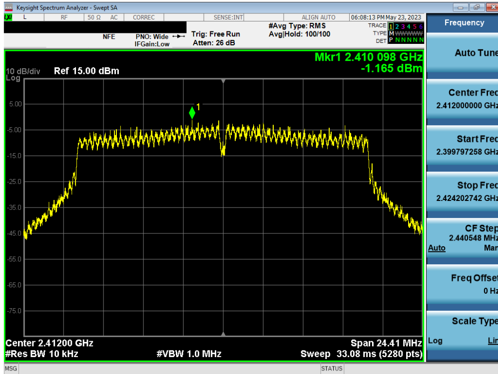
Plot 7-61. Power Spectral Density Plot MIMO ANT2 (802.11ac (2.4GHz) – Ch. 1)
