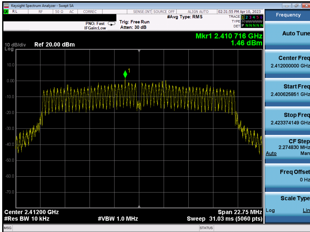
Plot 7-58. Power Spectral Density Plot MIMO ANT2 (802.11n (2.4GHz) – Ch. 1)
