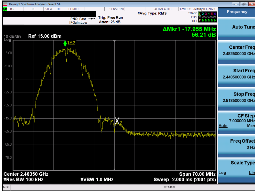
Plot 7-93. Band Edge Plot MIMO ANT2 (802.11b – Ch. 12)
