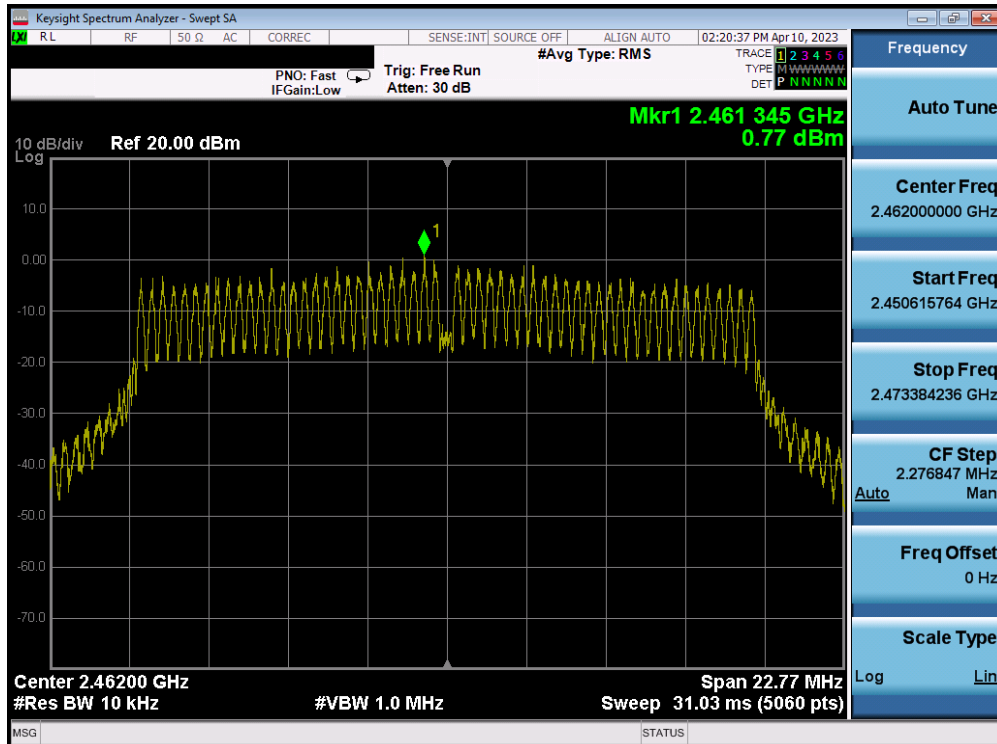
Plot 7-66. Power Spectral Density Plot MIMO ANT2 (802.11ax (2.4GHz) – Ch. 11)
