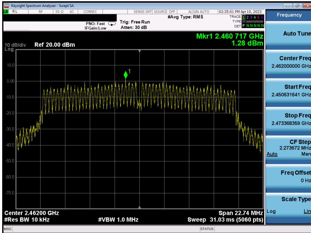
Plot 7-60. Power Spectral Density Plot MIMO ANT2 (802.11n (2.4GHz) – Ch. 11)
