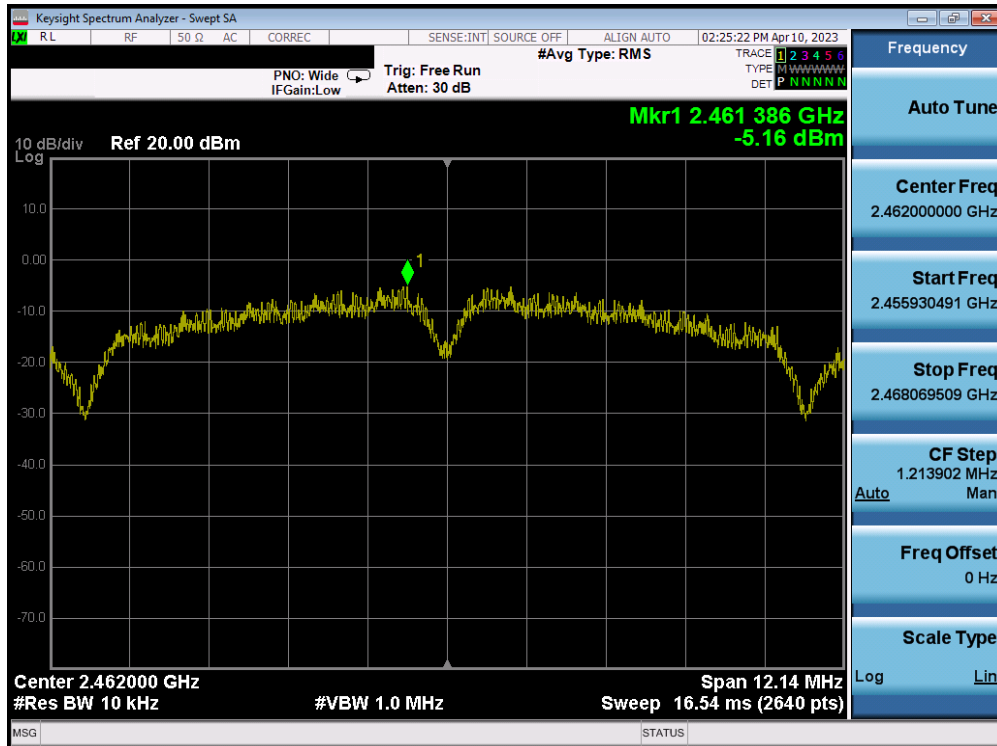
Plot 7-54. Power Spectral Density Plot MIMO ANT2 (802.11b – Ch. 11)
