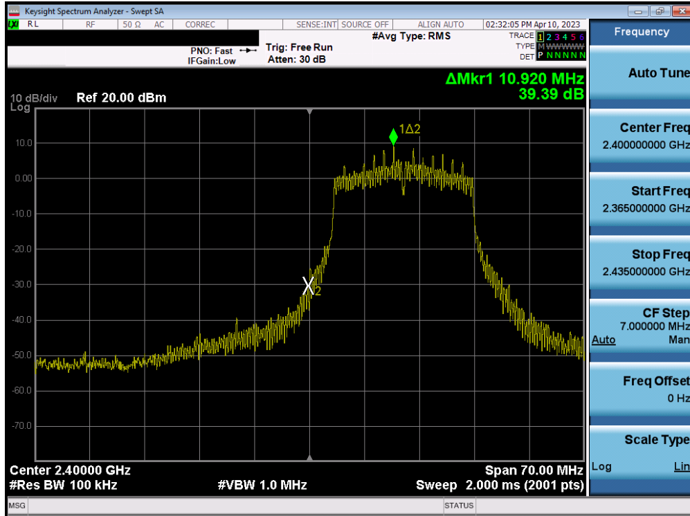
Plot 7-99. Band Edge Plot MIMO ANT2 (802.11n (2.4GHz) – Ch. 1)
