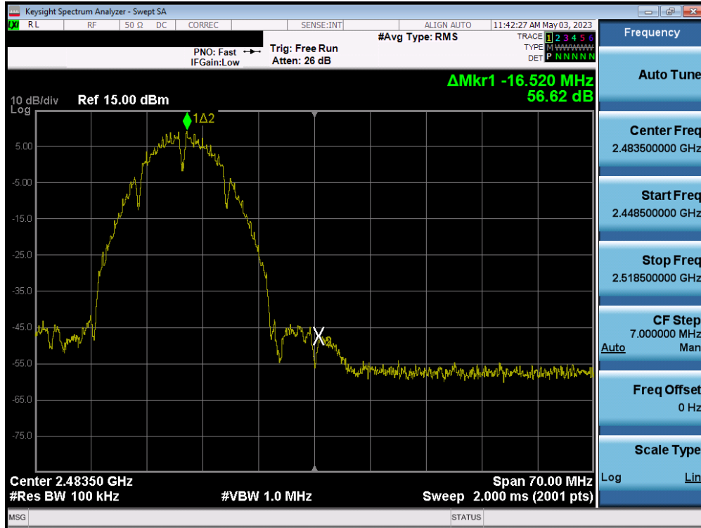
Plot 7-69. Band Edge Plot SISO ANT2 (802.11b – Ch. 12)
