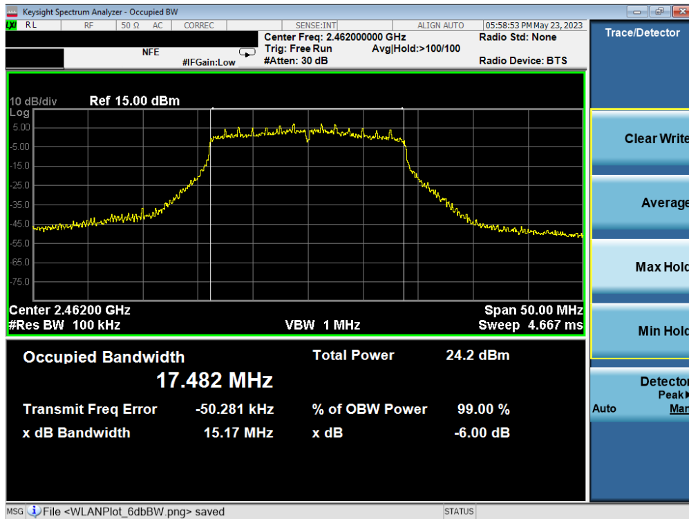
Plot 7-15. 6dB Bandwidth Plot MIMO ANT1 (802.11ac (2.4GHz) – Ch. 11)
