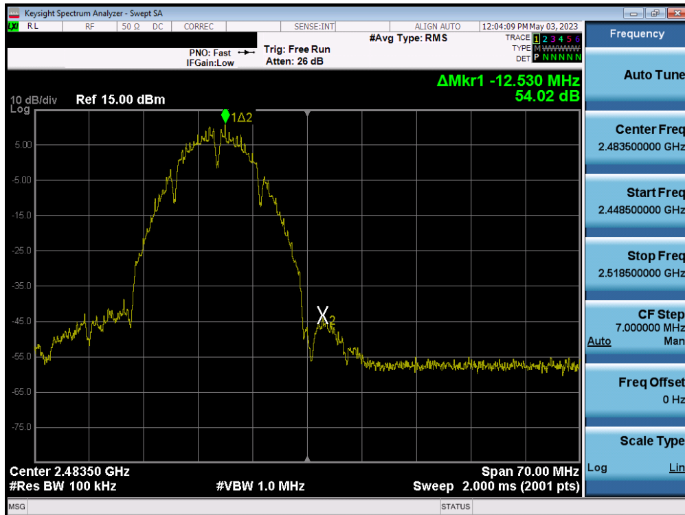
Plot 7-94. Band Edge Plot MIMO ANT2 (802.11b – Ch. 13)
