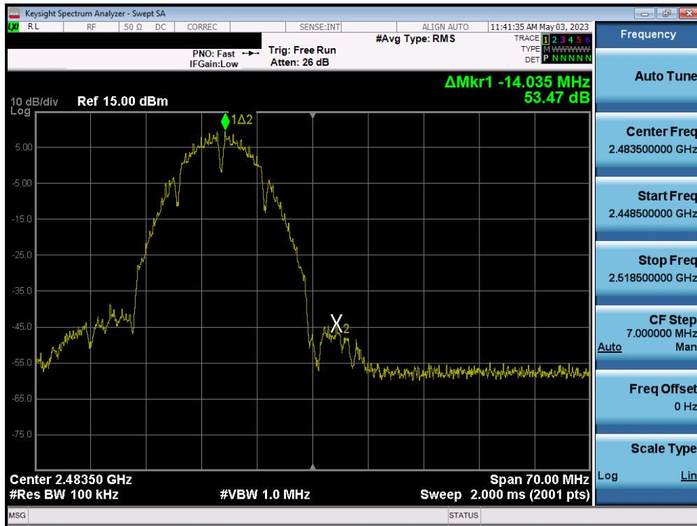
Plot 7-70. Band Edge Plot SISO ANT2 (802.11b – Ch. 13)
