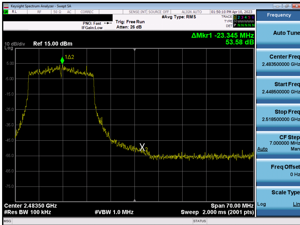
Plot 7-88. Band Edge Plot MIMO ANT1 (802.11ax (2.4GHz) – Ch. 11)
