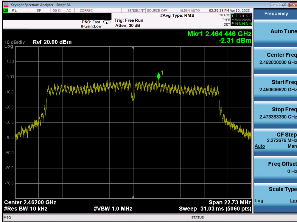
Plot 7-57. Power Spectral Density Plot MIMO ANT2 (802.11g – Ch. 11)
