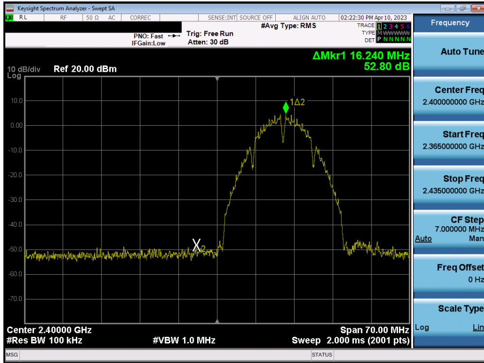
Plot 7-91. Band Edge Plot MIMO ANT2 (802.11b – Ch. 1)
