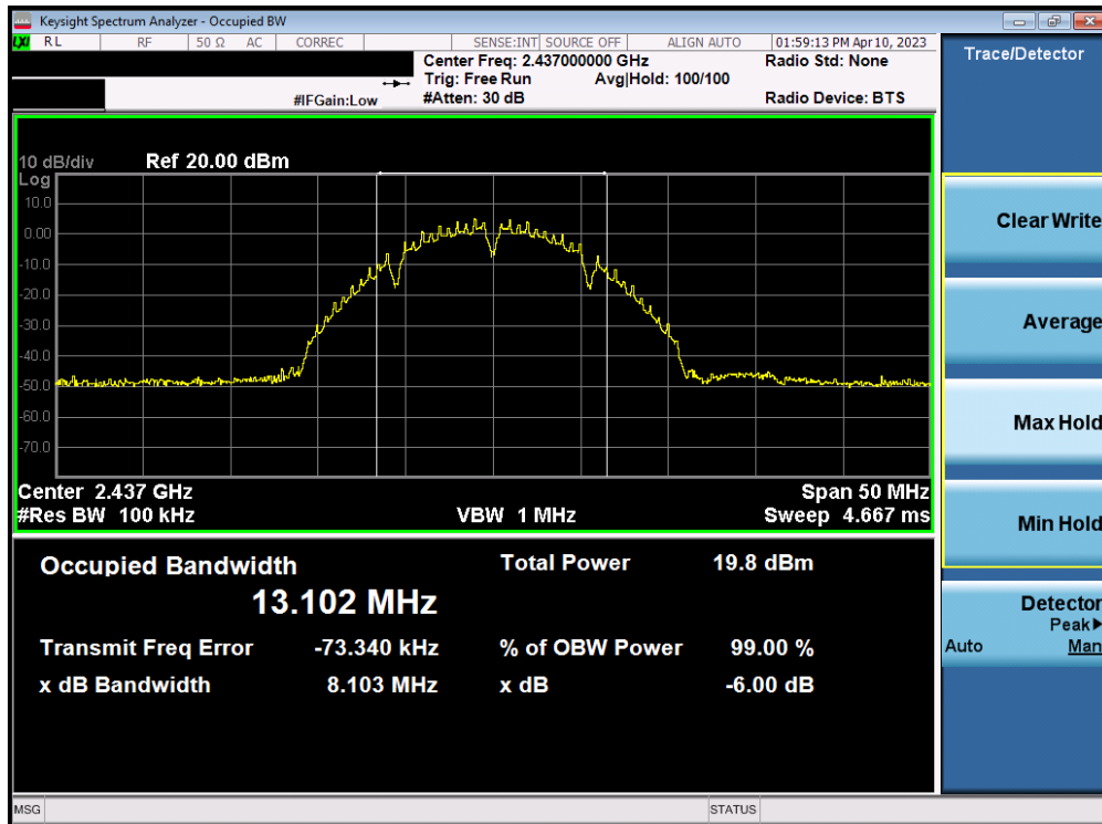
Plot 7-5. 6dB Bandwidth Plot MIMO ANT1 (802.11b – Ch. 6)
