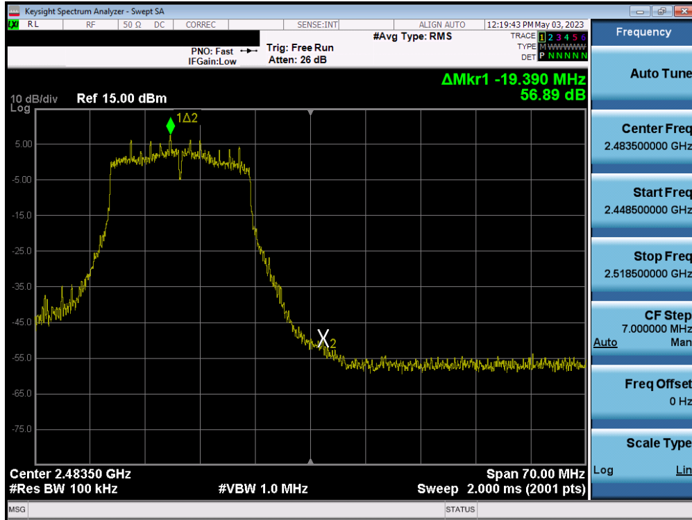
Plot 7-85. Band Edge Plot MIMO ANT1 (802.11ac (2.4GHz) – Ch. 12)
