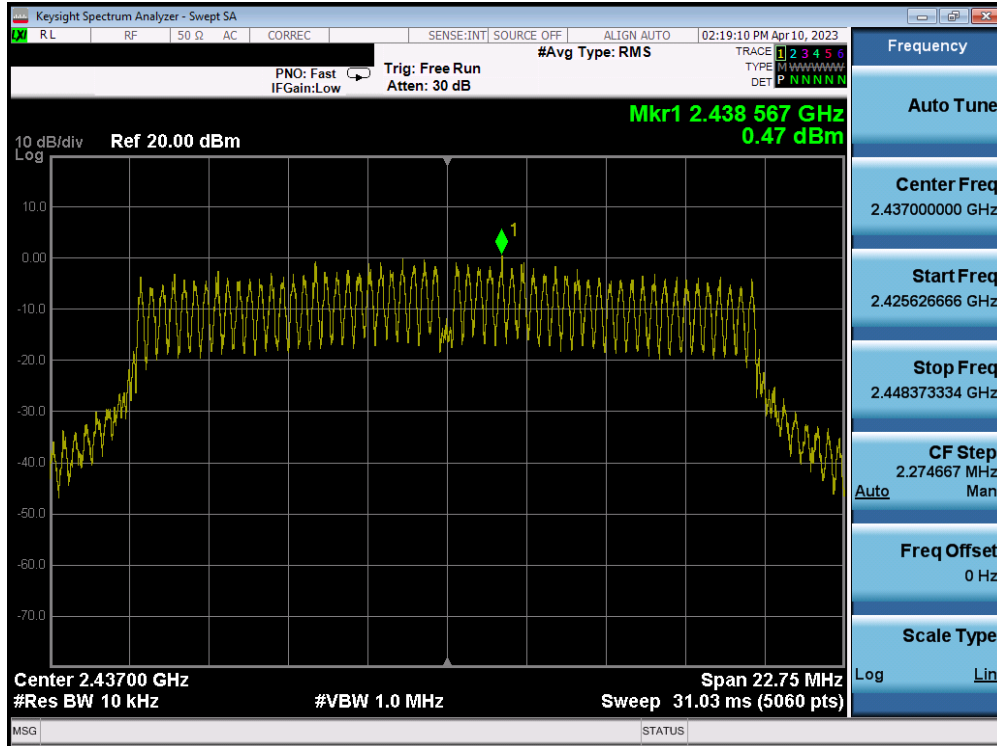
Plot 7-65. Power Spectral Density Plot MIMO ANT2 (802.11ax (2.4GHz) – Ch. 6)
