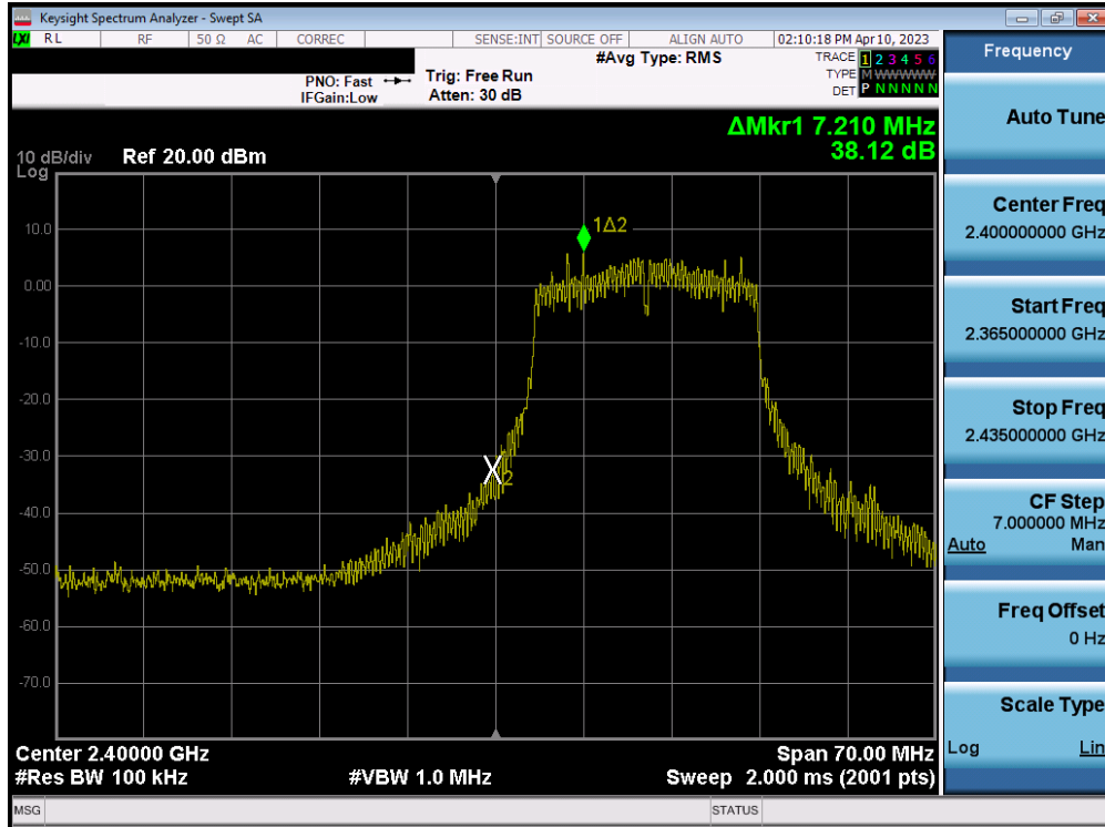
Plot 7-79. Band Edge Plot MIMO ANT1 (802.11n (2.4GHz) – Ch. 1)
