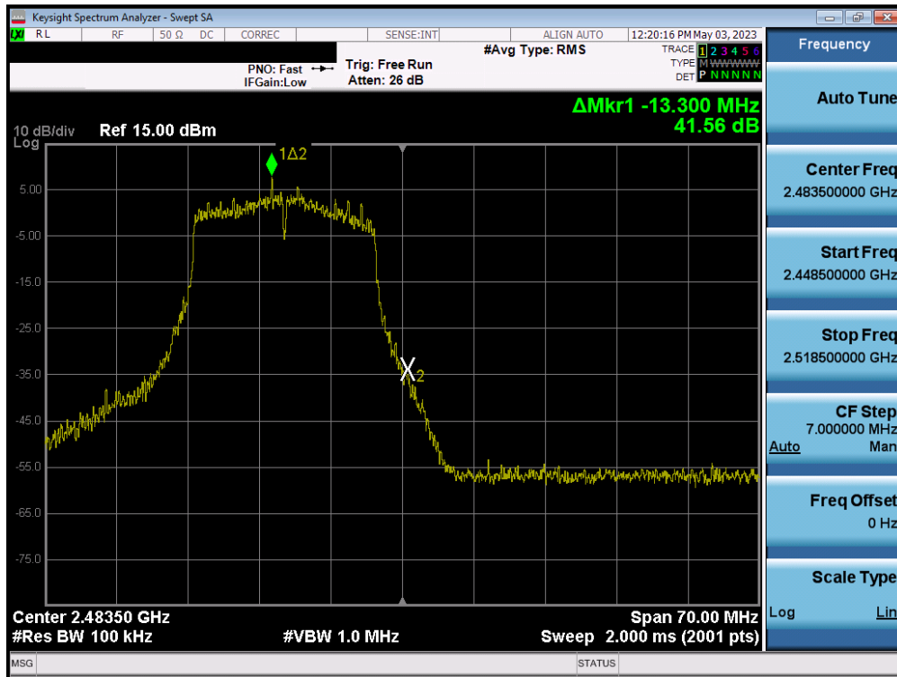
Plot 7-86. Band Edge Plot MIMO ANT1 (802.11ac (2.4GHz) – Ch. 13)
