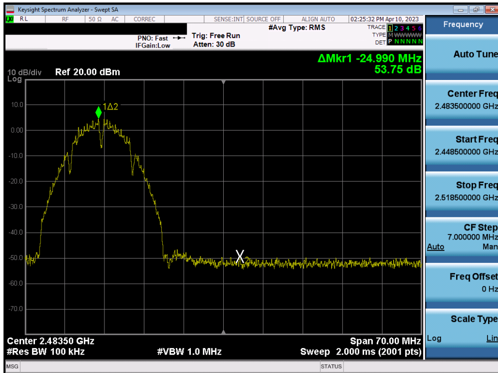
Plot 7-92. Band Edge Plot MIMO ANT2 (802.11b – Ch. 11)
