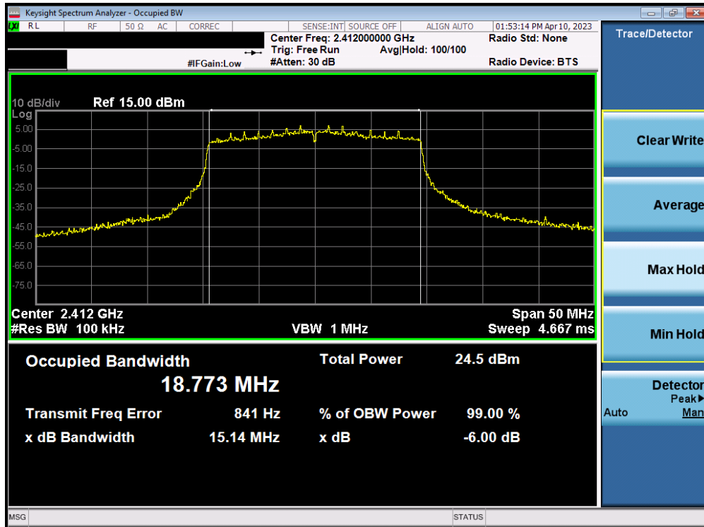
Plot 7-16. 6dB Bandwidth Plot MIMO ANT1 (802.11ax (2.4GHz) – Ch. 1)
