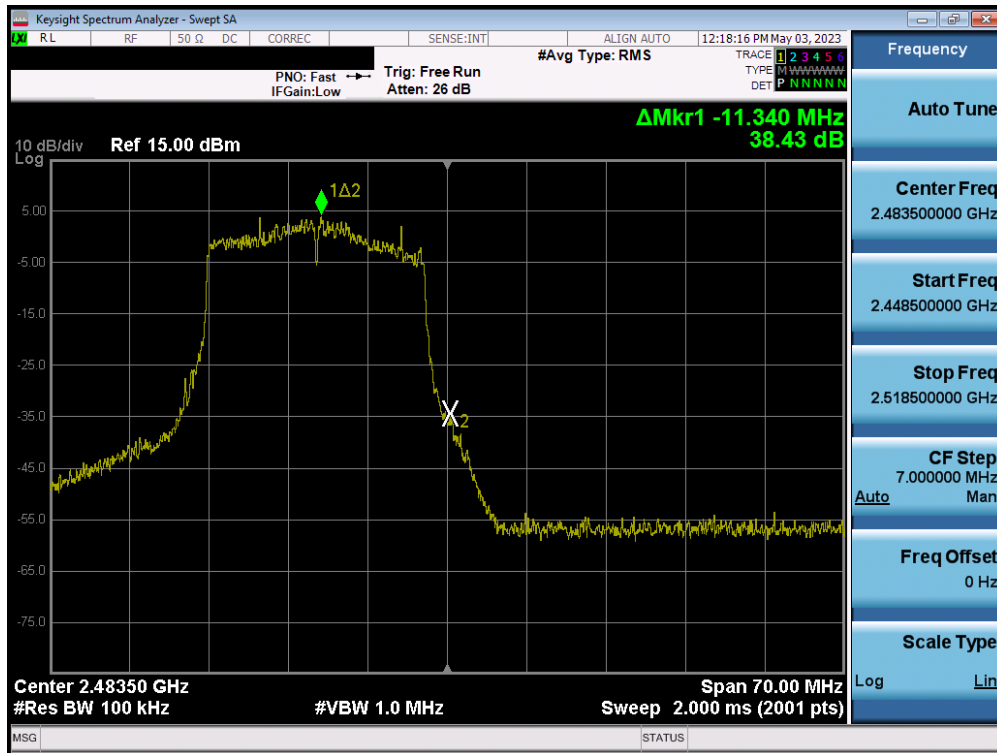
Plot 7-90. Band Edge Plot MIMO ANT1 (802.11ax (2.4GHz) – Ch. 13)
