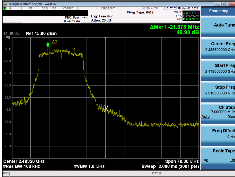
Plot 7-97. Band Edge Plot MIMO ANT2 (802.11g – Ch. 12)
