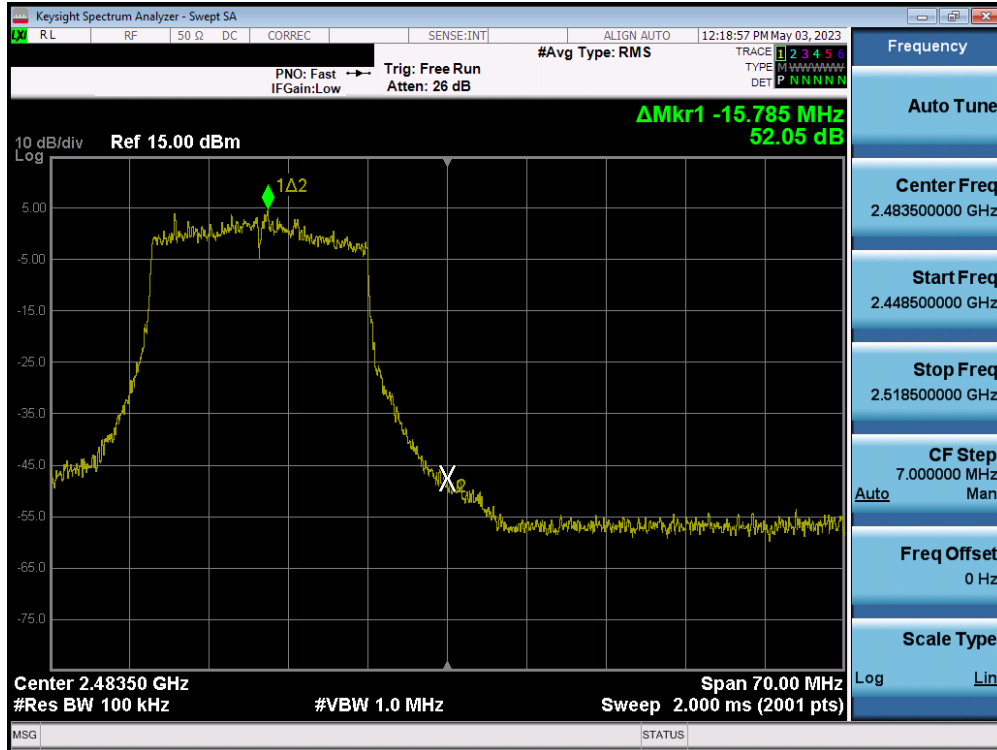
Plot 7-89. Band Edge Plot MIMO ANT1 (802.11ax (2.4GHz) – Ch. 12)
