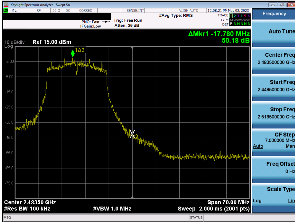
Plot 7-101. Band Edge Plot MIMO ANT2 (802.11n (2.4GHz) – Ch. 12)
