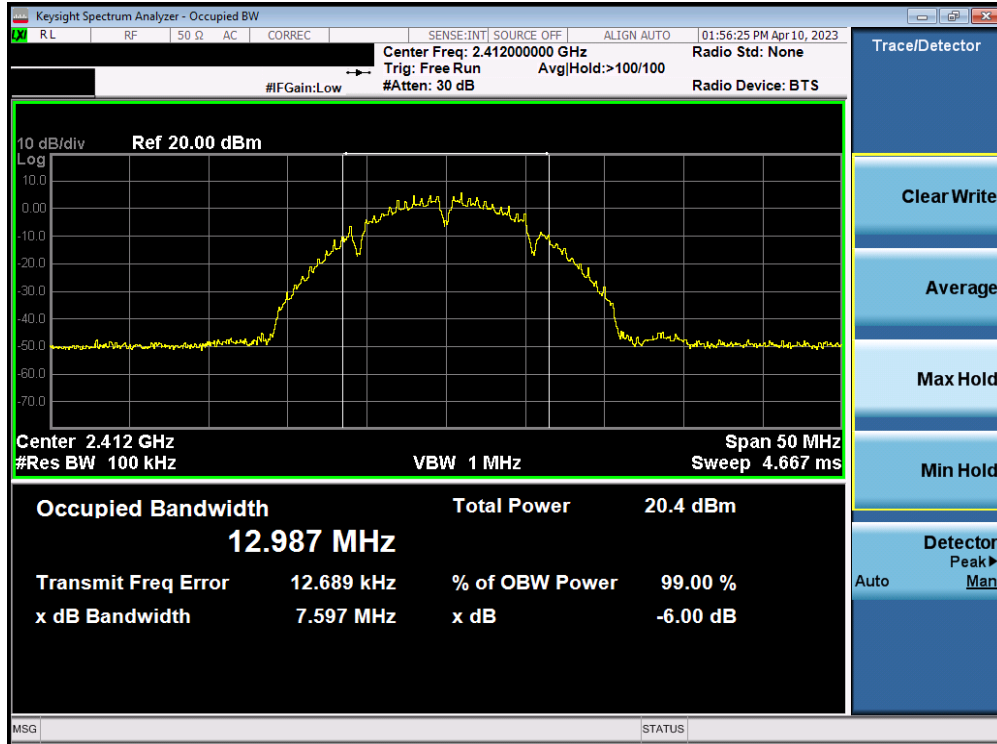
Plot 7-4. 6dB Bandwidth Plot MIMO ANT1 (802.11b – Ch. 1)
