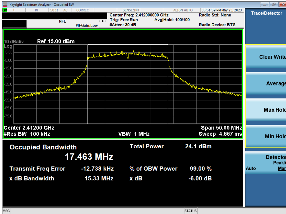
Plot 7-13. 6dB Bandwidth Plot MIMO ANT1 (802.11ac (2.4GHz) – Ch. 1)
