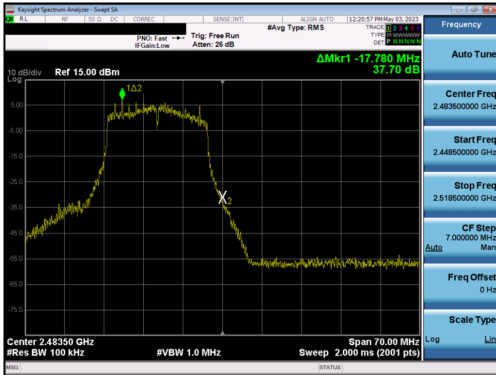
Plot 7-82. Band Edge Plot MIMO ANT1 (802.11n (2.4GHz) – Ch. 13)
