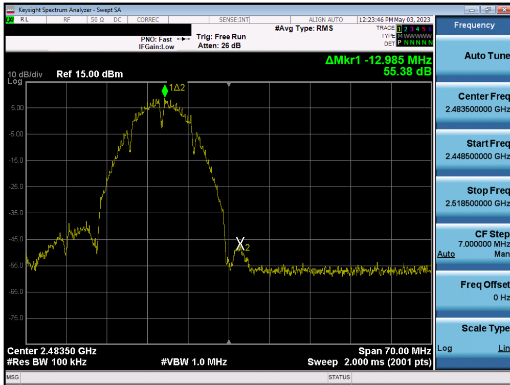
Plot 7-74. Band Edge Plot MIMO ANT1 (802.11b – Ch. 13)
