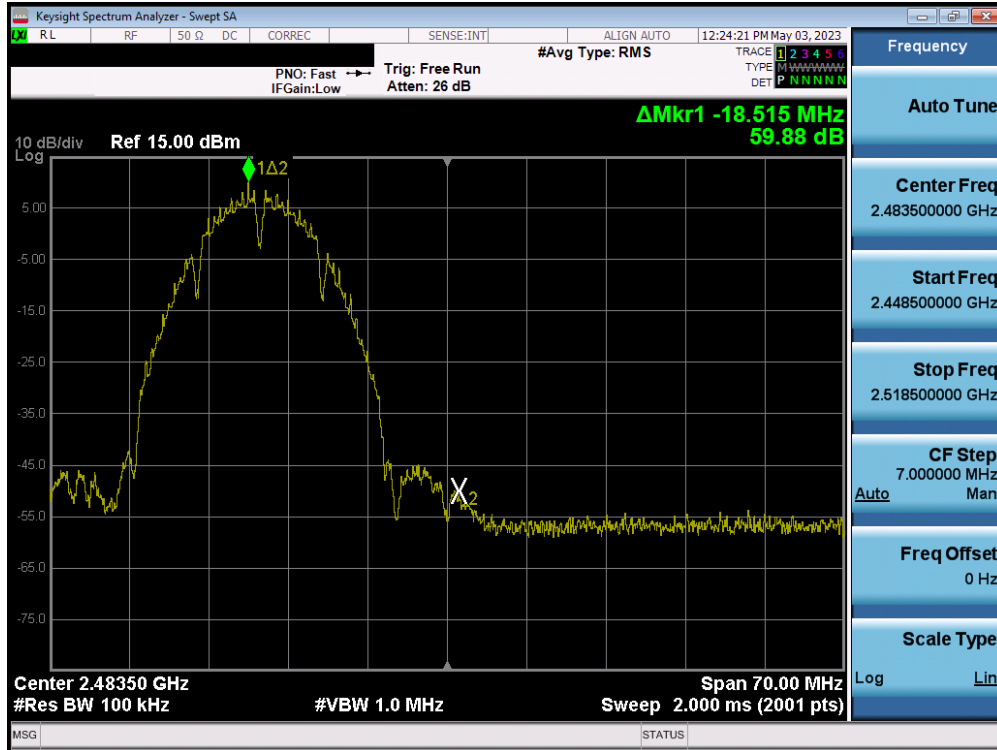
Plot 7-73. Band Edge Plot MIMO ANT1 (802.11b – Ch. 12)
