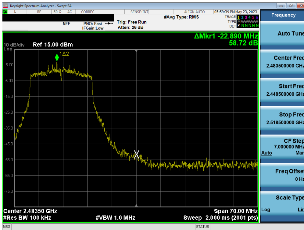
Plot 7-84. Band Edge Plot MIMO ANT1 (802.11ac (2.4GHz) – Ch. 11)
