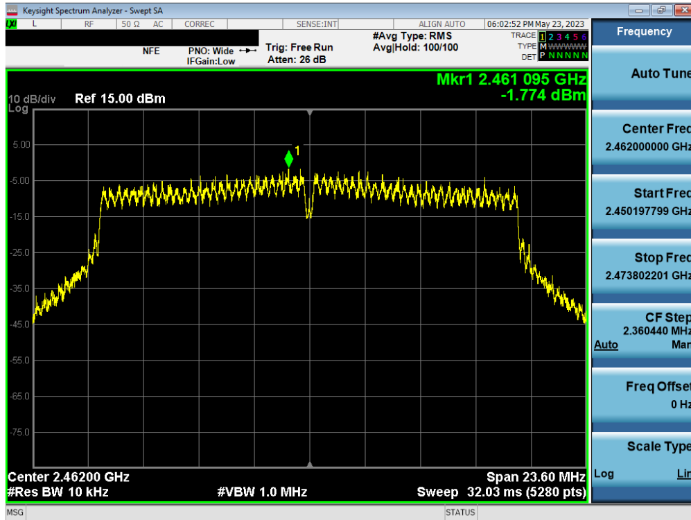
Plot 7-63. Power Spectral Density Plot MIMO ANT2 (802.11ac (2.4GHz) – Ch. 11)
