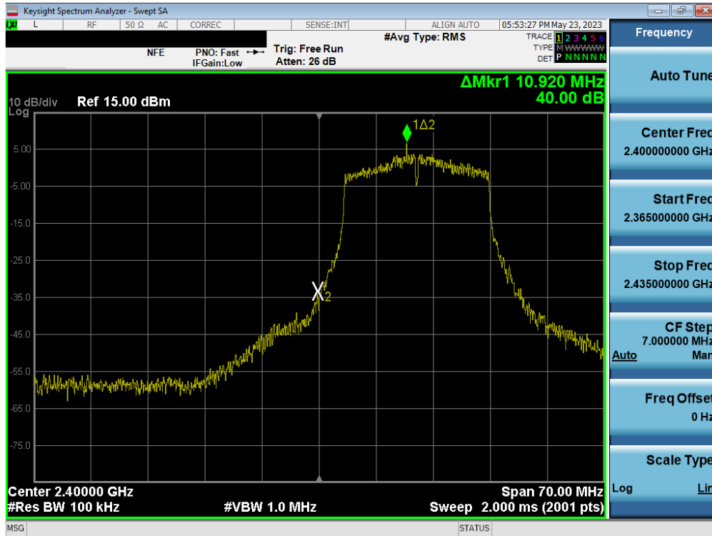
Plot 7-83. Band Edge Plot MIMO ANT1 (802.11ac (2.4GHz) – Ch. 1)
