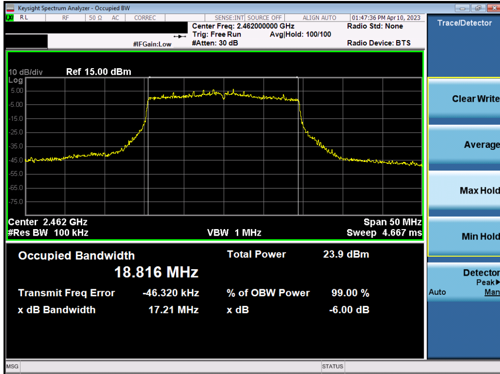
Plot 7-18. 6dB Bandwidth Plot MIMO ANT1 (802.11ax (2.4GHz) – Ch. 11)
