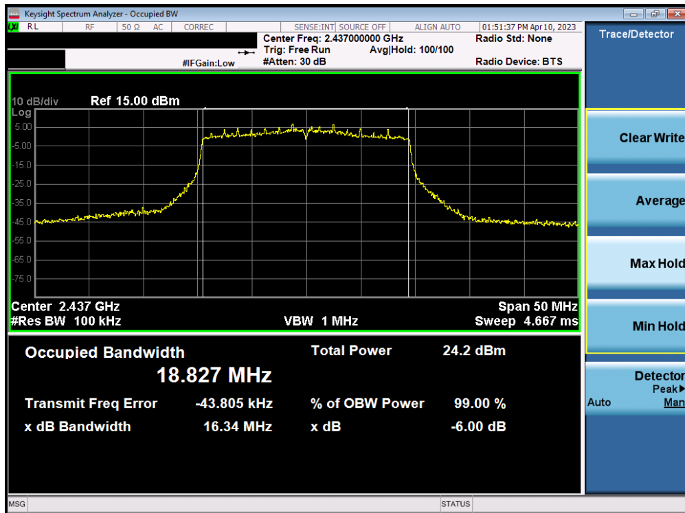
Plot 7-17. 6dB Bandwidth Plot MIMO ANT1 (802.11ax (2.4GHz) – Ch. 6)
