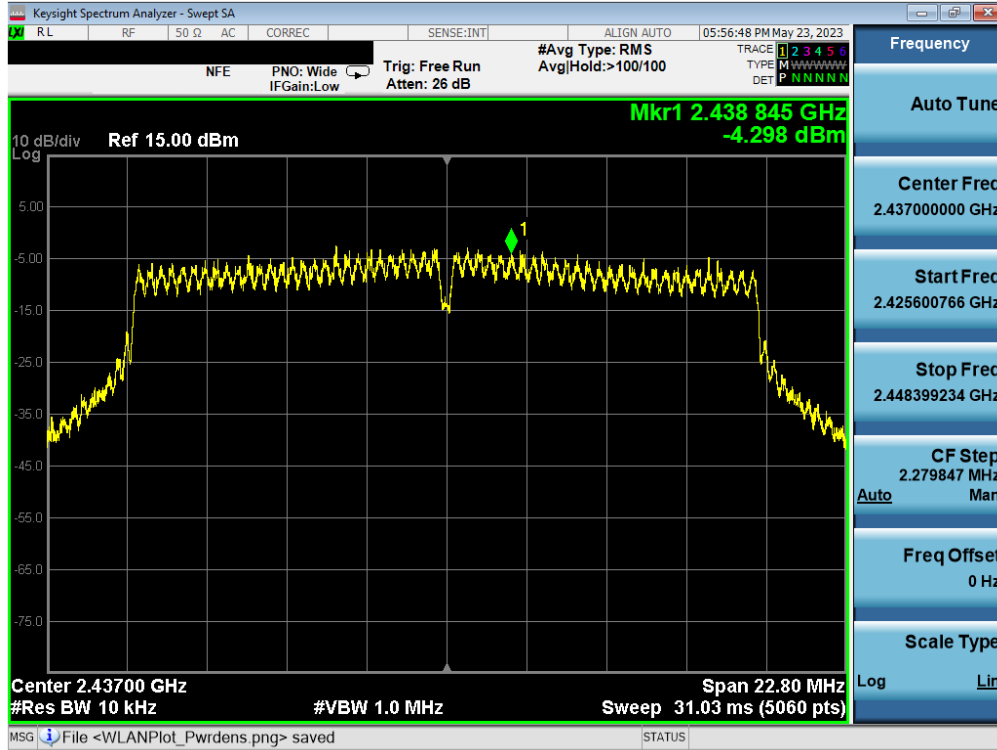
Plot 7-47. Power Spectral Density Plot MIMO ANT1 (802.11ac (2.4GHz) – Ch. 6)
