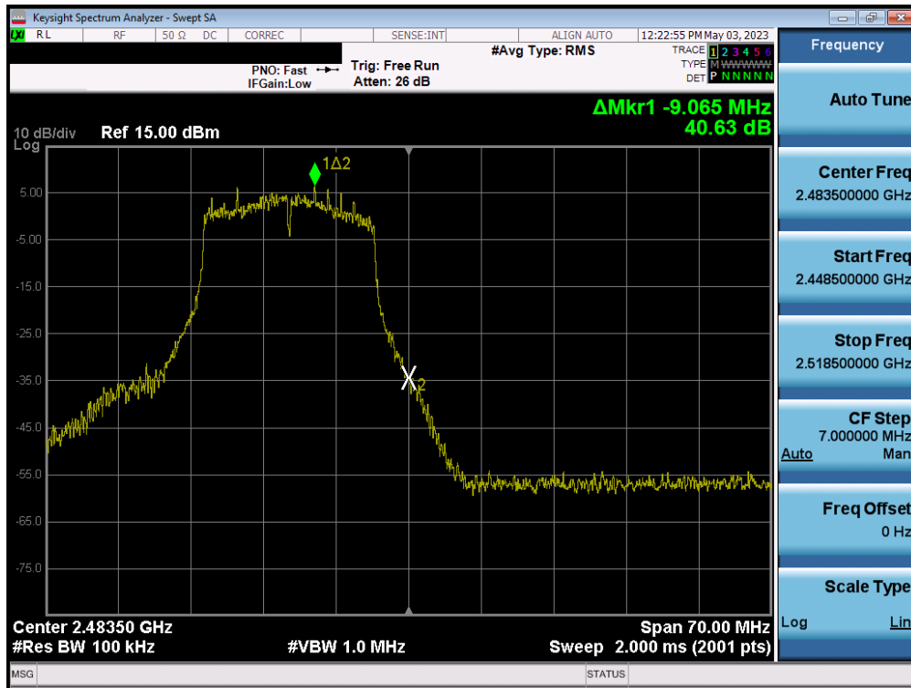
Plot 7-78. Band Edge Plot MIMO ANT1 (802.11g – Ch. 13)
