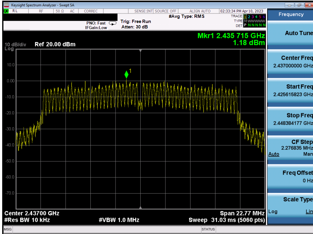
Plot 7-59. Power Spectral Density Plot MIMO ANT2 (802.11n (2.4GHz) – Ch. 6)
