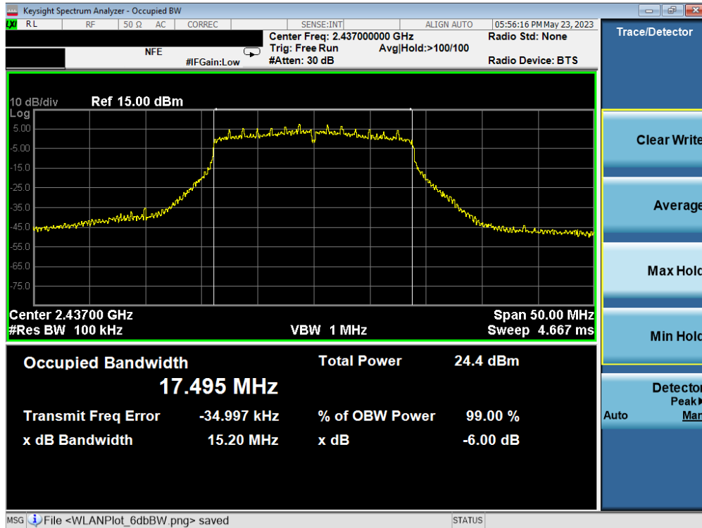
Plot 7-14. 6dB Bandwidth Plot MIMO ANT1 (802.11ac (2.4GHz) – Ch. 6)
