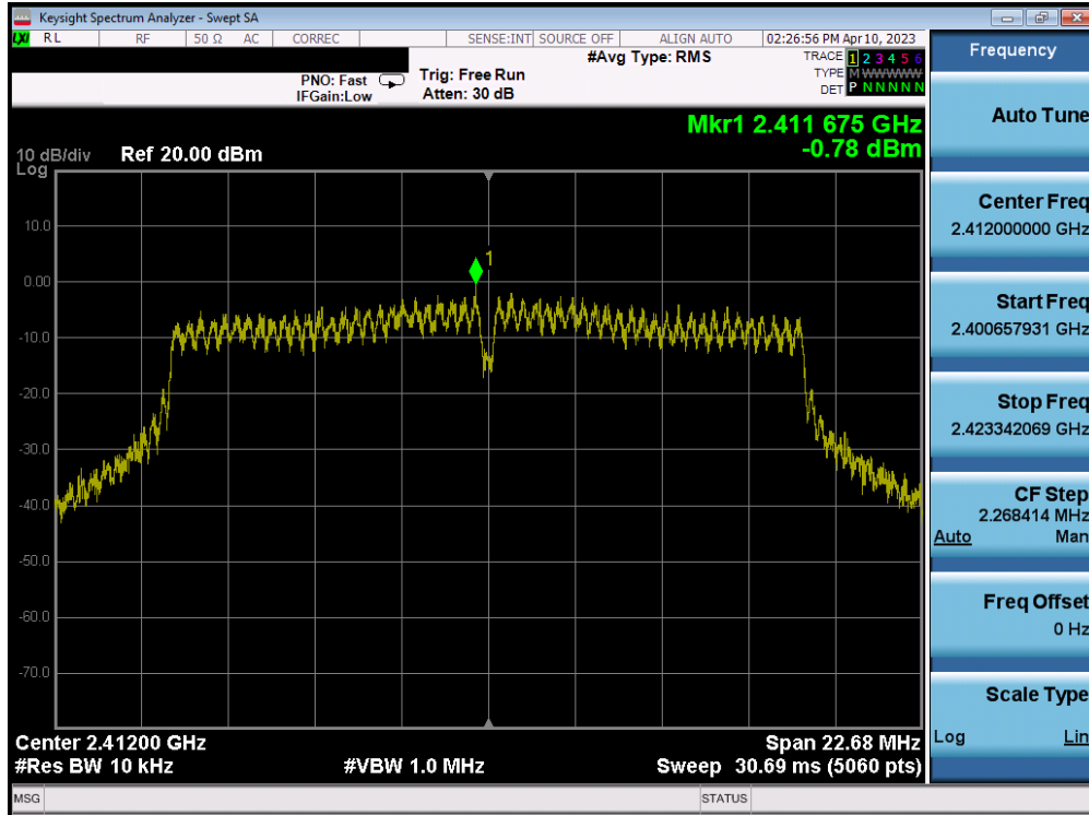
Plot 7-55. Power Spectral Density Plot MIMO ANT2 (802.11g – Ch. 1)
