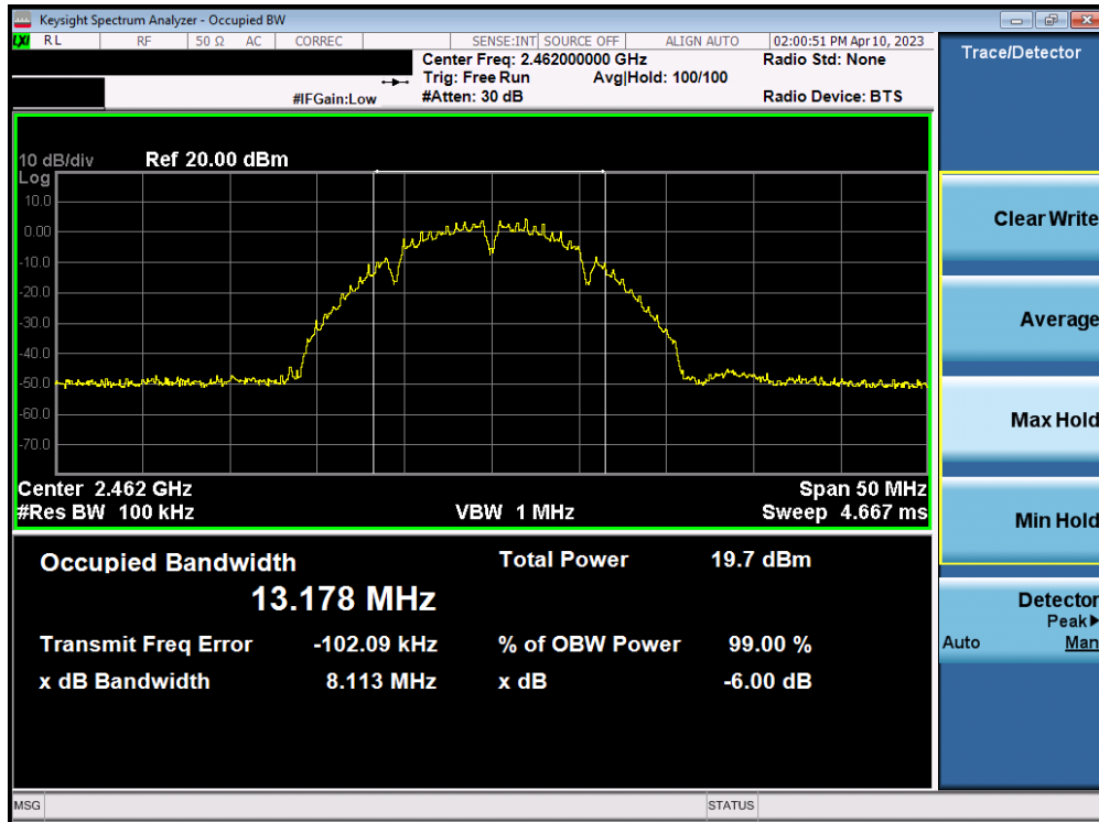
Plot 7-6. 6dB Bandwidth Plot MIMO ANT1 (802.11b – Ch. 11)
