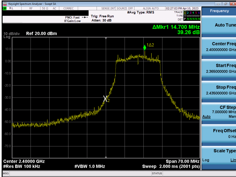
Plot 7-95. Band Edge Plot MIMO ANT2 (802.11g– Ch. 1)
