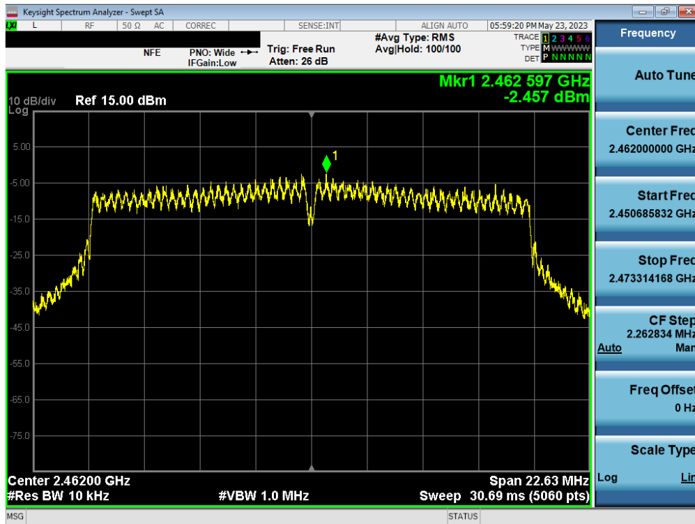
Plot 7-48. Power Spectral Density Plot MIMO ANT1 (802.11ac (2.4GHz) – Ch. 11)
