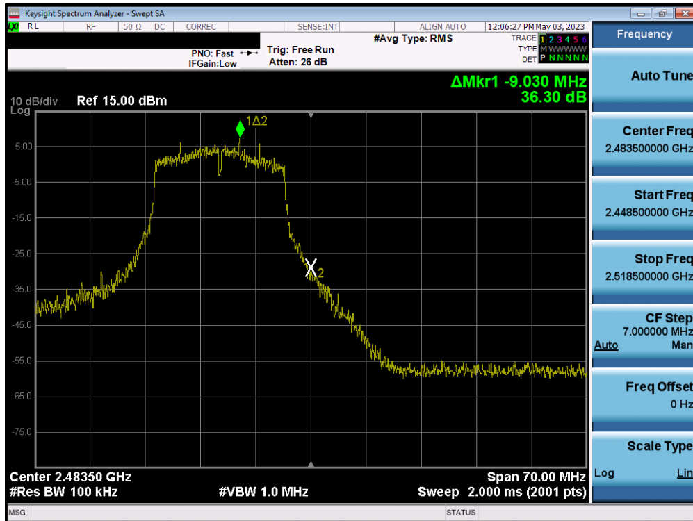
Plot 7-98. Band Edge Plot MIMO ANT2 (802.11g – Ch. 13)
