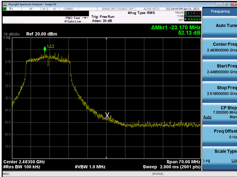
Plot 7-96. Band Edge Plot MIMO ANT2 (802.11g – Ch. 11)
