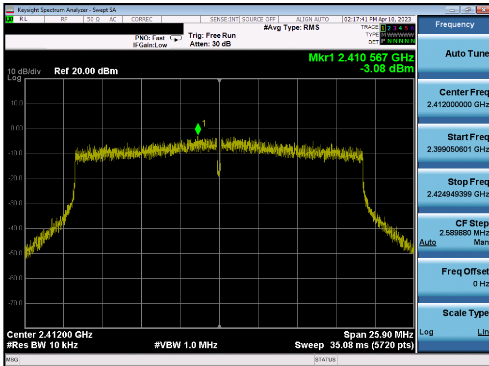
Plot 7-64. Power Spectral Density Plot MIMO ANT2 (802.11ax (2.4GHz) – Ch. 1)
