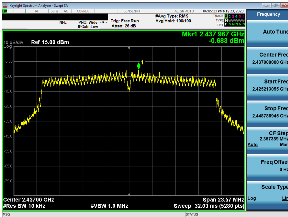
Plot 7-62. Power Spectral Density Plot MIMO ANT2 (802.11ac (2.4GHz) – Ch. 6)
