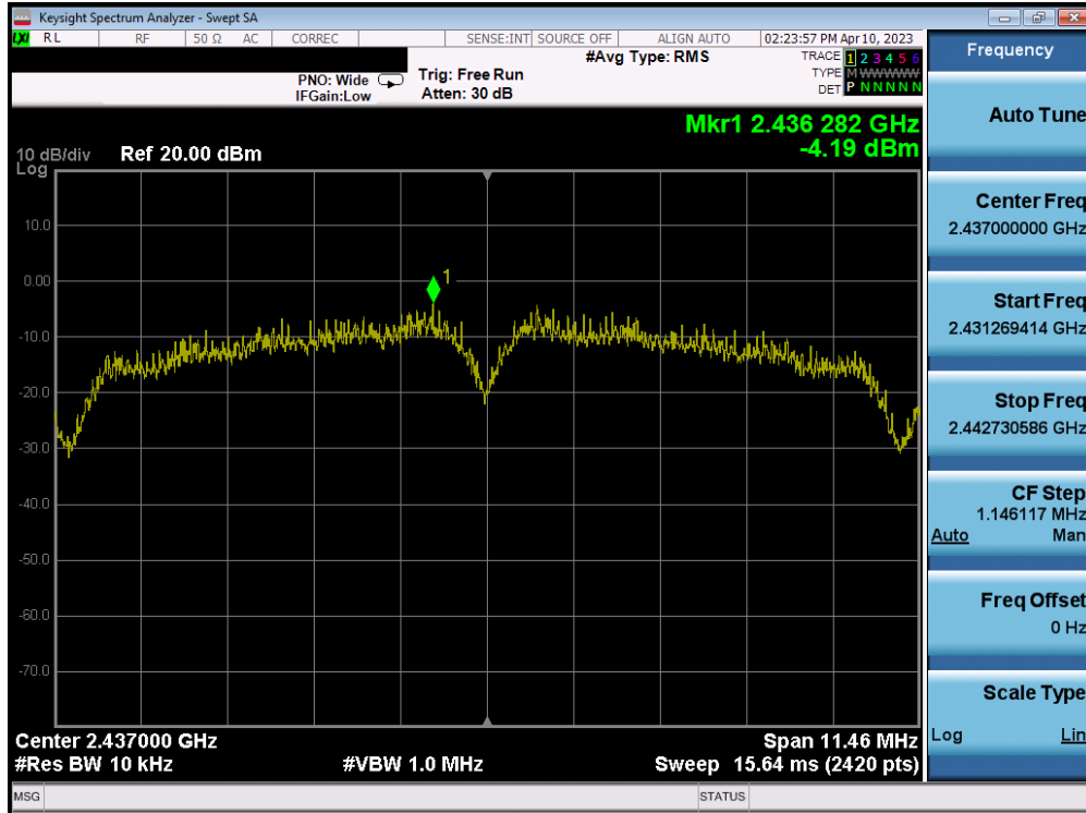
Plot 7-53. Power Spectral Density Plot MIMO ANT2 (802.11b – Ch. 6)
