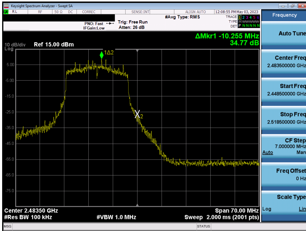
Plot 7-102. Band Edge Plot MIMO ANT2 (802.11n (2.4GHz) – Ch. 13)
