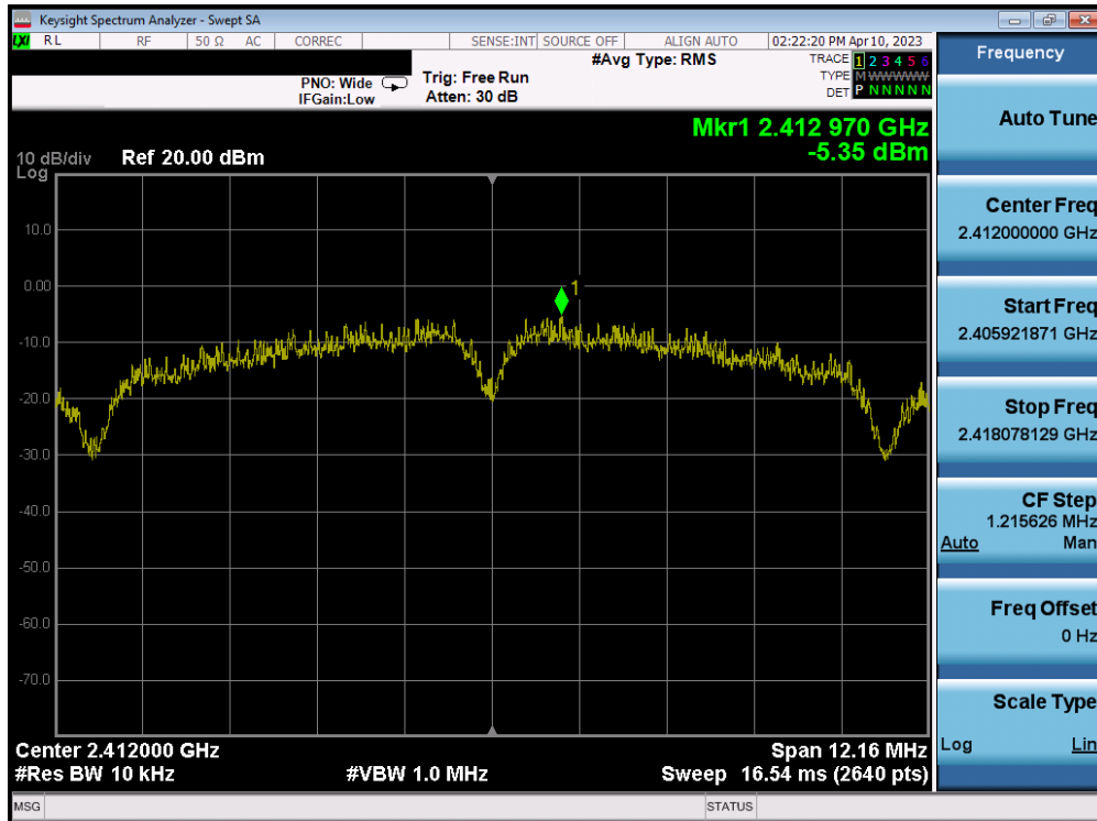
Plot 7-52. Power Spectral Density Plot MIMO ANT2 (802.11b – Ch. 1)
