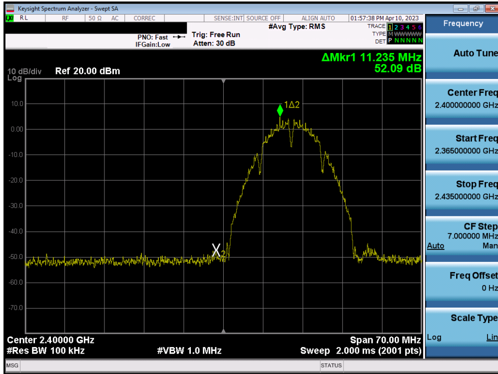
Plot 7-71. Band Edge Plot MIMO ANT1 (802.11b – Ch. 1)
