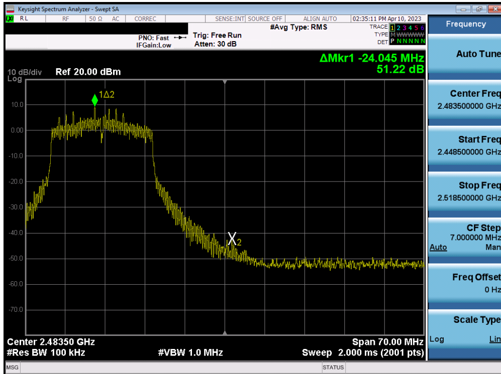
Plot 7-100. Band Edge Plot MIMO ANT2 (802.11n (2.4GHz) – Ch. 11)
