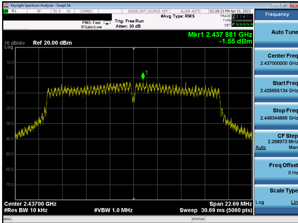
Plot 7-56. Power Spectral Density Plot MIMO ANT2 (802.11g – Ch. 6)
