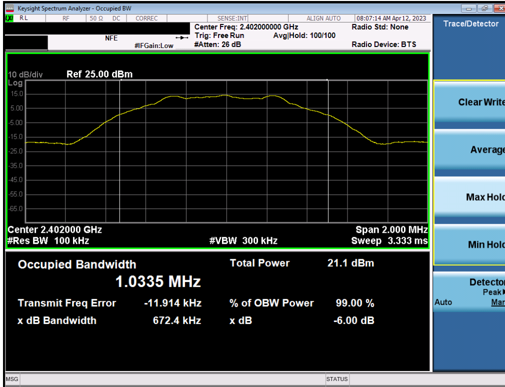
Plot 7-7. 6dB Bandwidth Plot (Bluetooth (LE), 1Mbps - Ch. 0) - ANT 1
