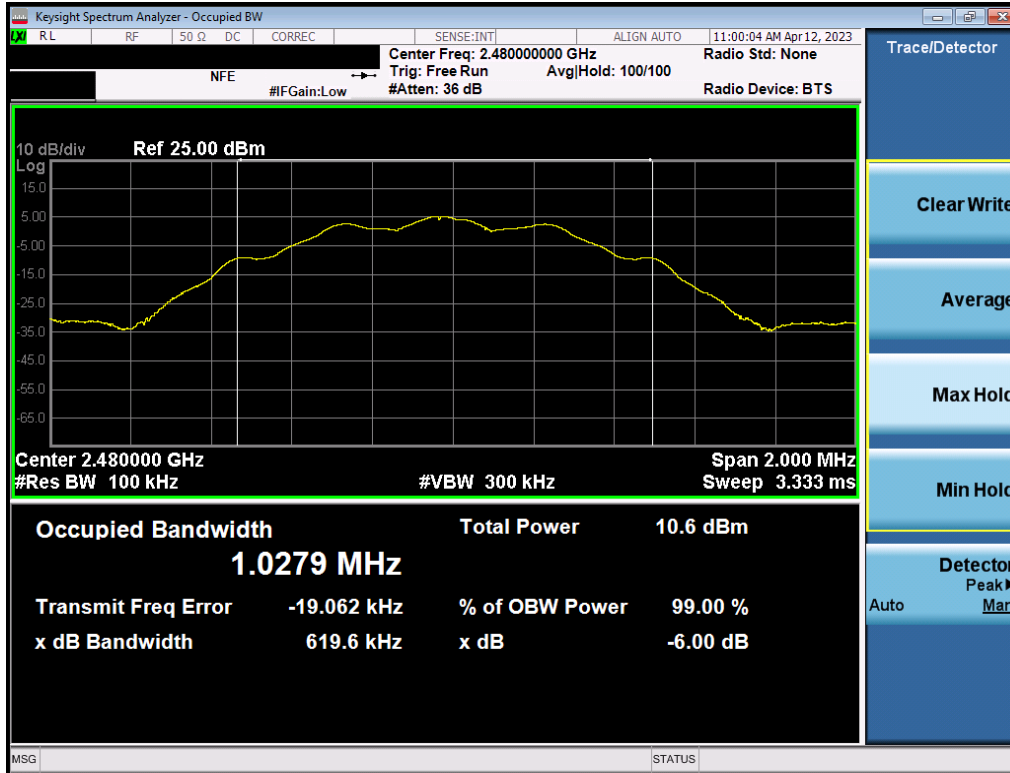
Plot 7-15. 6dB Bandwidth Plot (Bluetooth (LE), 125kbps – Ch. 39) – ANT 2
