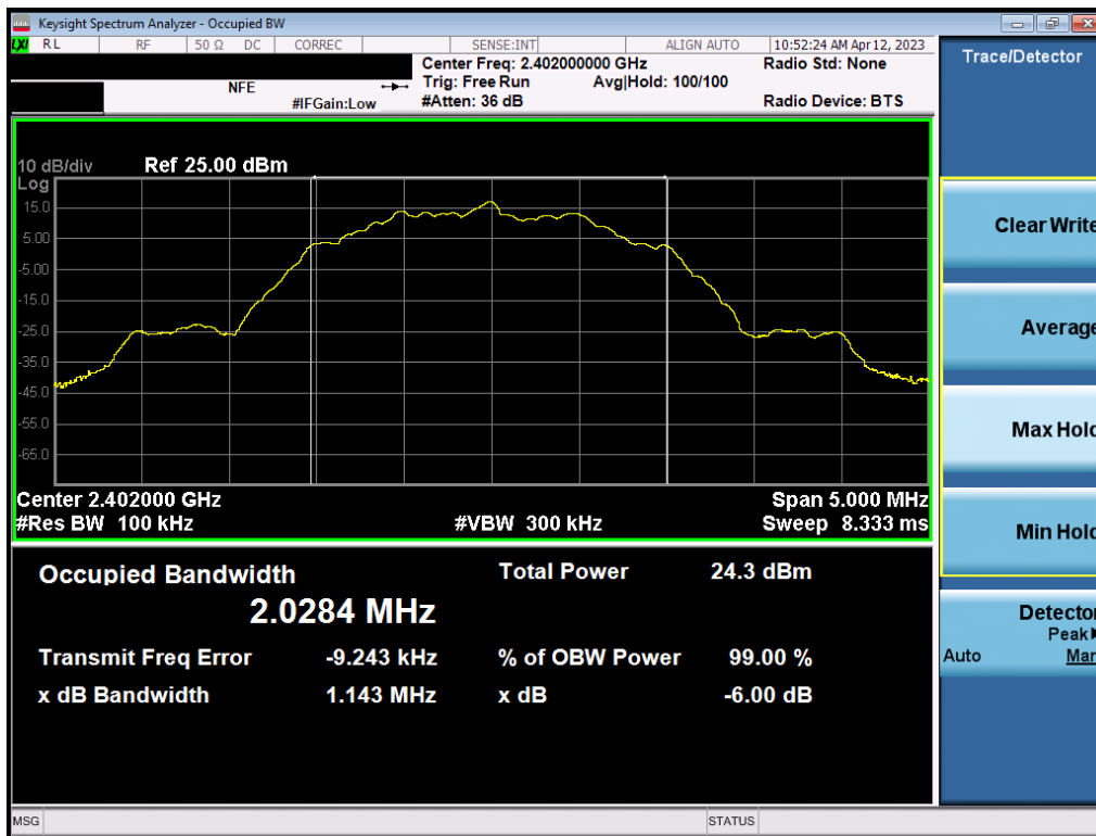
Plot 7-22. 6dB Bandwidth Plot (Bluetooth (LE), 2Mbps – Ch. 0) – ANT 2
