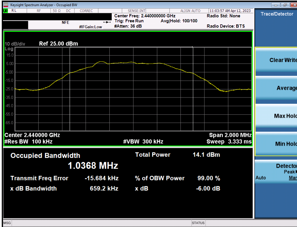
Plot 7-17. 6dB Bandwidth Plot (Bluetooth (LE), 500kbps – Ch. 19) – ANT 2
