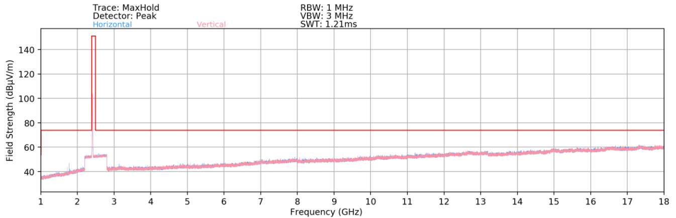
Plot 7-88. Radiated Spurious Plot above 1GHz SISO ANT2 (802.11b – Ch. 1) – Open
