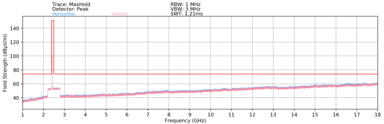
Plot 7-80. Radiated Spurious Plot above 1GHz SISO ANT1 (802.11b – Ch. 1) – Half Open
