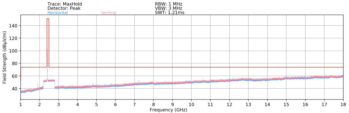
Plot 7-77. Radiated Spurious Plot above 1GHz SISO ANT1 (802.11b – Ch. 1) – Open
