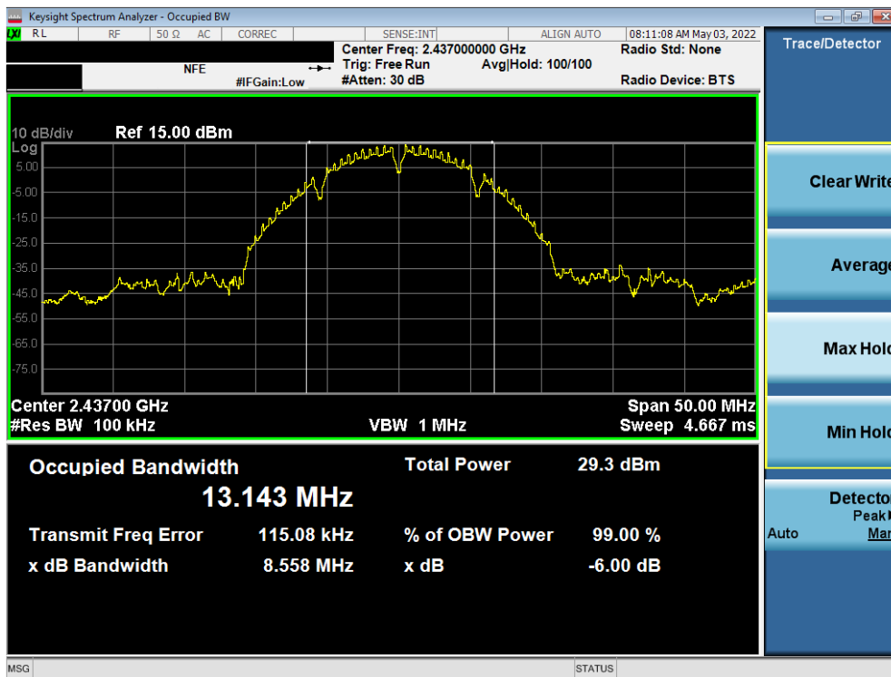
Plot 7-2. 6dB Bandwidth Plot SISO ANT1 (802.11b – Ch. 6)
