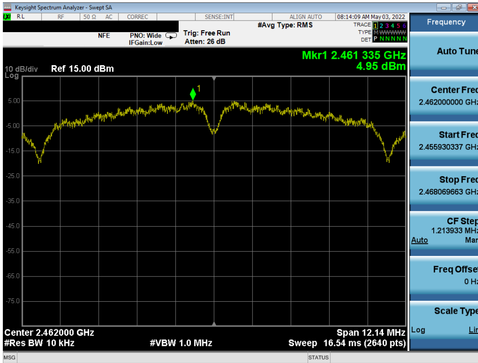
Plot 7-27. Power Spectral Density Plot SISO ANT1 (802.11b – Ch. 11)
