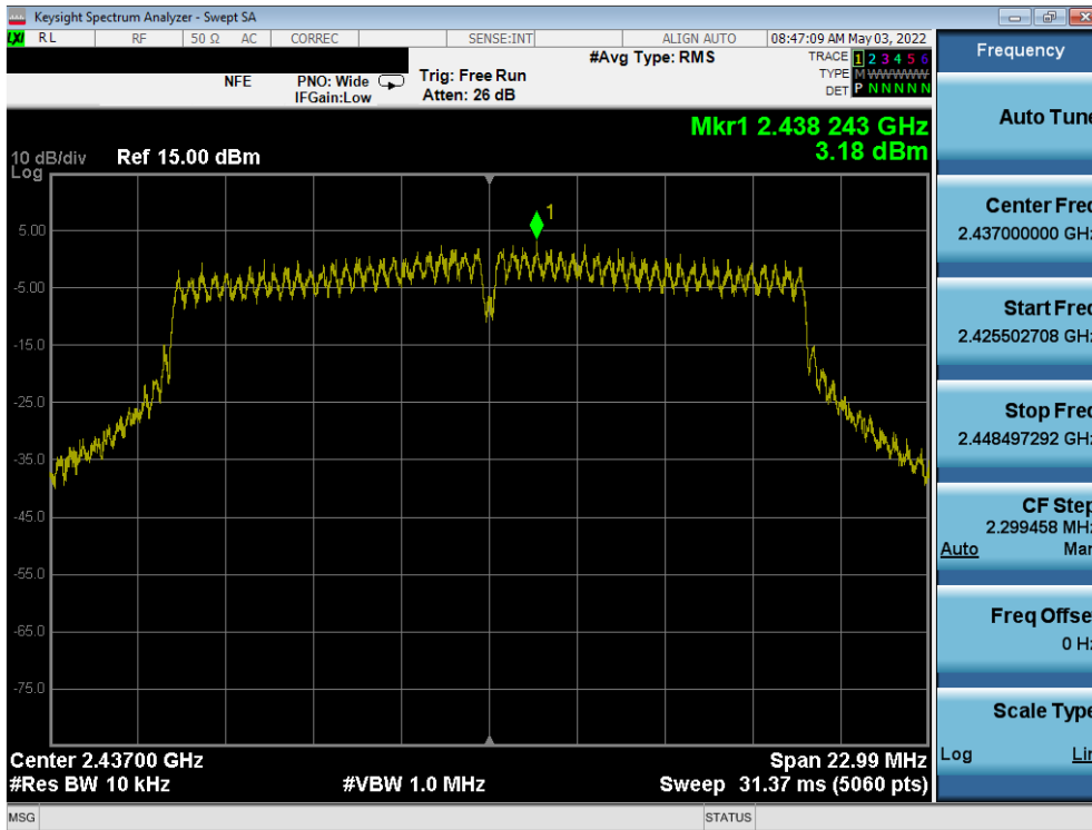
Plot 7-29. Power Spectral Density Plot SISO ANT1 (802.11g – Ch. 6)
