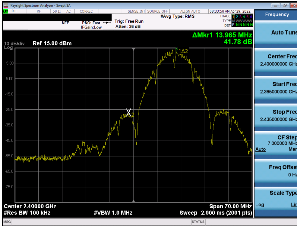
Plot 7-57. Band Edge Plot SISO ANT2 (802.11b – Ch. 1)
