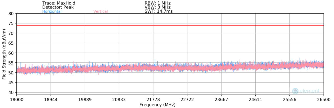
Plot 7-83. Radiated Spurious Plot above 18GHz SISO ANT1 – Open
