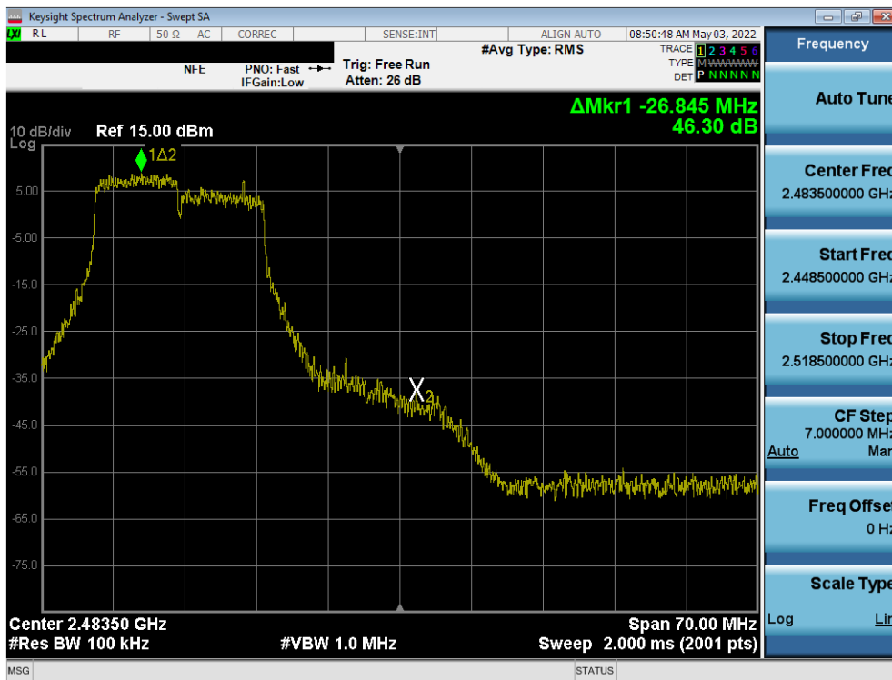
Plot 7-52. Band Edge Plot SISO ANT1 (802.11g - Ch. 11)
