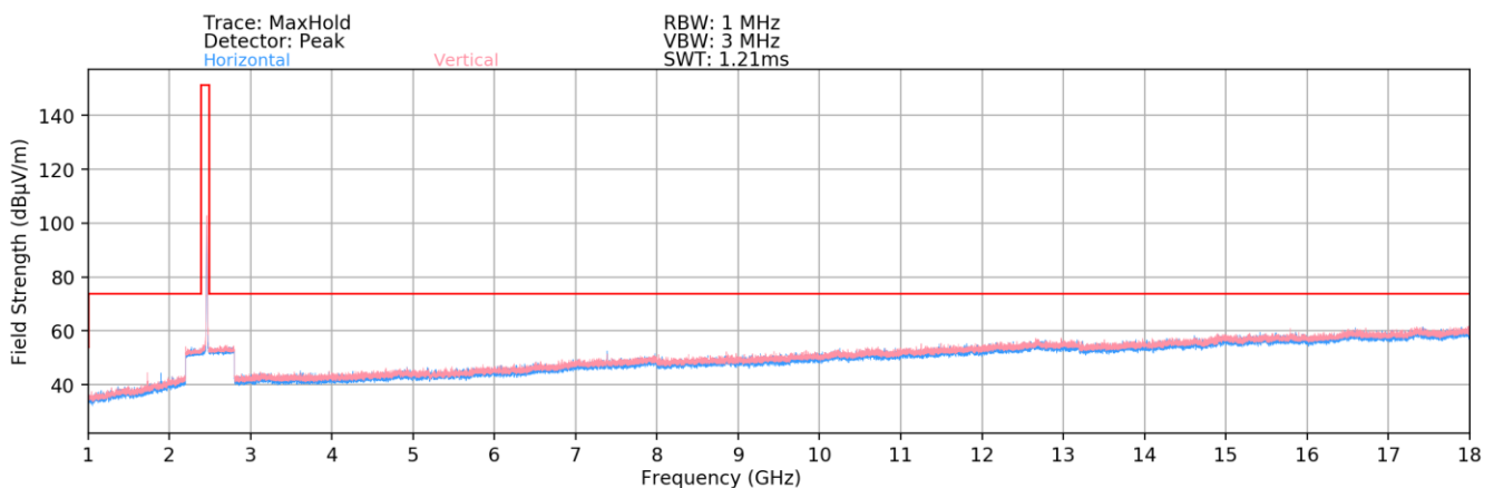
Plot 7-79. Radiated Spurious Plot above 1GHz SISO ANT1 (802.11b – Ch. 11) – Open
