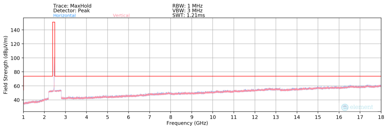
Plot 7-90. Radiated Spurious Plot above 1GHz SISO ANT2 (802.11b – Ch. 11) – Open
