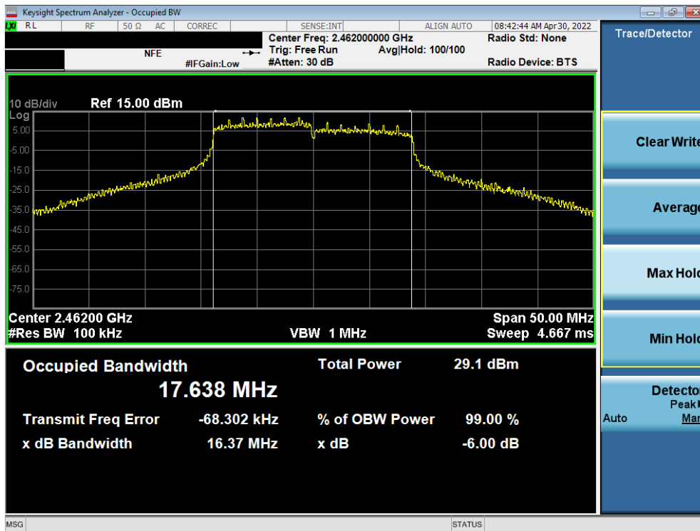
Plot 7-21. 6dB Bandwidth Plot SISO ANT2 (802.11n (2.4GHz) – Ch. 11)
