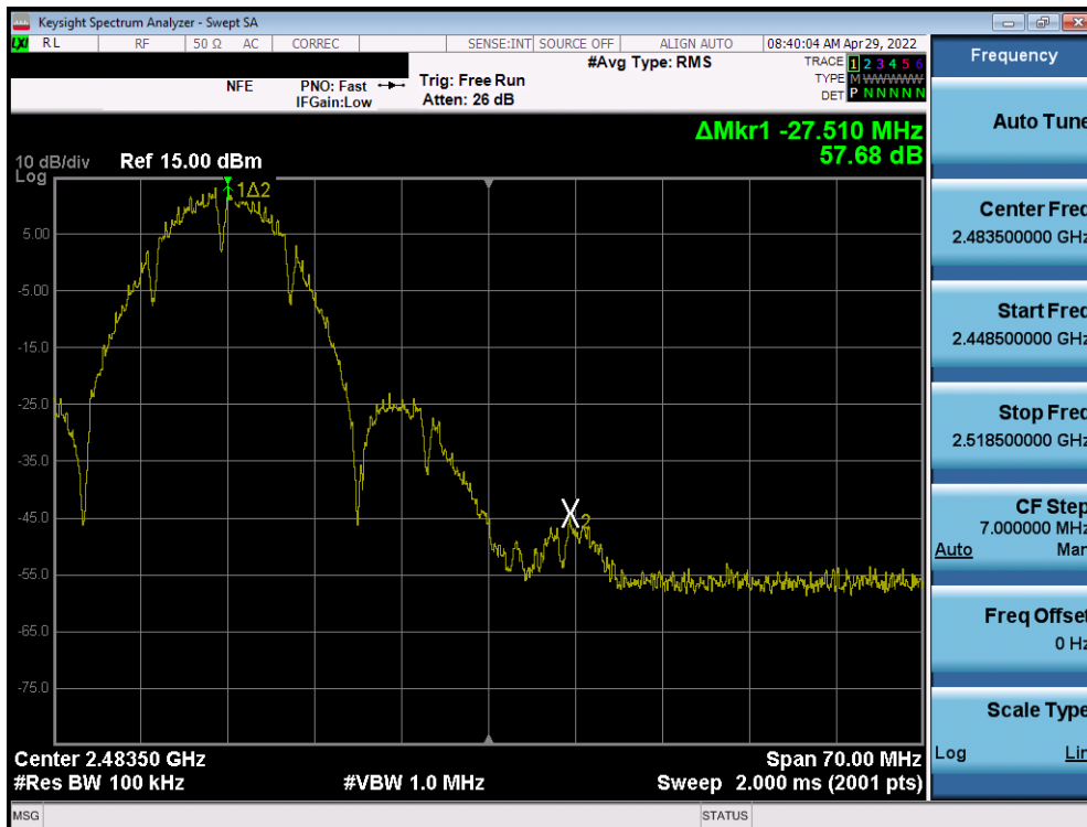
Plot 7-58. Band Edge Plot SISO ANT2 (802.11b – Ch. 11)
