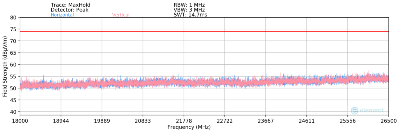
Plot 7-84. Radiated Spurious Plot above 18GHz SISO ANT1 – Half Open
