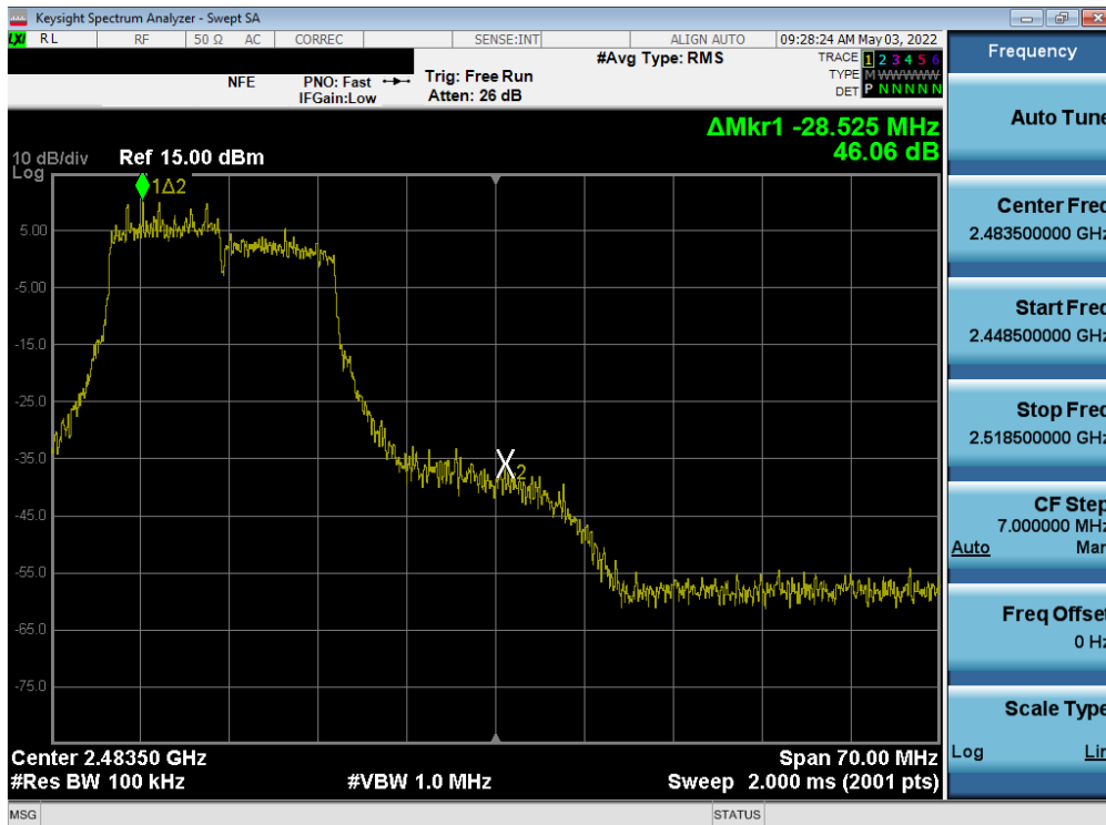
Plot 7-56. Band Edge Plot SISO ANT1 (802.11ax (2.4GHz) – Ch. 11)
