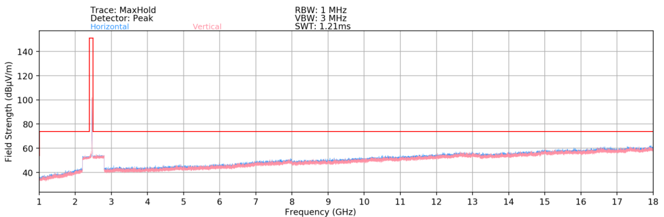
Plot 7-82. Radiated Spurious Plot above 1GHz SISO ANT1 (802.11b – Ch. 11) – Half Open
