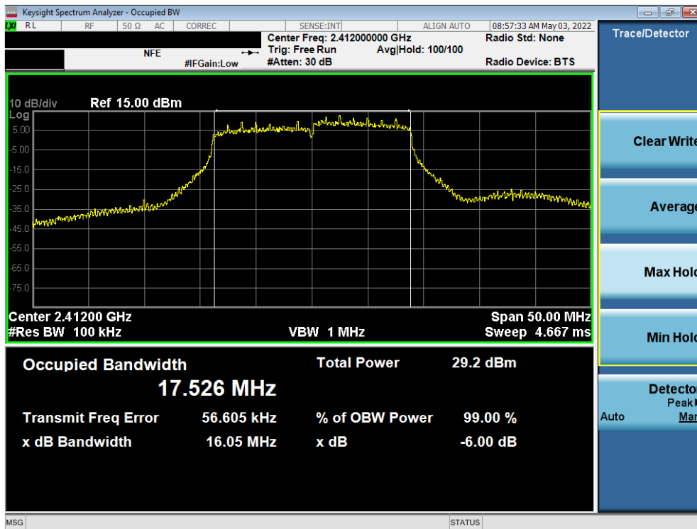
Plot 7-7. 6dB Bandwidth Plot SISO ANT1 (802.11n (2.4GHz) – Ch. 1)
