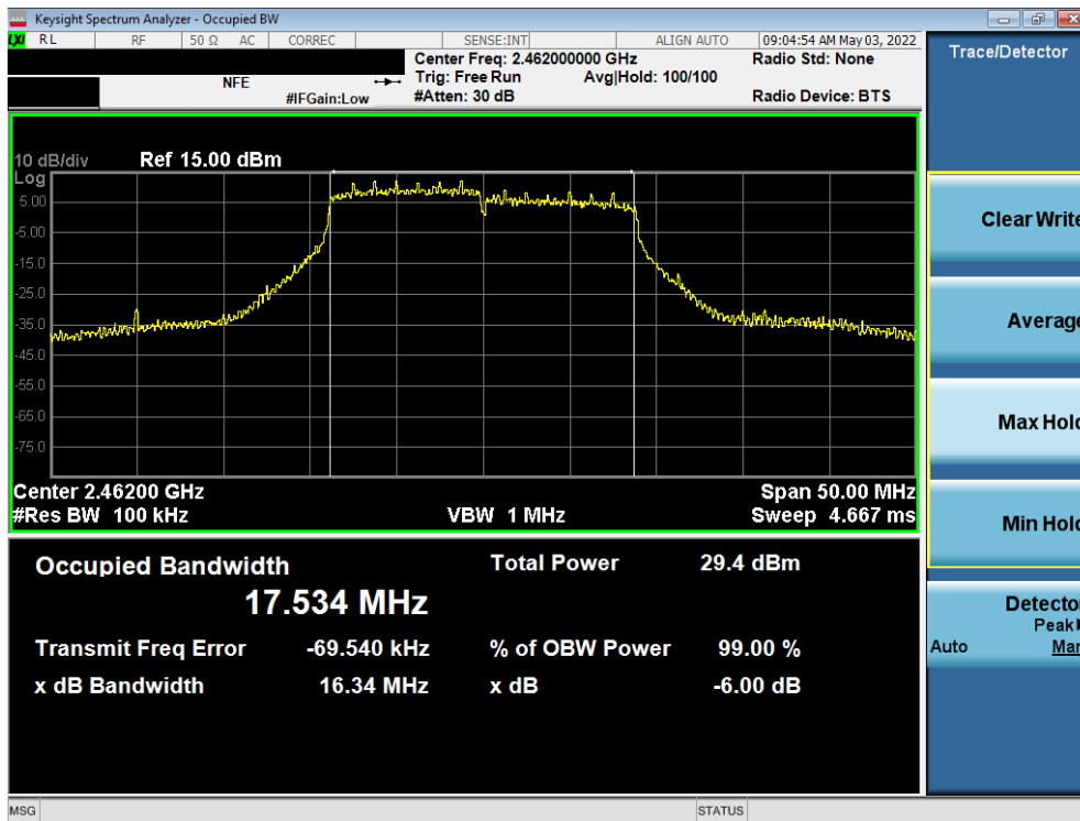
Plot 7-9. 6dB Bandwidth Plot SISO ANT1 (802.11n (2.4GHz) – Ch. 11)
