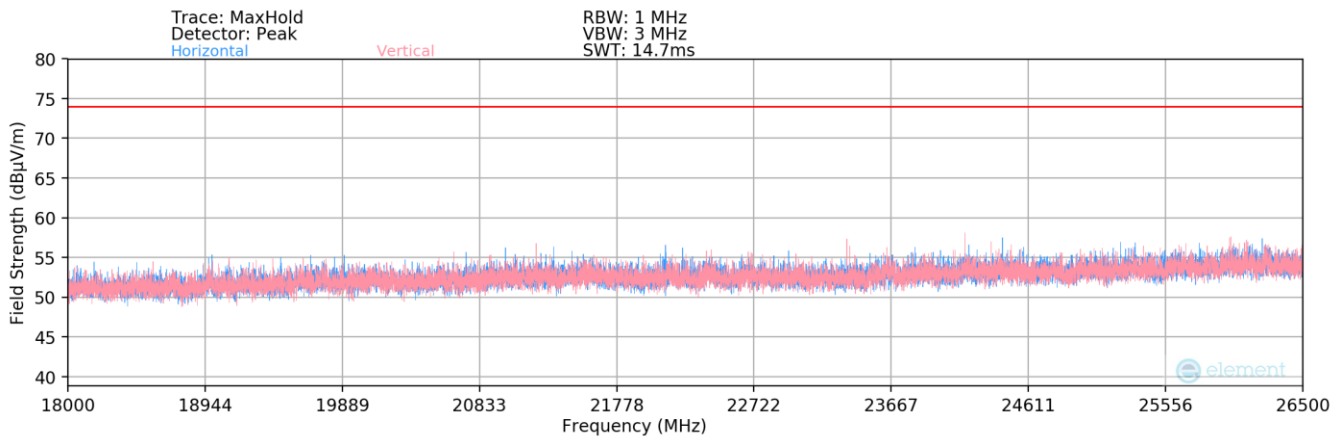
Plot 7-91. Radiated Spurious Plot above 18GHz SISO ANT2 – Half Open
