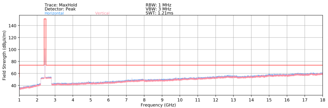
Plot 7-81. Radiated Spurious Plot above 1GHz SISO ANT1 (802.11b – Ch. 6) – Half Open
