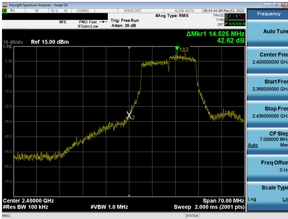
Plot 7-51. Band Edge Plot SISO ANT1 (802.11g- Ch. 1)
