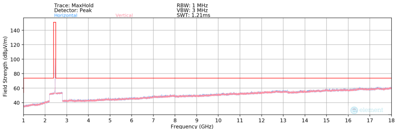
Plot 7-87. Radiated Spurious Plot above 1GHz SISO ANT2 (802.11b – Ch. 11) – Half Open
