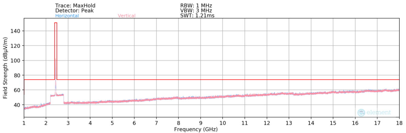
Plot 7-86. Radiated Spurious Plot above 1GHz SISO ANT2 (802.11b – Ch. 6) – Half Open
