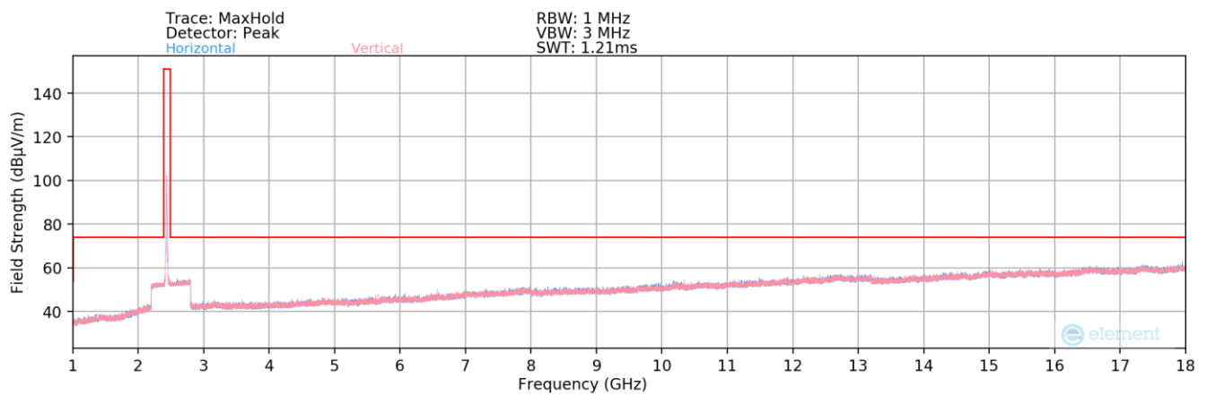
Plot 7-89. Radiated Spurious Plot above 1GHz SISO ANT2 (802.11b – Ch. 6) – Open
