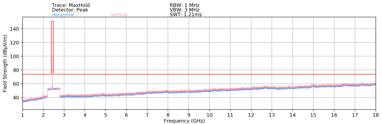
Plot 7-78. Radiated Spurious Plot above 1GHz SISO ANT1 (802.11b – Ch. 6) – Open
