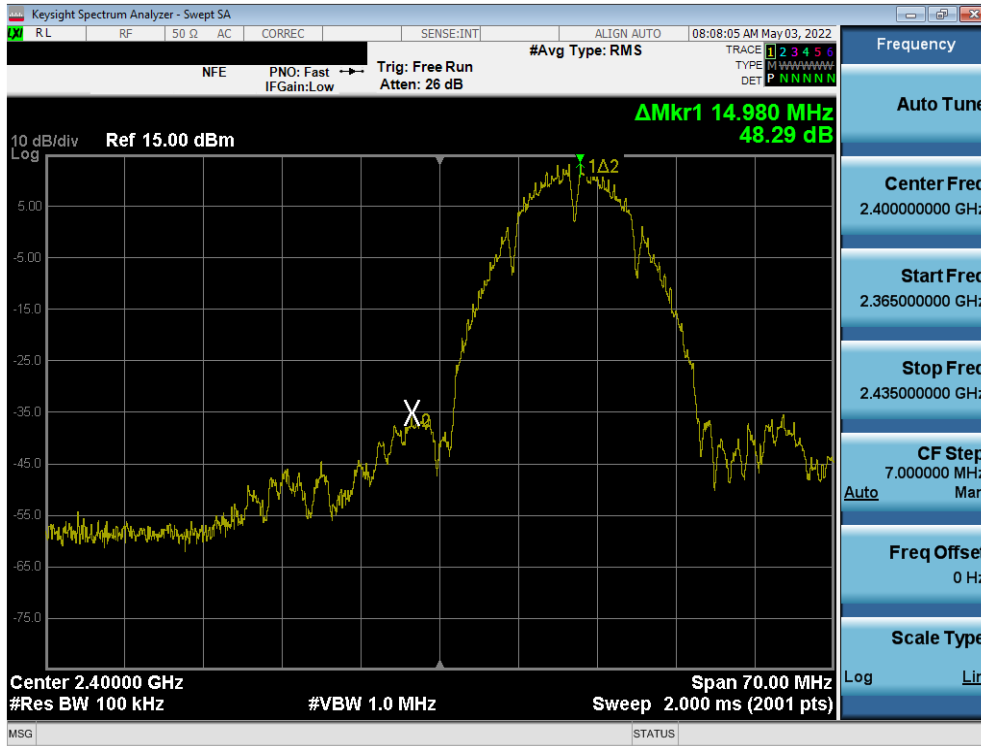
Plot 7-49. Band Edge Plot SISO ANT1 (802.11b – Ch. 1)
