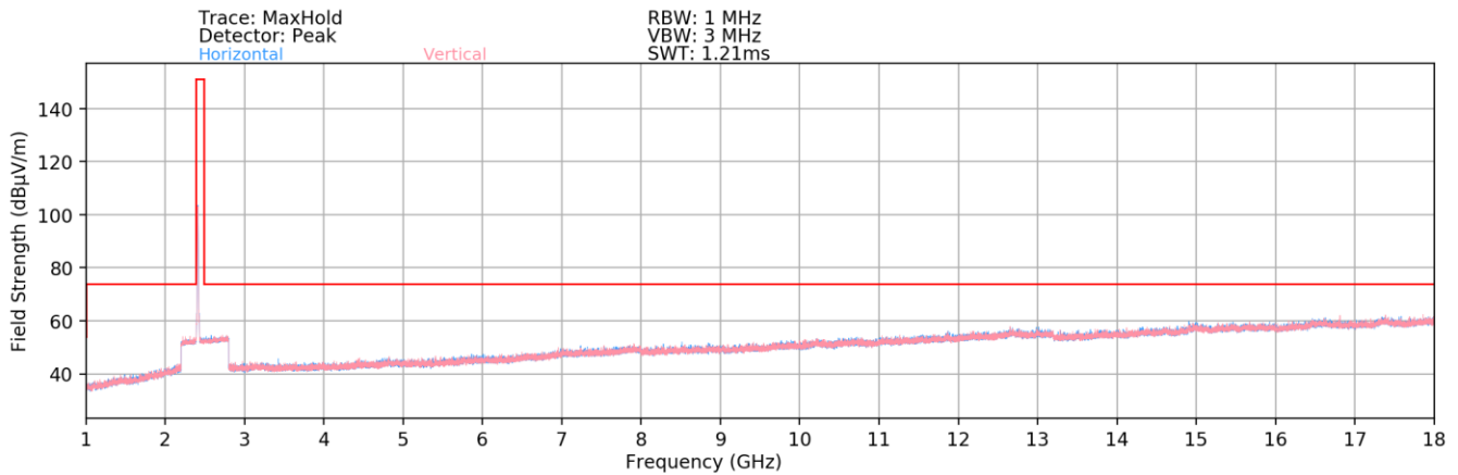
Plot 7-85. Radiated Spurious Plot above 1GHz SISO ANT2 (802.11b – Ch. 1) – Half Open
