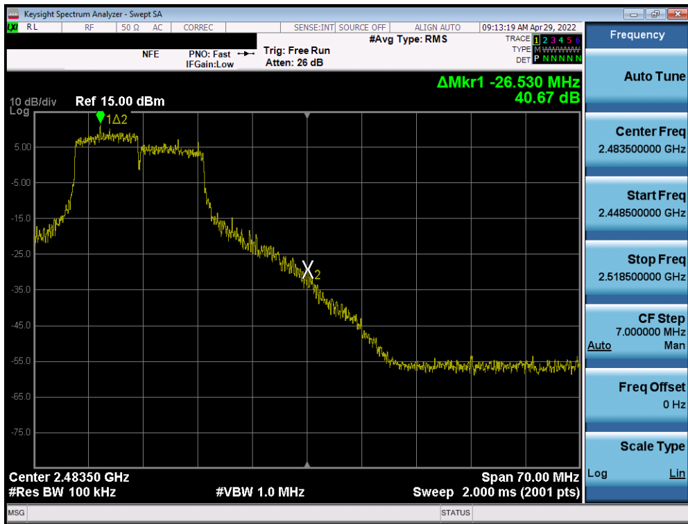
Plot 7-60. Band Edge Plot SISO ANT2 (802.11g - Ch. 11)
