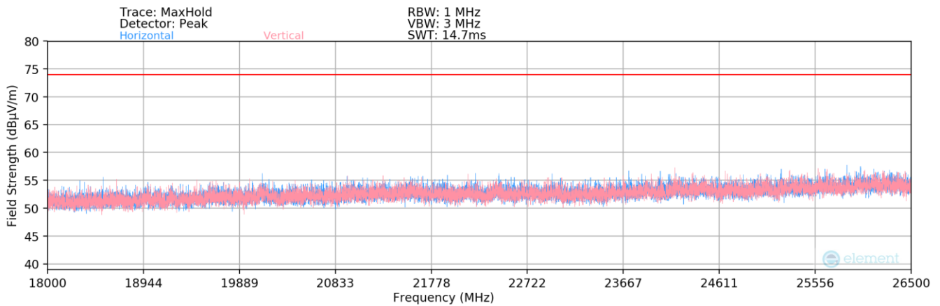
Plot 7-92. Radiated Spurious Plot above 18GHz SISO ANT2 – Open
