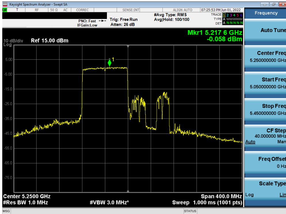
Plot 7-202. Power Spectral Density Plot SISO ANT1 (160MHz L BW 802.11ax – Full Tones (UNII Band 1/2A) – Ch. 50)
