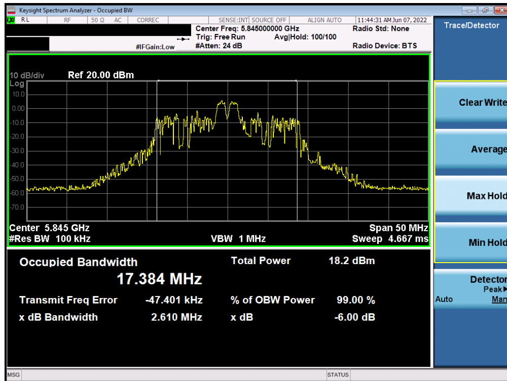
Plot 7-135. 6dB Bandwidth Plot ANT2 (20MHz BW 802.11ax – 26 Tones (UNII Band 3/4) – Ch. 169)
