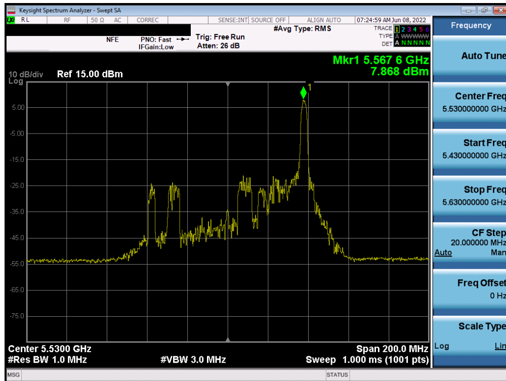
Plot 7-177. Power Spectral Density Plot SISO ANT1 (80MHz BW 802.11ax – 26 Tones (UNII Band 2C) – Ch. 106)
