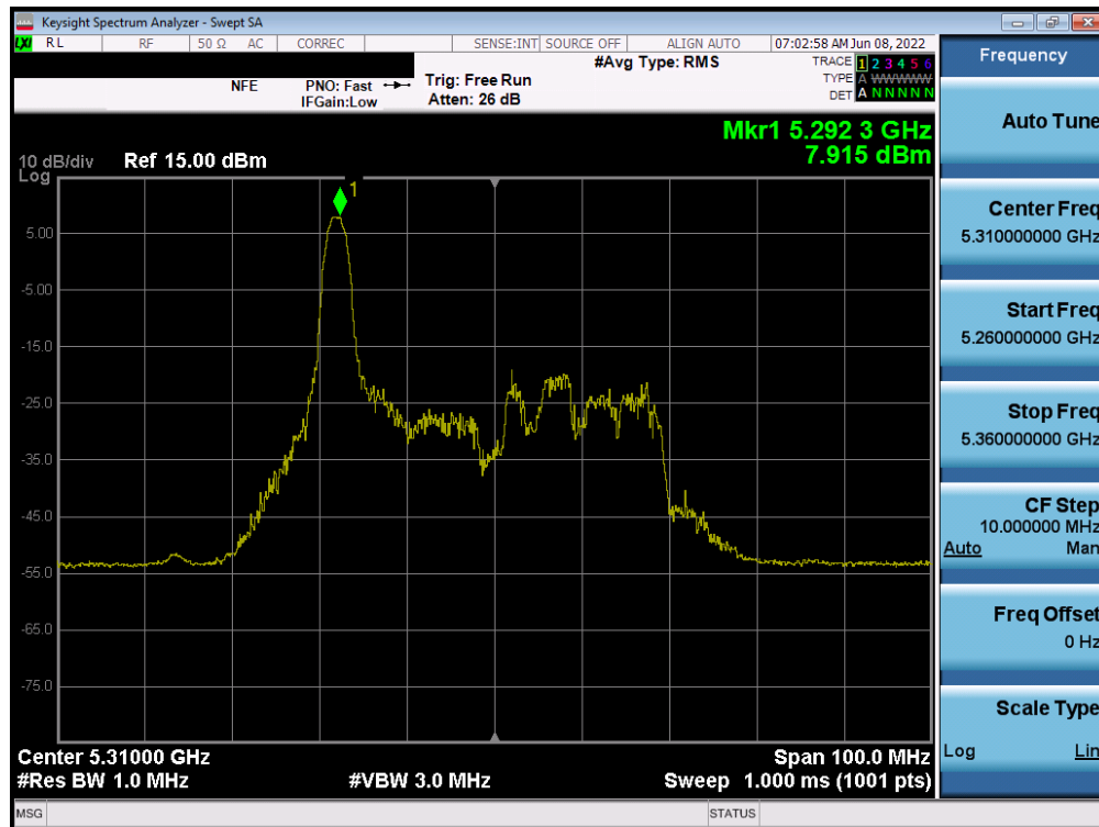
Plot 7-169. Power Spectral Density Plot SISO ANT1 (40MHz BW 802.11ax – 26 Tones (UNII Band 2A) – Ch. 62)
