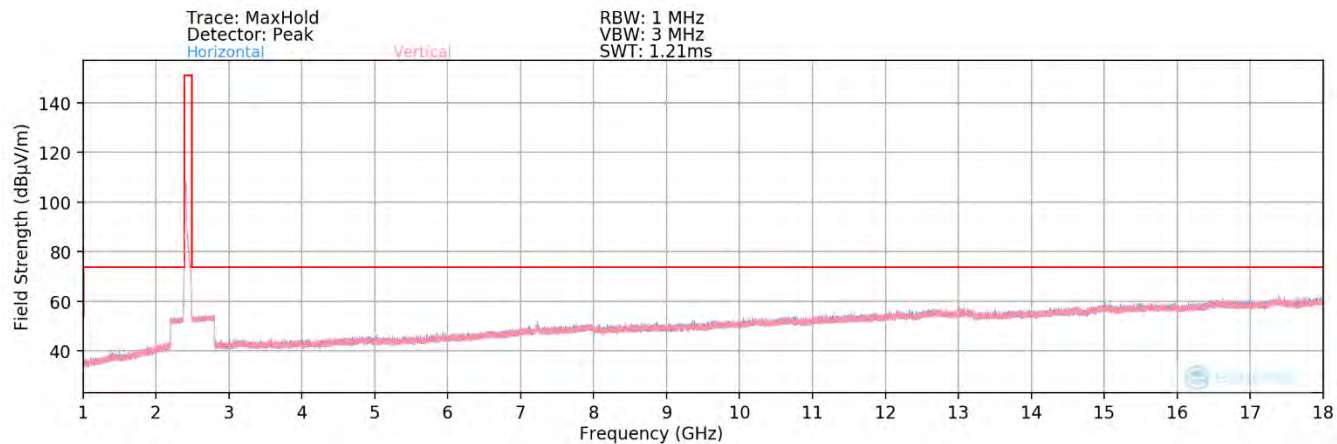
Plot 7-87. Radiated Spurious Plot above 1GHz MIMO (802.11ax OFDMA – 242 Tones – Ch. 1) – Half Open
