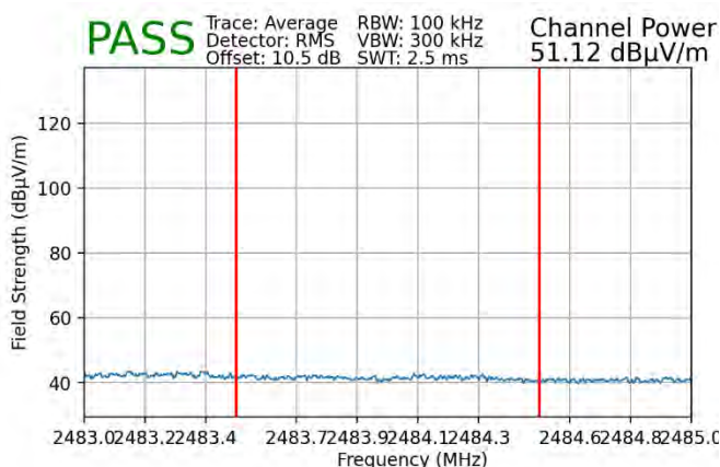
Plot 7-127. Radiated Restricted Upper Band Edge Measurement MIMO (Average – 242 Tones)
