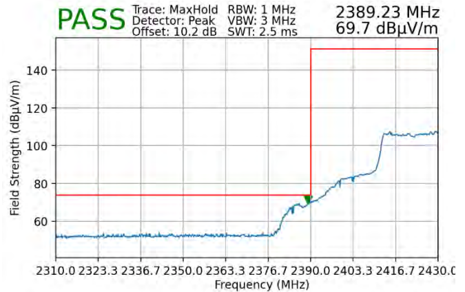
Plot 7-122. Radiated Restricted Lower Band Edge Measurement MIMO (Peak – 242 Tones)
