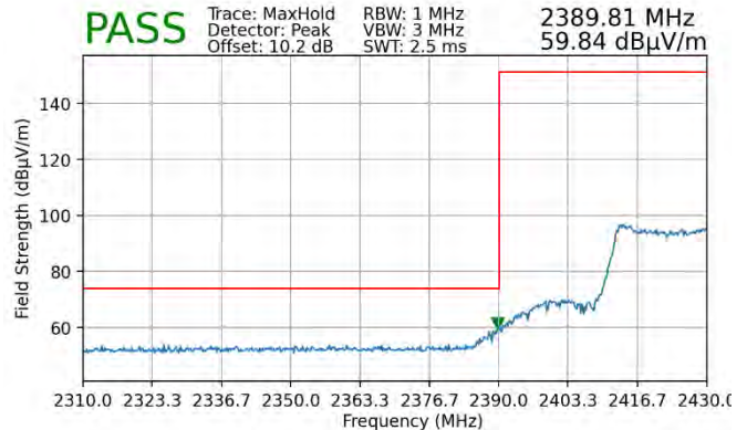
Plot 7-106. Radiated Restricted Lower Band Edge Measurement SISO ANT2 (Peak – 242 Tones)
