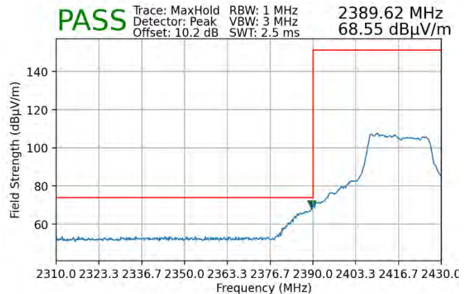
Plot 7-120. Radiated Restricted Lower Band Edge Measurement MIMO (Peak – 242 Tones)
