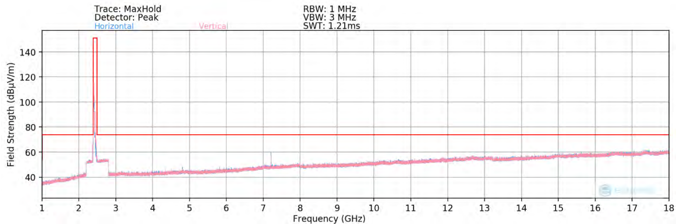
Plot 7-84. Radiated Spurious Plot above 1GHz MIMO (802.11ax OFDMA – 26 Tones – Ch. 1) – Open
