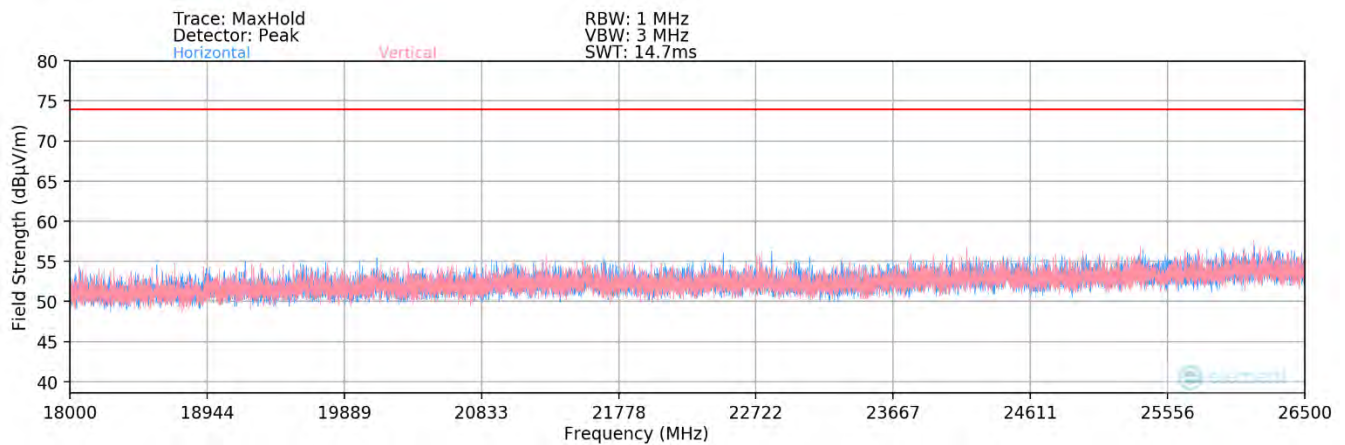
Plot 7-80. Radiated Spurious Plot above 18GHz SISO ANT2 (802.11ax OFDMA – 242 Tones) – Open
