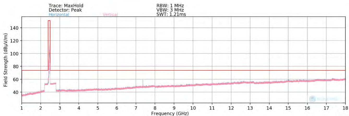
Plot 7-86. Radiated Spurious Plot above 1GHz MIMO (802.11ax OFDMA – 26 Tones – Ch. 11) – Open
