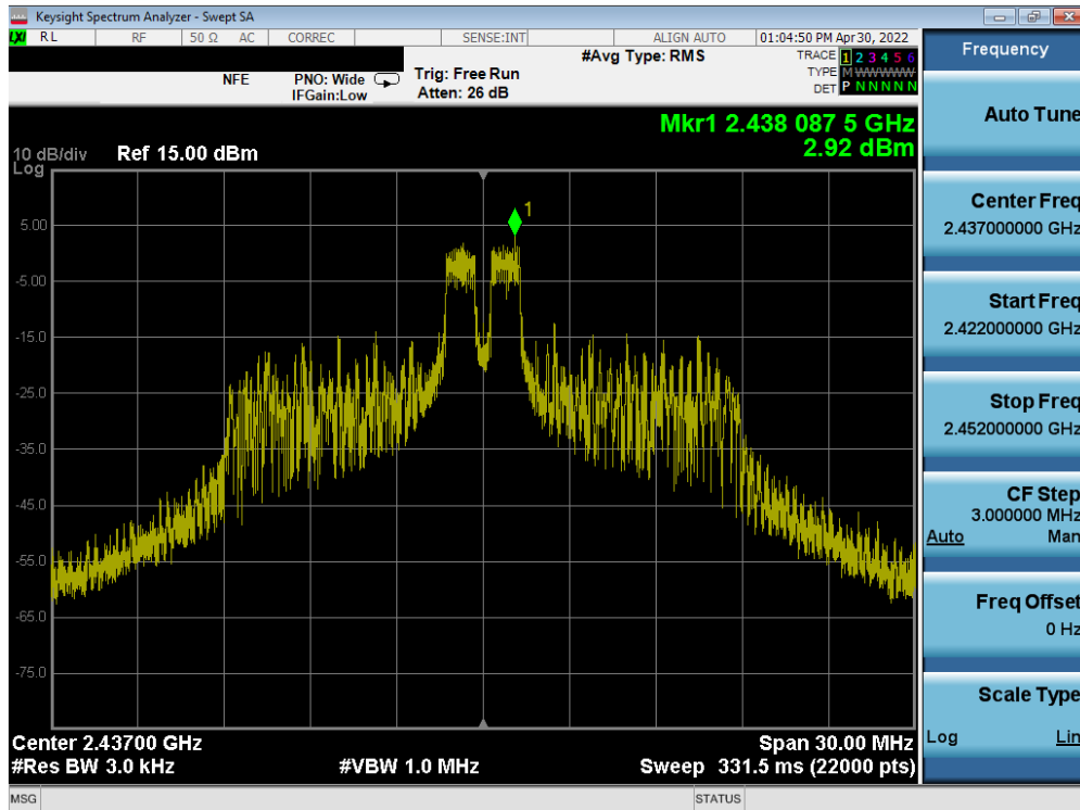
Plot 7-14. Power Spectral Density Plot ANT1 (802.11ax OFDMA – 26 Tones – Ch. 6)
