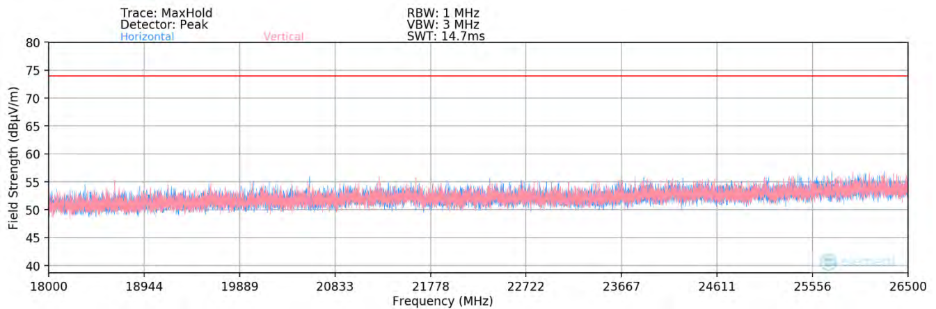
Plot 7-96. Radiated Spurious Plot above 18GHz MIMO (802.11ax OFDMA – 242 Tones) – Open
