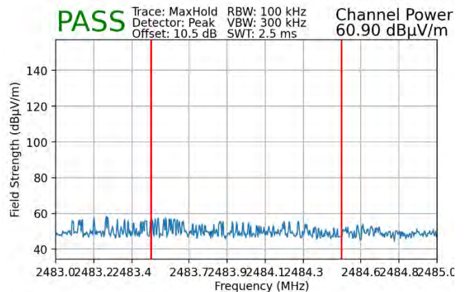
Plot 7-124. Radiated Restricted Upper Band Edge Measurement MIMO (Peak – 242 Tones)
