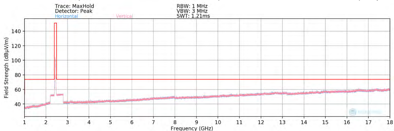
Plot 7-75. Radiated Spurious Plot above 1GHz SISO ANT2 (802.11ax OFDMA – 242 Tones – Ch. 6) – Open
