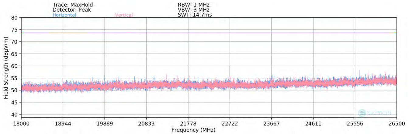
Plot 7-93. Radiated Spurious Plot above 18GHz MIMO (802.11ax OFDMA – 26 Tones) – Half Open
