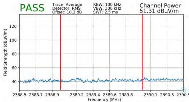
Plot 7-113. Radiated Restricted Lower Band Edge Measurement MIMO (Average – 106 Tones)
