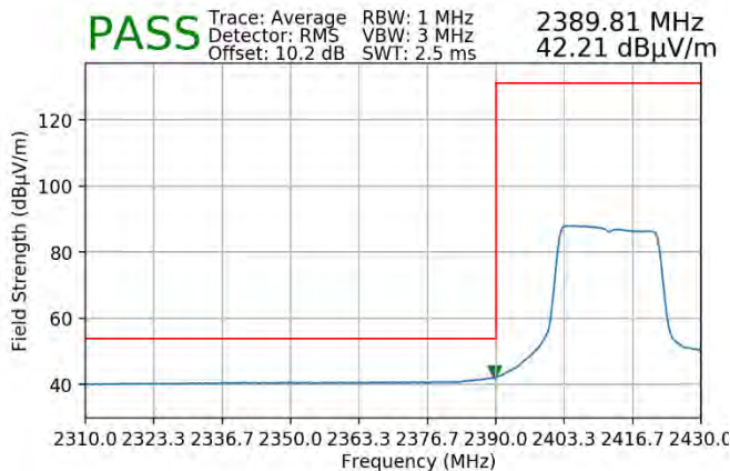
Plot 7-101. Radiated Restricted Lower Band Edge Measurement SISO ANT2 (Average – 242 Tones)
