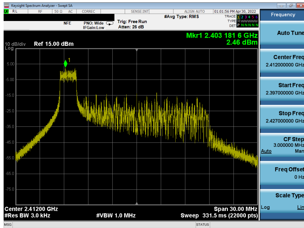
Plot 7-13. Power Spectral Density Plot ANT1 (802.11ax OFDMA – 26 Tones – Ch. 1)
