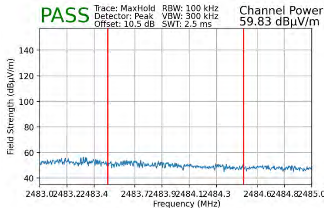
Plot 7-126. Radiated Restricted Upper Band Edge Measurement SISO MIMO (Peak – 242 Tones)
