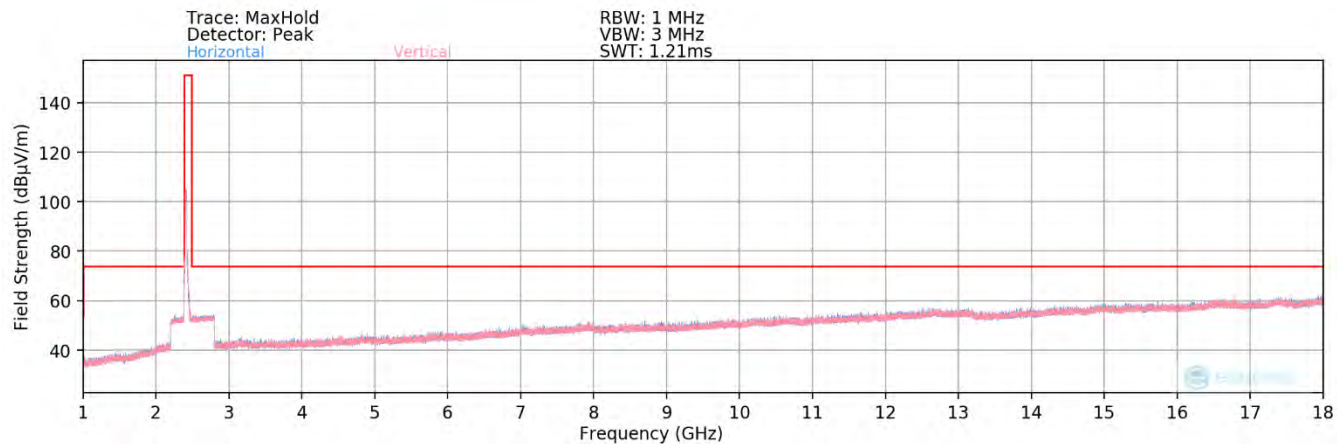
Plot 7-74. Radiated Spurious Plot above 1GHz SISO ANT2 (802.11ax OFDMA – 242 Tones – Ch. 1) – Open
