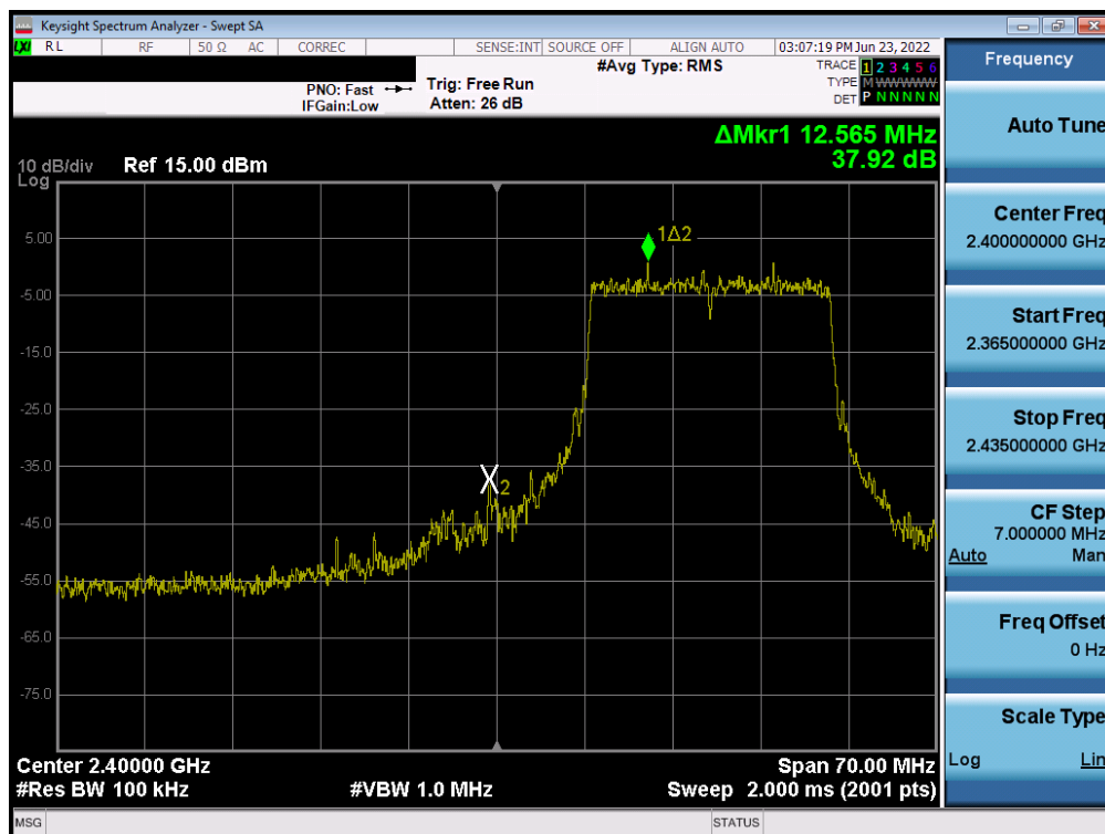
Plot 7-28. Band Edge Plot ANT1 (802.11ax OFDMA – 242 Tones – Ch. 2)
