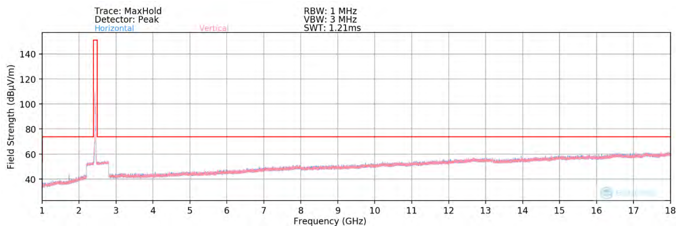
Plot 7-69. Radiated Spurious Plot above 1GHz SISO ANT2 (802.11ax OFDMA – 26 Tones – Ch. 6) – Open
