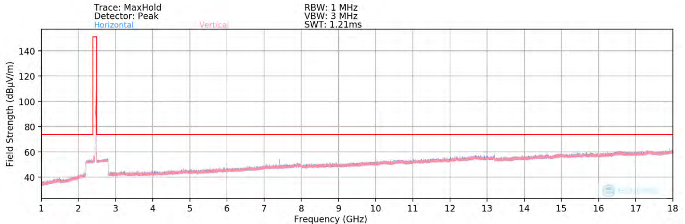
Plot 7-67. Radiated Spurious Plot above 1GHz SISO ANT2 (802.11ax OFDMA – 26 Tones – Ch. 11) – Half Open
