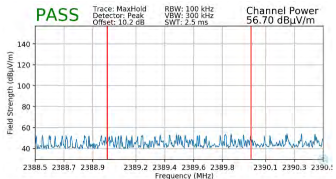
Plot 7-98. Radiated Restricted Lower Band Edge Measurement SISO ANT2 (Peak – 106 Tones)
