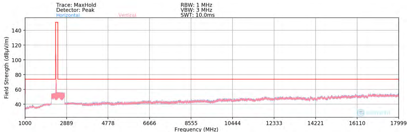
Plot 7-68. Radiated Spurious Plot above 1GHz SISO ANT2 (802.11ax OFDMA – 26 Tones – Ch. 1) – Open
