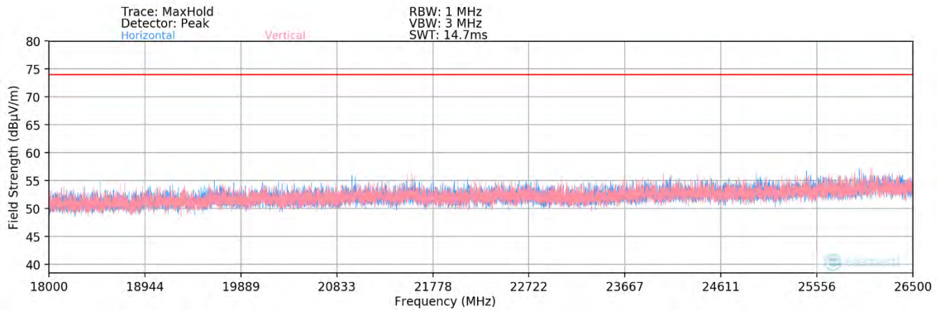
Plot 7-94. Radiated Spurious Plot above 18GHz MIMO (802.11ax OFDMA – 26 Tones) – Open
