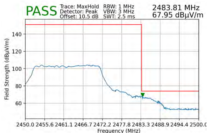
Plot 7-128. Radiated Restricted Upper Band Edge Measurement MIMO (Peak – 242 Tones)
