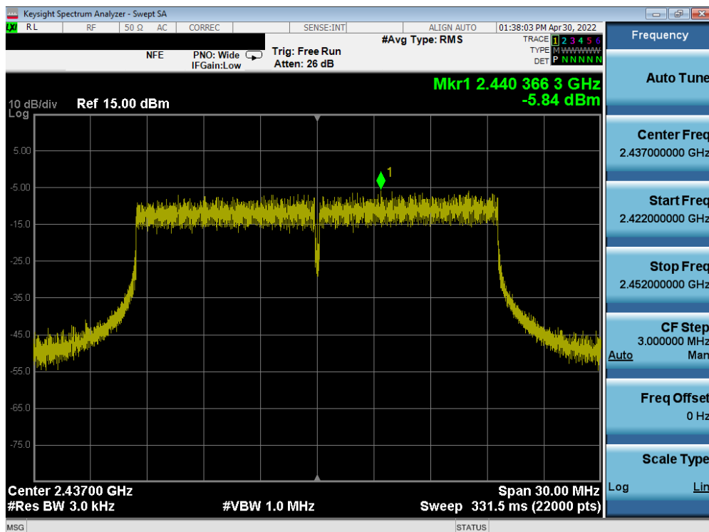
Plot 7-17. Power Spectral Density Plot ANT1 (802.11ax OFDMA – 242 Tones – Ch. 6)
