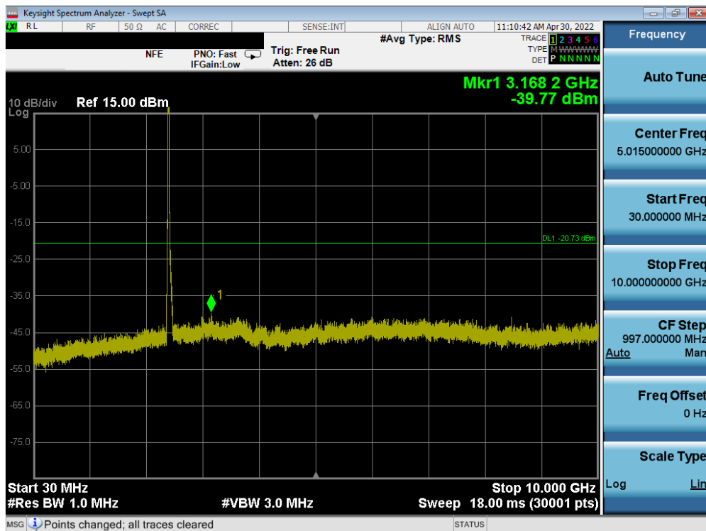
Plot 7-59. Conducted Spurious Plot SISO ANT2 (802.11ax OFDMA – 242 Tones – Ch. 1)
