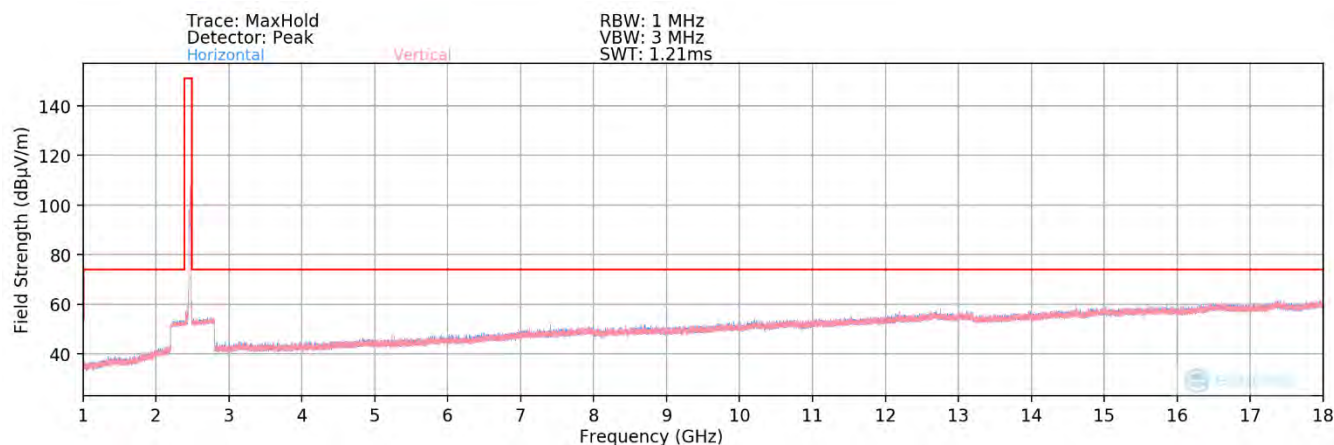
Plot 7-70. Radiated Spurious Plot above 1GHz SISO ANT2 (802.11ax OFDMA – 26 Tones – Ch. 11) – Open
