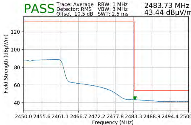
Plot 7-107. Radiated Restricted Upper Band Edge Measurement SISO ANT2 (Average – 242 Tones)
