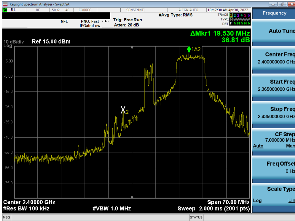
Plot 7-33. Band Edge Plot SISO ANT2 (802.11ax OFDMA – 106 Tones – Ch. 1)
