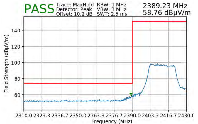
Plot 7-102. Radiated Restricted Lower Band Edge Measurement SISO ANT2 (Peak – 242 Tones)
