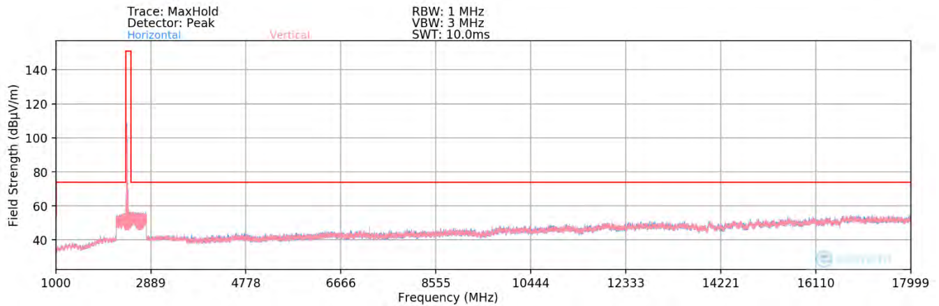
Plot 7-65. Radiated Spurious Plot above 1GHz SISO ANT2 (802.11ax OFDMA – 26 Tones – Ch. 1) – Half Open
