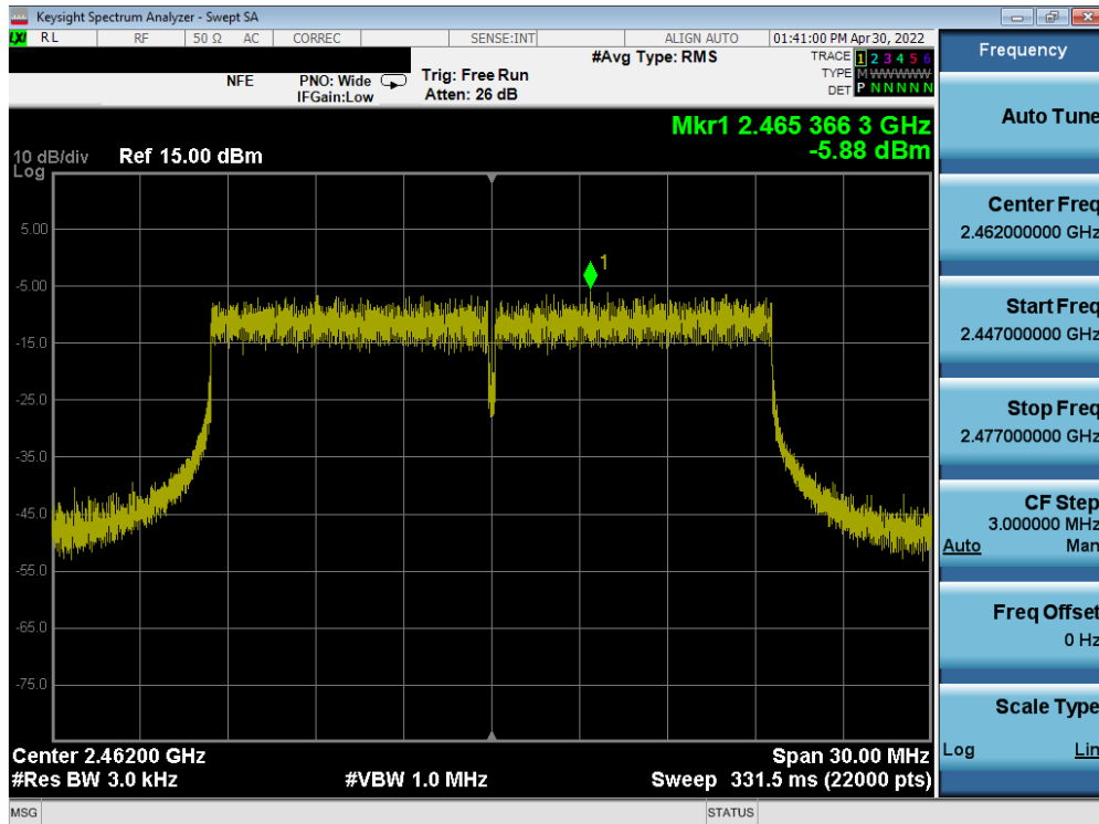
Plot 7-18. Power Spectral Density Plot ANT1 (802.11ax OFDMA – 242 Tones – Ch. 11)
