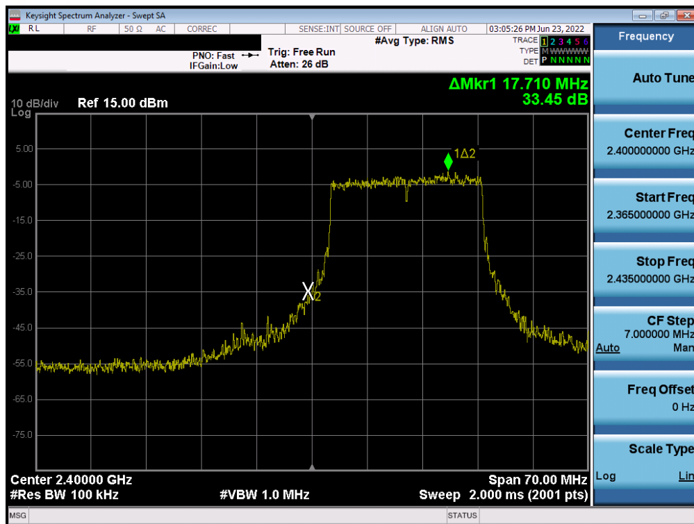
Plot 7-27. Band Edge Plot ANT1 (802.11ax OFDMA – 242 Tones – Ch. 1)
