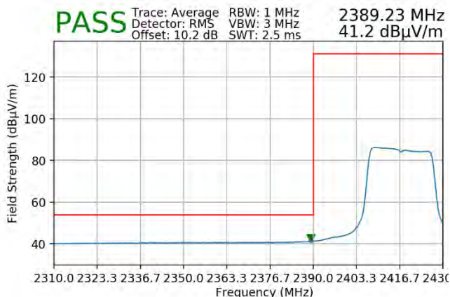
Plot 7-103. Radiated Restricted Lower Band Edge Measurement SISO ANT2 (Average – 242 Tones)
