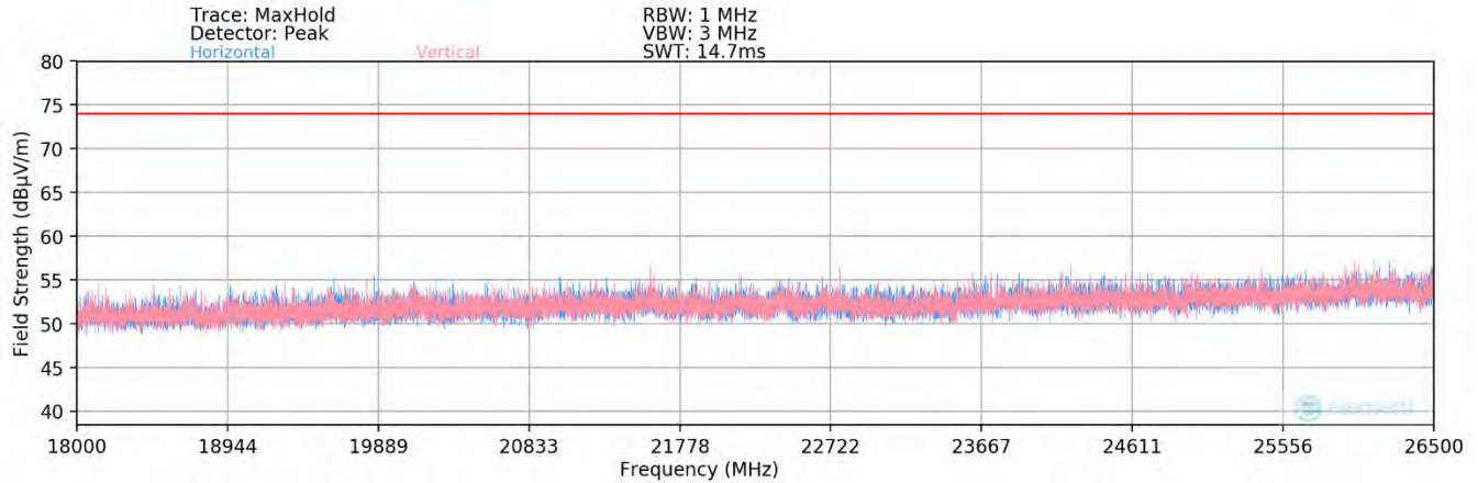
Plot 7-95. Radiated Spurious Plot above 18GHz MIMO (802.11ax OFDMA – 242 Tones) – Half Open
