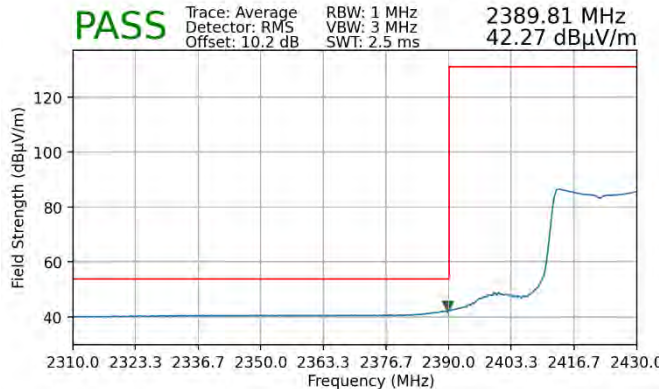
Plot 7-105. Radiated Restricted Lower Band Edge Measurement SISO ANT2 (Average – 242 Tones)
