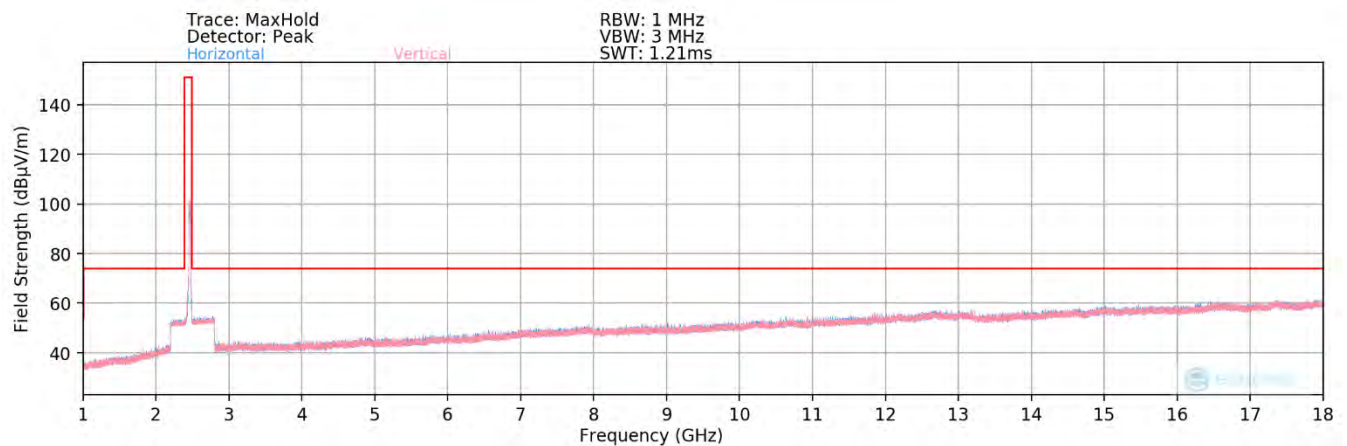
Plot 7-73. Radiated Spurious Plot above 1GHz SISO ANT2 (802.11ax OFDMA – 242 Tones – Ch. 11) – Half Open
