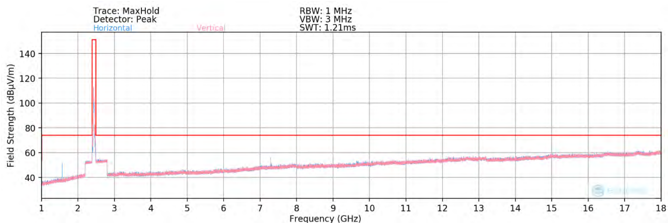
Plot 7-85. Radiated Spurious Plot above 1GHz MIMO (802.11ax OFDMA – 26 Tones – Ch. 6) – Open
