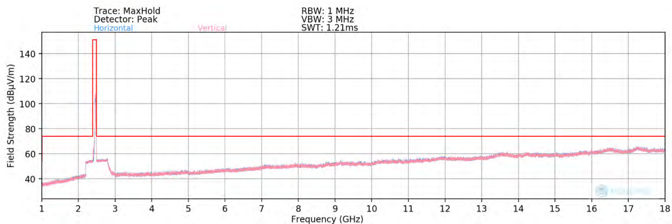
Plot 7-92. Radiated Spurious Plot above 1GHz MIMO (802.11ax OFDMA – 242 Tones – Ch. 11) – Open
