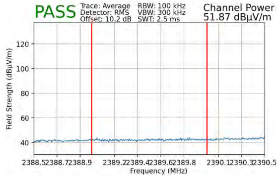
Plot 7-117. Radiated Restricted Lower Band Edge Measurement MIMO (Average – 242 Tones)
