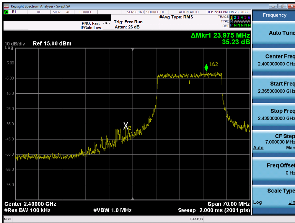
Plot 7-36. Band Edge Plot SISO ANT1 (802.11ax OFDMA – 242 Tones – Ch. 2)
