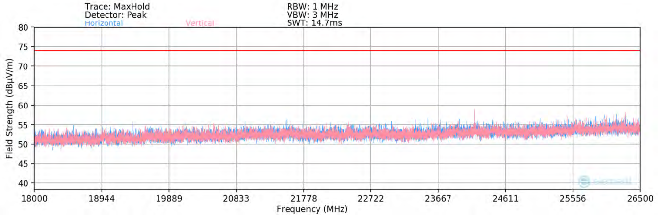
Plot 7-79. Radiated Spurious Plot above 18GHz SISO ANT2 (802.11ax OFDMA – 242 Tones) – Half Open
