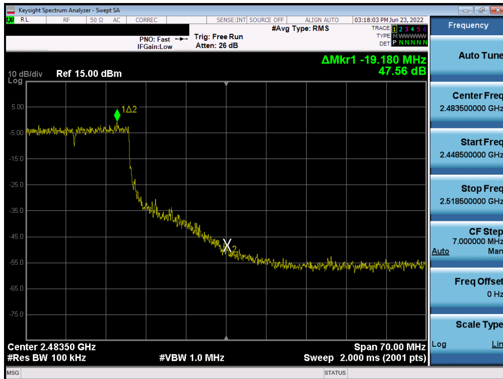
Plot 7-39. Band Edge Plot SISO ANT1 (802.11ax OFDMA – 242 Tones – Ch. 10)
