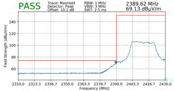
Plot 7-118. Radiated Restricted Lower Band Edge Measurement MIMO (Peak – 242 Tones)
