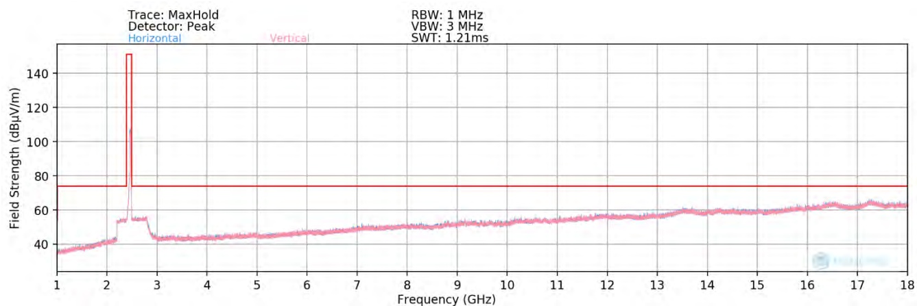
Plot 7-89. Radiated Spurious Plot above 1GHz MIMO (802.11ax OFDMA – 242 Tones – Ch. 11) – Half Open
