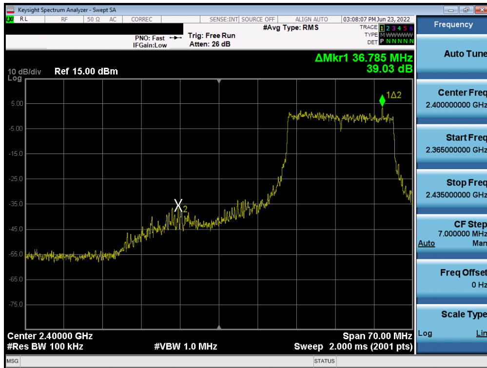
Plot 7-29. Band Edge Plot ANT1 (802.11ax OFDMA – 242 Tones – Ch. 3)
