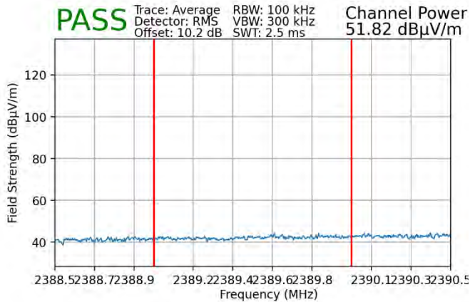
Plot 7-121. Radiated Restricted Lower Band Edge Measurement MIMO (Average – 242 Tones)
