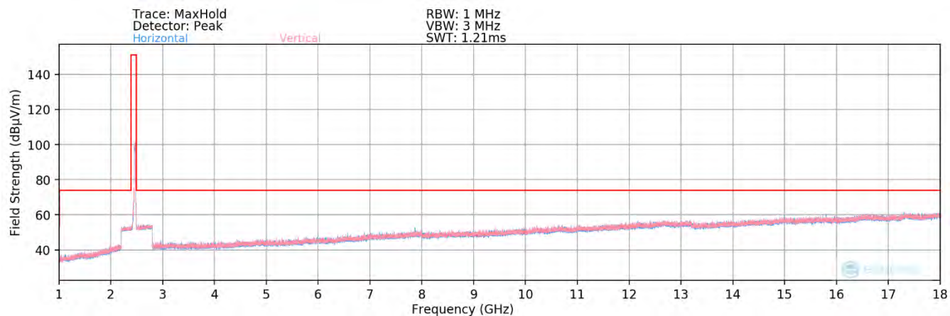
Plot 7-76. Radiated Spurious Plot above 1GHz SISO ANT2 (802.11ax OFDMA – 242 Tones – Ch. 11) – Open
