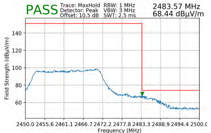
Plot 7-112. Radiated Restricted Upper Band Edge Measurement SISO ANT2 (Peak – 242 Tones)
