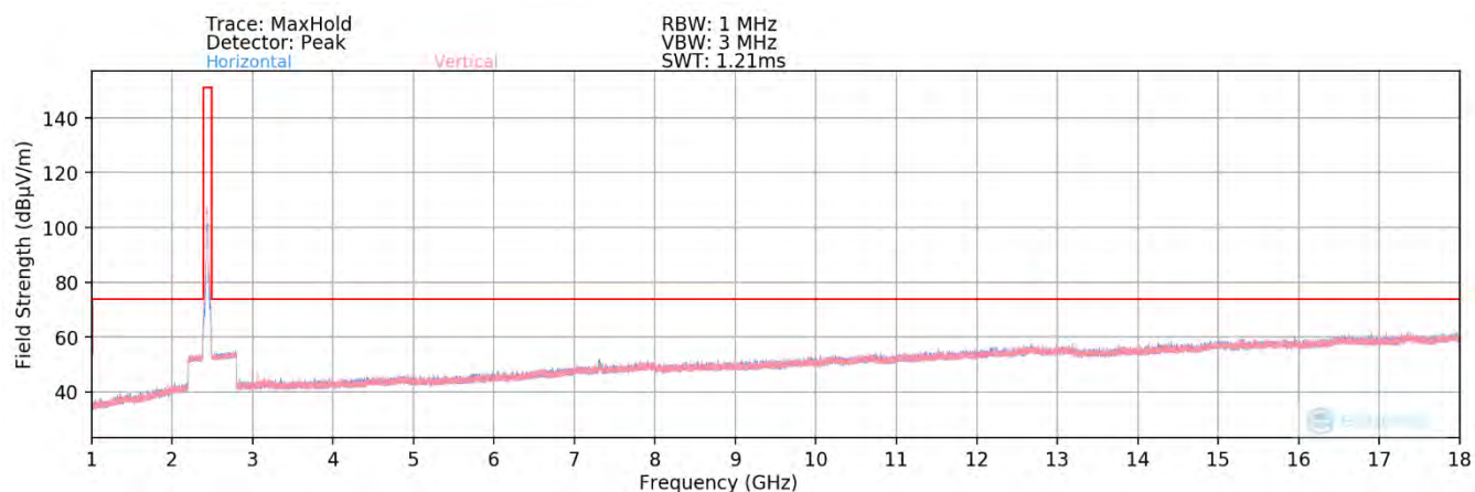
Plot 7-88. Radiated Spurious Plot above 1GHz MIMO (802.11ax OFDMA – 242 Tones – Ch. 6) – Half Open
