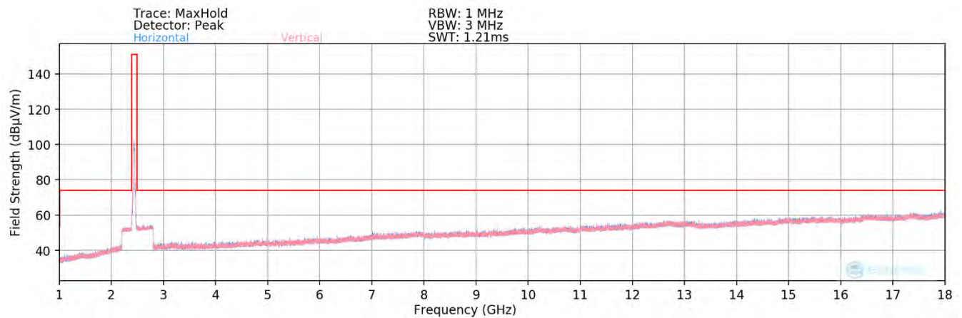
Plot 7-72. Radiated Spurious Plot above 1GHz SISO ANT2 (802.11ax OFDMA – 242 Tones – Ch. 6) – Half Open
