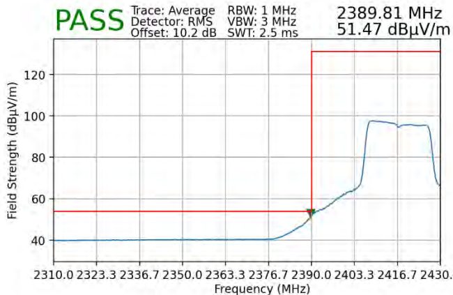
Plot 7-119. Radiated Restricted Lower Band Edge Measurement MIMO (Average – 242 Tones)
