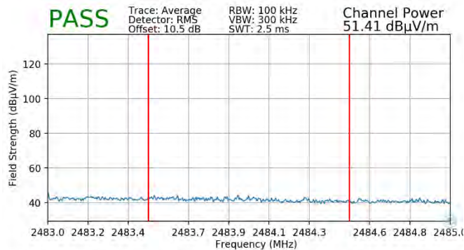
Plot 7-115. Radiated Restricted Upper Band Edge Measurement MIMO (Average – 106 Tones)
