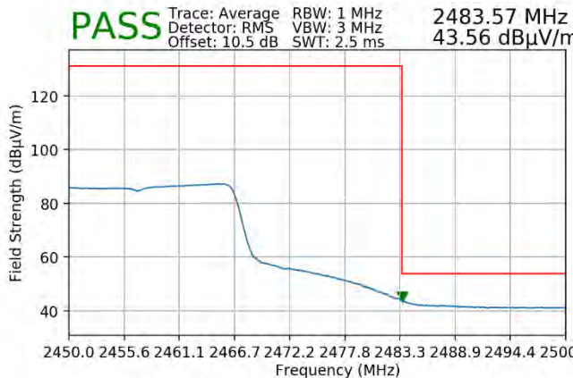
Plot 7-109. Radiated Restricted Upper Band Edge Measurement SISO ANT2 (Average – 242 Tones)
