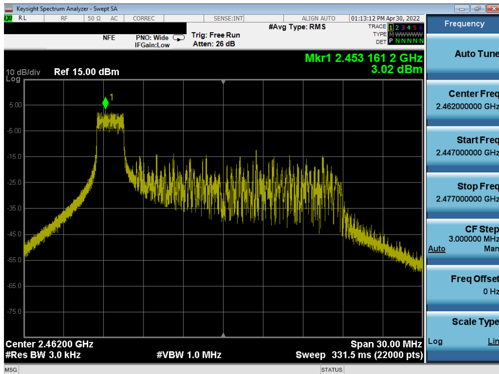
Plot 7-15. Power Spectral Density Plot ANT1 (802.11ax OFDMA – 26 Tones – Ch. 11)
