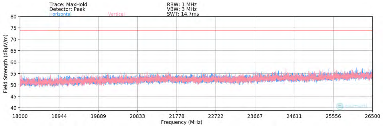
Plot 7-77. Radiated Spurious Plot above 18GHz SISO ANT2 (802.11ax OFDMA – 26 Tones) – Half Open
