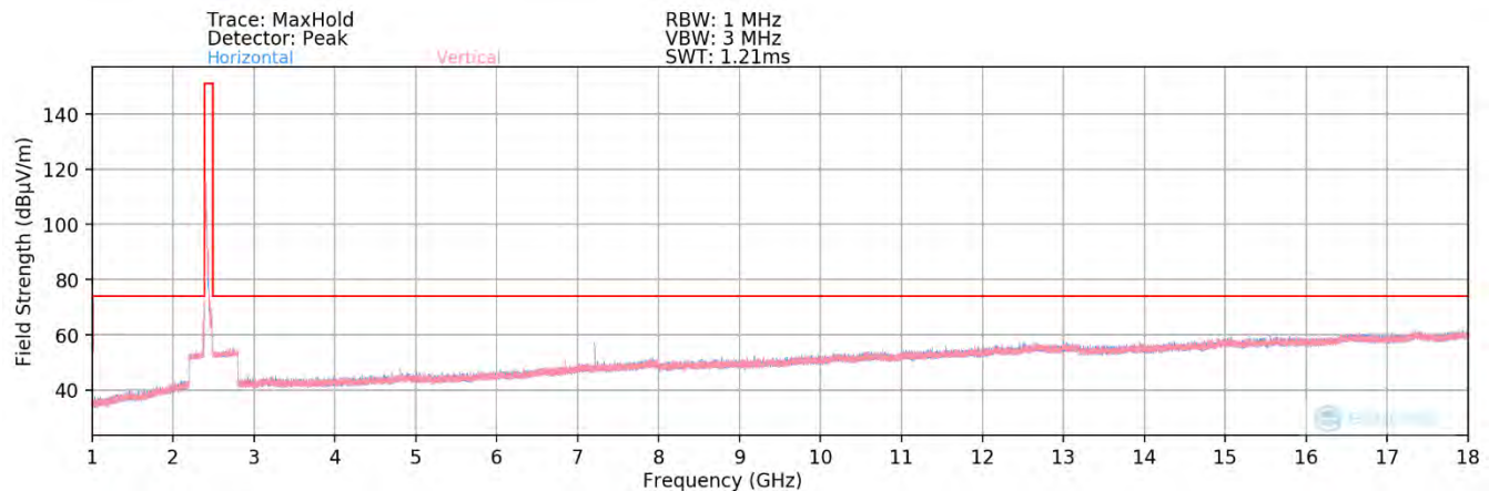
Plot 7-81. Radiated Spurious Plot above 1GHz MIMO (802.11ax OFDMA – 26 Tones – Ch. 1) – Half Open
