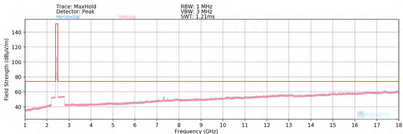
Plot 7-91. Radiated Spurious Plot above 1GHz MIMO (802.11ax OFDMA – 242 Tones – Ch. 6) – Open
