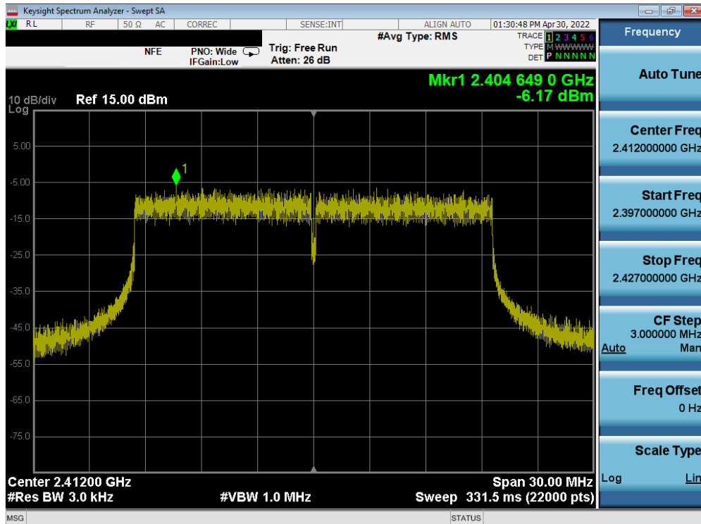
Plot 7-16. Power Spectral Density Plot ANT1 (802.11ax OFDMA – 242 Tones – Ch. 1)
