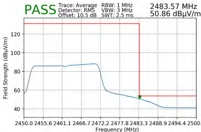
Plot 7-111. Radiated Restricted Upper Band Edge Measurement SISO ANT2 (Average – 242 Tones)
