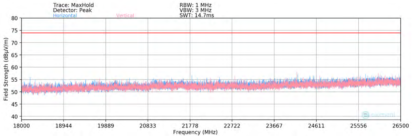
Plot 7-78. Radiated Spurious Plot above 18GHz SISO ANT2 (802.11ax OFDMA – 26 Tones) – Open
