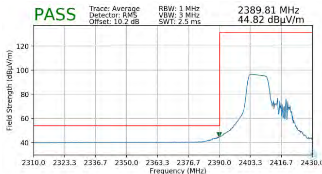
Plot 7-97. Radiated Restricted Lower Band Edge Measurement SISO ANT2 (Average – 106 Tones)
