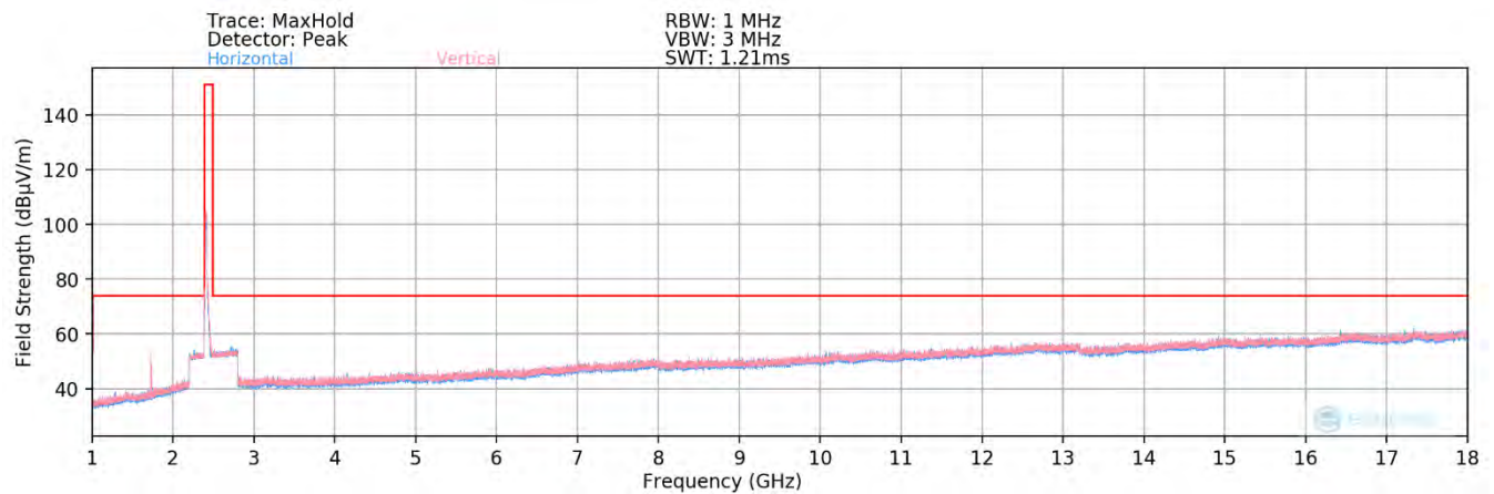
Plot 7-71. Radiated Spurious Plot above 1GHz SISO ANT2 (802.11ax OFDMA – 242 Tones – Ch. 1) – Half Open
