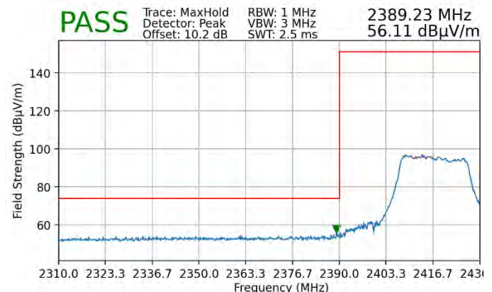
Plot 7-104. Radiated Restricted Lower Band Edge Measurement SISO ANT2 (Peak – 242 Tones)
