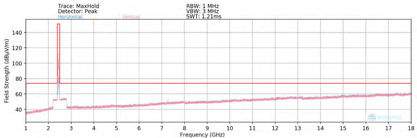
Plot 7-82. Radiated Spurious Plot above 1GHz MIMO (802.11ax OFDMA – 26 Tones – Ch. 6) – Half Open
