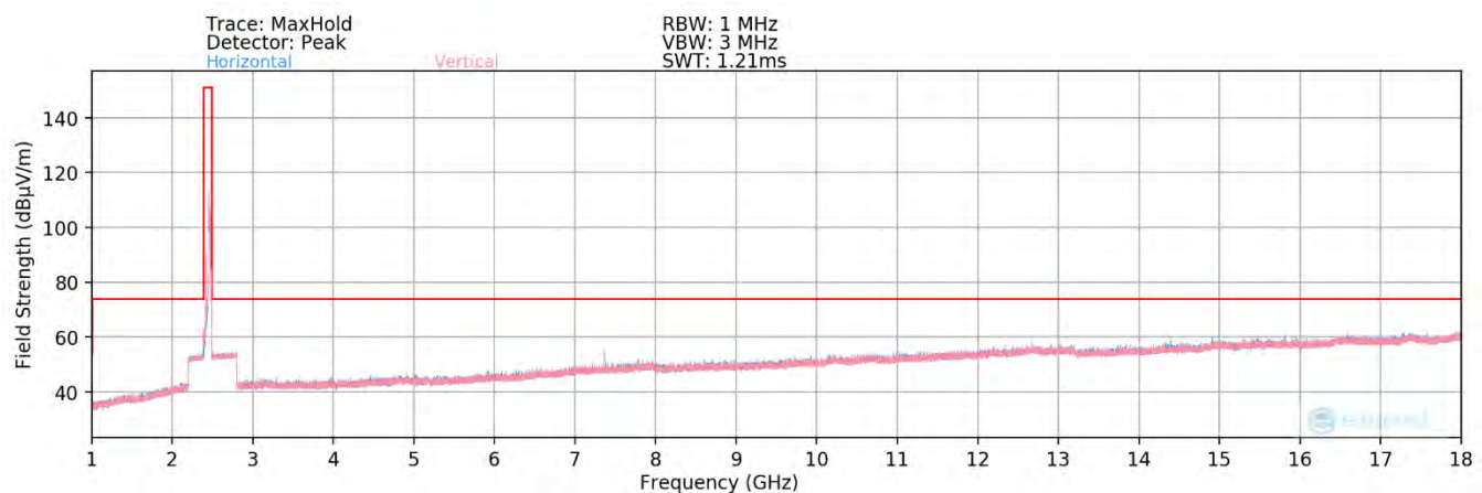
Plot 7-83. Radiated Spurious Plot above 1GHz MIMO (802.11ax OFDMA – 26 Tones – Ch. 11) – Half Open
