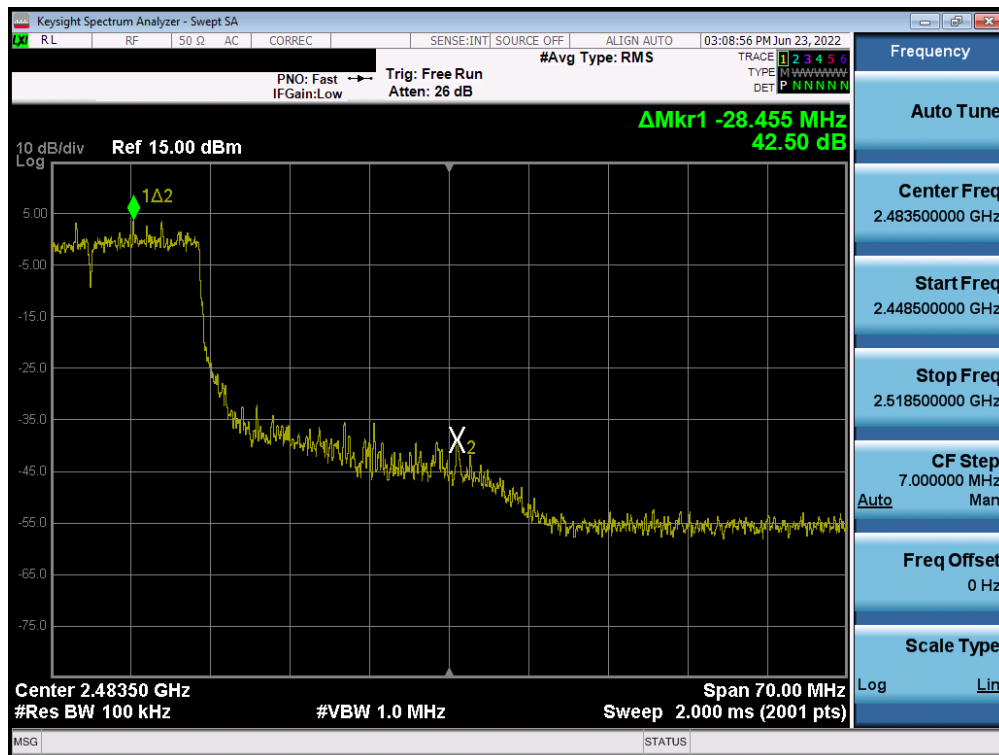
Plot 7-30. Band Edge Plot ANT1 (802.11ax OFDMA – 242 Tones – Ch. 9)
