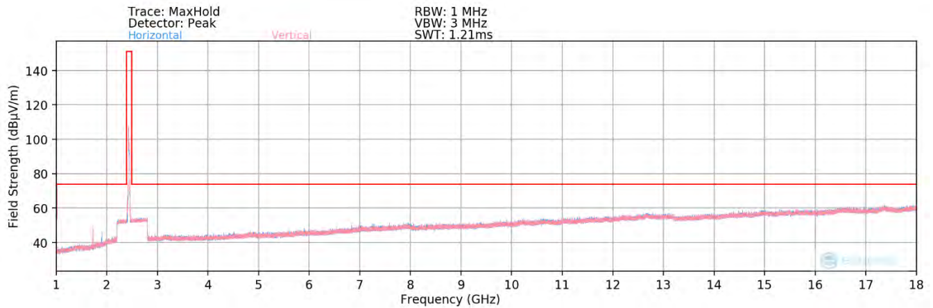
Plot 7-66. Radiated Spurious Plot above 1GHz SISO ANT2 (802.11ax OFDMA – 26 Tones – Ch. 6) – Half Open
