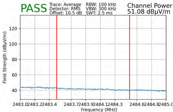
Plot 7-125. Radiated Restricted Upper Band Edge Measurement MIMO (Average – 242 Tones)
