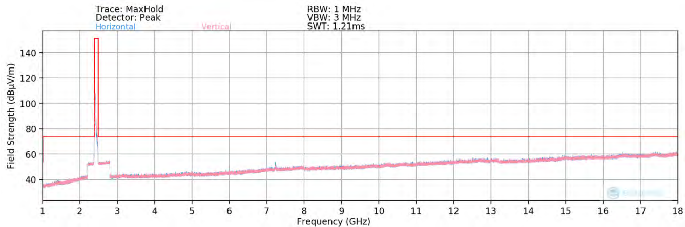
Plot 7-90. Radiated Spurious Plot above 1GHz MIMO (802.11ax OFDMA – 242 Tones – Ch. 1) – Open
