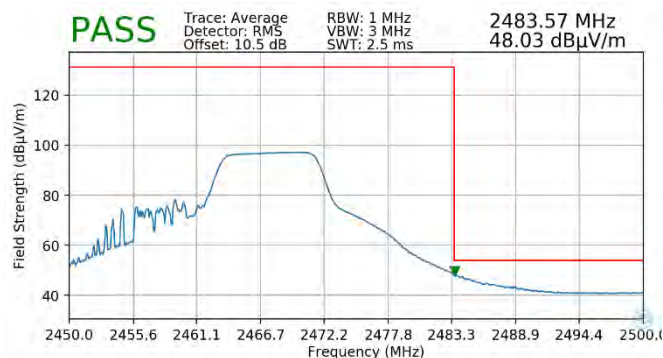
Plot 7-99. Radiated Restricted Upper Band Edge Measurement SISO ANT2 (Average – 106 Tones)
