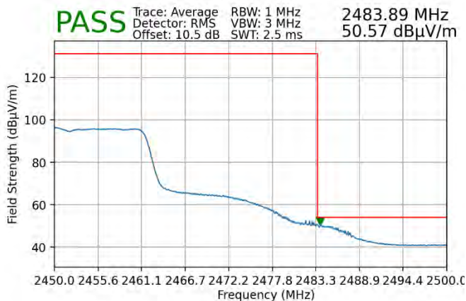
Plot 7-123. Radiated Restricted Upper Band Edge Measurement MIMO (Average – 242 Tones)
