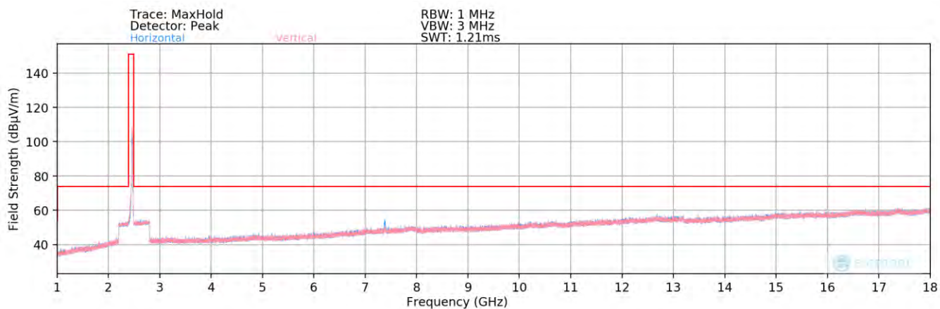
Plot 7-90. Radiated Spurious Plot above 1GHz MIMO/CDD (802.11g - Ch. 11) - Open
