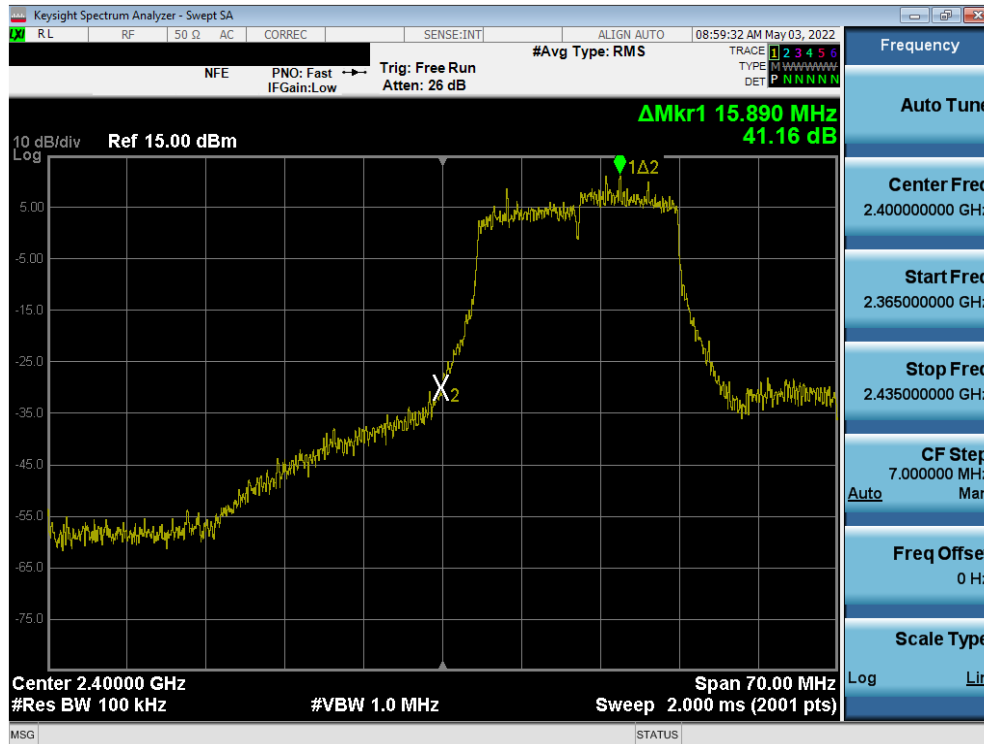
Plot 7-53. Band Edge Plot ANT1 (802.11n (2.4GHz) – Ch. 1)
