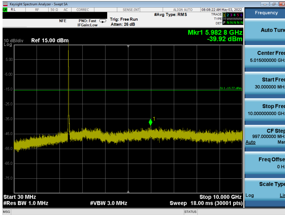
Plot 7-65. Conducted Spurious Plot ANT1 (802.11b – Ch. 1)
