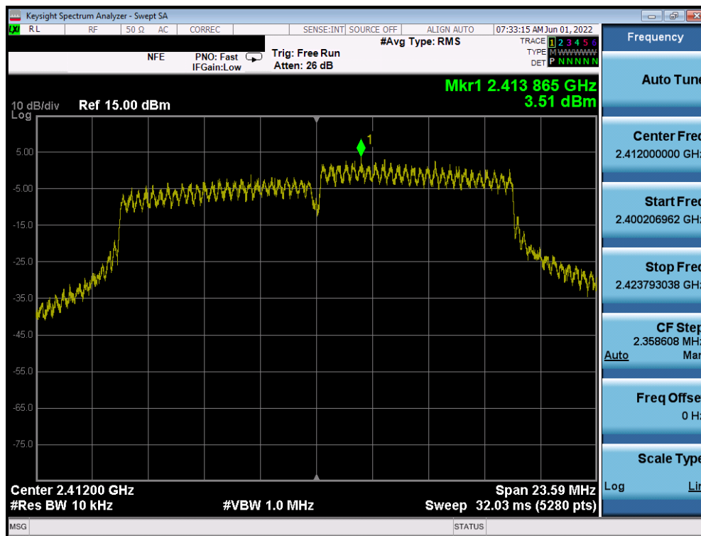
Plot 7-28. Power Spectral Density Plot ANT1 (802.11g – Ch. 1)
