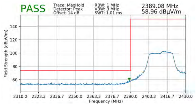
Plot 7-94. Radiated Restricted Band Edge Measurement SISO ANT2 with WCP (Peak)
