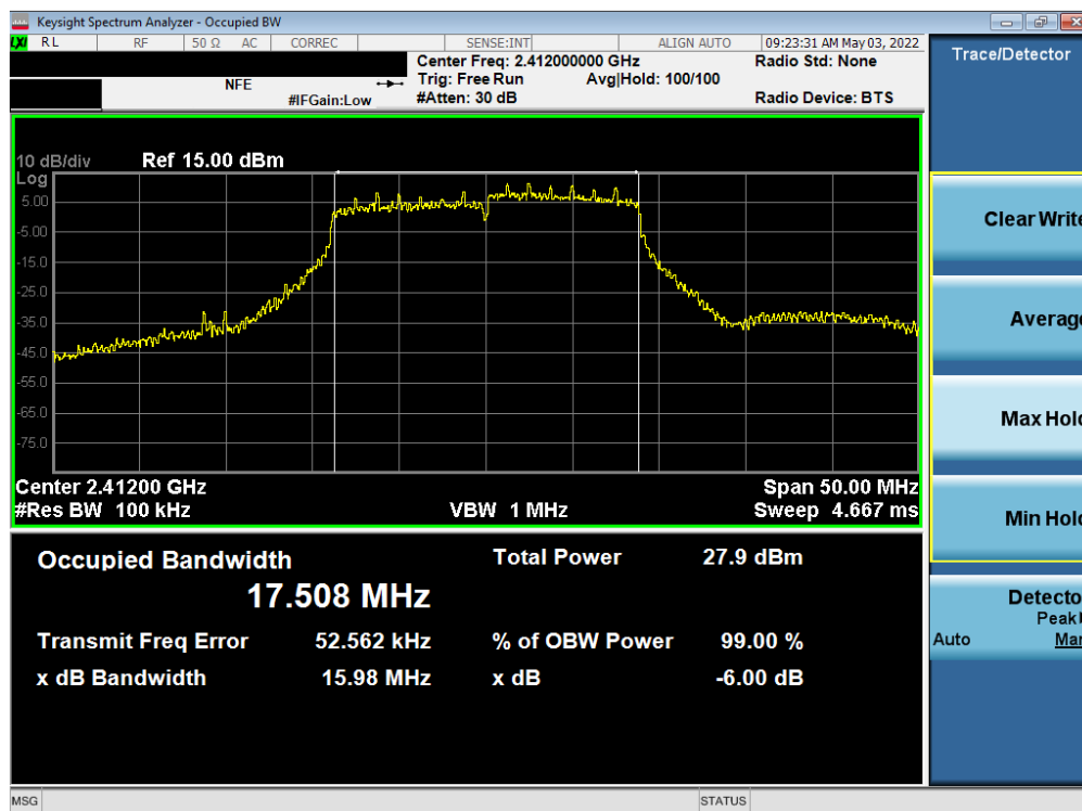
Plot 7-10. 6dB Bandwidth Plot ANT1 (802.11ax (2.4GHz) – Ch. 1)
