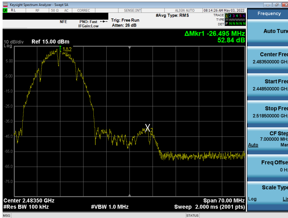
Plot 7-50. Band Edge Plot ANT1 (802.11b – Ch. 11)
