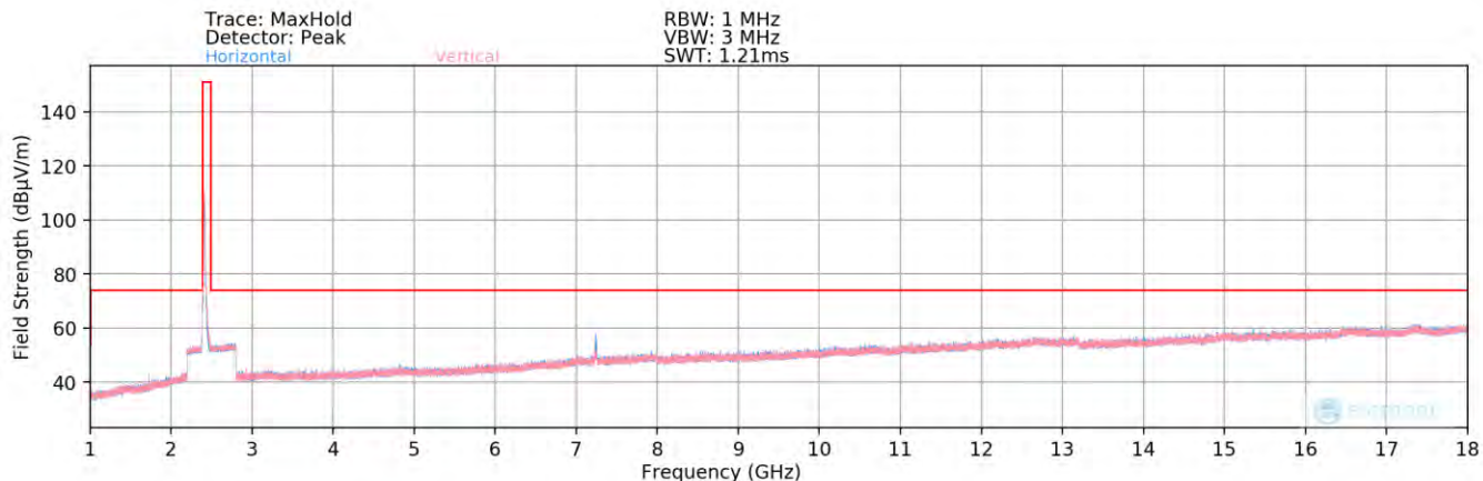
Plot 7-88. Radiated Spurious Plot above 1GHz MIMO/CDD (802.11g - Ch. 1) - Open
