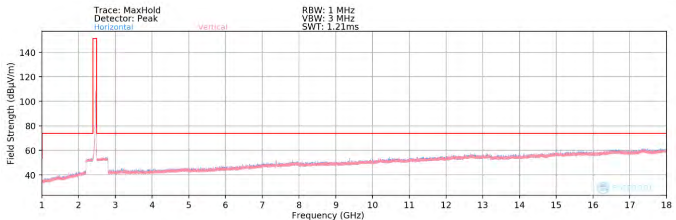
Plot 7-87. Radiated Spurious Plot above 1GHz MIMO/CDD (802.11g – Ch. 11) – Half Open
