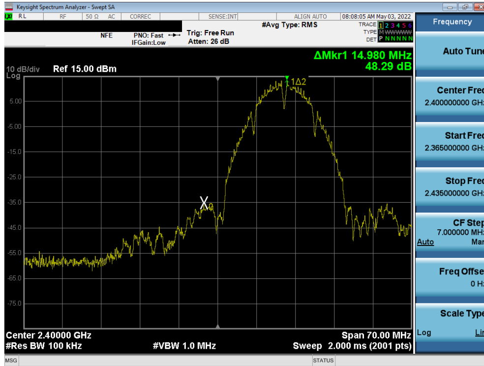
Plot 7-49. Band Edge Plot ANT1 (802.11b – Ch. 1)
