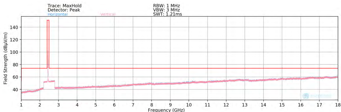
Plot 7-81. Radiated Spurious Plot above 1GHz SISO ANT2 (802.11b - Ch. 6) - Open
