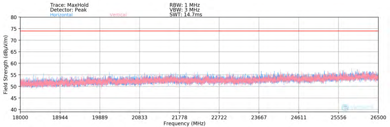
Plot 7-84. Radiated Spurious Plot above 18GHz SISO ANT2 – Open
