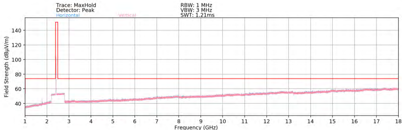
Plot 7-80. Radiated Spurious Plot above 1GHz SISO ANT2 (802.11b - Ch. 1) - Open
