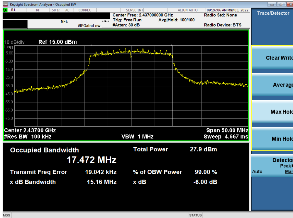
Plot 7-11. 6dB Bandwidth Plot ANT1 (802.11ax (2.4GHz) – Ch. 6)
