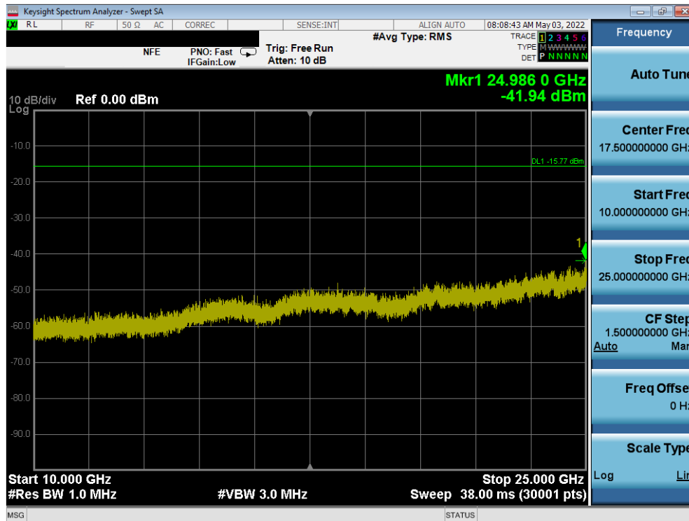
Plot 7-66. Conducted Spurious Plot ANT1 (802.11b – Ch. 1)
