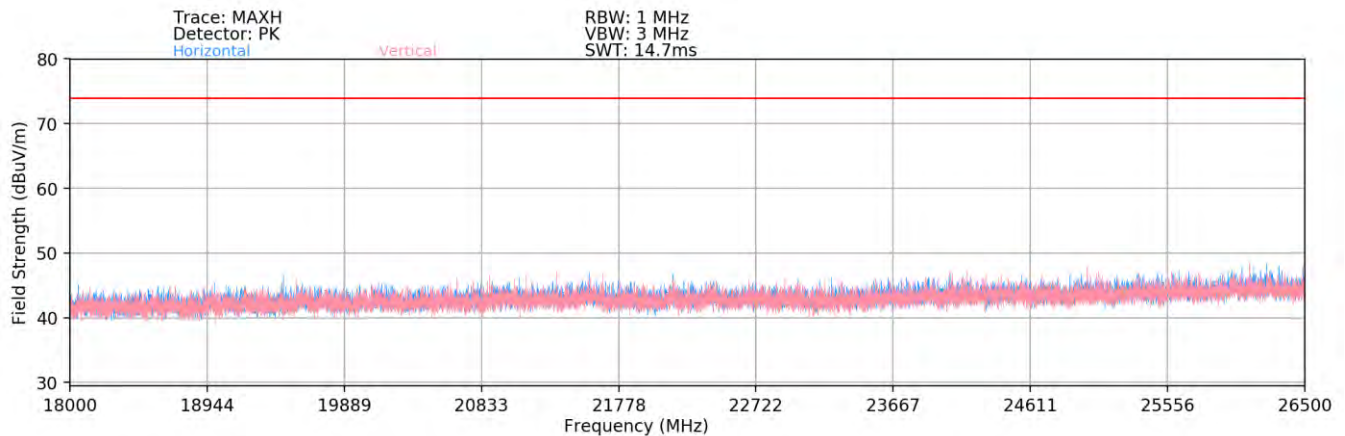
Plot 7-92. Radiated Spurious Plot above 18GHz MIMO/CDD – Open
