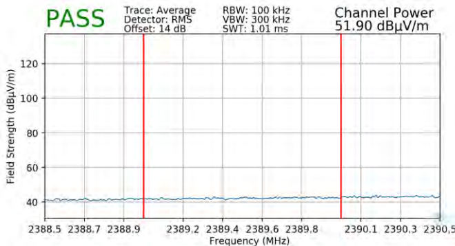
Plot 7-97. Radiated Restricted Lower Band Edge Measurement MIMO (Average)
