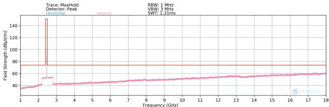
Plot 7-82. Radiated Spurious Plot above 1GHz SISO ANT2 (802.11b - Ch. 11) - Open
