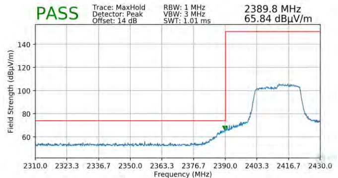
Plot 7-98. Radiated Restricted Lower Band Edge Measurement MIMO (Peak)
