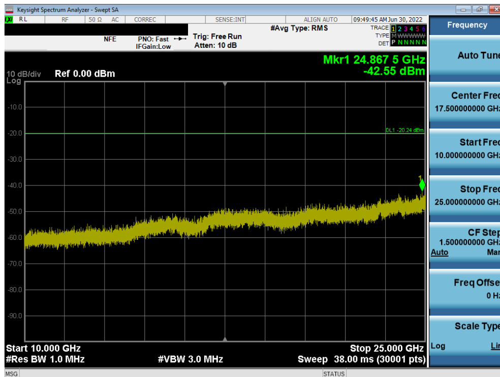
Plot 7-70. Conducted Spurious Plot ANT1 (802.11b – Ch. 11)
