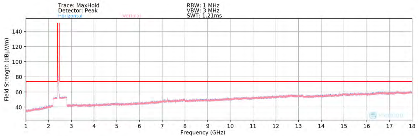
Plot 7-85. Radiated Spurious Plot above 1GHz MIMO/CDD (802.11g – Ch. 1) – Half Open
