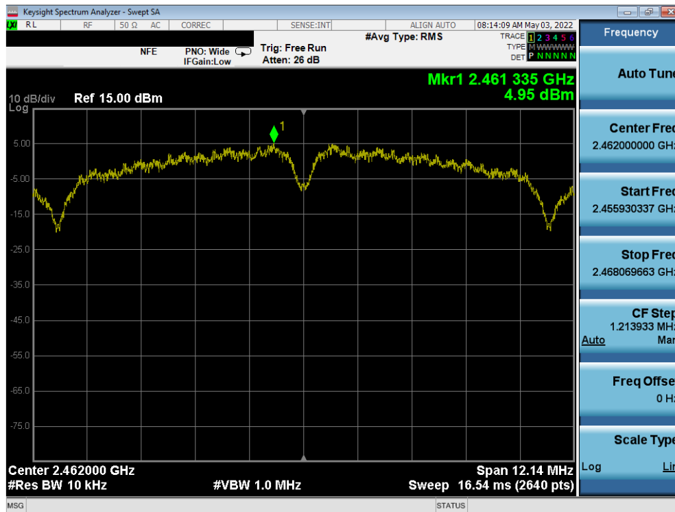
Plot 7-27. Power Spectral Density Plot ANT1 (802.11b – Ch. 11)
