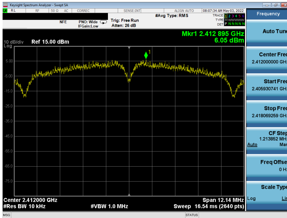
Plot 7-25. Power Spectral Density Plot ANT1 (802.11b – Ch. 1)
