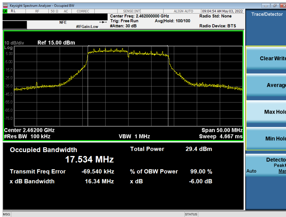
Plot 7-9. 6dB Bandwidth Plot ANT1 (802.11n (2.4GHz) – Ch. 11)
