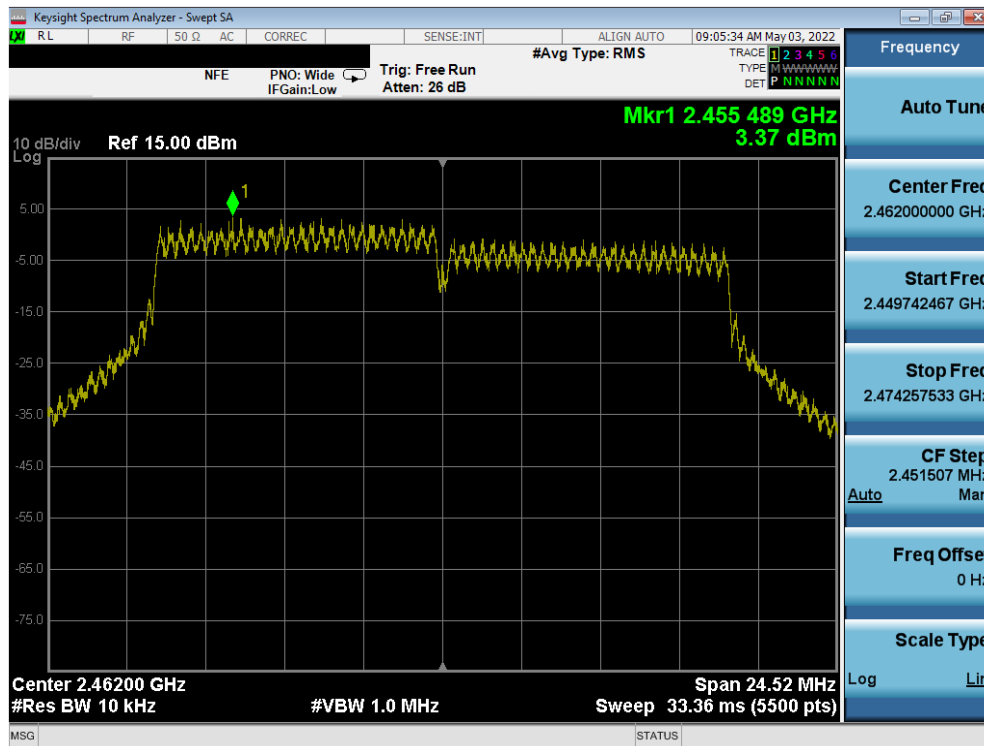
Plot 7-33. Power Spectral Density Plot ANT1 (802.11n (2.4GHz) – Ch. 11)
