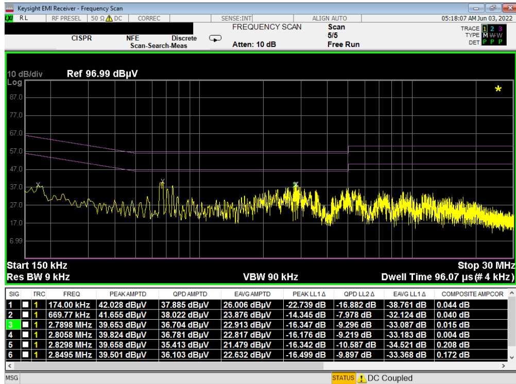
Plot 7-106. Line Conducted Plot with 802.11b (L1) – Closed
