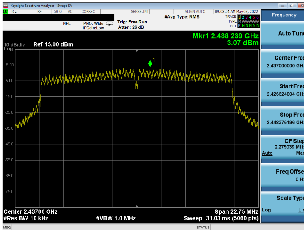
Plot 7-32. Power Spectral Density Plot ANT1 (802.11n (2.4GHz) – Ch. 6)
