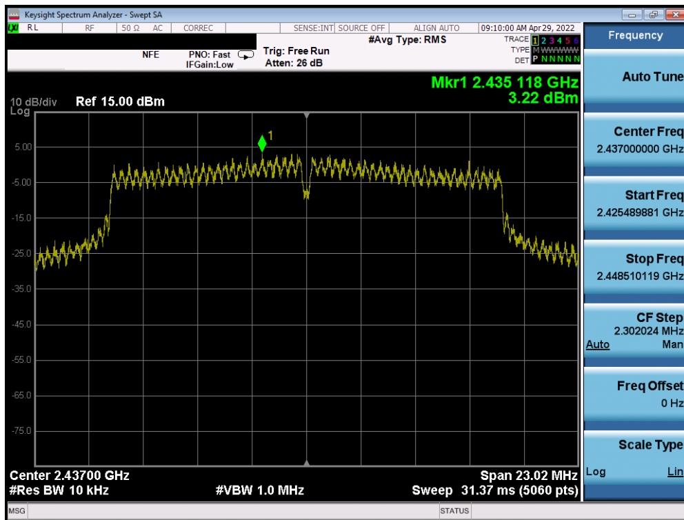
Plot 7-41. Power Spectral Density Plot SISO ANT2 (802.11g – Ch. 6)
