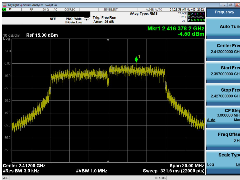
Plot 7-34. Power Spectral Density Plot ANT1 (802.11ax (2.4GHz) – Ch. 1)
