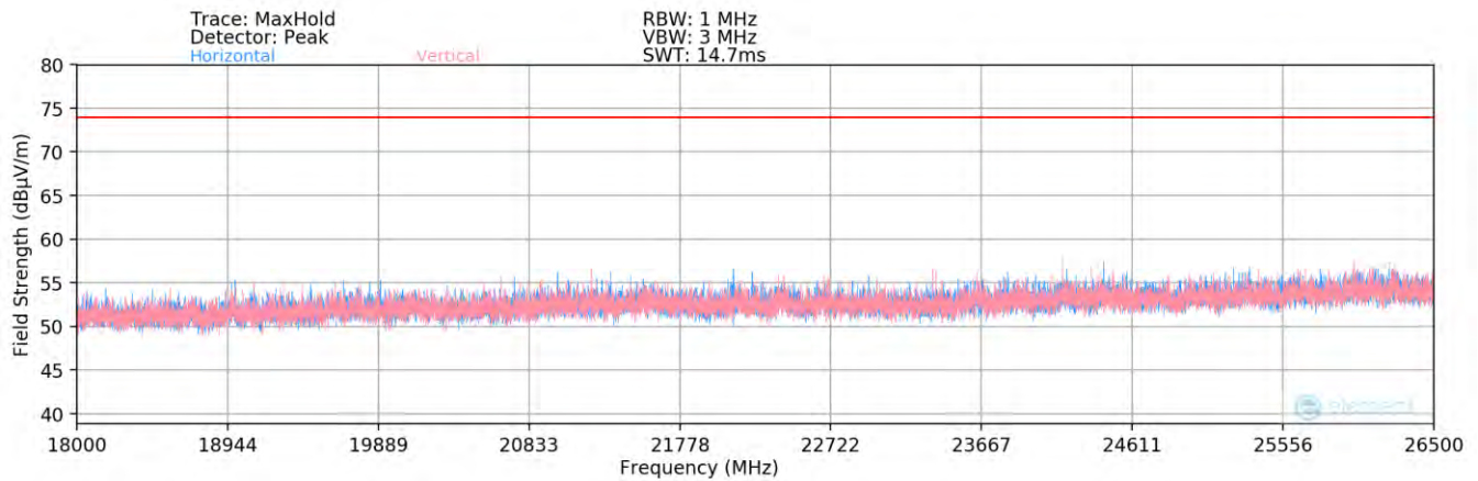
Plot 7-83. Radiated Spurious Plot above 18GHz SISO ANT2 – Half Open
