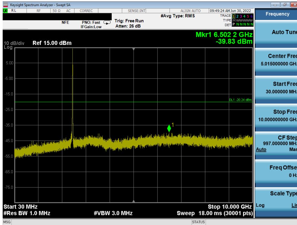
Plot 7-69. Conducted Spurious Plot ANT1 (802.11b – Ch. 11)
