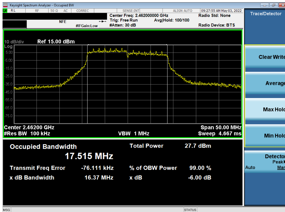
Plot 7-12. 6dB Bandwidth Plot ANT1 (802.11ax (2.4GHz) – Ch. 11)
