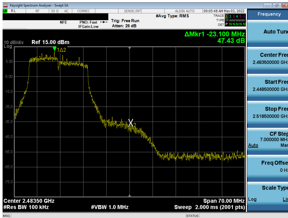
Plot 7-54. Band Edge Plot ANT1 (802.11n (2.4GHz) – Ch. 11)
