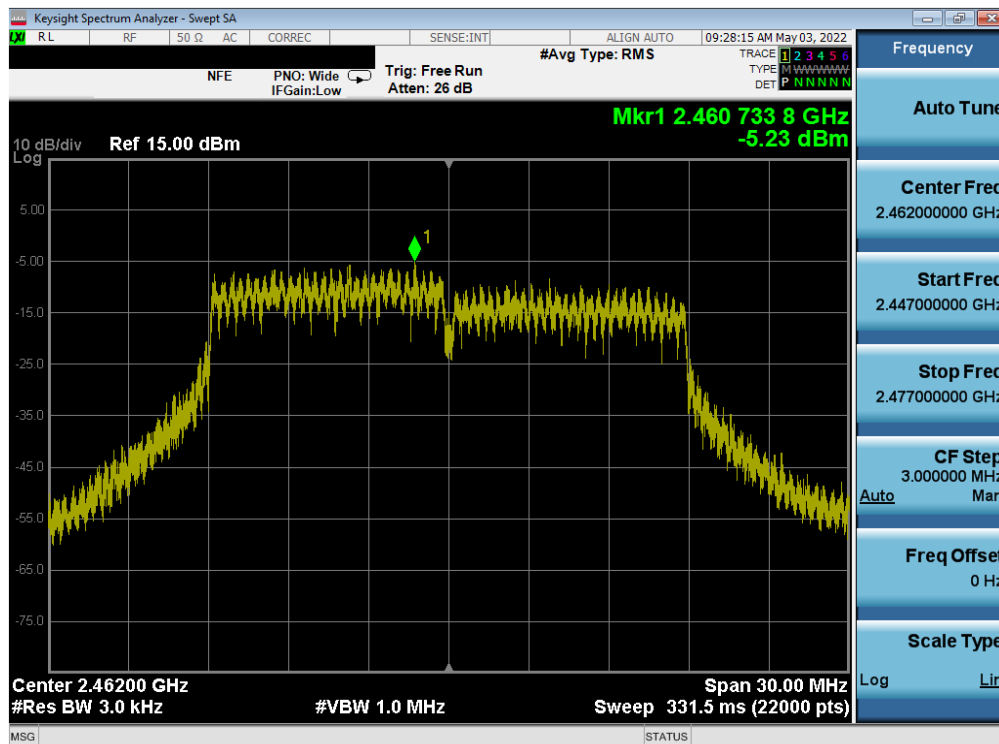
Plot 7-36. Power Spectral Density Plot ANT1 (802.11ax (2.4GHz) – Ch. 11)
