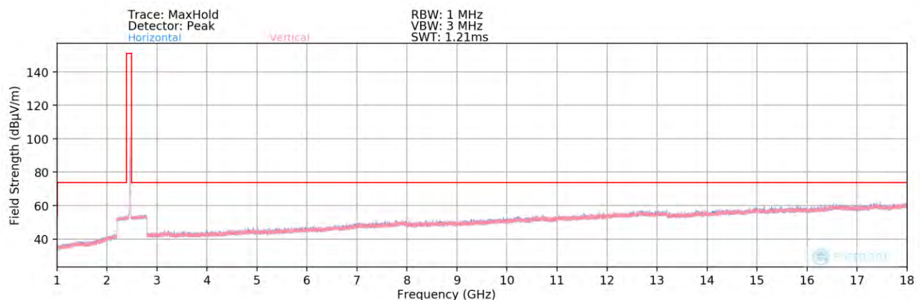
Plot 7-79. Radiated Spurious Plot above 1GHz SISO ANT2 (802.11b – Ch. 11) – Half Open
