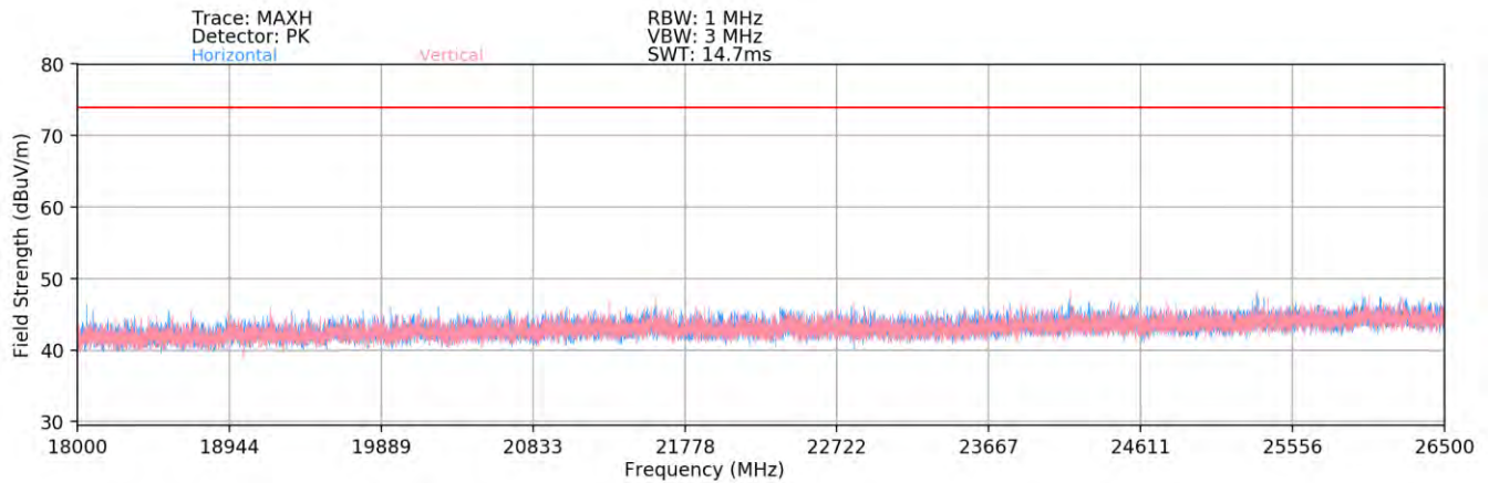
Plot 7-91. Radiated Spurious Plot above 18GHz MIMO/CDD – Half Open
