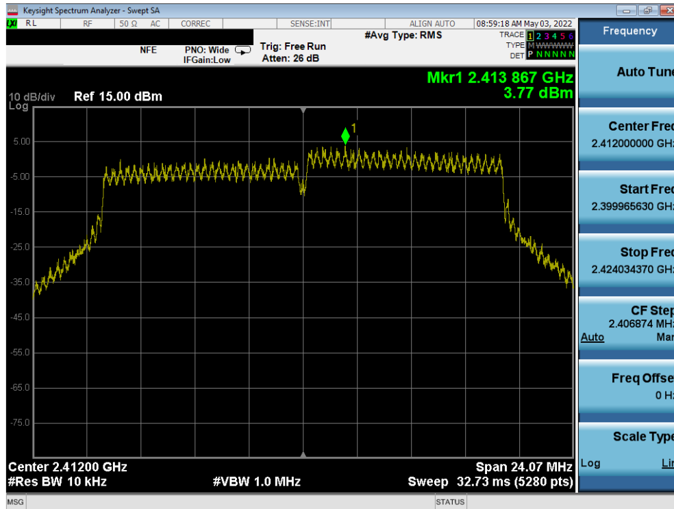
Plot 7-31. Power Spectral Density Plot ANT1 (802.11n (2.4GHz) – Ch. 1)
