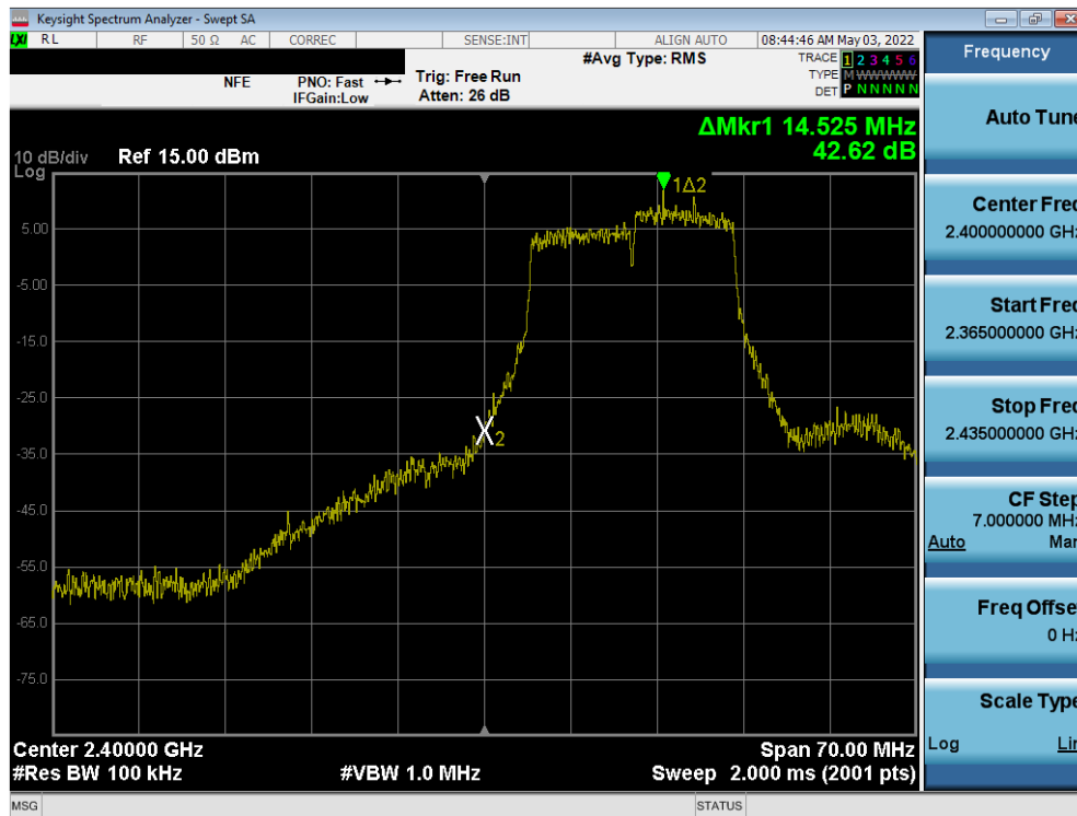
Plot 7-51. Band Edge Plot ANT1 (802.11g– Ch. 1)
