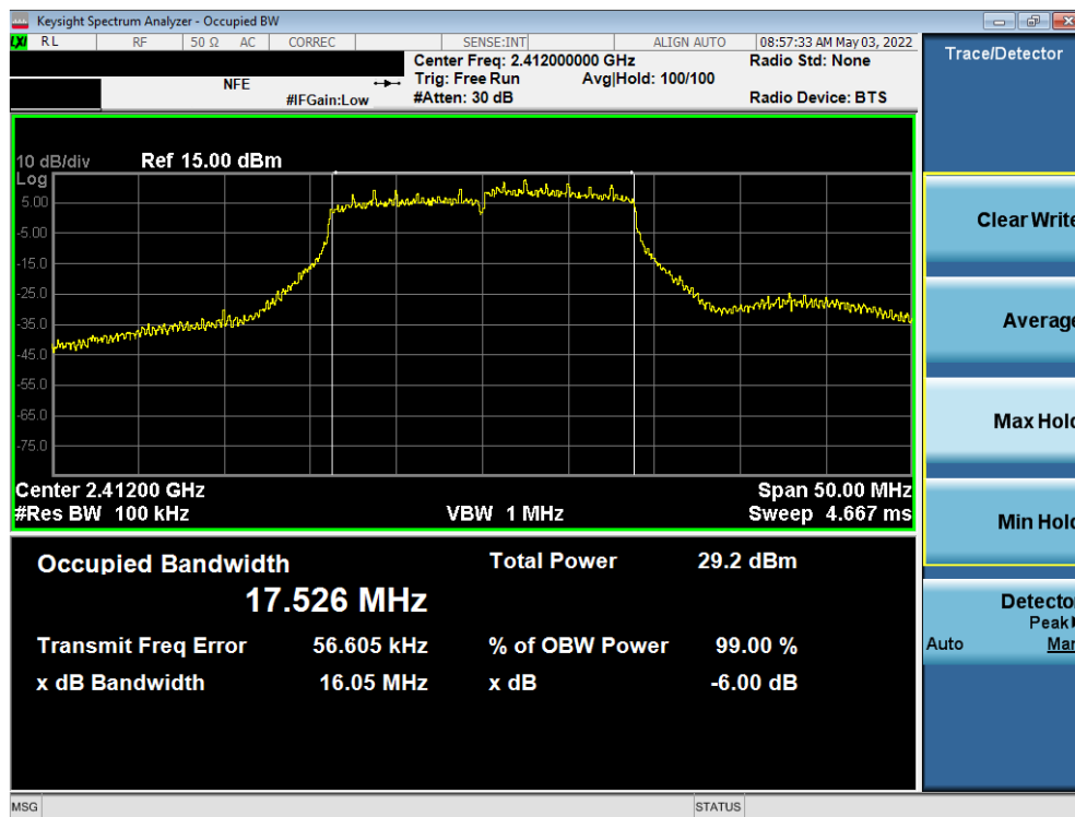
Plot 7-7. 6dB Bandwidth Plot ANT1 (802.11n (2.4GHz) – Ch. 1)
