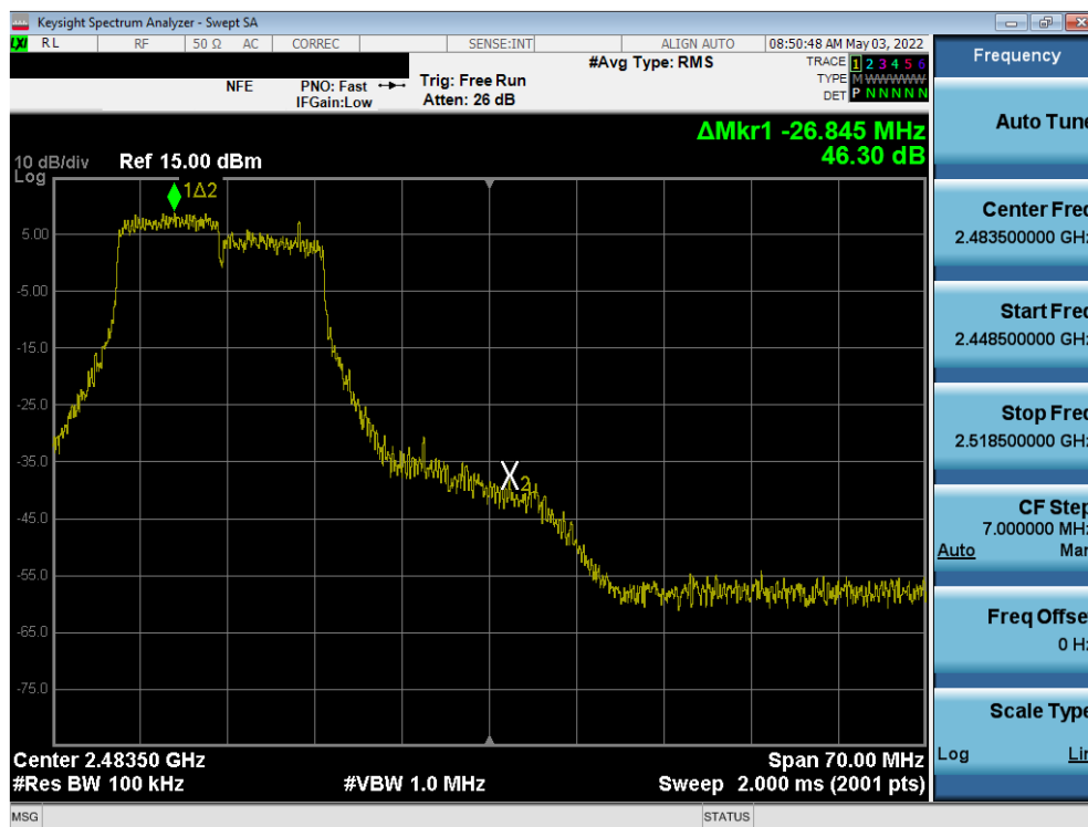
Plot 7-52. Band Edge Plot ANT1 (802.11g – Ch. 11)
