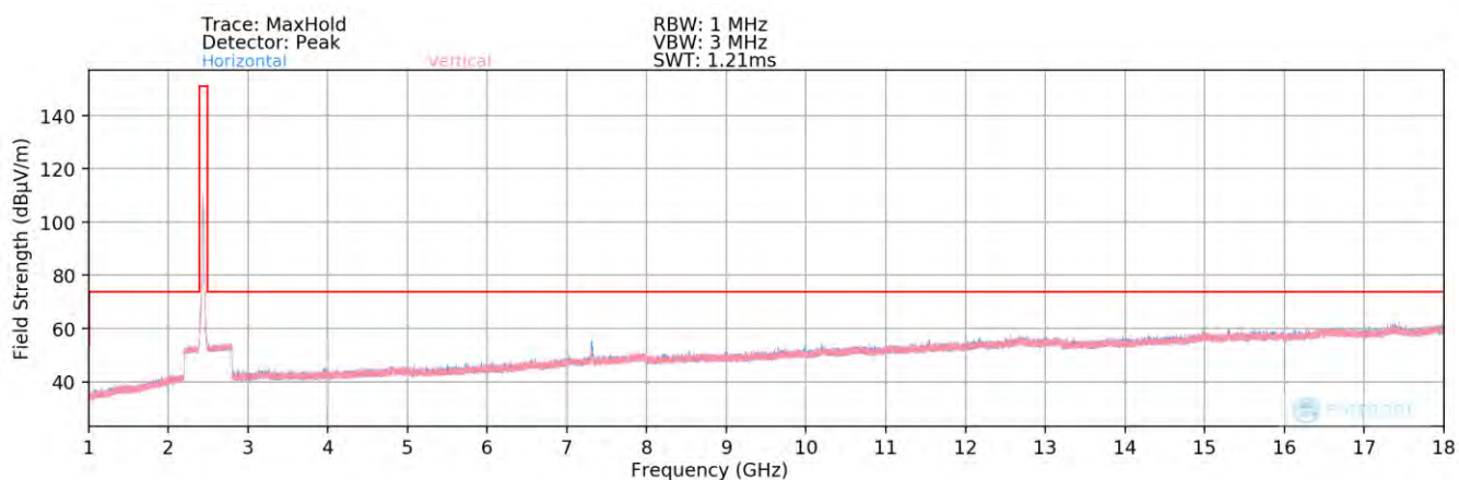
Plot 7-89. Radiated Spurious Plot above 1GHz MIMO/CDD (802.11g - Ch. 6) - Open
