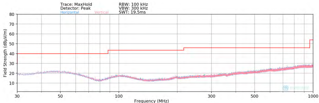
Plot 7-103. Radiated Spurious Plot below 1GHz
