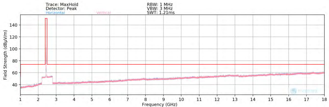
Plot 7-78. Radiated Spurious Plot above 1GHz SISO ANT2 (802.11b – Ch. 6) – Half Open
