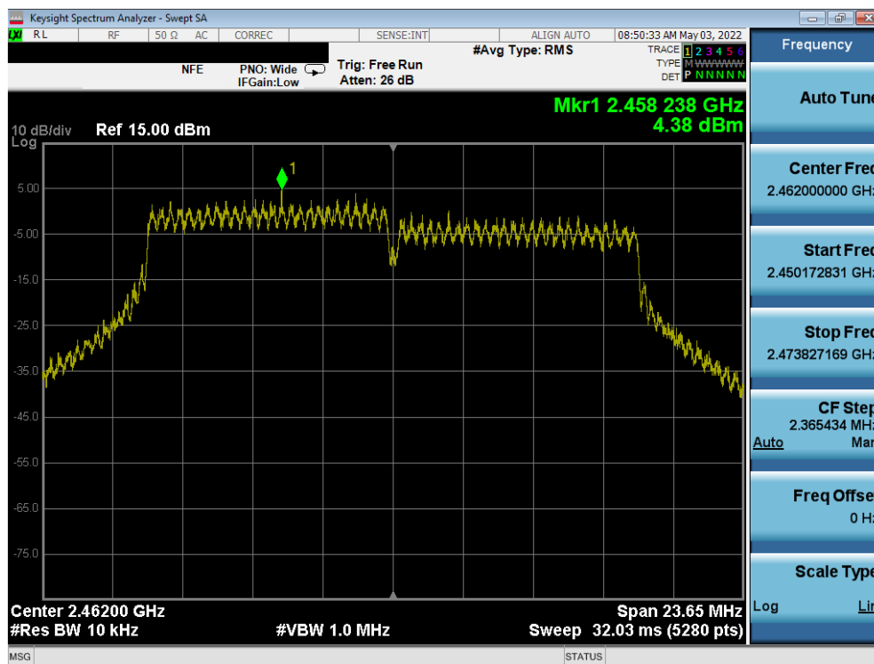
Plot 7-30. Power Spectral Density Plot ANT1 (802.11g – Ch. 11)
