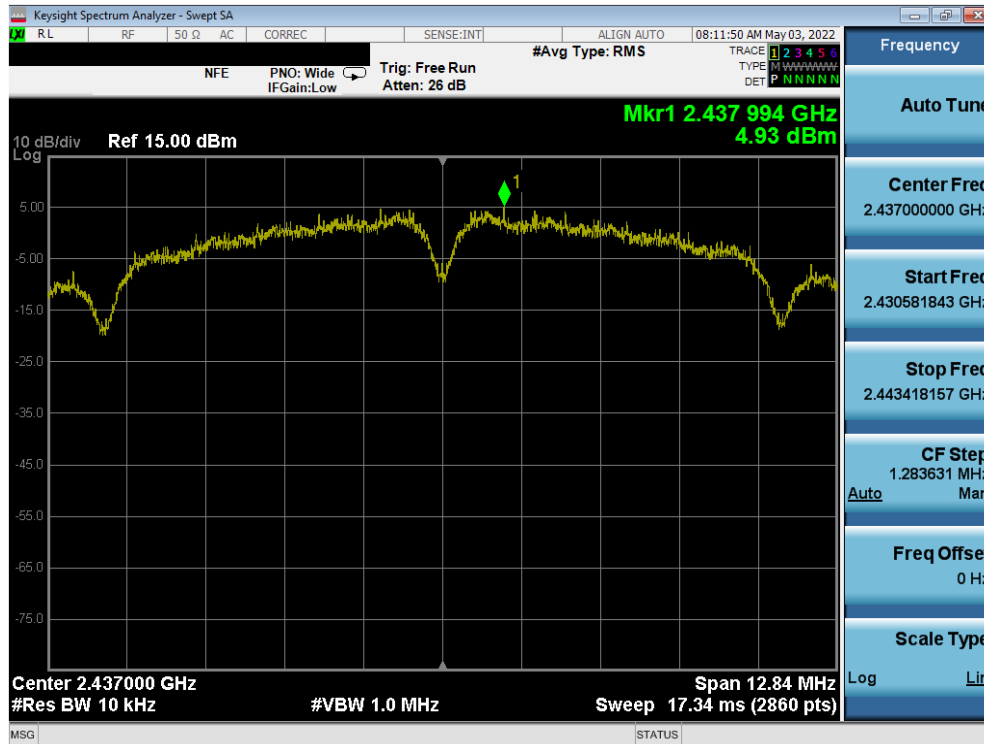
Plot 7-26. Power Spectral Density Plot ANT1 (802.11b – Ch. 6)
