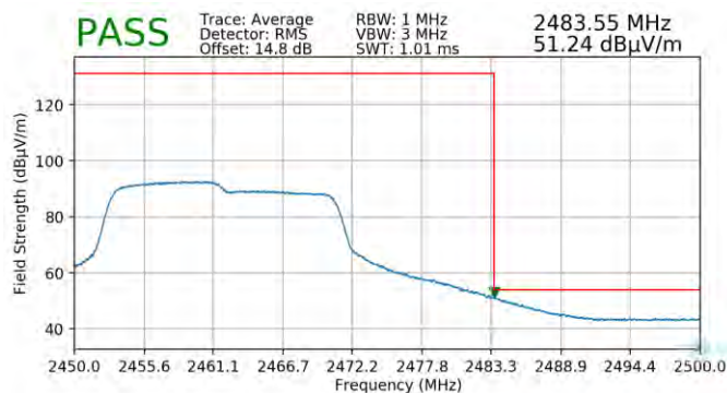
Plot 7-95. Radiated Restricted Upper Band Edge Measurement SISO ANT2 (Average)
