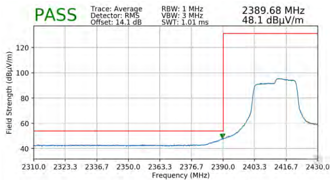
Plot 7-93. Radiated Restricted Band Edge Measurement SISO ANT2 with WCP (Average)
