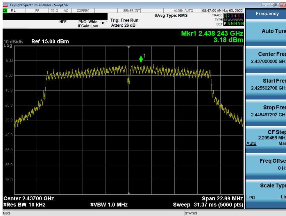
Plot 7-29. Power Spectral Density Plot ANT1 (802.11g – Ch. 6)
