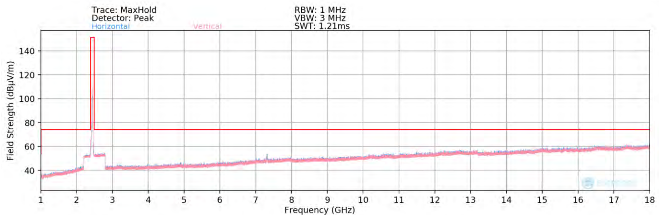
Plot 7-86. Radiated Spurious Plot above 1GHz MIMO/CDD (802.11g – Ch. 6) – Half Open
