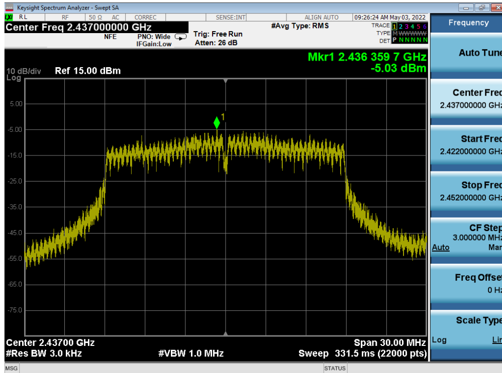
Plot 7-35. Power Spectral Density Plot ANT1 (802.11ax (2.4GHz) – Ch. 6)
