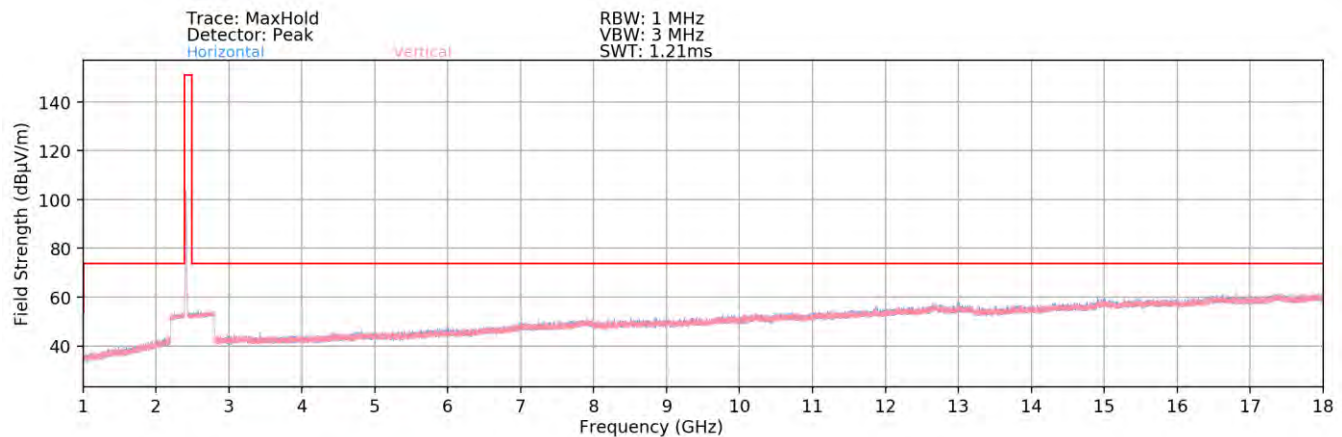
Plot 7-77. Radiated Spurious Plot above 1GHz SISO ANT2 (802.11b – Ch. 1) – Half Open
