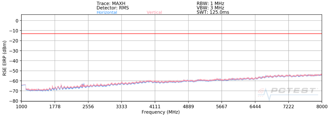
Plot 7-39. Radiated Spurious Plot Above 1GHz (LTE Band 14) – OPEN
