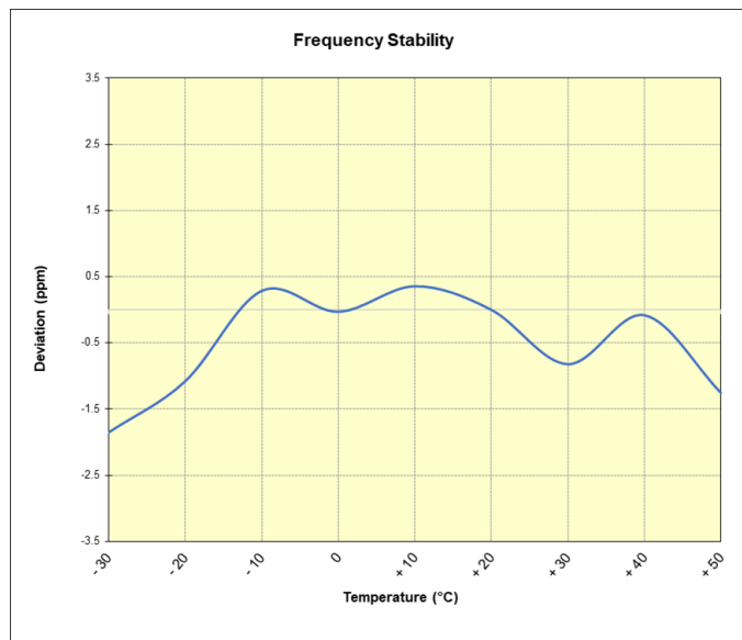
Plot 7-44. LTE Band 26 Frequency Stability Chart
