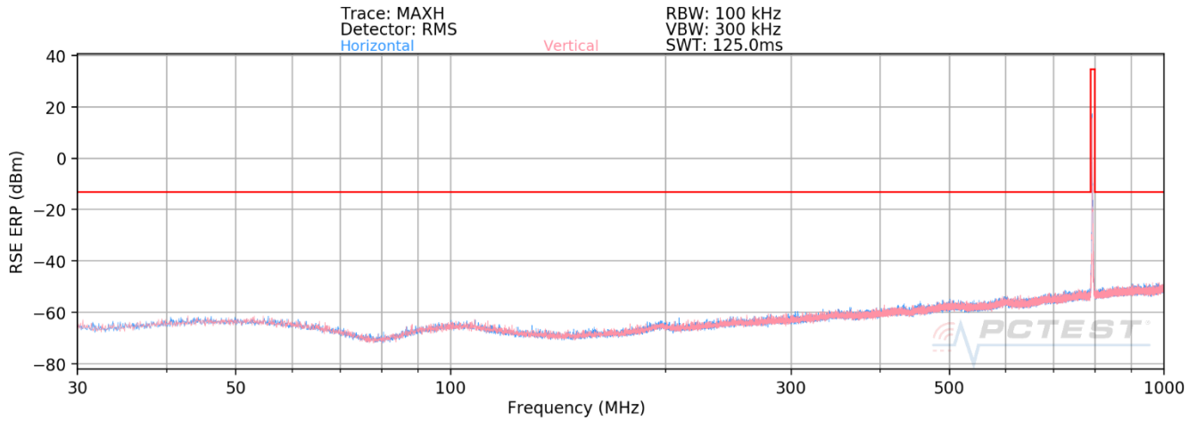
Plot 7-40. Radiated Spurious Plot Below 1GHz (LTE Band 26) – OPEN
