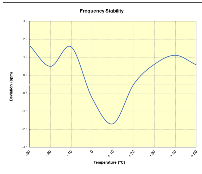
Plot 7-43. LTE Band 14 Frequency Stability Chart
