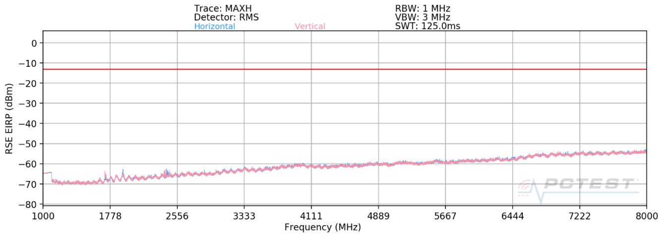
Plot 7-38. Radiated Spurious Plot Above 1GHz (LTE Band 14) – HALF OPEN
