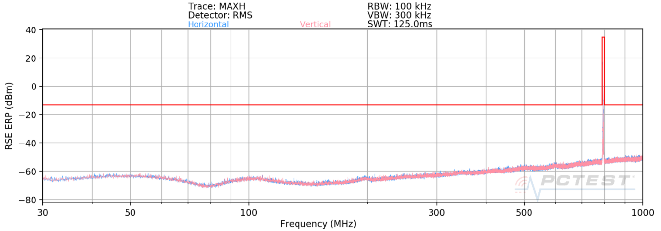
Plot 7-37. Radiated Spurious Plot Below 1GHz (LTE Band 14) – HALF OPEN
