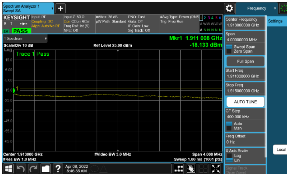
Plot 7-160. Extended Upper Band Edge Plot (NR Band n2 - 15MHz QPSK – Full RB)
