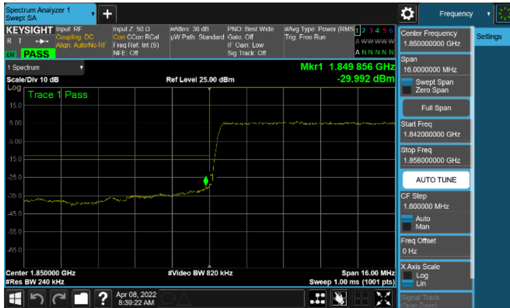
Plot 7-151. Lower Band Edge Plot (NR Band n25/2 - 20MHz QPSK – Full RB)
