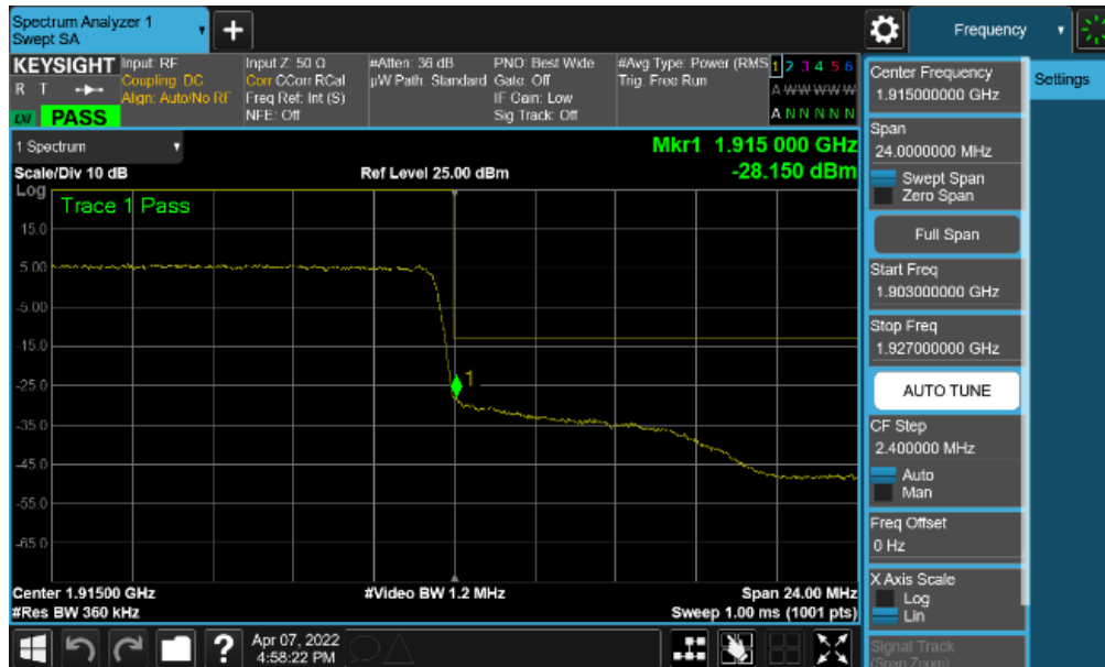
Plot 7-145. Upper Band Edge Plot (NR Band n25 - 30MHz QPSK – Full RB)
