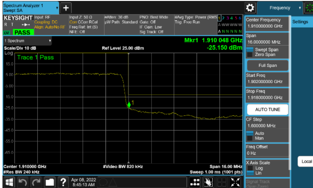
Plot 7-153. Upper Band Edge Plot (NR Band n2 - 20MHz QPSK – Full RB)
