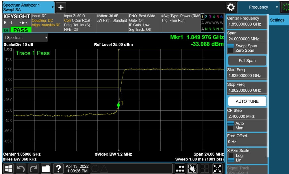
Plot 7-179. Lower Band Edge Plot (NR Band n25 - 30MHz QPSK – Full RB)
