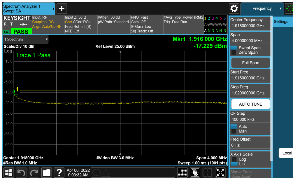
Plot 7-168. Extended Upper Band Edge Plot (NR Band n25 - 10MHz QPSK – Full RB)
