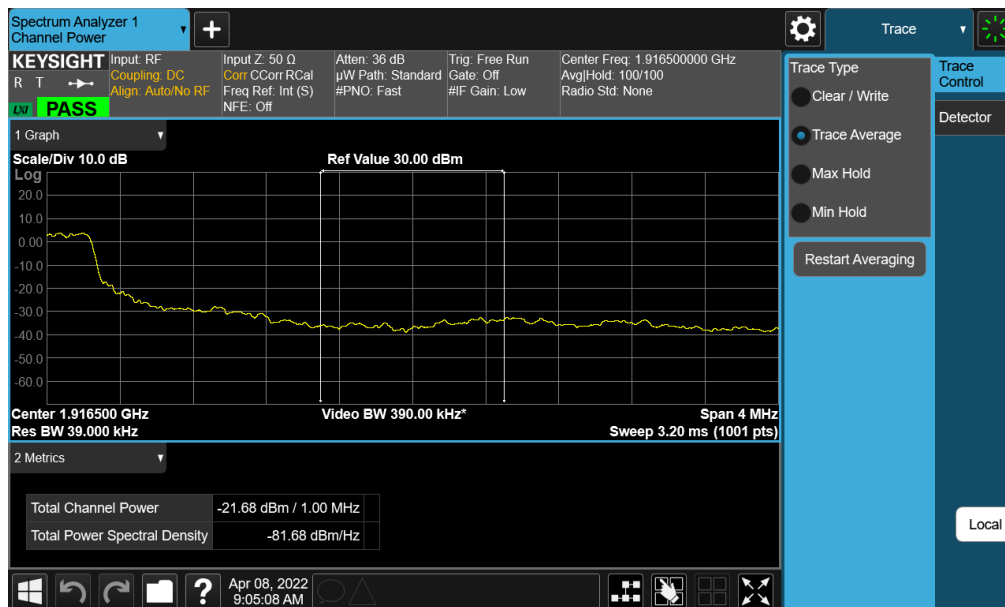
Plot 7-174. Extended Upper Band Edge Plot (NR Band n25 – 5MHz QPSK – Full RB)
