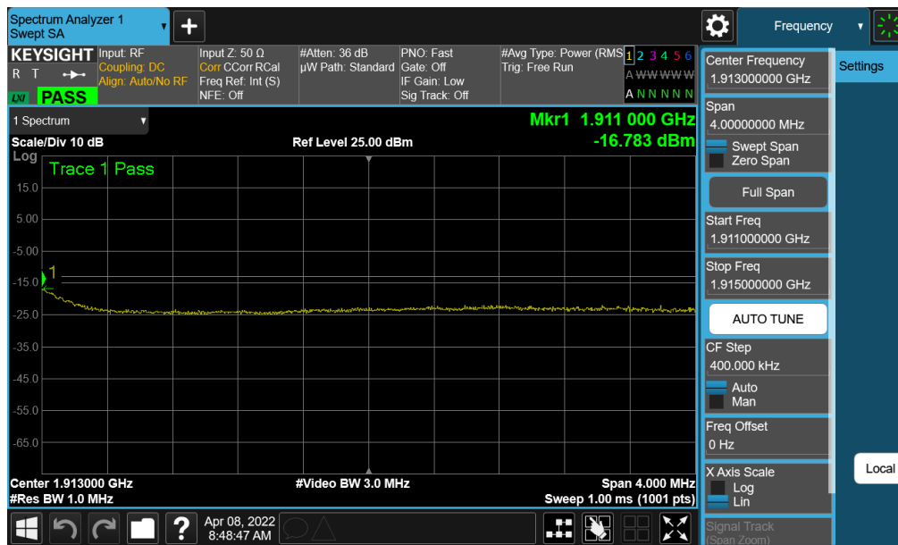
Plot 7-166. Extended Upper Band Edge Plot (NR Band n2 - 10MHz QPSK – Full RB)
