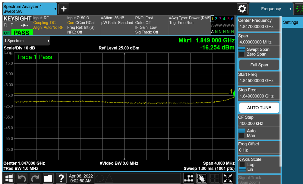
Plot 7-164. Extended Lower Band Edge Plot (NR Band n25/2 - 10MHz QPSK – Full RB)
