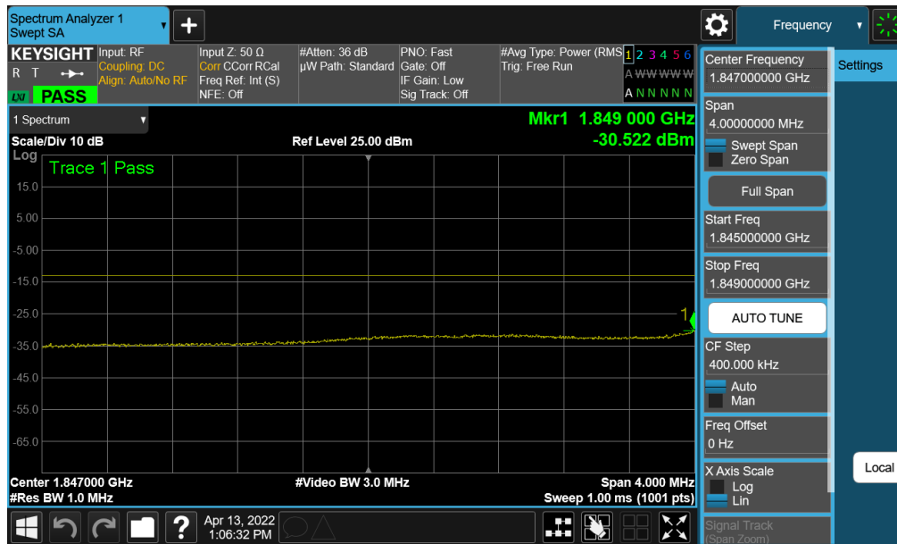
Plot 7-176. Extended Lower Band Edge Plot (NR Band n25 - 40MHz QPSK – Full RB)
