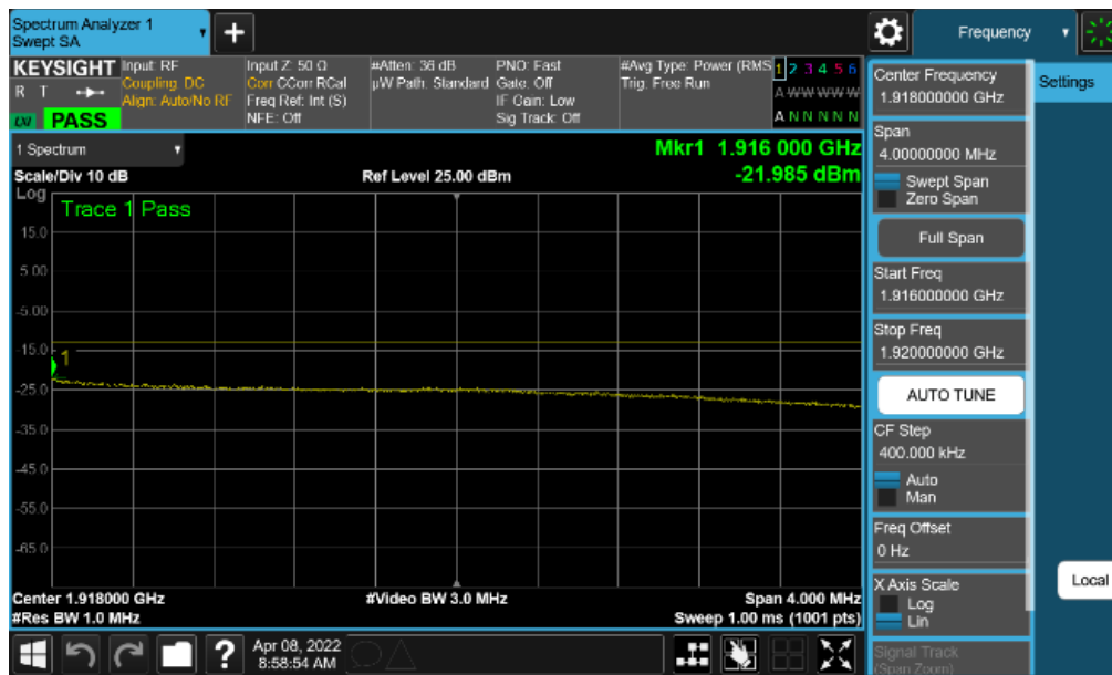
Plot 7-156. Extended Upper Band Edge Plot (NR Band n25 - 20MHz QPSK – Full RB)
