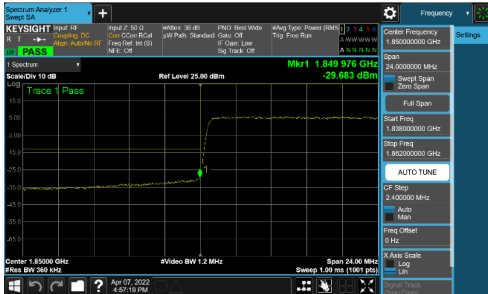
Plot 7-143. Lower Band Edge Plot (NR Band n25 - 30MHz QPSK – Full RB)
