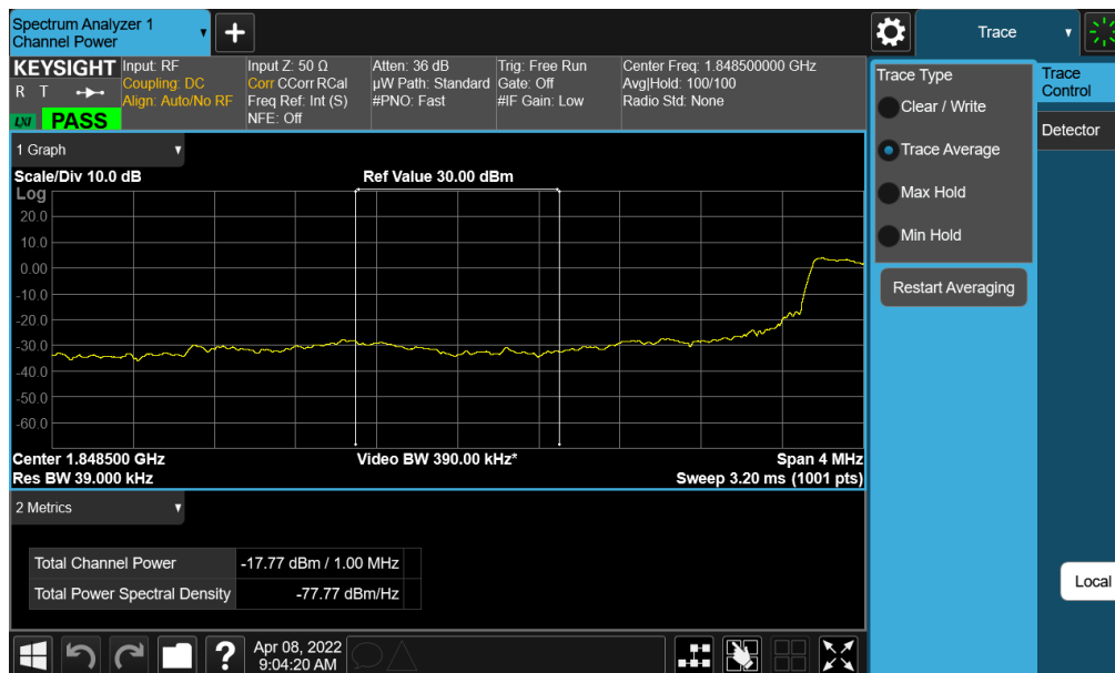
Plot 7-170. Extended Lower Band Edge Plot (NR Band n25/2 – 5MHz QPSK – Full RB)
