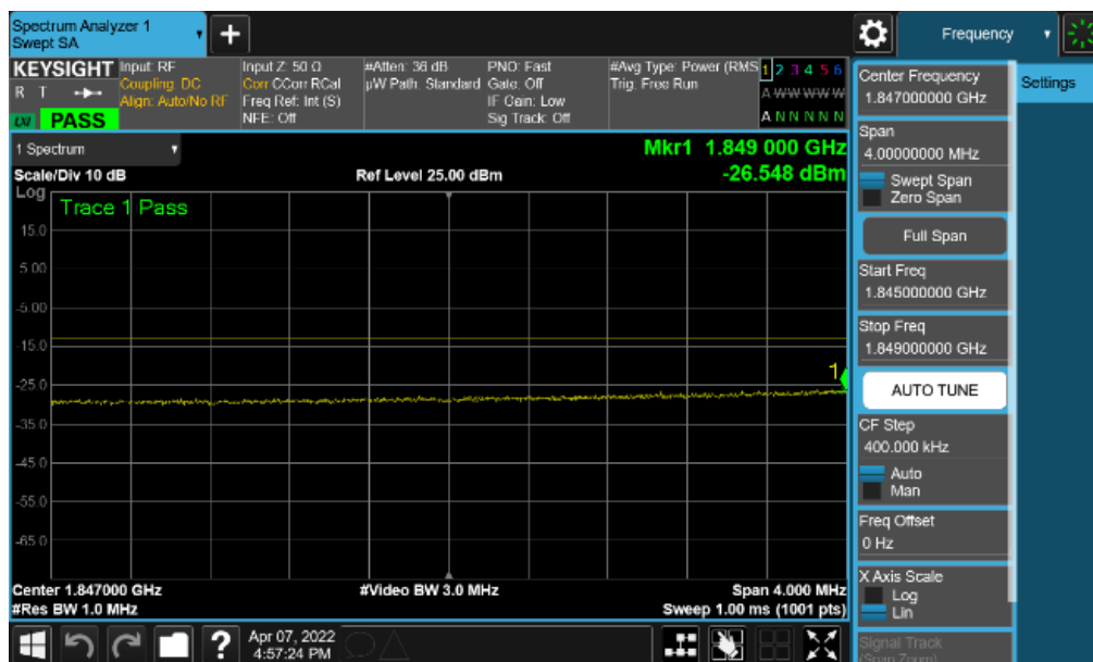
Plot 7-144. Extended Lower Band Edge Plot (NR Band n25 - 30MHz QPSK – Full RB)
