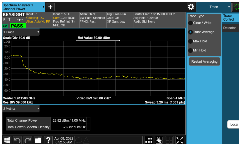
Plot 7-172. Extended Upper Band Edge Plot (NR Band n2 – 5MHz QPSK – Full RB)
