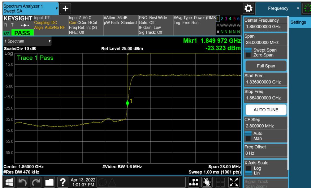
Plot 7-175. Lower Band Edge Plot (NR Band n25 - 40MHz QPSK – Full RB)
