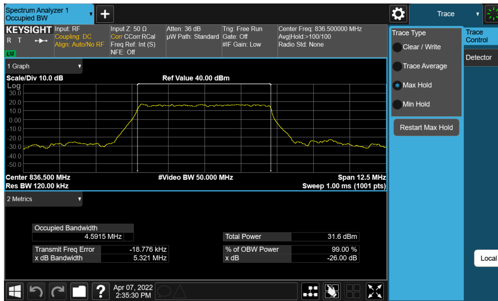
Plot 7-20. Occupied Bandwidth Plot (NR Band n5 - 5MHz π/2 BPSK - Full RB)
