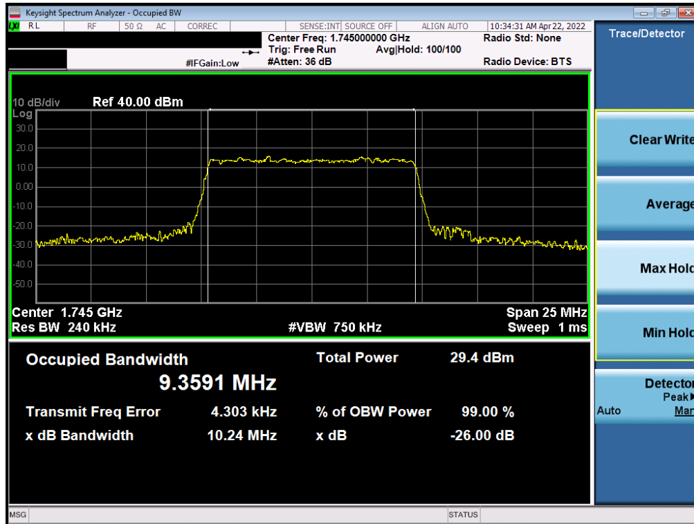
Plot 7-87. Occupied Bandwidth Plot (NR Band n66 - 10.0MHz CP-OFDM 16QAM - Full RB)
