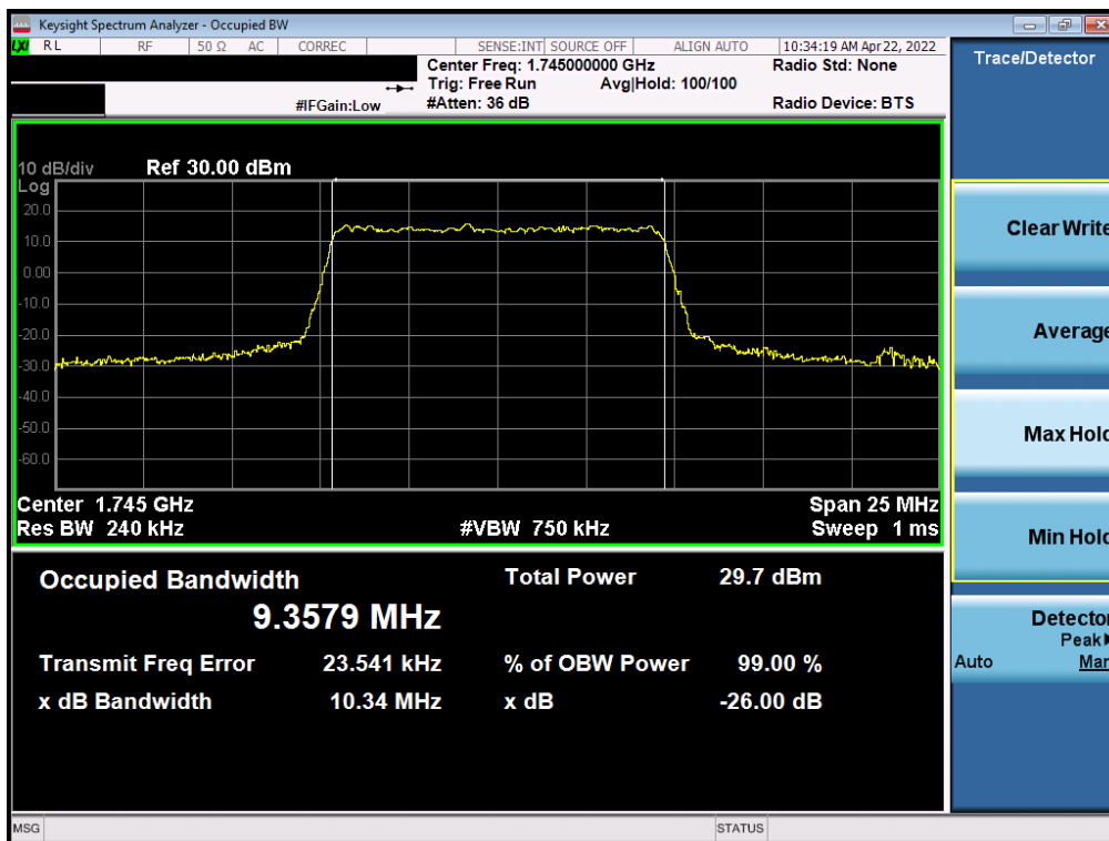
Plot 7-86. Occupied Bandwidth Plot (NR Band n66 - 10.0MHz CP-OFDM QPSK - Full RB)
