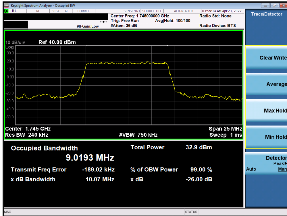
Plot 7-67. Occupied Bandwidth Plot (NR Band n66- 10MHz DFT-s-OFDM BPSK - Full RB)
