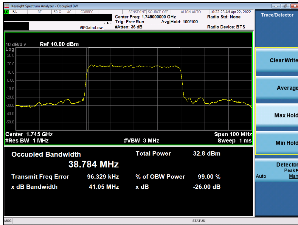
Plot 7-73. Occupied Bandwidth Plot (NR Band n66- 40MHz DFT-s-OFDM BPSK - Full RB)
