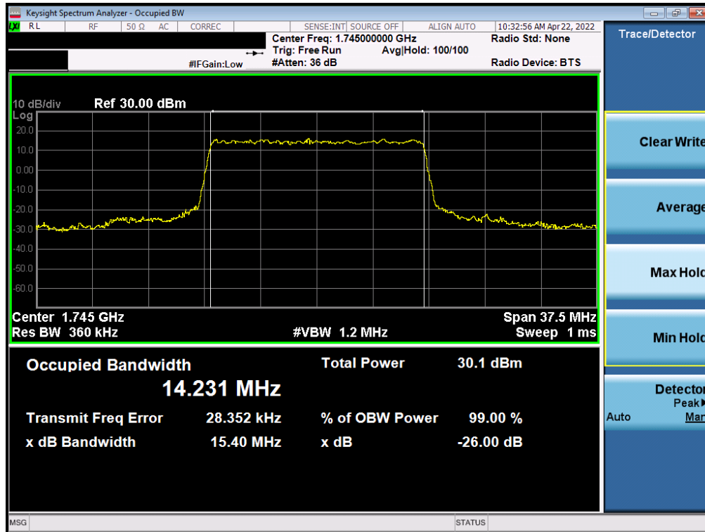
Plot 7-83. Occupied Bandwidth Plot (NR Band n66 - 15.0MHz CP-OFDM QPSK - Full RB)
