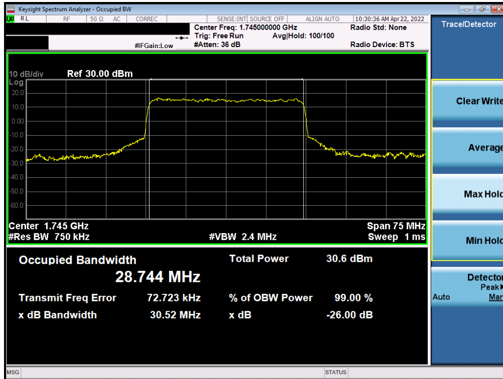
Plot 7-77. Occupied Bandwidth Plot (NR Band n66 - 30.0MHz CP-OFDM QPSK - Full RB)
