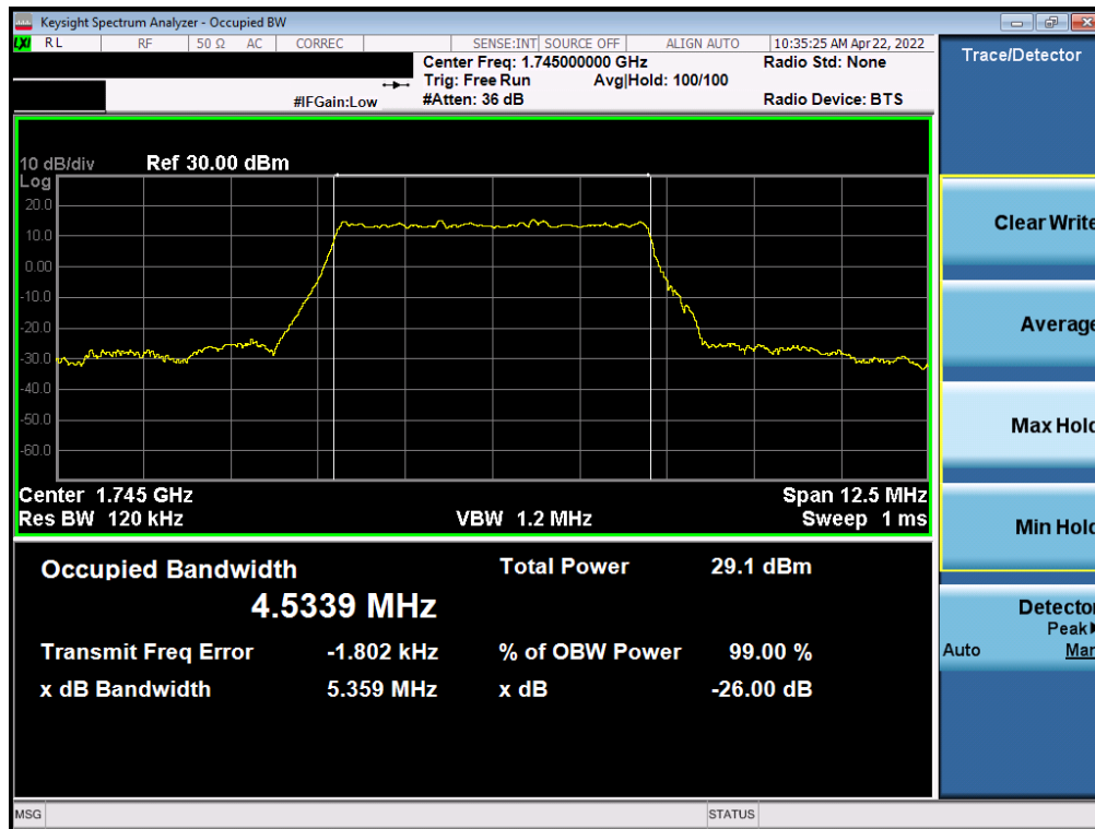
Plot 7-89. Occupied Bandwidth Plot (NR Band n66 - 5.0MHz CP-OFDM QPSK - Full RB)
