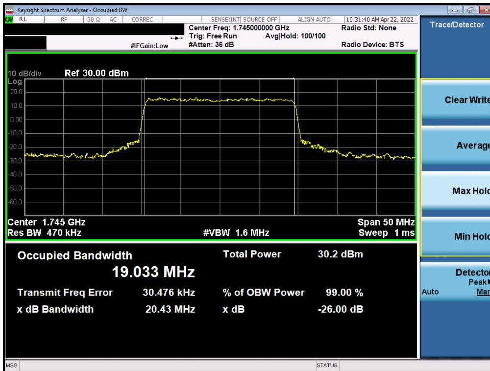
Plot 7-80. Occupied Bandwidth Plot (NR Band n66 - 20.0MHz CP-OFDM QPSK - Full RB)
