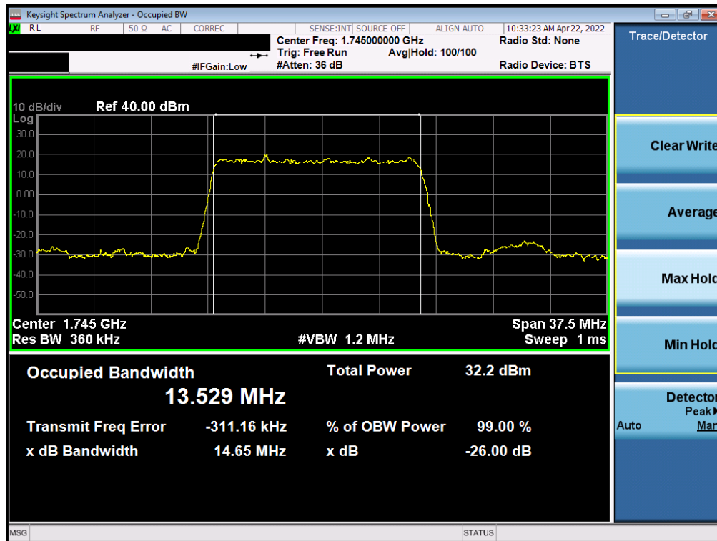
Plot 7-82. Occupied Bandwidth Plot (NR Band n66 - 15.0MHz DFT-s-OFDM BPSK - Full RB)
