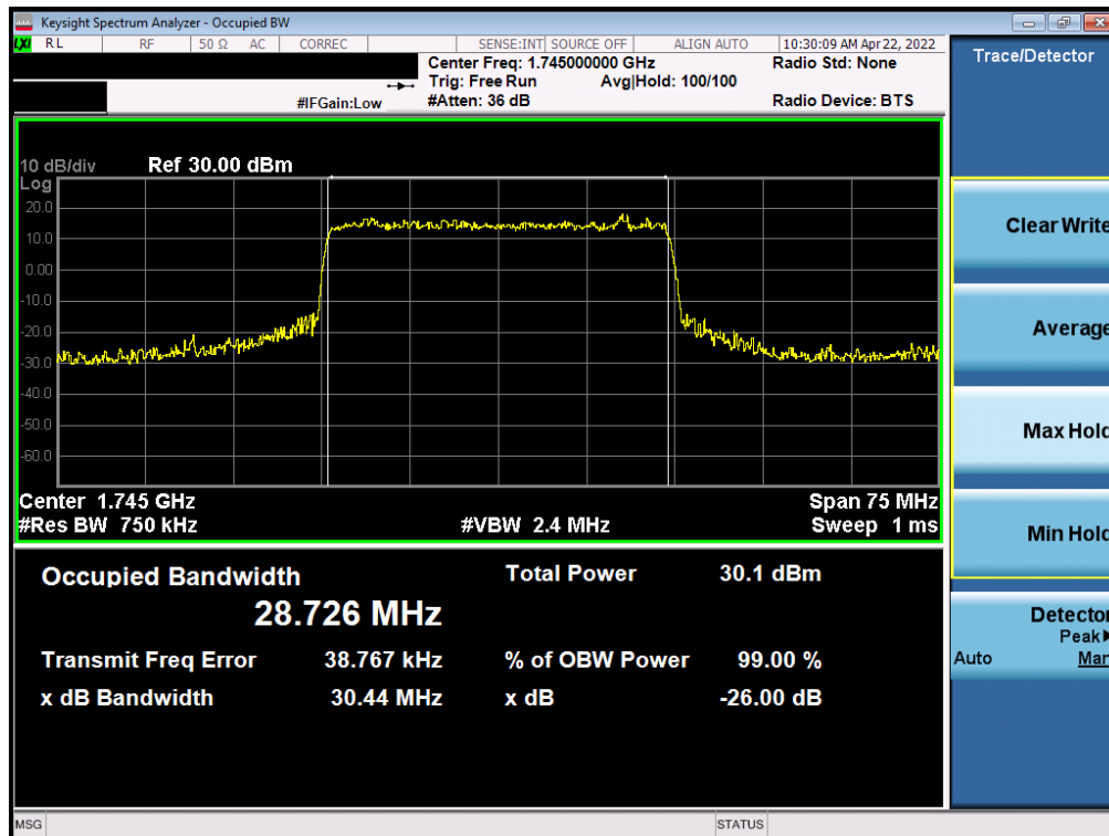
Plot 7-78. Occupied Bandwidth Plot (NR Band n66 - 30.0MHz CP-OFDM 16QAM - Full RB)
