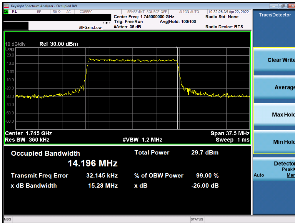
Plot 7-84. Occupied Bandwidth Plot (NR Band n66 - 15.0MHz CP-OFDM 16QAM - Full RB)
