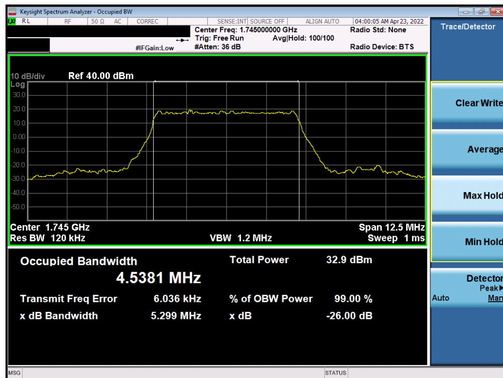
Plot 7-70. Occupied Bandwidth Plot (NR Band n66- 5MHz DFT-s-OFDM BPSK - Full RB)
