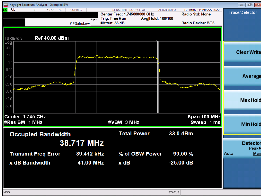
Plot 7-55. Occupied Bandwidth Plot (NR Band n66- 40MHz DFT-s-OFDM BPSK - Full RB)
