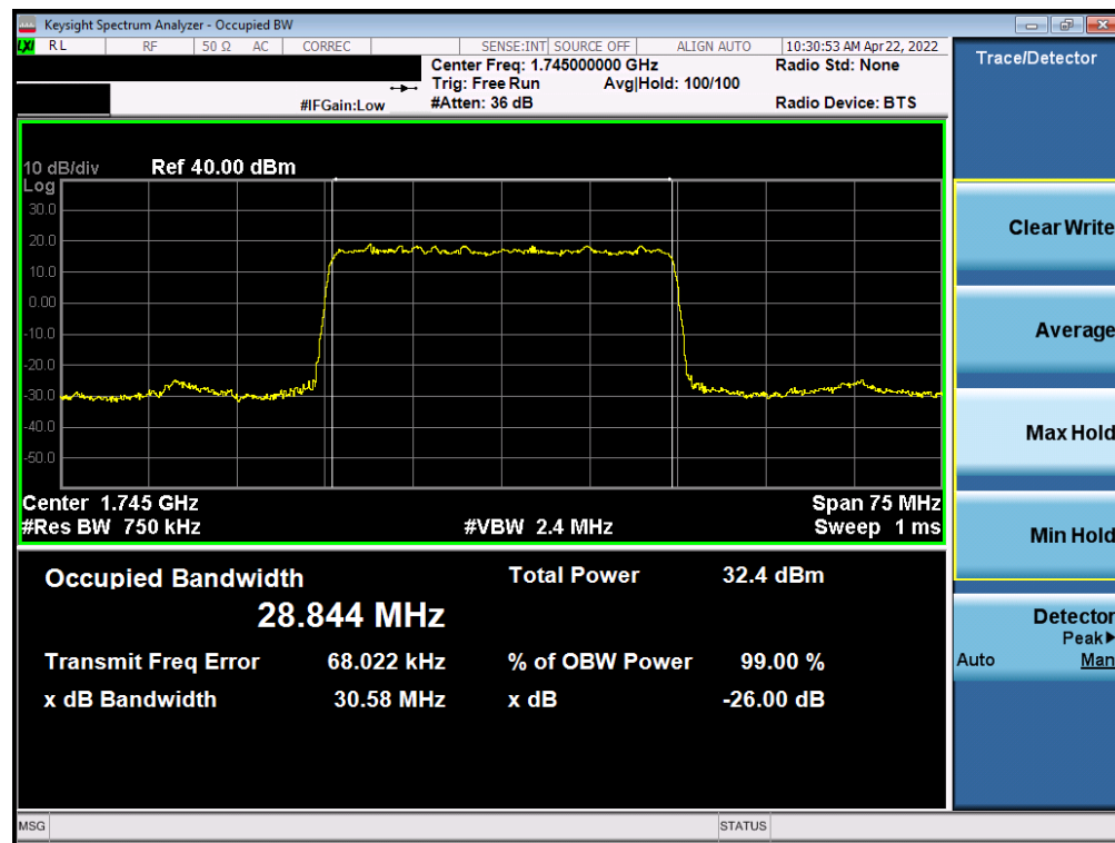
Plot 7-76. Occupied Bandwidth Plot (NR Band n66- 30MHz DFT-s-OFDM BPSK - Full RB)
