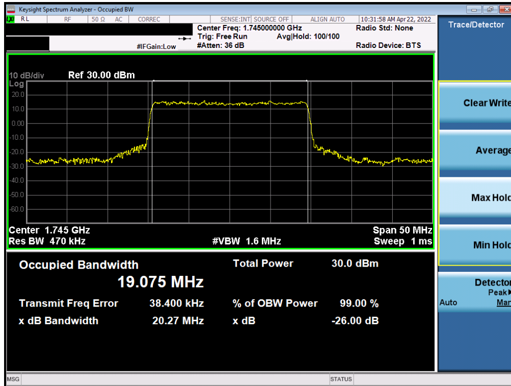
Plot 7-81. Occupied Bandwidth Plot (NR Band n66 - 20.0MHz CP-OFDM 16QAM - Full RB)
