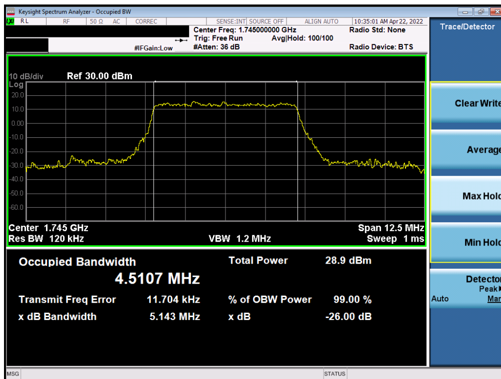
Plot 7-90. Occupied Bandwidth Plot (NR Band n66 - 5.0MHz CP-OFDM 16QAM - Full RB)
