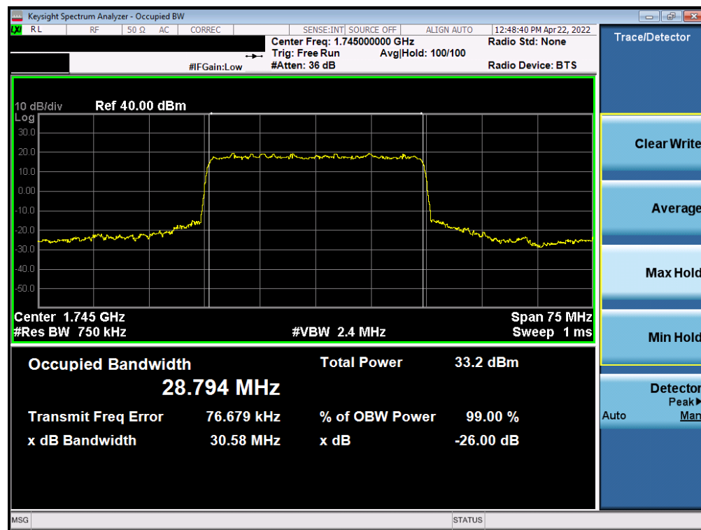
Plot 7-58. Occupied Bandwidth Plot (NR Band n66- 30MHz DFT-s-OFDM BPSK - Full RB)
