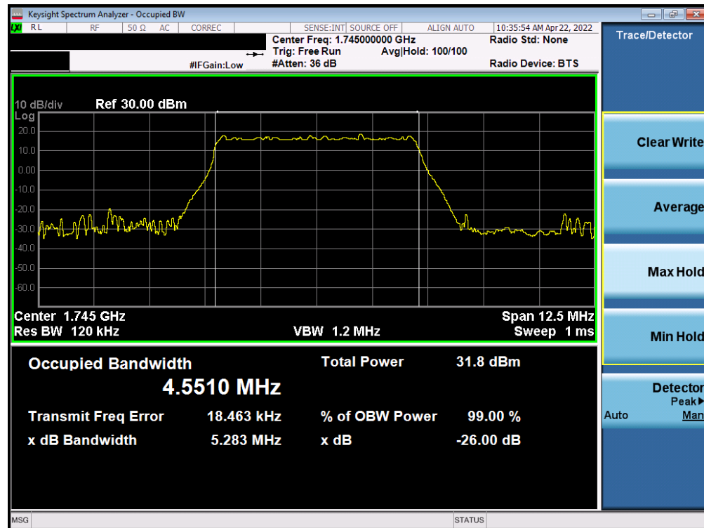
Plot 7-88. Occupied Bandwidth Plot (NR Band n66- 5MHz DFT-s-OFDM BPSK - Full RB)
