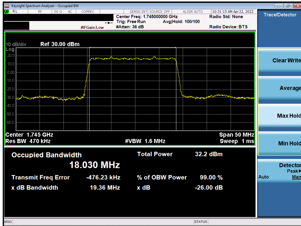
Plot 7-79. Occupied Bandwidth Plot (NR Band n66- 20MHz DFT-s-OFDM BPSK - Full RB)
