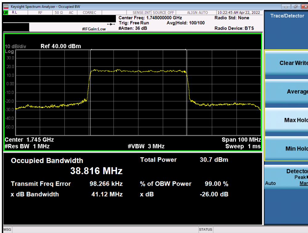
Plot 7-74. Occupied Bandwidth Plot (NR Band n66 - 40.0MHz CP-OFDM QPSK - Full RB)
