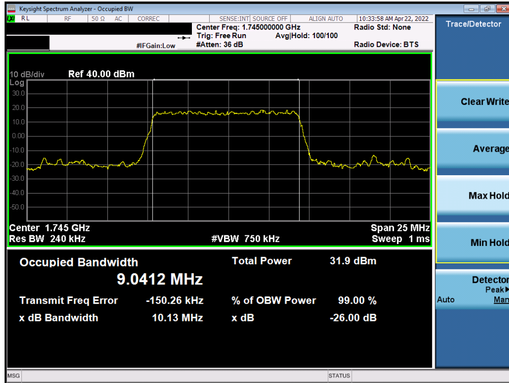
Plot 7-85. Occupied Bandwidth Plot (NR Band n66- 10MHz DFT-s-OFDM BPSK - Full RB)
