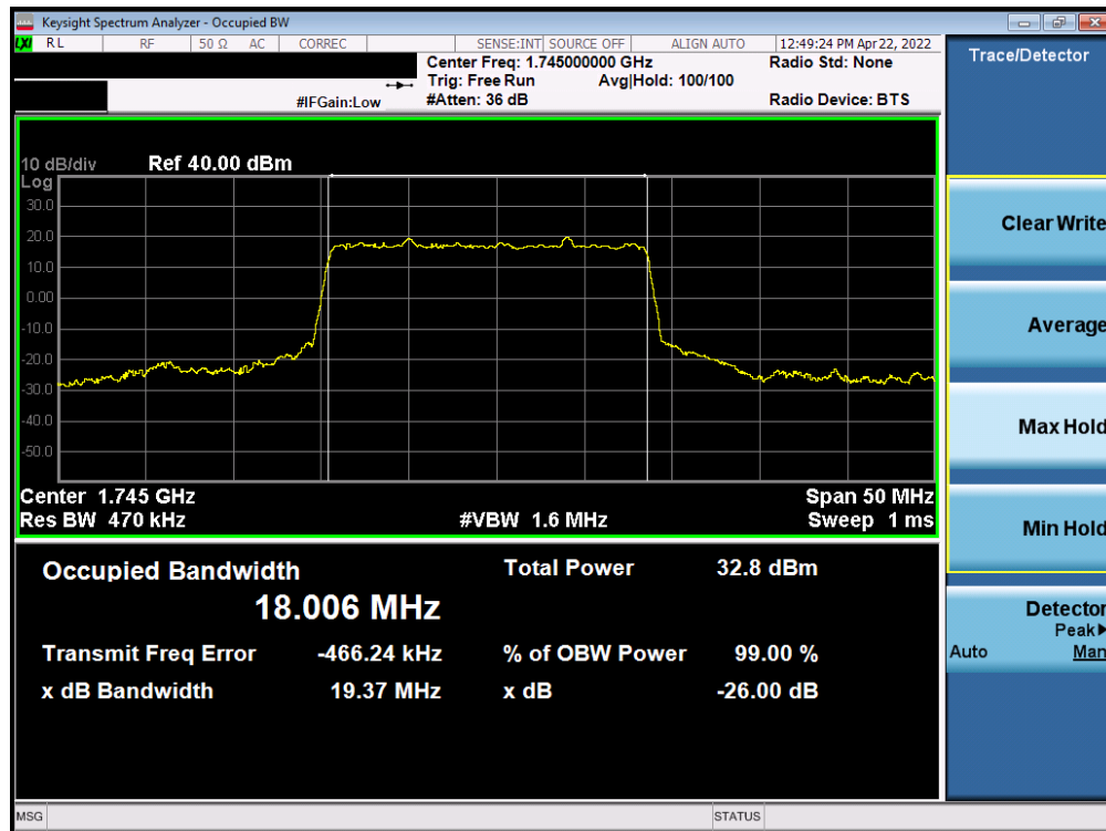
Plot 7-61. Occupied Bandwidth Plot (NR Band n66- 20MHz DFT-s-OFDM BPSK - Full RB)
