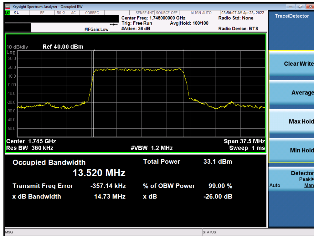
Plot 7-64. Occupied Bandwidth Plot (NR Band n66- 15MHz DFT-s-OFDM BPSK - Full RB)
