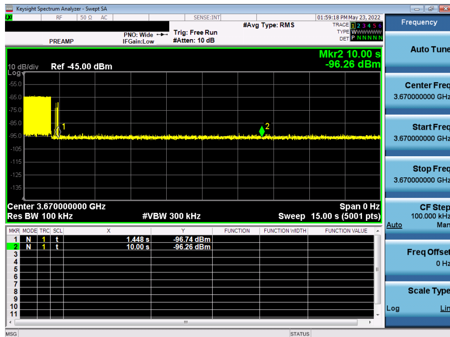
Plot 7-197. Run#2 End User Device Discontinues Operations within 10s
