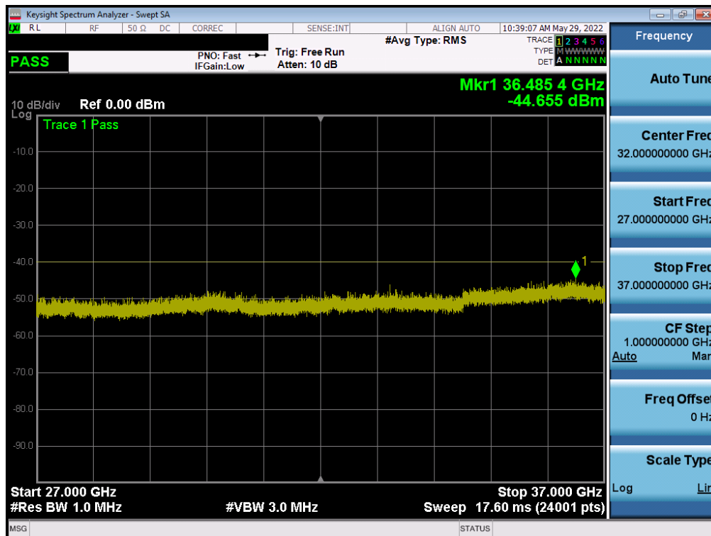
Plot 7-80. Conducted Spurious Plot (NR Band n48 - 40MHz QPSK - Low Channel - Ant E)
