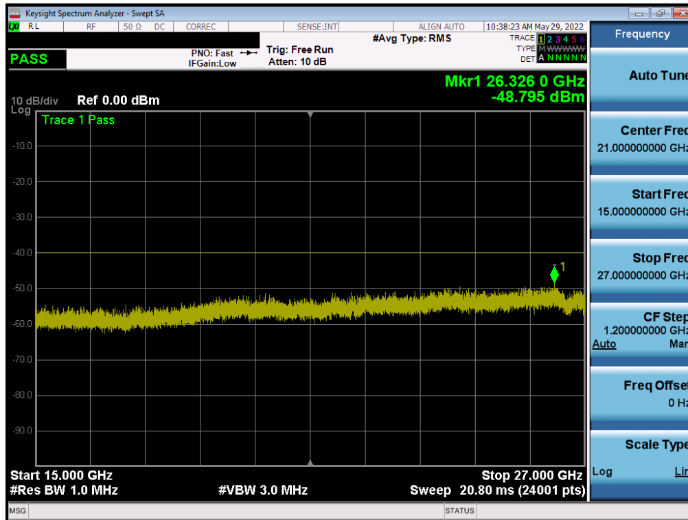
Plot 7-79. Conducted Spurious Plot (NR Band n48 - 40MHz QPSK - Low Channel - Ant E)
