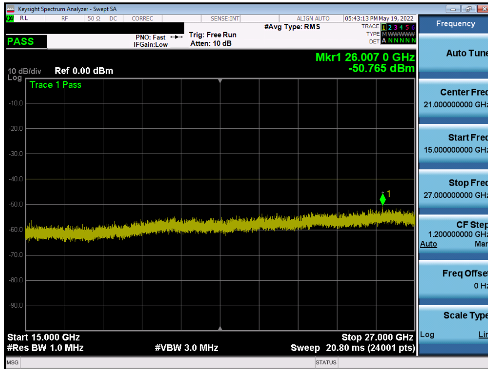
Plot 7-55. Conducted Spurious Plot (NR Band n48 - 40MHz QPSK - Low Channel - Ant F)
