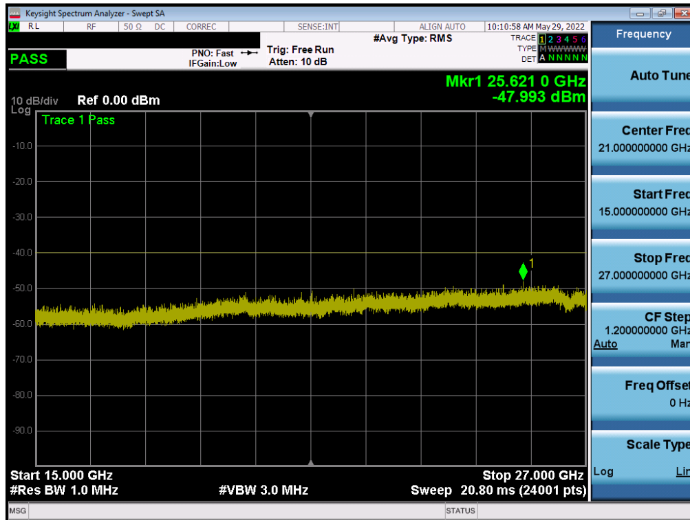
Plot 7-75. Conducted Spurious Plot (NR Band n48 - 40MHz QPSK - High Channel - Ant I)
