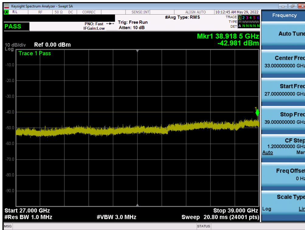
Plot 7-76. Conducted Spurious Plot (NR Band n48 - 40MHz QPSK - High Channel - Ant I)
