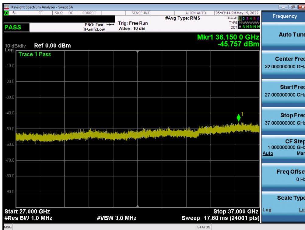
Plot 7-56. Conducted Spurious Plot (NR Band n48 - 40MHz QPSK - Low Channel - Ant F)
