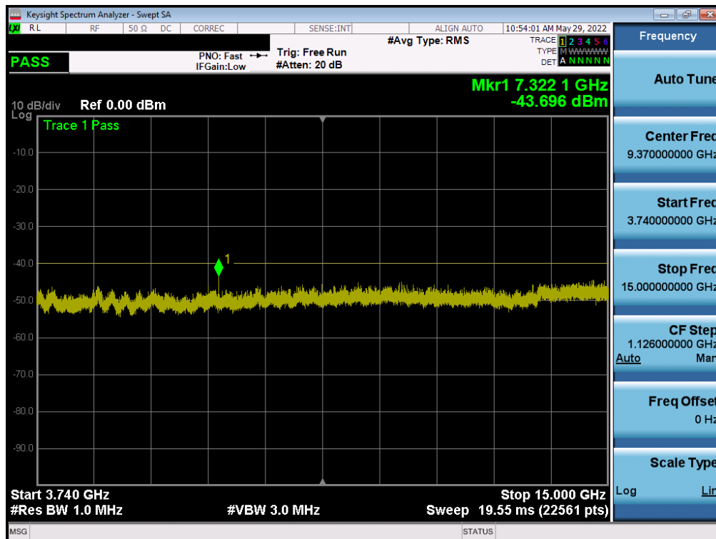
Plot 7-86. Conducted Spurious Plot (NR Band n48 - 40MHz QPSK - High Channel - Ant E)
