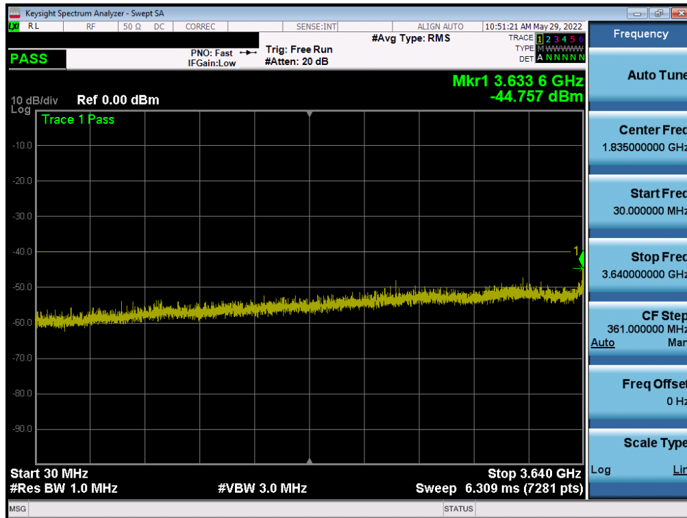
Plot 7-85. Conducted Spurious Plot (NR Band n48 - 40MHz QPSK - High Channel - Ant E)
