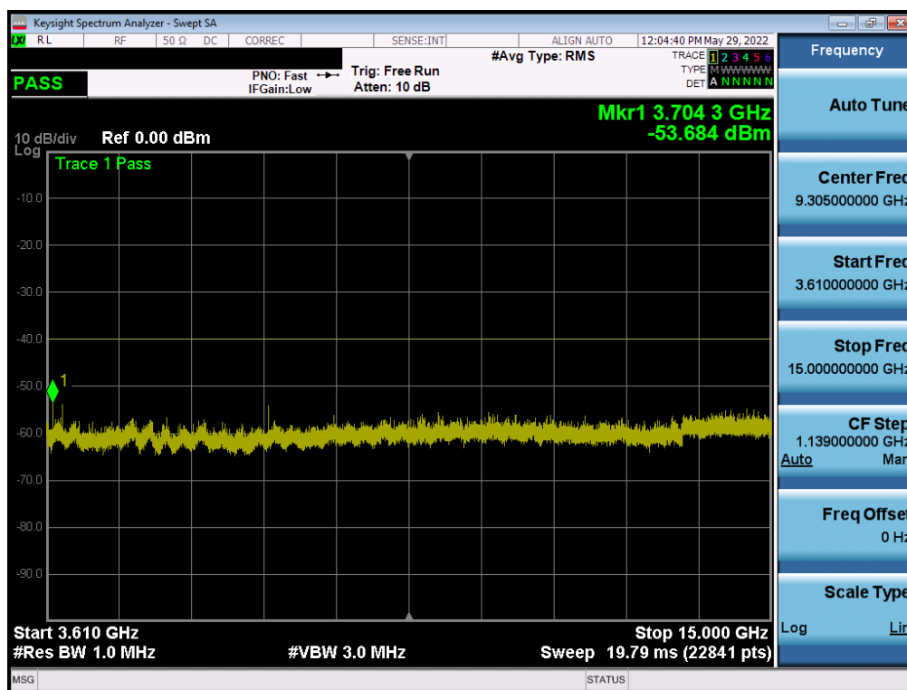
Plot 7-90. Conducted Spurious Plot (NR Band n48 - 40MHz QPSK - Low Channel - Ant C)
