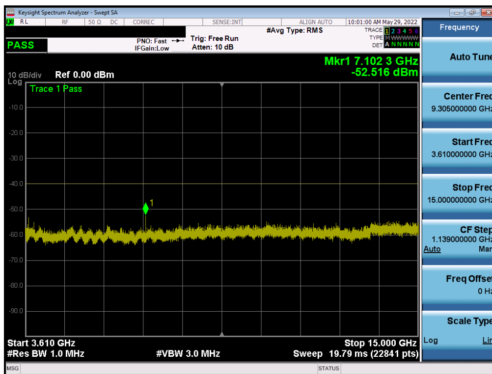
Plot 7-66. Conducted Spurious Plot (NR Band n48 - 40MHz QPSK - Low Channel - Ant I)
