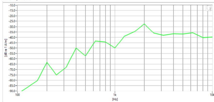
Noise Spectrum
