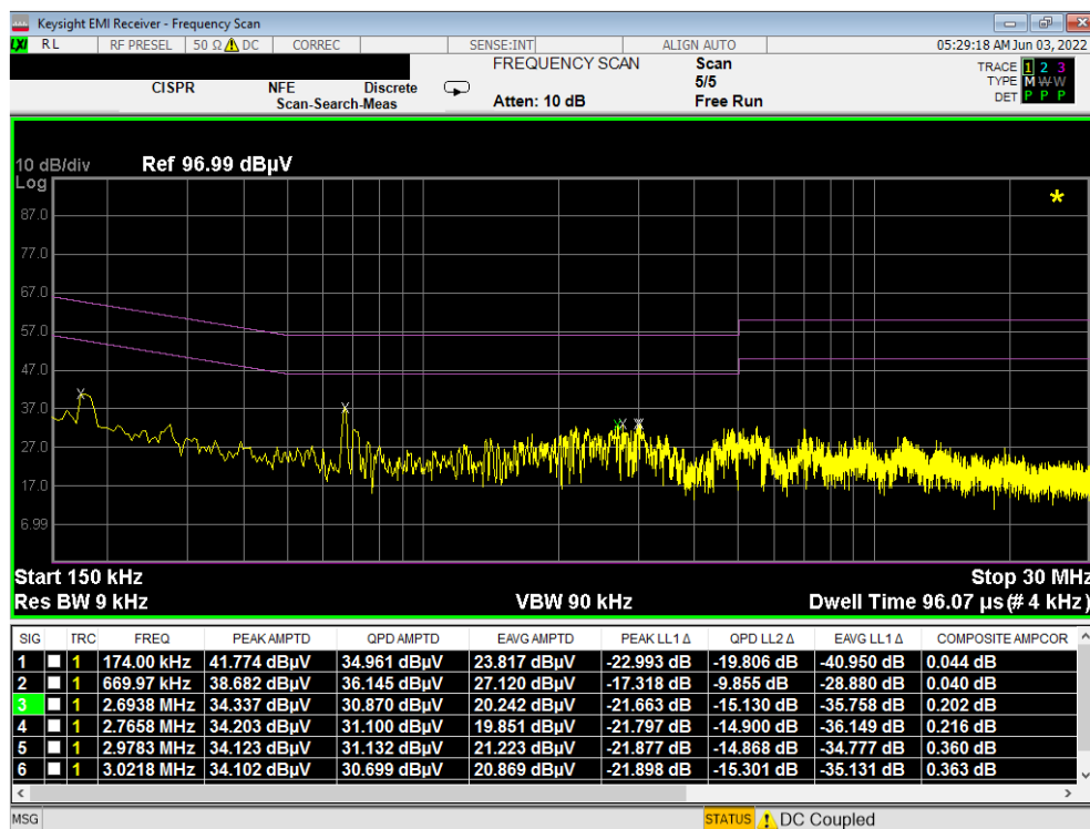
Plot 7-512. Line Conducted Plot with 802.11a UNII Band 3 (N) – Closed
