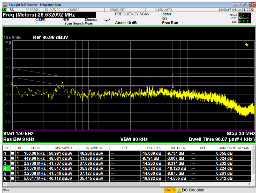
Plot 7-505. Line Conducted Plot with 802.11a UNII Band 2C (L1) – Open
