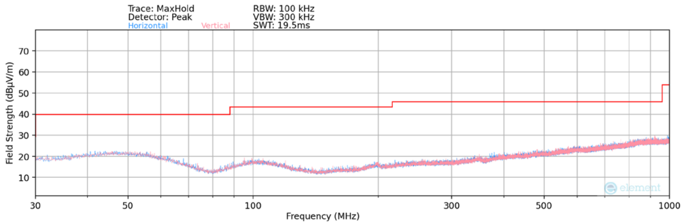
Plot 7-495. Radiated Spurious Plot below 1GHz (5GHz – 2.4 GHz)
