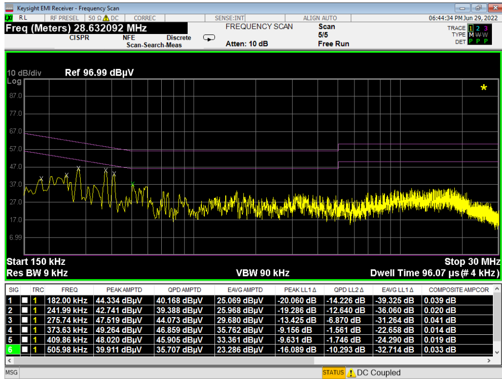
Plot 7-506. Line Conducted Plot with 802.11a UNII Band 2C (L1) – Closed
