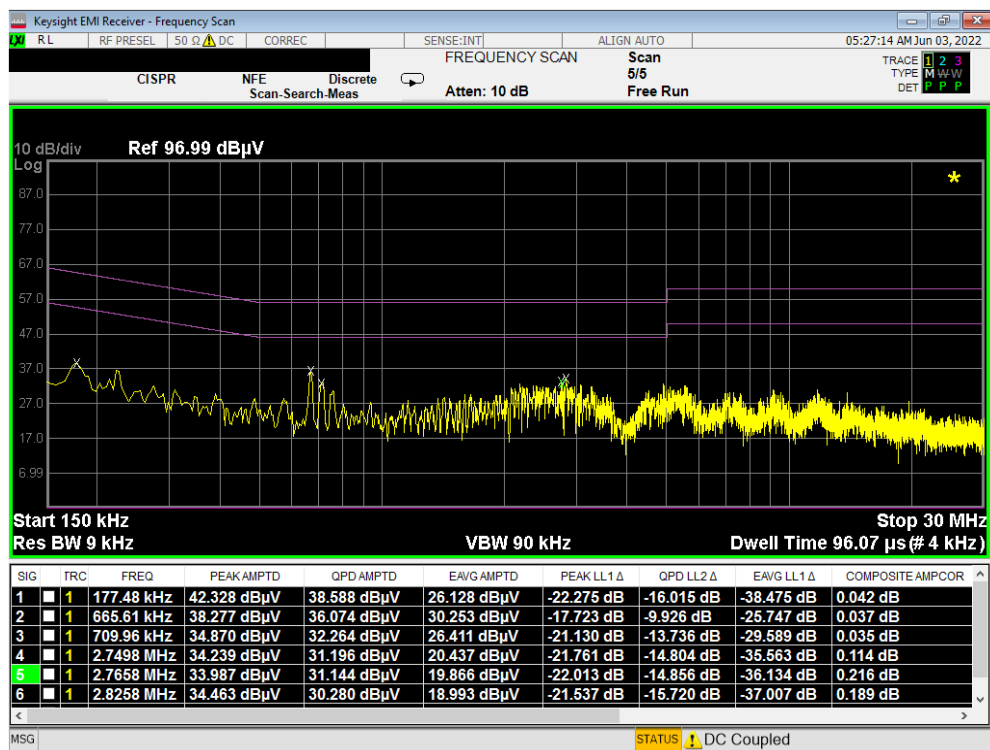
Plot 7-508. Line Conducted Plot with 802.11a UNII Band 2C (N) – Closed
