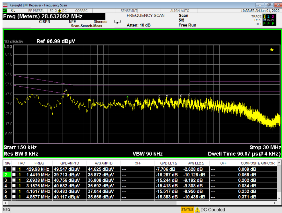
Plot 7-501. Line Conducted Plot with 802.11a UNII Band 2A (L1) – Open
