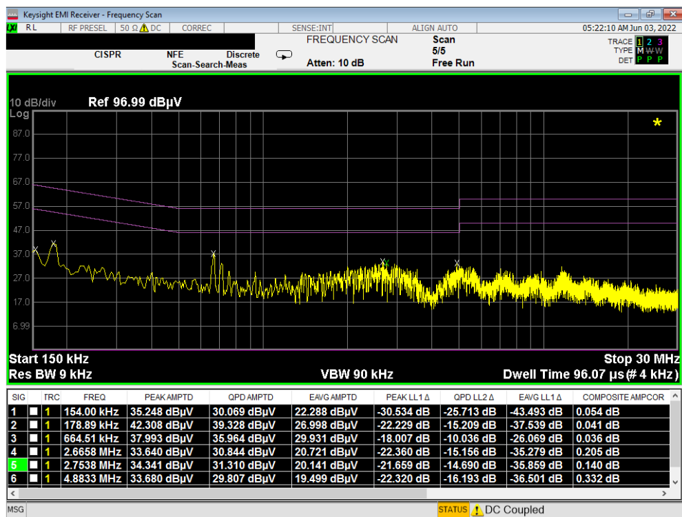
Plot 7-504. Line Conducted Plot with 802.11a UNII Band 2A (N) – Closed
