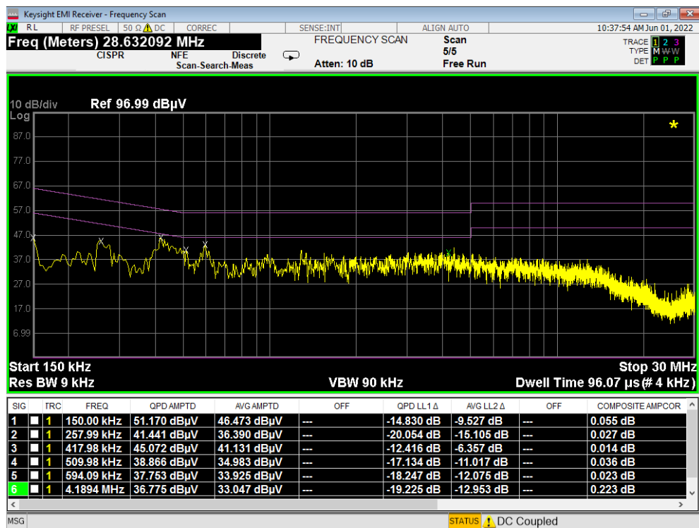
Plot 7-507. Line Conducted Plot with 802.11a UNII Band 2C (N) – Open
