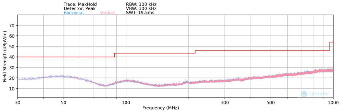
Plot 7-494. Radiated Spurious Plot below 1GHz (2.4GHz – 5GHz)
