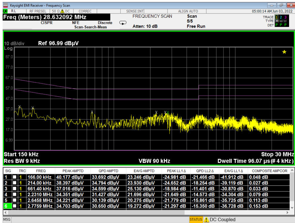
Plot 7-499. Line Conducted Plot with 802.11a UNII Band 1 (N) – Open
