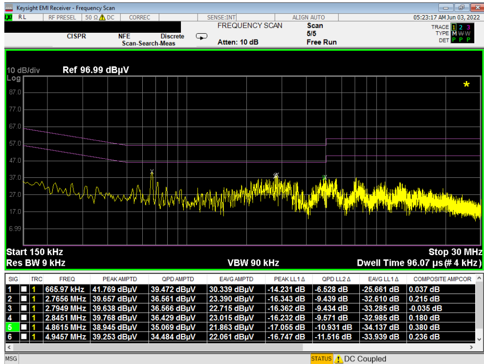
Plot 7-502. Line Conducted Plot with 802.11a UNII Band 2A (L1) – Closed
