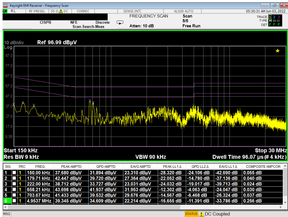
Plot 7-510. Line Conducted Plot with 802.11a UNII Band 3 (L1) – Closed
