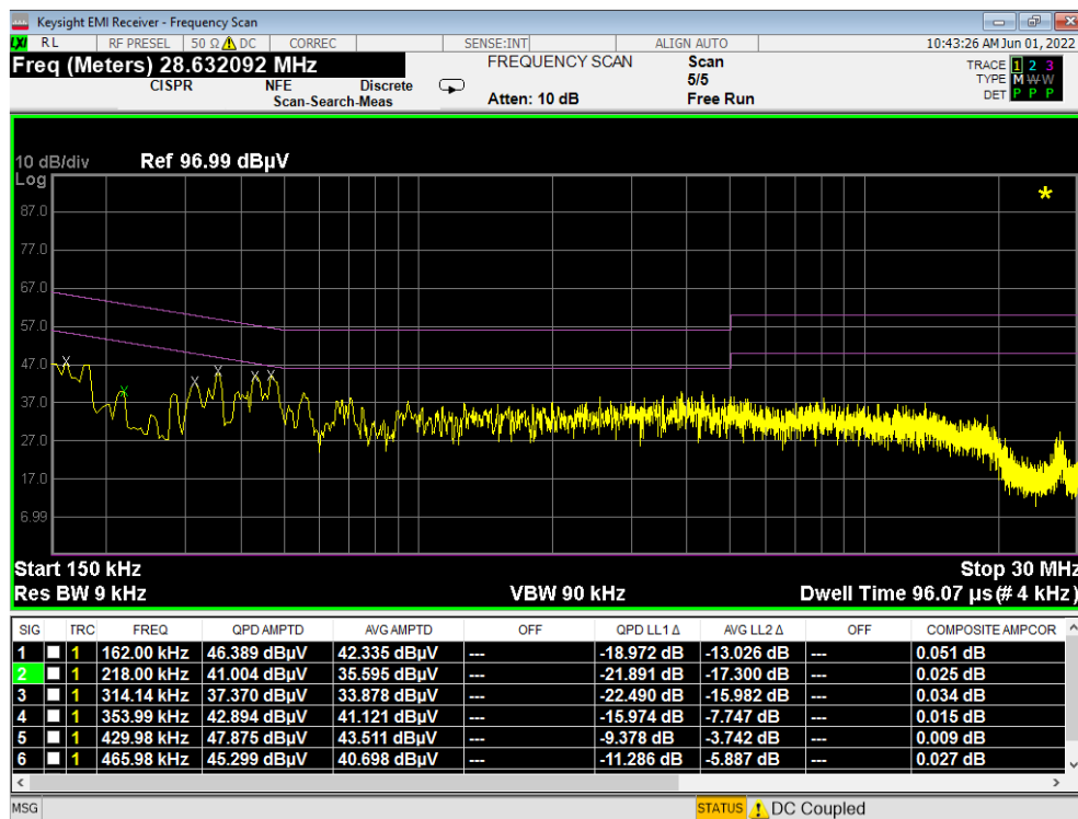
Plot 7-511. Line Conducted Plot with 802.11a UNII Band 3 (N) – Open
