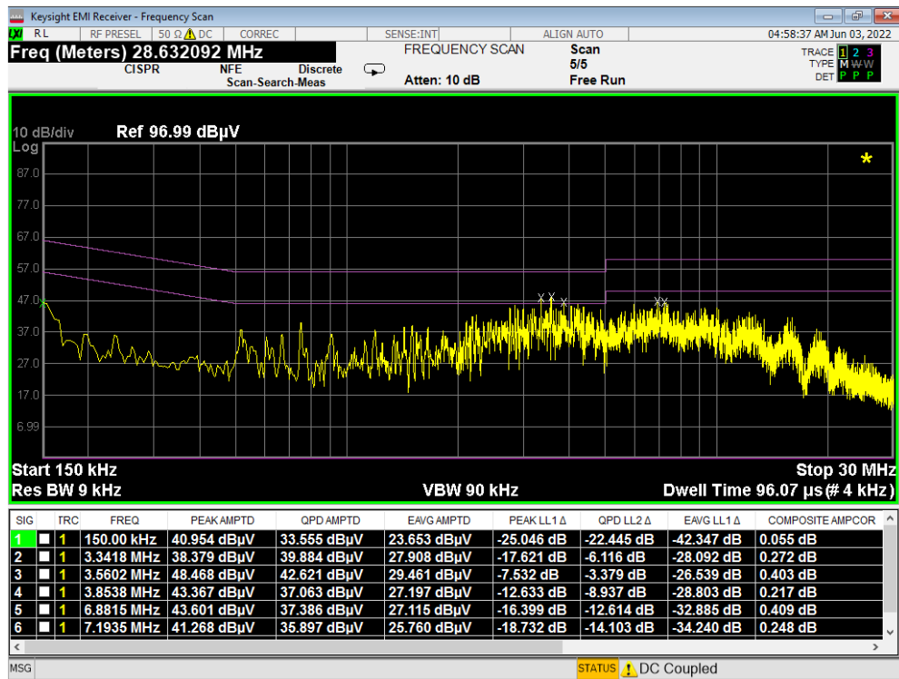
Plot 7-497. Line Conducted Plot with 802.11a UNII Band 1 (L1) – Open
