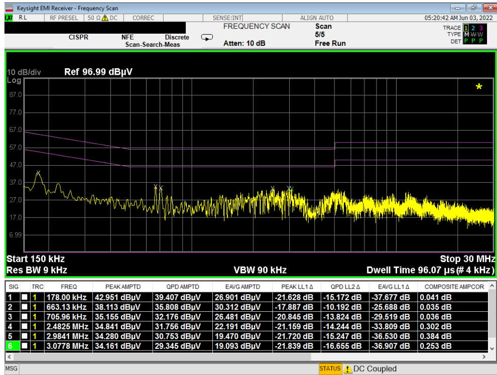
Plot 7-500. Line Conducted Plot with 802.11a UNII Band 1 (N) – Closed
