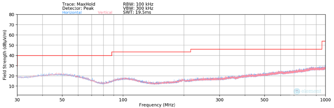
Plot 7-496. Radiated Spurious Plot below 1GHz (Dual Band Simult. Tx)
