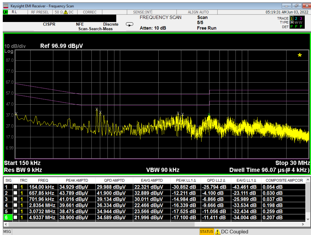
Plot 7-498. Line Conducted Plot with 802.11a UNII Band 1 (L1) – Closed
