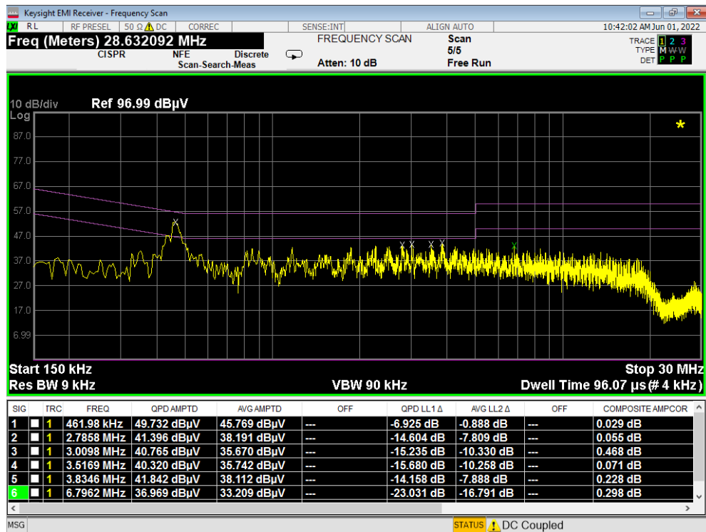
Plot 7-509. Line Conducted Plot with 802.11a UNII Band 3 (L1) – Open
