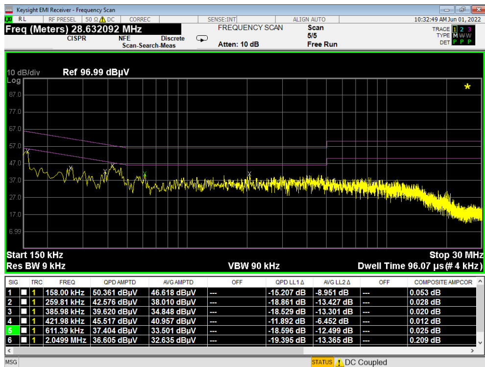
Plot 7-503. Line Conducted Plot with 802.11a UNII Band 2A (N) – Open
