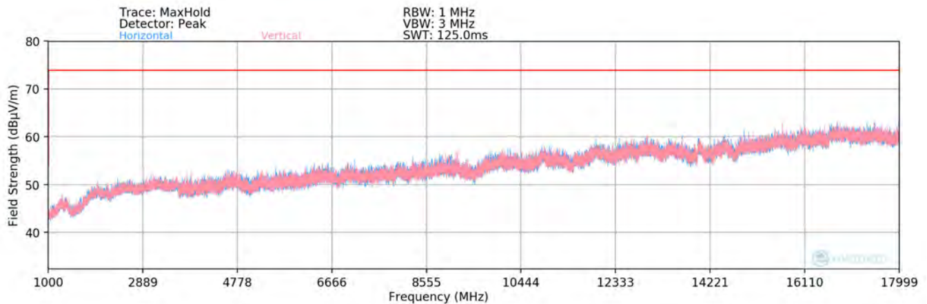
Plot 7-4. Radiated Spurious Plot above 1GHz [Radiated Test Config. 2]
