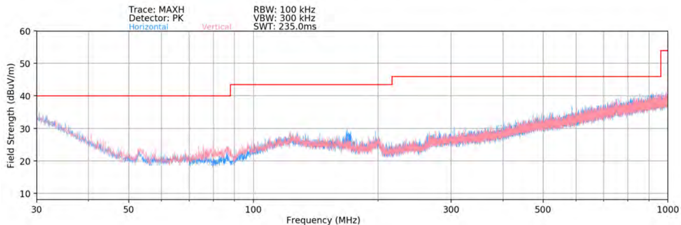
Plot 7-1. Radiated Spurious Plot below 1GHz [Radiated Test Config. 1]
