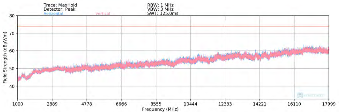
Plot 7-6. Radiated Spurious Plot above 1GHz [Radiated Test Config. 3]
