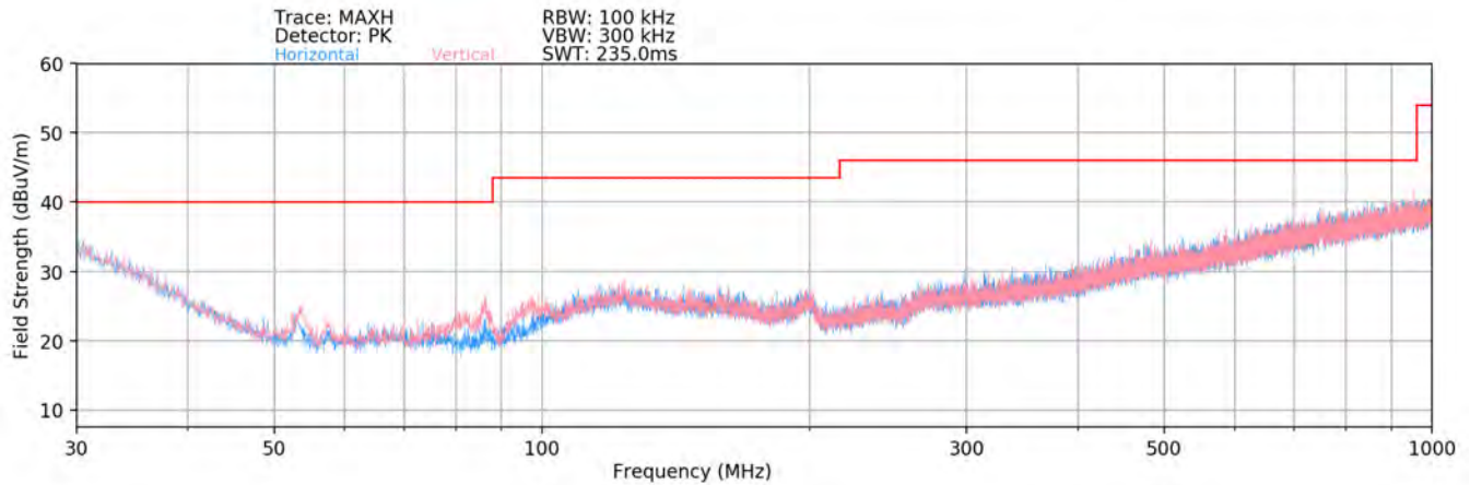
Plot 7-9. Radiated Spurious Plot below 1GHz [Radiated Test Config. 5]
