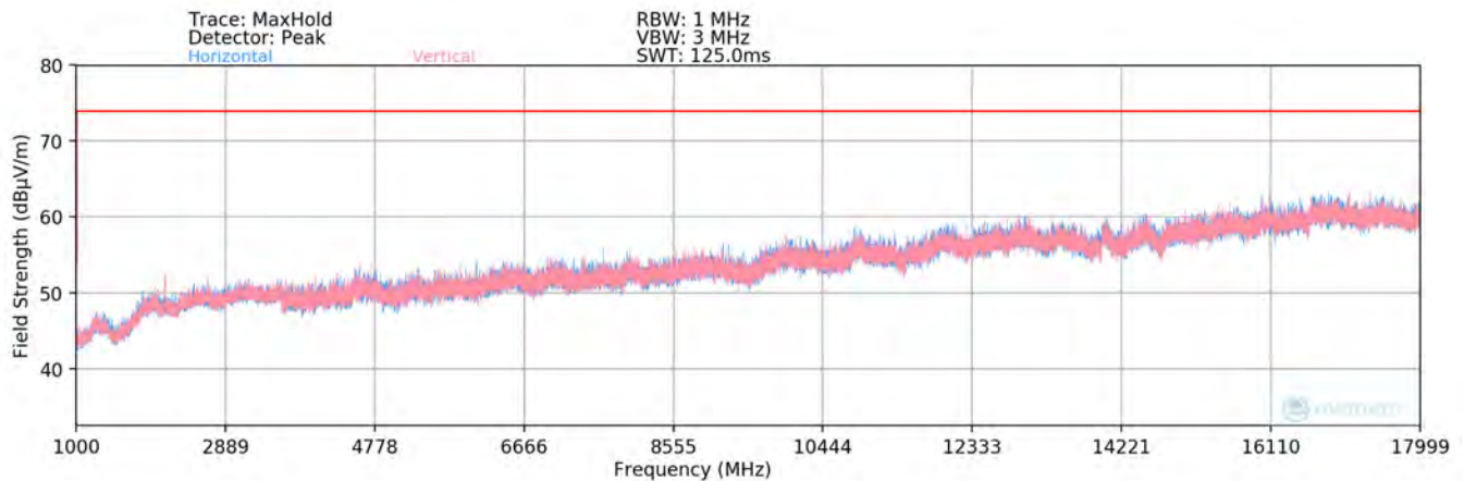
Plot 7-10. Radiated Spurious Plot above 1GHz [Radiated Test Config. 5]
