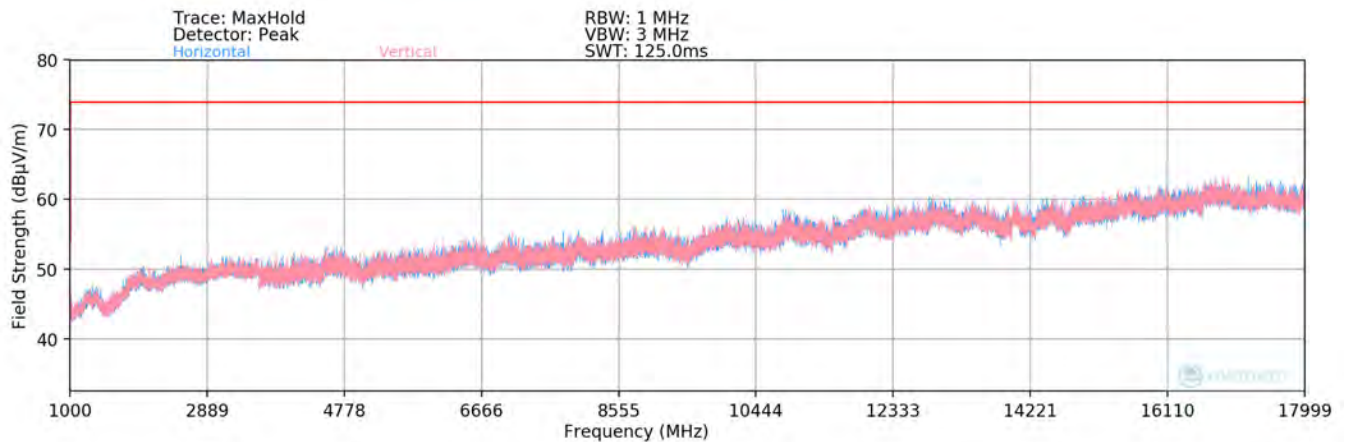
Plot 7-8. Radiated Spurious Plot above 1GHz [Radiated Test Config. 4]
