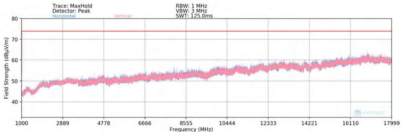
Plot 7-2. Radiated Spurious Plot above 1GHz [Radiated Test Config. 1]
