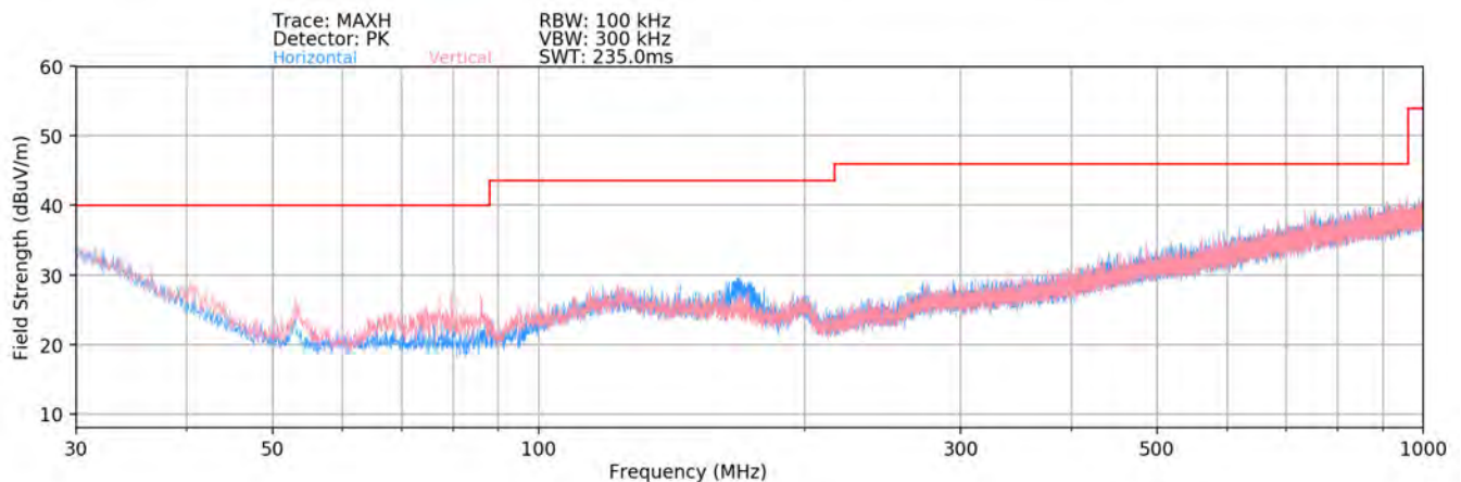
Plot 7-5. Radiated Spurious Plot below 1GHz [Radiated Test Config. 3]
