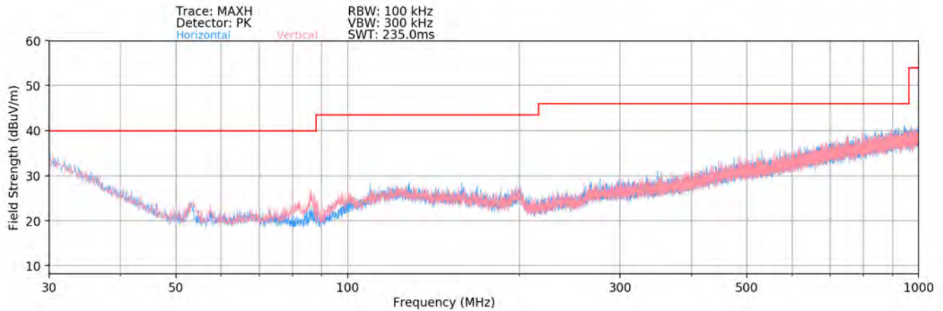
Plot 7-7. Radiated Spurious Plot below 1GHz [Radiated Test Config. 4]
