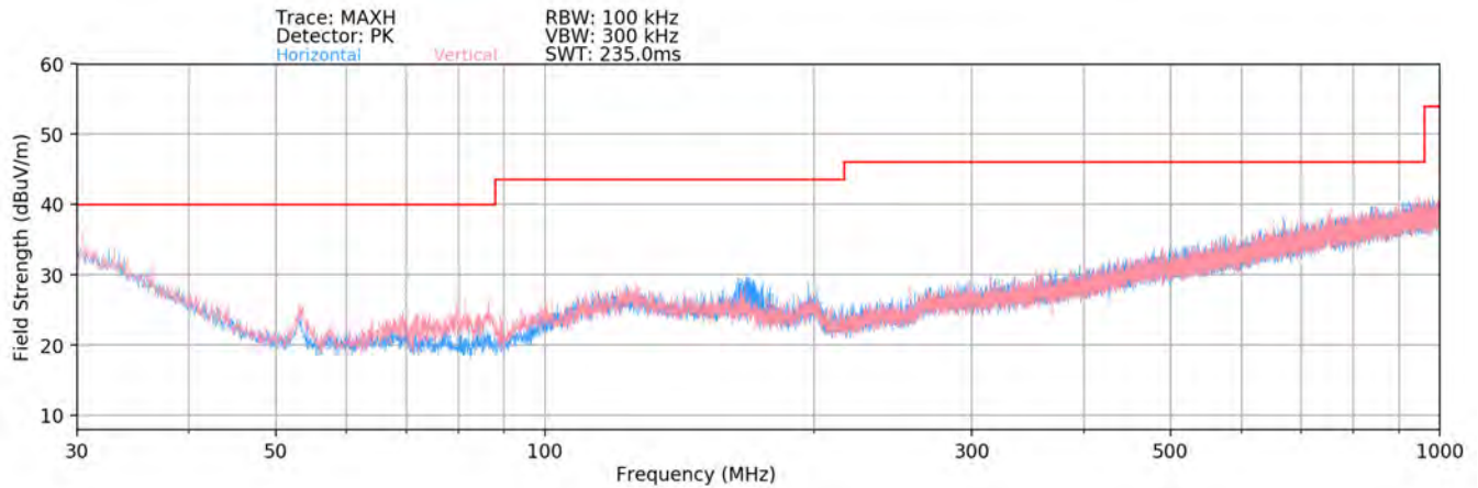
Plot 7-3. Radiated Spurious Plot below 1GHz [Radiated Test Config. 2]
