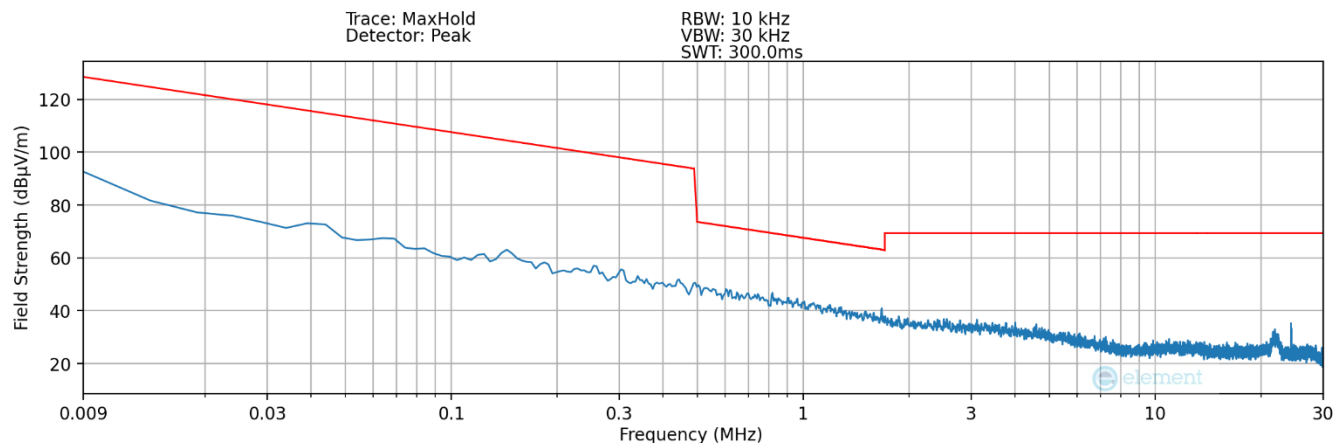
Plot 7-4. Radiated Spurious Plot 9kHz – 30MHz (Pol. X – Device to Device WPT) - Variant
