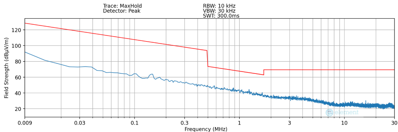
Plot 7-5. Radiated Spurious Plot 9kHz – 30MHz (Pol. Y – Device to Device WPT) - Variant
