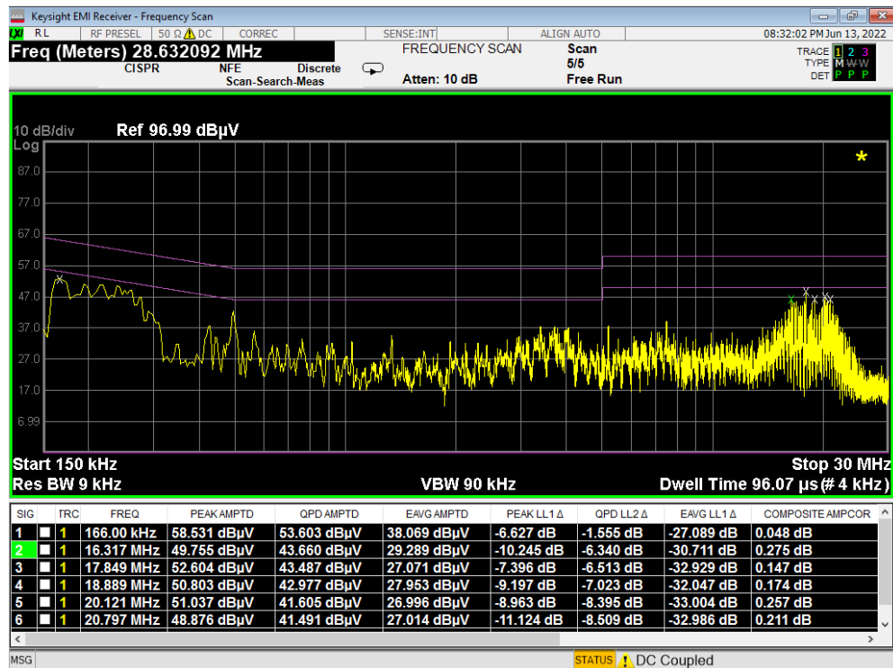
Plot 7-8. Line-Conducted Test Plot (N) - Device to Device WPT
