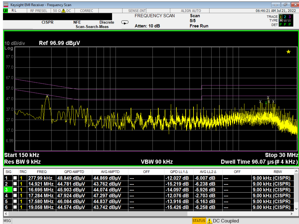
Plot 7-9. Line-Conducted Test Plot (L1) - Device to Device WPT - Variant
