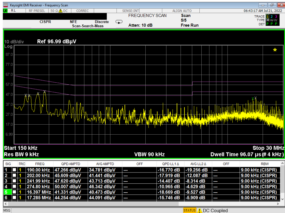
Plot 7-10. Line-Conducted Test Plot (N) - Device to Device WPT - Variant
