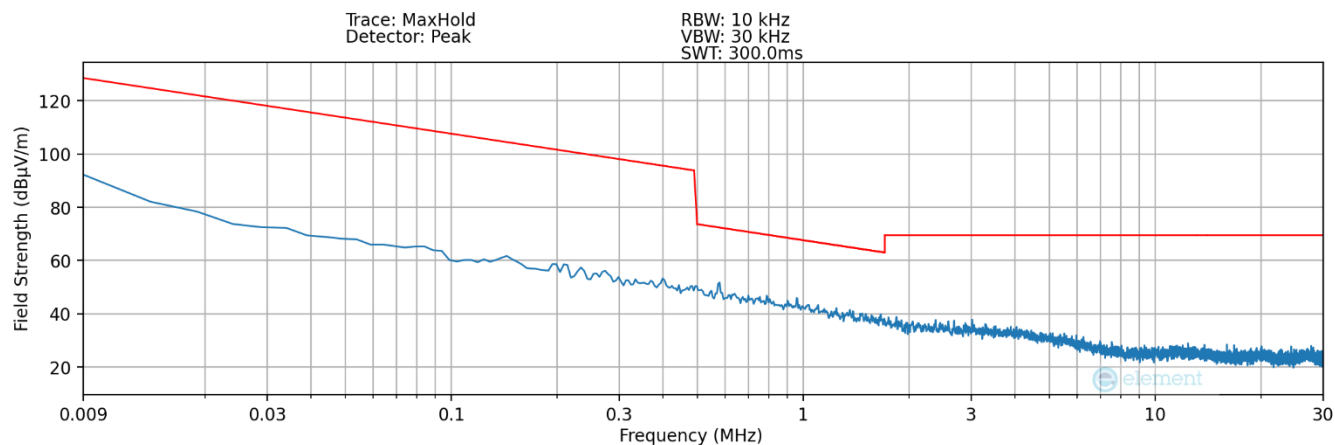
Plot 7-6. Radiated Spurious Plot 9kHz – 30MHz (Pol. Z – Device to Device WPT) - Variant
