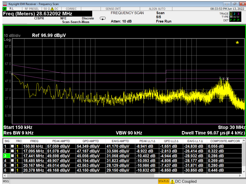
Plot 7-7. Line-Conducted Test Plot (L1) - Device to Device WPT
