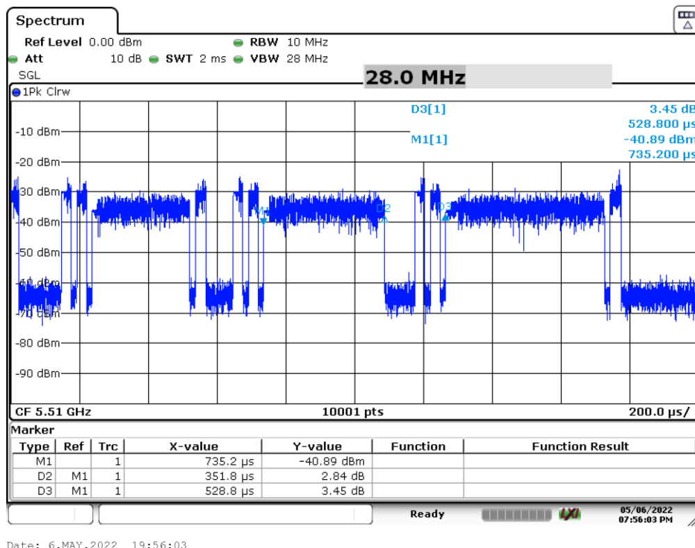
Figure 9-1. Band 2C Pulse Width and Period
