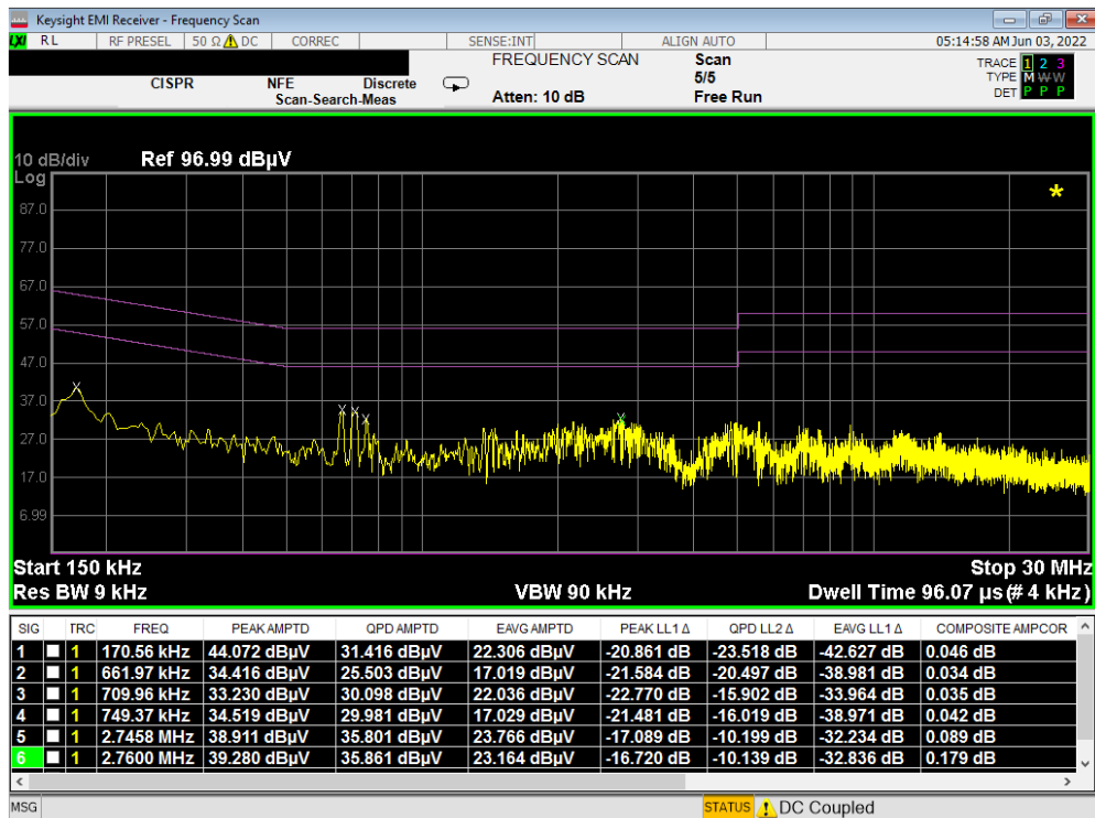
Plot 7-108. Line Conducted Plot with Bluetooth LE (N) - Closed
