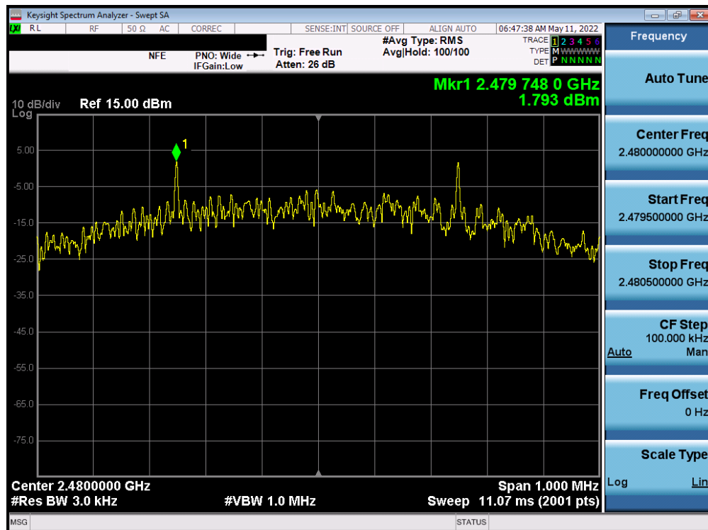
Plot 7-66. Power Spectral Density Plot (Bluetooth (LE), 500kbps – Ch. 39)
