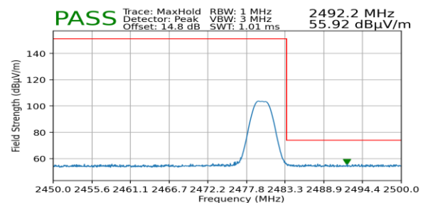
Plot 7-102. Radiated Restricted Upper Band Edge Measurement (Peak) – ANT 1
