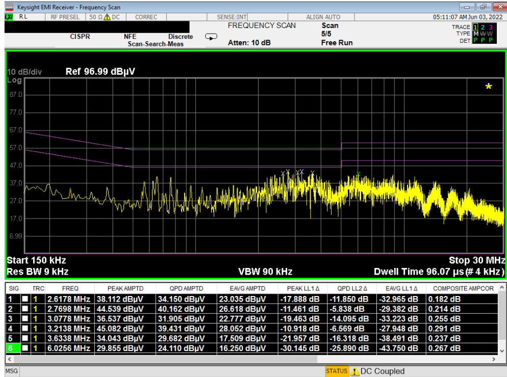
Plot 7-107. Line Conducted Plot with Bluetooth LE (L1) - Closed
