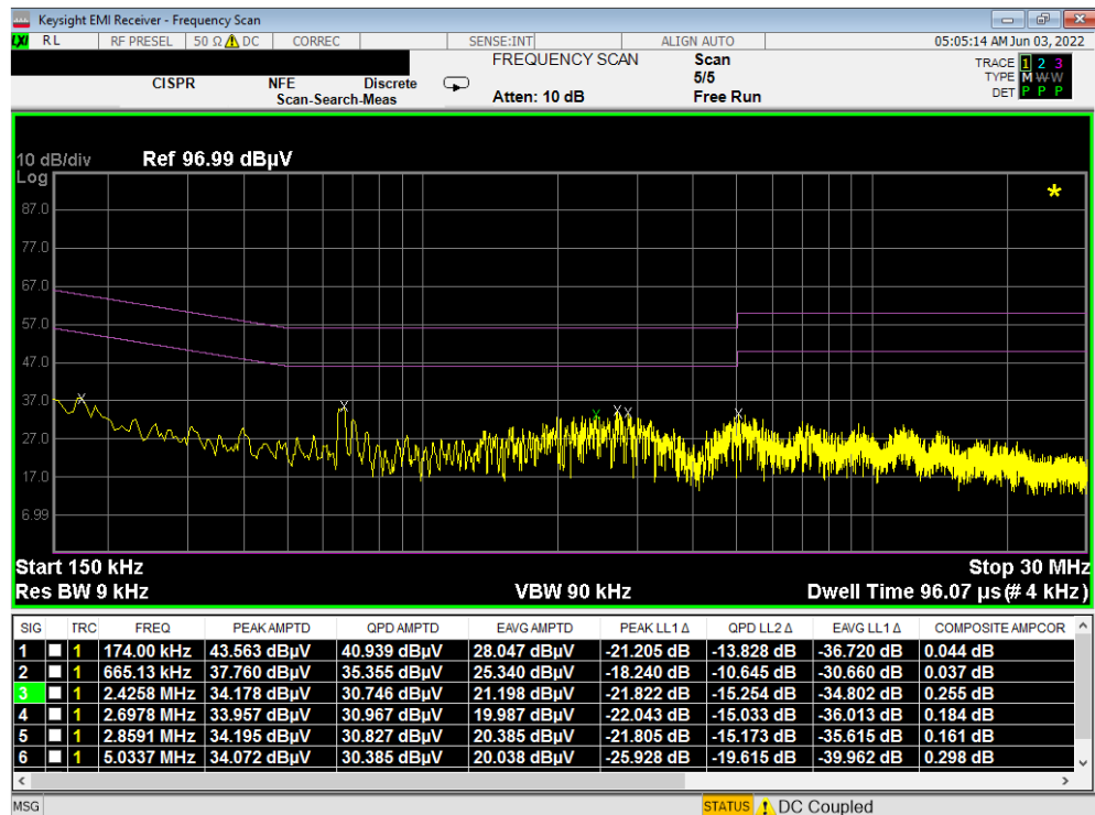
Plot 7-106. Line Conducted Plot with Bluetooth LE (N) – Open
