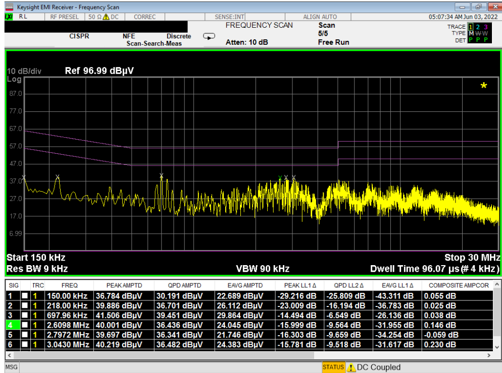
Plot 7-105. Line Conducted Plot with Bluetooth LE (L1) – Open
