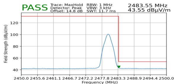
Plot 7-101. Radiated Restricted Upper Band Edge Measurement (Average) – ANT 1
