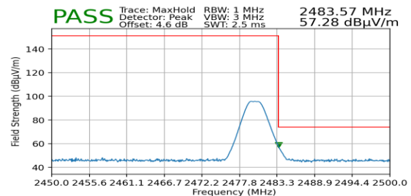
Plot 7-104. Radiated Restricted Upper Band Edge Measurement (Peak) – ANT 2
