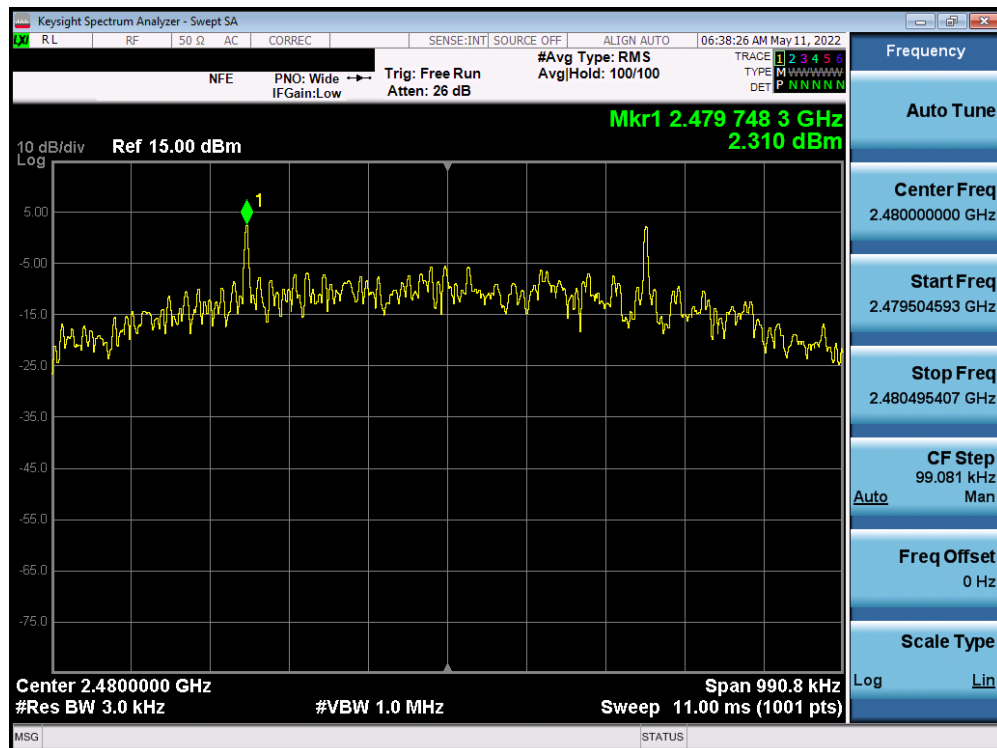
Plot 7-54. Power Spectral Density Plot (Bluetooth (LE), 500kbps – Ch. 39)
