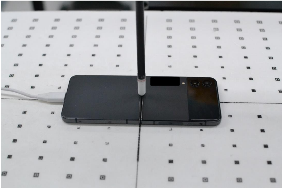
Test Setup Photo 3 – Folder Open, Back Side
