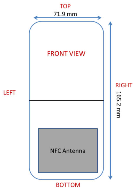
Figure J-2 NFC Antenna Locations Open Configuration
