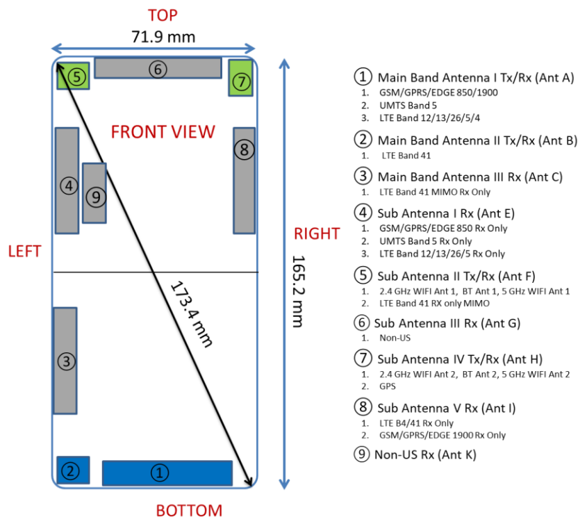
Figure J-1 DUT Antenna Locations Open Configuration
