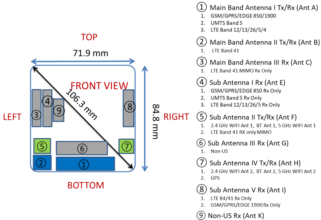
Figure J-1 DUT Antenna Locations Closed Configuration
