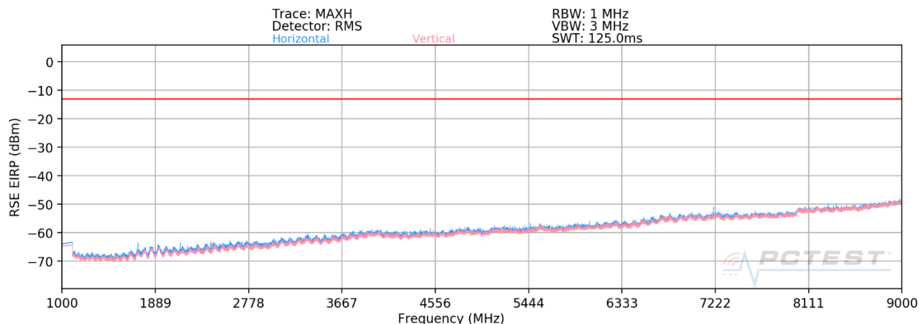
Plot 7-24. Radiated Spurious Plot Above 1GHz (LTE Band 26) – OPEN
