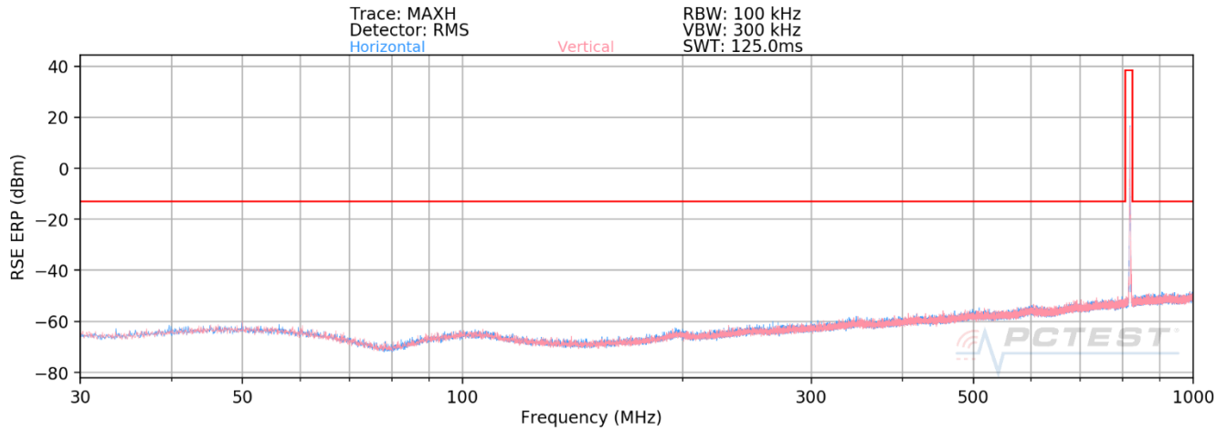
Plot 7-22. Radiated Spurious Plot Below 1GHz (LTE Band 26) – HALF OPEN
