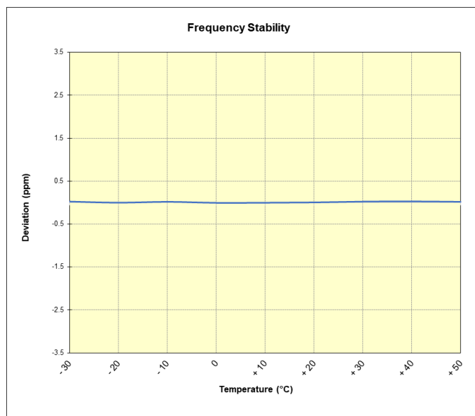
Plot 7-25. LTE Band 26 Frequency Stability Chart
