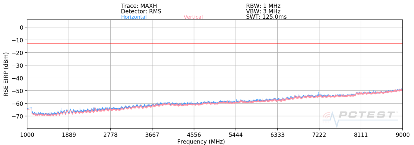
Plot 7-23. Radiated Spurious Plot Above 1GHz (LTE Band 26) – HALF OPEN
